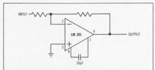
INVERTING AMPLIFIER
