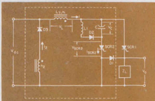
1. SCR swinging turn-off circuit to control power SCR1 is built with the components enclosed by the dashed lines. Load impedance has no effect on its operation.
