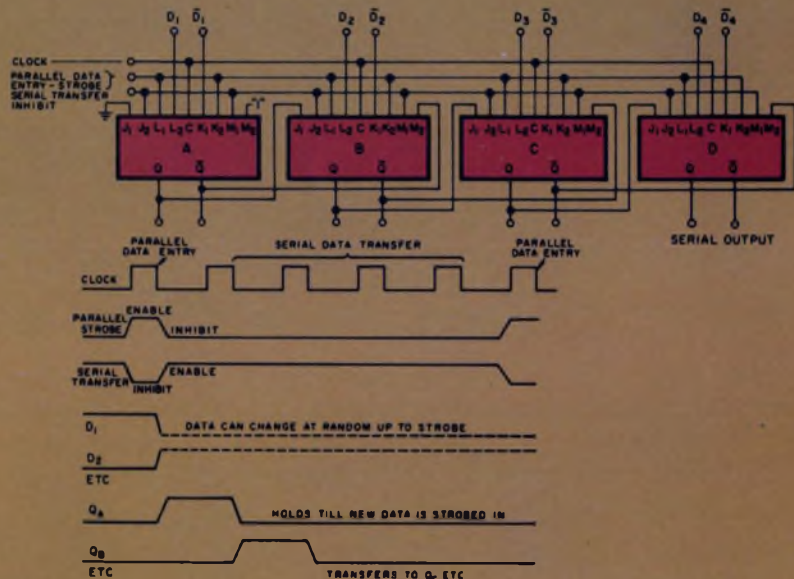
Fig. 5—In parallel to serial converter data is inserted through one set of 0Red inputs on each flip-flop.
