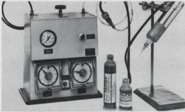
2. Extrusion-type automatic dispensing unit applies solder. The shot timer, Kenics model 500 SIFM, pulses air into the dispensing hopper. The dispenser, Pyles model 950-60X, is outfitted with a needle nozzle which dispenses solder in response to the pulses. Tubing is standard Polyflow plastic.
