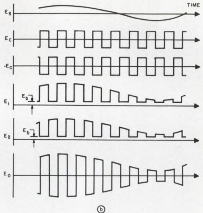
Amplitude modulated output, E_o , is obtained with the simple circuit (a). All waveforms on common time base are shown in (b).
