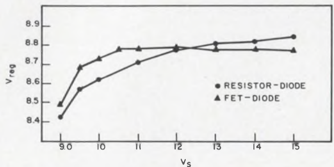
Stable voltage output results when a series resistor in a standard regulator circuit (a) is replaced by a suitable FET (b). The improvement is shown in (c).
