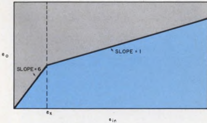
4. Duo-gain characteristic shows small-signal gain = 6 ( e_{in} < e_x ) and large-signal gain = 1 ( e_{in} > e_x ). e_x is the voltage across R_x .
