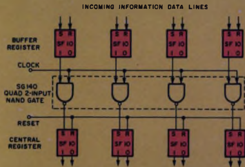
Fig. 1—Flip-flop register application.
