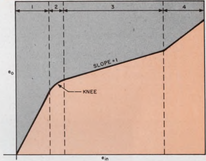
1. The basic circuit for a tunnel-diode log-amp stage (top) produces duo-gain characteristics (bottom). The circuit exploits regions 1 and 3. Region 2, the curve's knee, is minimized by selection of R_x . Region 4 is not used.
