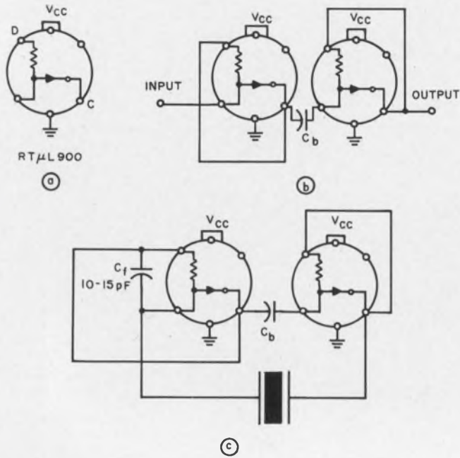
Crystal-controlled oscillator uses only two discrete capacitors in addition to the crystal.
