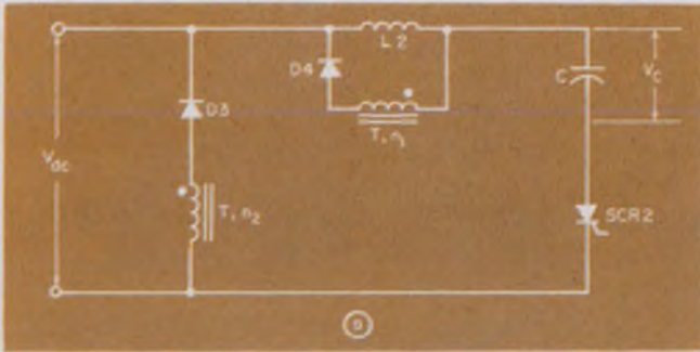
3. The active portion of the circuit of Fig. 2 is shown in (a). Its equivalent circuit appears in (b).
