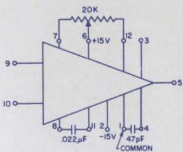
FREQUENCY COMPENSATION CIRCUIT FOR 6 dB/OCTAVE ROLLOFF (Ref: Note 2) FIGURE 3
