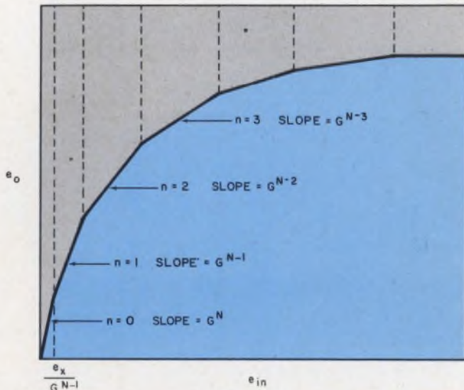
5. Cascading many stages yields an amplifier with a linear response for small signals and a logarithmic response for large signals.
