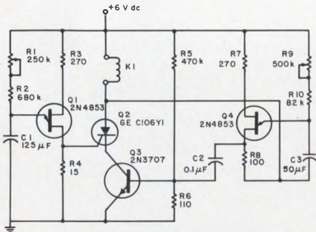
Very slow astable multivibrator uses separate timing circuits, Q1 and Q4, to turn the relay K1 on and off. Both the frequency and duty cycle can be varied independently.
