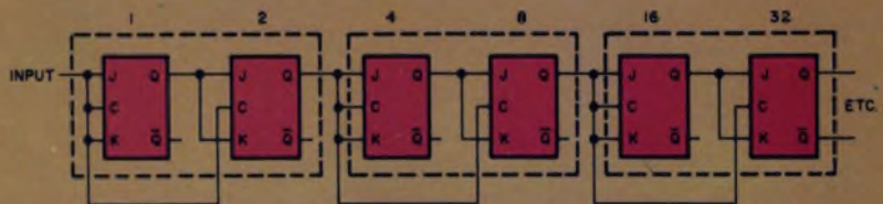
Fig. 7—Semi-ripple counter employs dual J-Ks with common clock.
