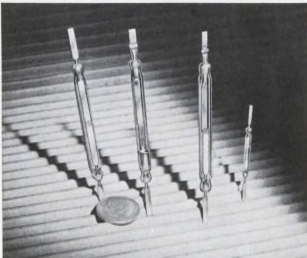
Left to right: General Purpose, Mercury-Wetted, High Voltage, MicroClareed
