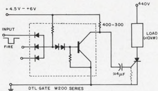
SCR firing circuit uses single IC and two discrete components.
