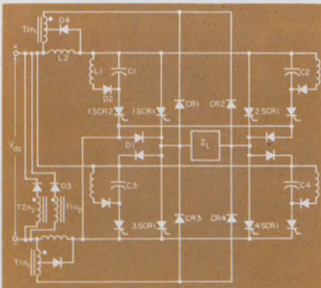
4. Simplified schematic of a 1.5-kVA inverter using the swinging turn-off circuit is shown without high-voltage suppressing and balancing networks. SCR1s form a bridge to provide a square-wave voltage across the load Z_L . Turn-off circuit for 1SCR1 consists of L1 , D2 , C1 , 1SCR2, D1 , D3 , T1 , L2 , D4 . CR1 , CR2 , CR3 , CR4 provide current paths to discharge inductive loads into supply. See box for the component values.
