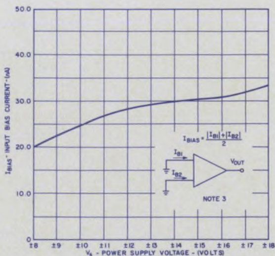
INPUT BIAS CURRENT VS POWER SUPPLY VOLTAGE
