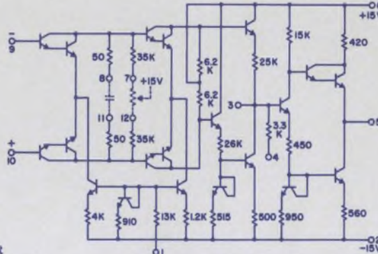
CIRCUIT DIAGRAM FIGURE 4
