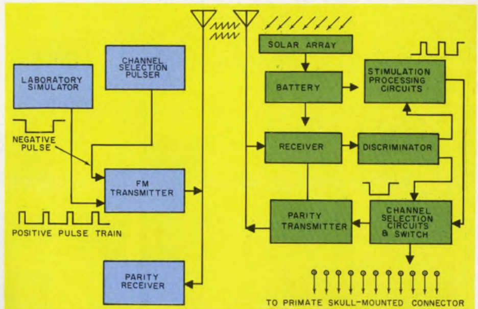
1. General Electric Mark II telestimulator permits remote stimulation of more than one monkey in outdoor primate colony. Miniaturized switch steps output pulses through 11 electrodes.
