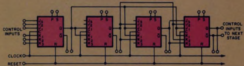
Fig. 4—Synchronous binary counter takes advantage of multiple J and K Inputs.
