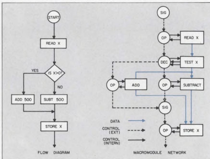
Macromodule concept (circles and blocks above) permits flow diagram (left) to be translated easily into a hardware data-processing network (right).
