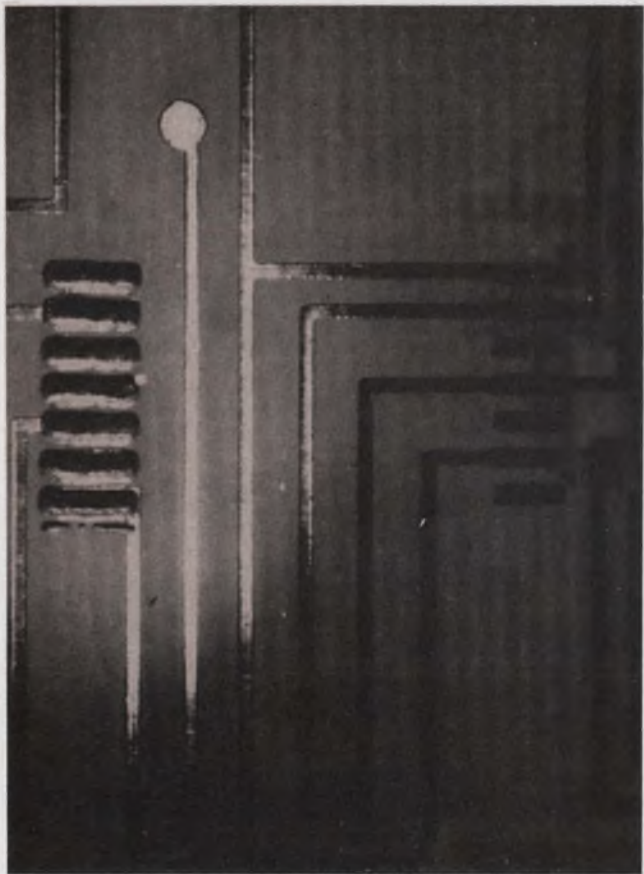
3. Two methods for joining flat packs to PC boards. On the flat pack above, solder cream is directly applied to the leads. On the board below, solder cream is deposited straight onto the bonding pads.
