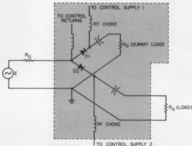
1. Basic attenuator circuit is built around two RF diodes. Both the generator and load impedances are assumed to be equal to R_0 . The diodes are pin type and have resistive impedances through their bias range. The attenuation is continuously variable through the bias of the diodes, which varies their impedances from about 0.5 to 5000 ohms.
