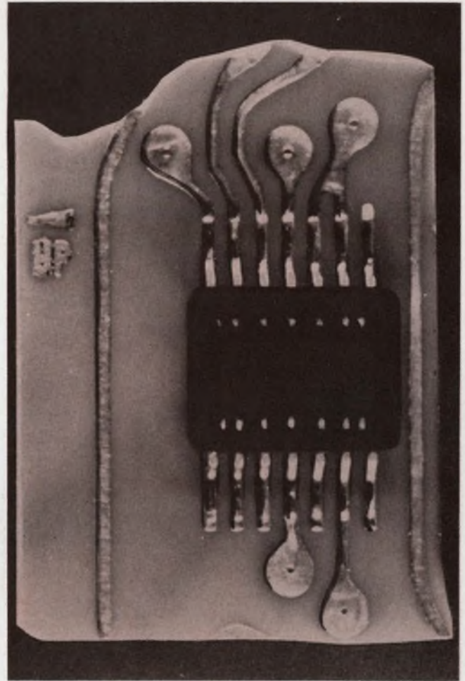
4. Completed assembly using solder cream on the bonding pads. Note the absence of bridging.
