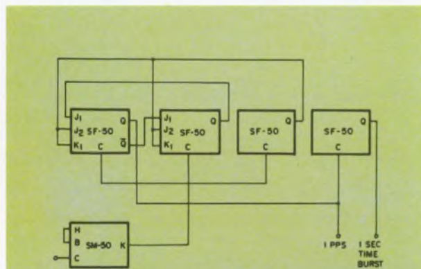
Fig. 1—Simple, accurate 1-Hertz generator using SUHL ICs.
