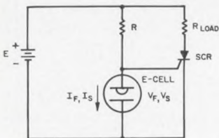
1. Basic timing circuit requires resistor and SCR. V_F is voltage in timing condition, V_S afterward. The max forward current I_F must exceed sum of stop current, I_S , and threshold current to fire SCR gate.
