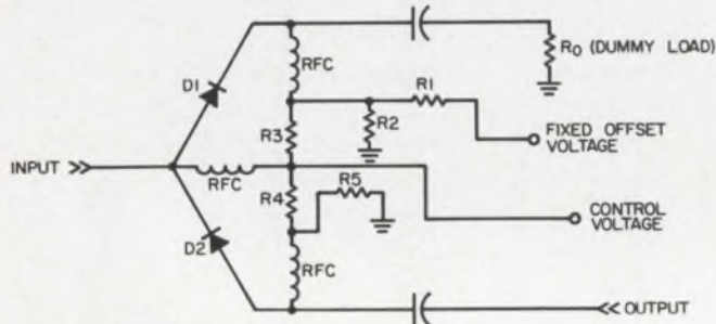
4. A single control source may bias both diodes if one of the diodes is reversed. Here diode D2 is reversed with respect to its original direction in Fig. 1.
