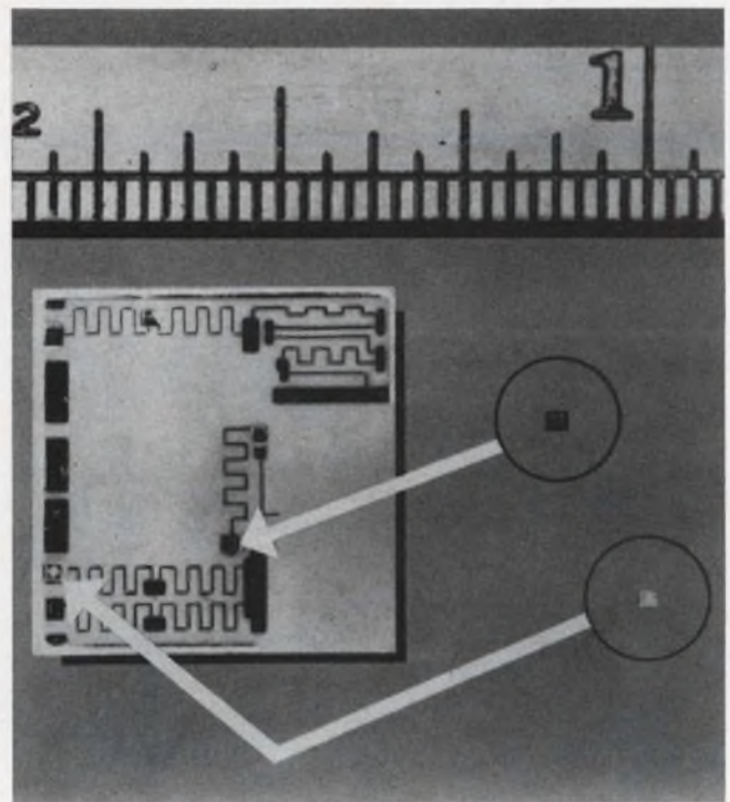
6. Active devices joined to a hybrid microcircuit. The same soldering techniques as for flat packs may be used.
