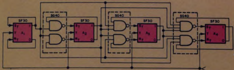
Fig. 3—Synchronous binary counter with SRT flip-flops.
