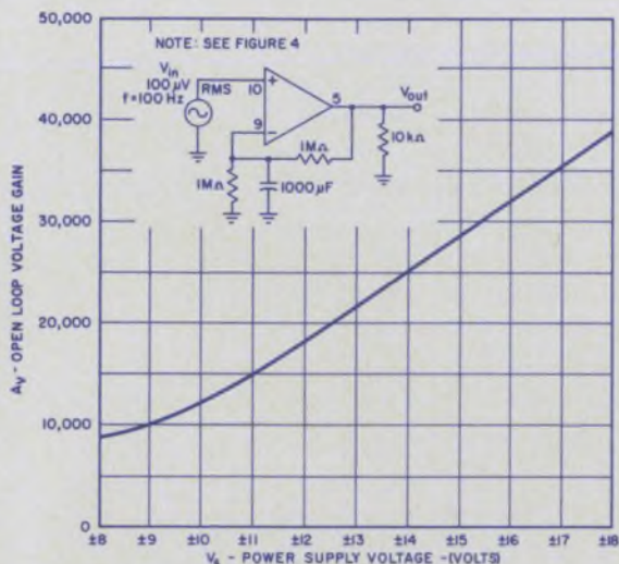
OPEN LOOP VOLTAGE GAIN VS POWER SUPPLY VOLTAGE
