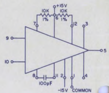
STANDARD TEST CIRCUIT (Ref: Note 3) FIGURE 5
