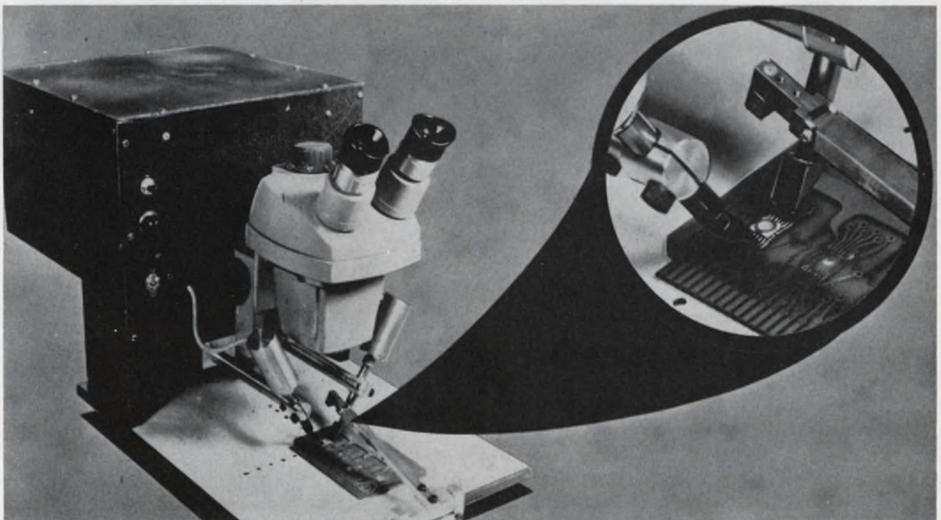
5. Typical resistance soldering setup. A Weller Electric Corp. unit is used. Soldering temperature is about 100°F
