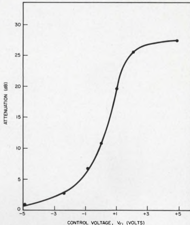
6. Measured variation of continuously variable attenuation with control voltage V_{C1} shows rapid control. The switching time of the device over the entire attenuation range is less than 300 ns.
