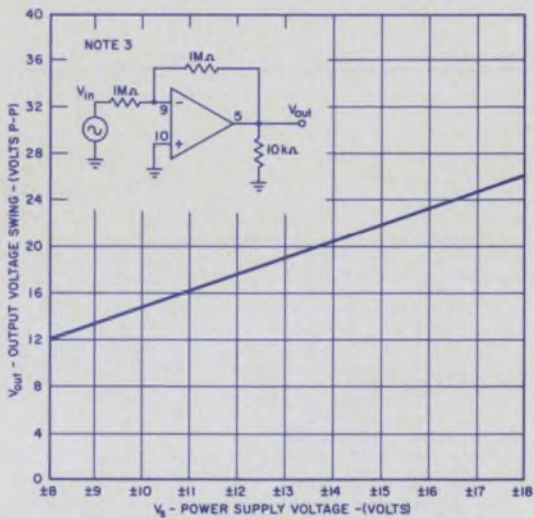
OUTPUT VOLTAGE SWING VS POWER SUPPLY VOLTAGE
