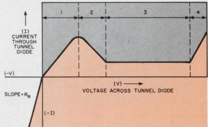
3. Four approximately linear regions make up the characteristic curve of a tunnel diode.
