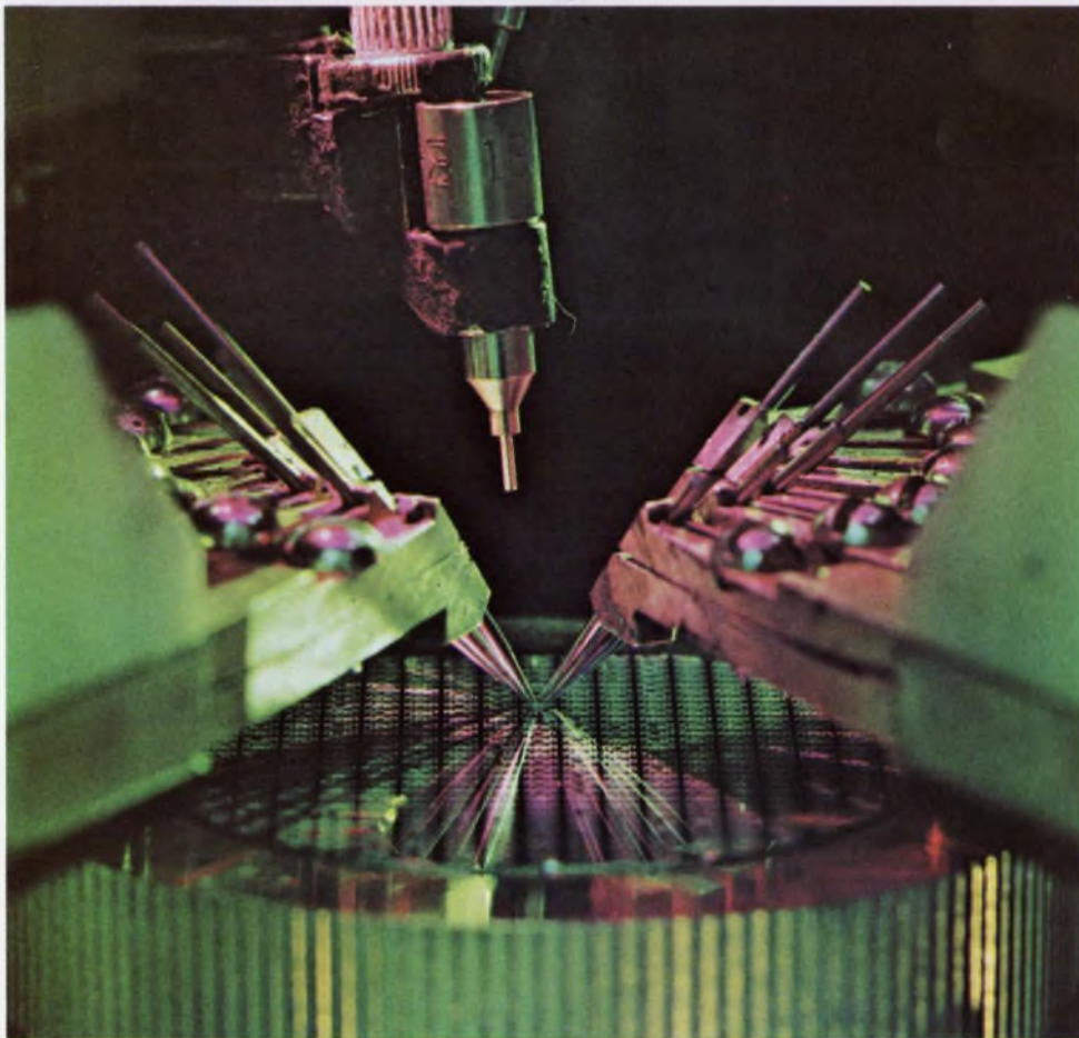
Mechanized wafer-level testing with this 14-point probe.
