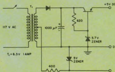
Fig. 2—Power source for low-frequency generator.
