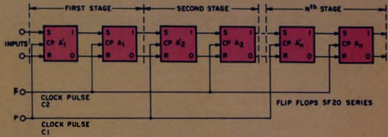
Fig. 2—Shift register—dual rank.
