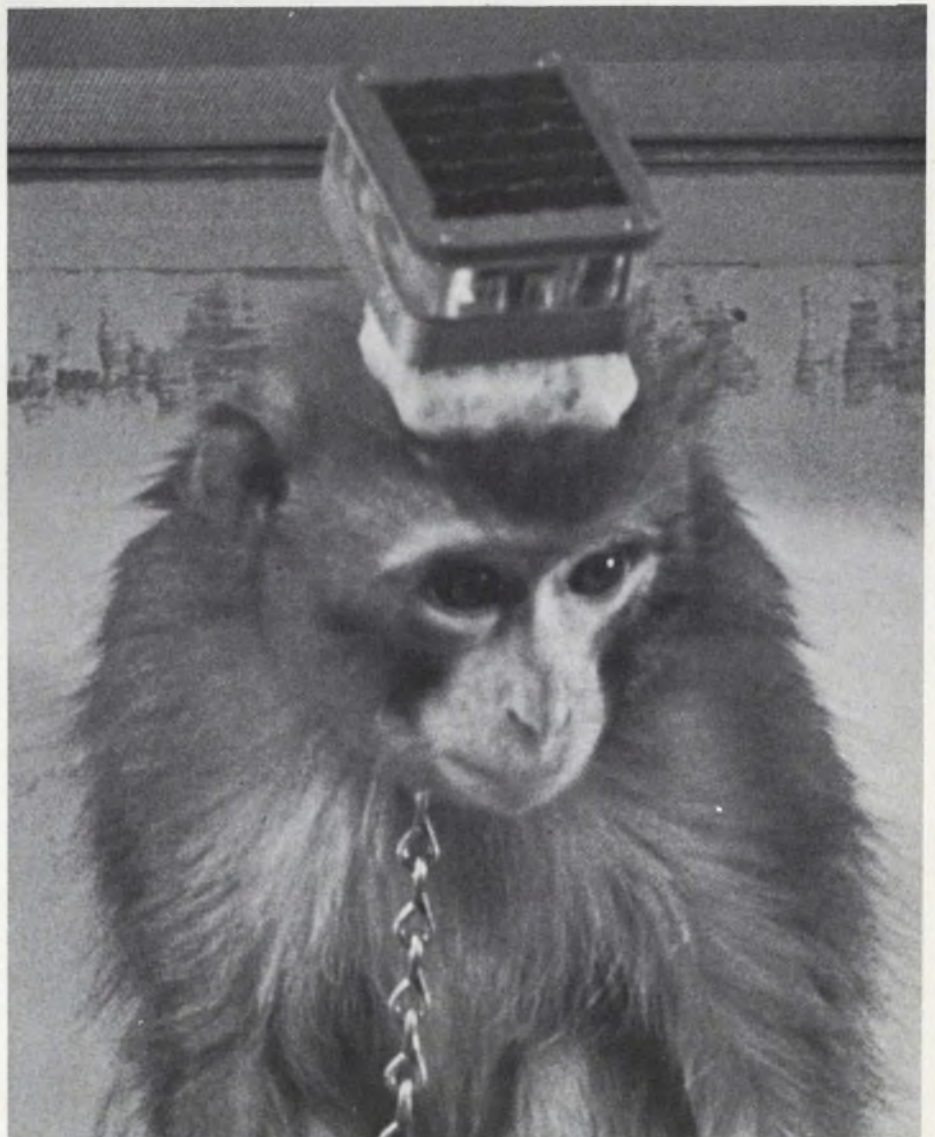
Solar array powers receiver-stimulator developed by General Electric Co. for Dr. Bryan Robinson. Head-mounted unit weighs 200 grams and measures 7 x 6 x 3 cm.
