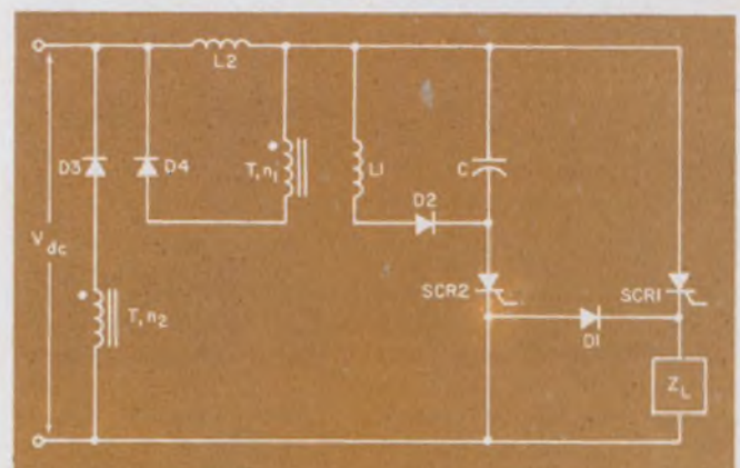
2. High voltages across diode D_3 can be avoided by modifying the basic turn-off circuit of Fig. 1; diode D_4 was added and the components were slightly rearranged.
