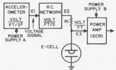
3. Double-integration function is performed as E-cell provides a signal source which indicates the distance from the voltage output of an accelerometer. Uses are in airborne cargo drops or ordnance.
