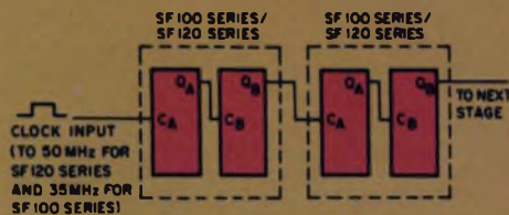
Fig. 6—High-speed ripple counter can be clocked at up to 50 MHz.
