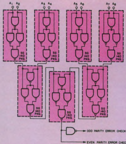
Fig. 3—Parity checking for 8-bit binary word which includes the parity bit.
