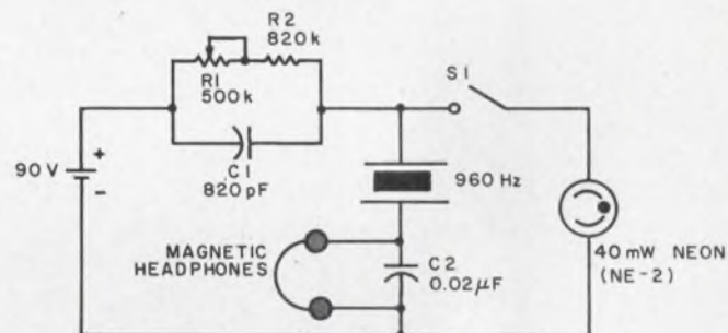
Versatile relaxation oscillator results when a neon bulb is combined with an audio crystal.
