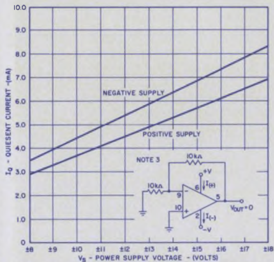
QUIESCENT CURRENT VS POWER SUPPLY VOLTAGE
