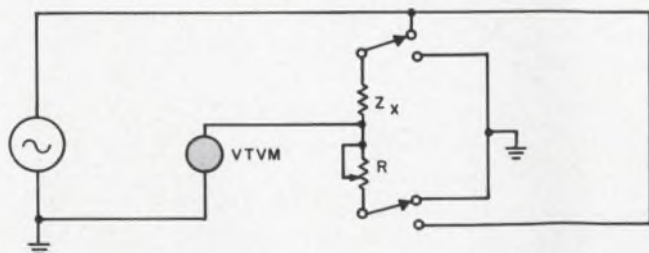
Real part of Z is determined by adjusting R until voltages across Z_x and R are equal. The value is then read off the dial of the decade box, R .
