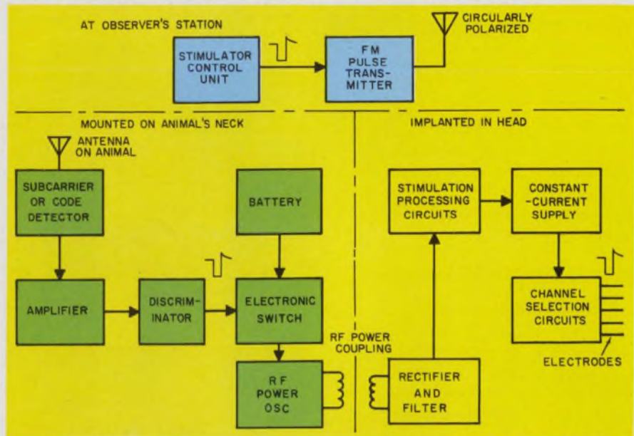
2. Microminiaturized implantable stimulator would draw power from electronics pack mounted on animal without using leads that pierce the scalp. Integrated circuits and biological power source might permit implantation of receiver and antenna as well.
