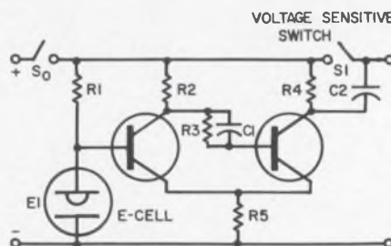
2. Fixed time-delay circuit uses an E-cell to fire Schmitt trigger. When S_0 closes, the charged cell starts timing. When it is timed out, its voltage rises, firing the Schmitt circuit at 0.5 V. This fires S_1 through C_2 .
