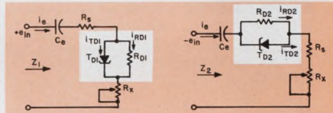
2. Equivalent circuits for the tunnel-diode-resistor network show positive excursions of the input (left) and negative excursions (right).
