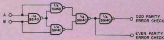
Fig. 2—ODD/EVEN parity checking for two bits.
