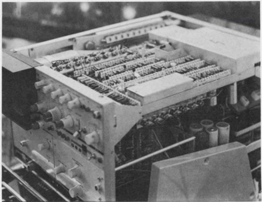
Interior of a Polish 60-MHz oscilloscope shows the large components and side-by-side packaging used. The OSA601 has passive devices suspended between two ceramic strips with slots for the leads to be soldered into.
