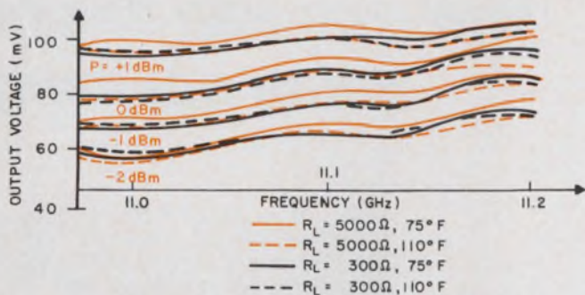
11. The detected output voltage changes with the load resistor (solid lines) and with temperature (dashed lines). Higher power levels increase the negative effect of T_c .
