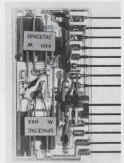
Flip-flop draws 150 \mu W 126
