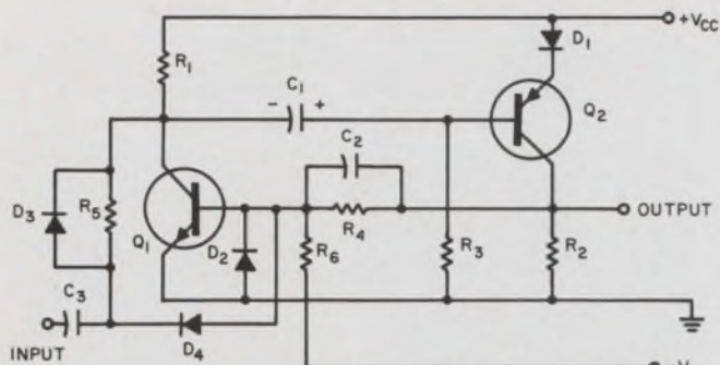
3. In a complementary monostable multivibrator both Q_1 and Q_2 are normally on.
