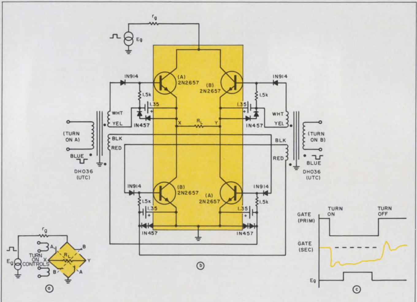
Switch-bridge controls direction of load drive (a). Complete circuit (b) is used with ungrounded loads as a bi-directional
