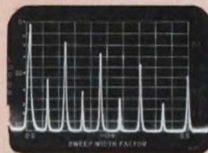
Harmonic analysis of distorted sine wave. 40 db log amplitude scale used.
