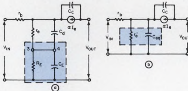
6. The design technique may be extended into another realm of Class A operation, by adding an appropriate RC network between nodes 3 and 4 (a). Because R_E C_E = r_e C_d , a simpler equivalent circuit (b) results.
