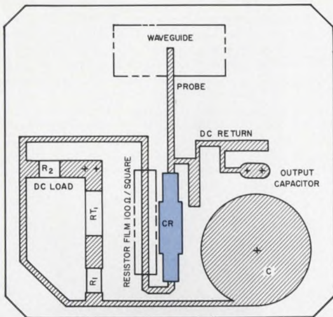
5. Stripline detector mount eliminates the critical mounting problems of the diode encountered in waveguide mounts. This mount, when combined with a tuned probe, makes the backward diode a high-quality detector. RT_1 , a temperature-sensitive resistor, is usually not needed.
