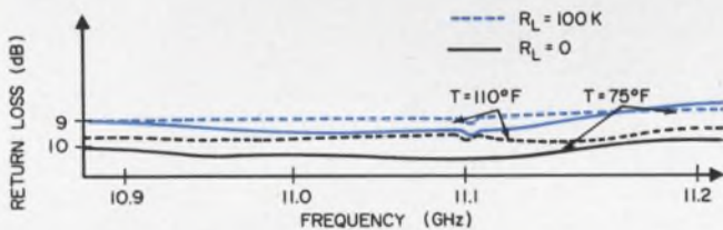
6. Return loss of the stripline mount remains fairly constant over a 200 MHz band that centers around 11.1 GHz. A matched load (solid black line) reduces the return loss by about 1 dB. The increase in temperature also reduces the return loss.
