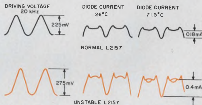
13. Gross temperature instability may occur in some backward diode. It appears as a double trace in the output current that changes the average current.
