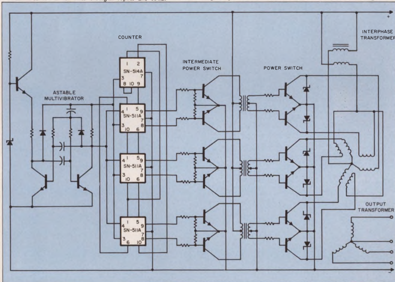
4. Over-all schematic of the three-phase inverter. The final volume of the inverter package is only 60 cubic inches.
