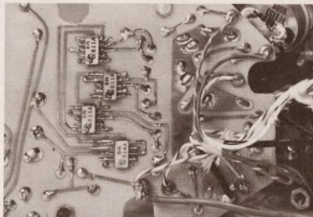
2. The integrated circuits are soldered to the printed-circuit board. Their flat shape simplifies the mechanical packaging problem.
