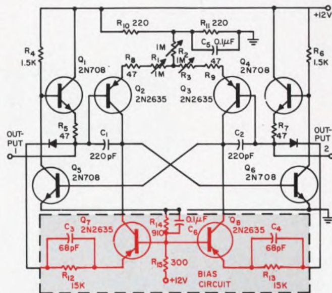
7. Linear improvement in the wide-range astable multi is achieved by adding four more transistors.
