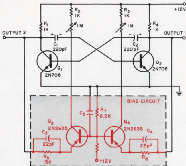
6. Wide-range astable multi uses two transistors for constant biasing.
