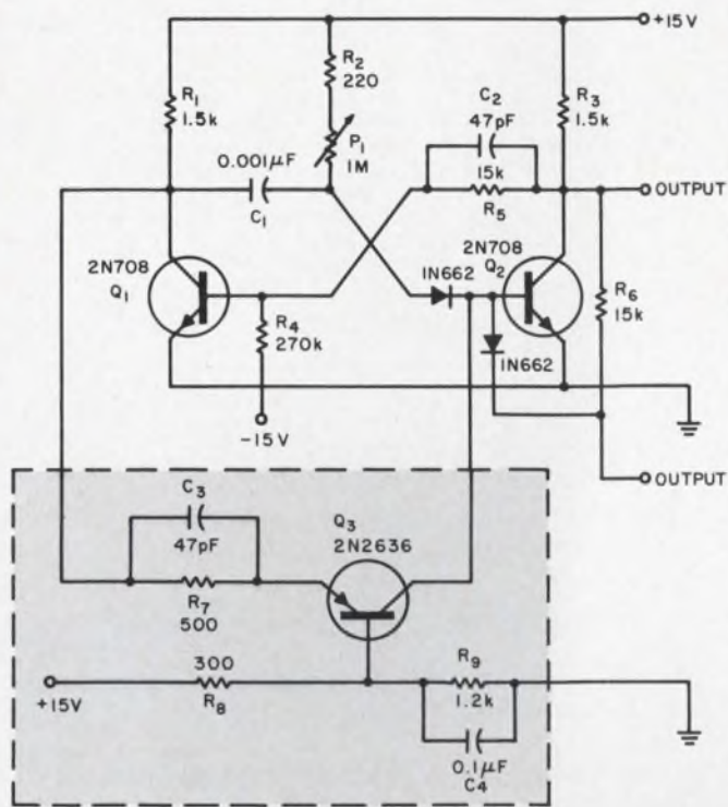
1. Monostable multi adjusts its timing by varying potentiometer P_1 . But this also affects biasing. Adding the bias circuit allows the resistor combination of R_2 and P_1 to be used for timing only. Range goes from 1 to 200 \mu s.
