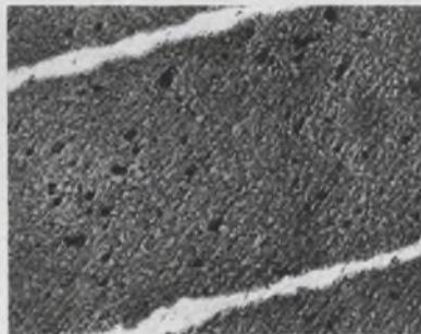
Dielectric of a second make of conventional CK ceramic
