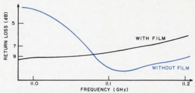
7. Resistive film over the dc path has a critical effect on the amount of reflected RF energy and therefore on the vswr of the mount. Measurements again were taken in a 200 MHz band around 11.1 GHz.
