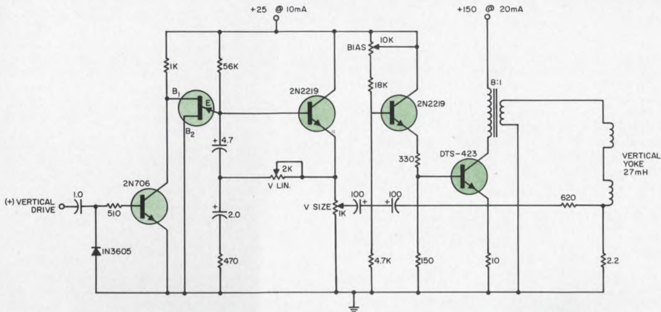
1. Efficiency and linearity result when high-voltage transistors and a UJT are used in this deflection amplifier.
