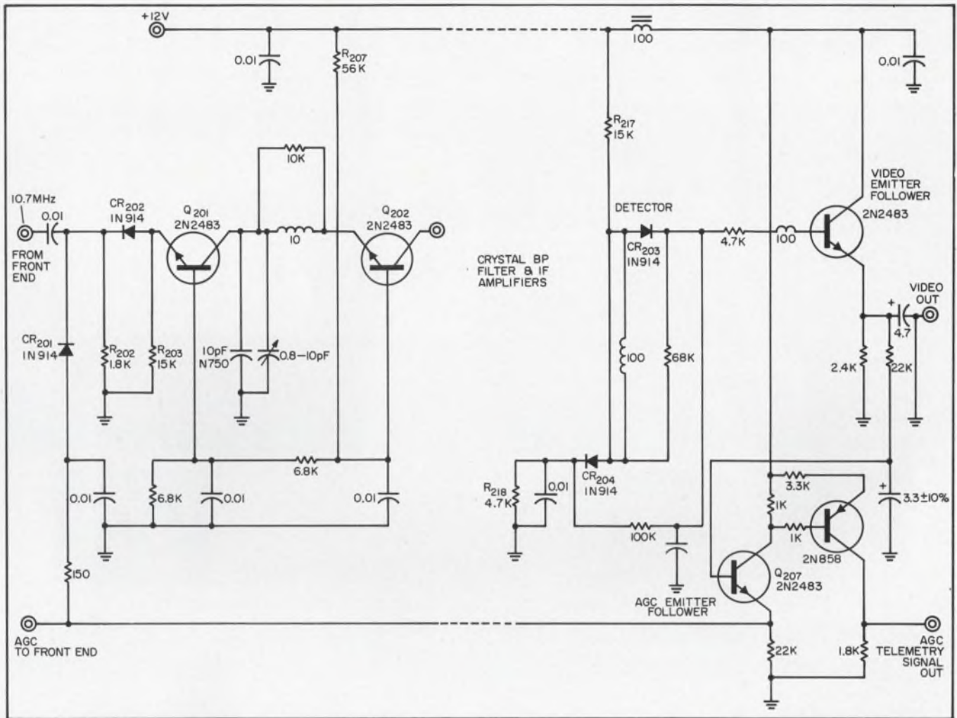
2. Agc voltage is derived directly from the AM detector through the agc emitter follower Q_{207} .
