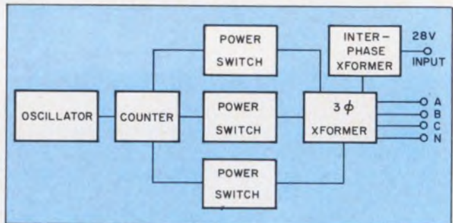
1. Three-phase inverter uses four IC packages and 15 transistors. The power-switch block includes two transistor switches in parallel.
