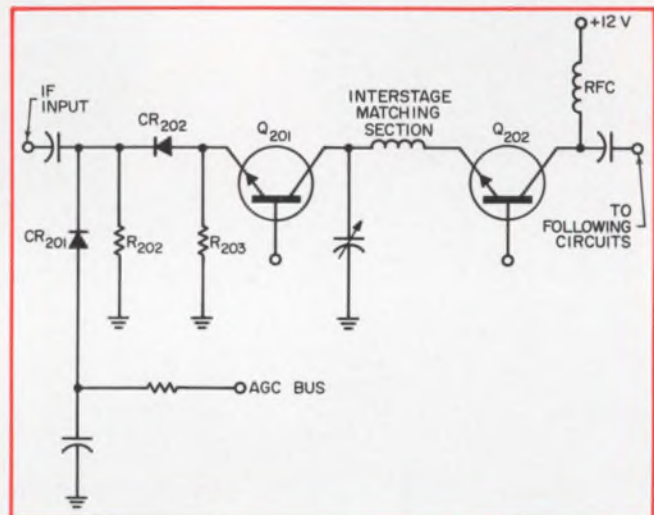
1. Basic agc circuit uses combination of reverse agc and diodes in series and parallel with the signal path.
