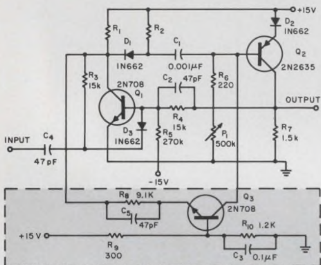
4. Wide-range technique can also be applied to the complementary monostable multi.
