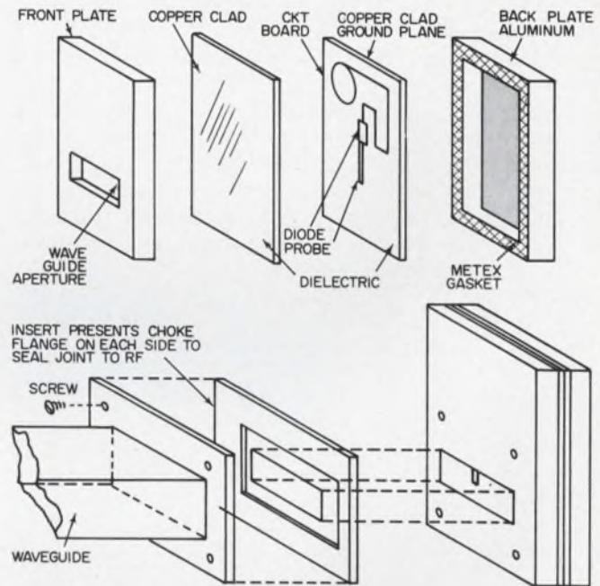
8. A sketch of the mount shows how it is constructed and how it fits on the waveguide flange.
