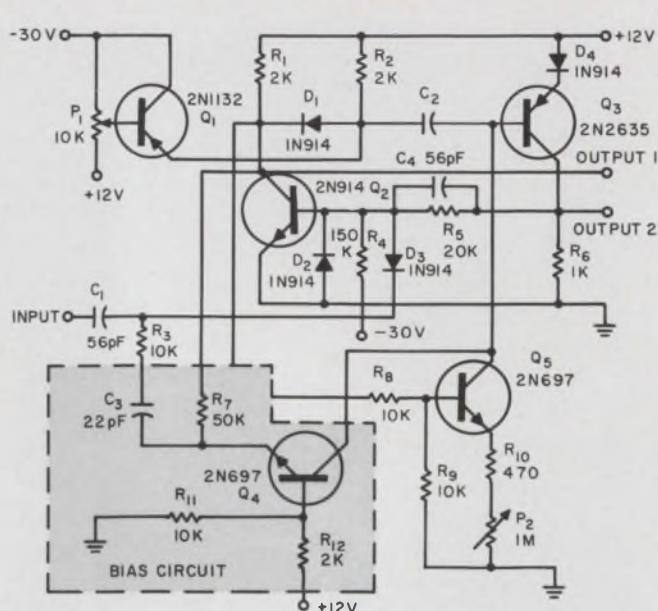
5. Linear complementary monostable multi results from still another current source.
