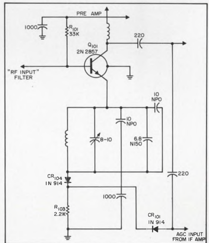
3. Input stage agc is applied at Q_{101} through CR_{101} , shunting the collector signal circuit, and R_{103} .
