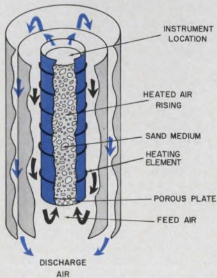
Heat controlled sand medium is used for temperature calibration.
