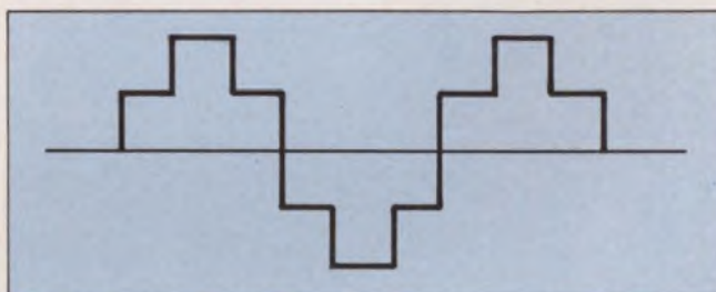
3. Quasi-square waveform of the output line-to-line voltage greatly reduces the harmonic content of the signal.
