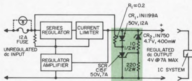
Simple crowbar circuit provides fast shut-off of power supply so that over-voltage transients do not damage integrated circuits.
