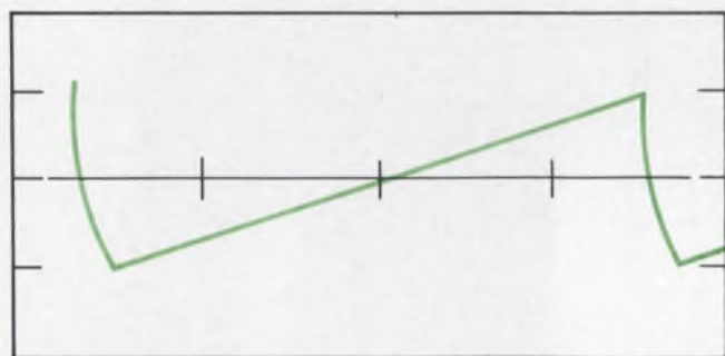
2. The output amplifier collector voltage (a) is 350 volts peak-to-peak. Here the horizontal scale is 5.0 ms/div and the vertical 100 V/div. Linearity of the yoke current (b) is due to feedback. Vertical scale here is 0.25 A/div; horizontal, 5 ms/div.
