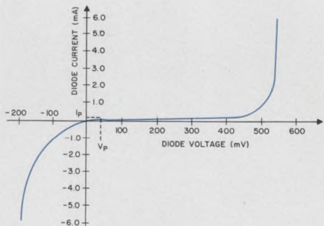
1. Typical I-V curve for backward diodes is very similar to that of a point-contact diode, when turned upside down. Therefore the backward diode may be used as if the n region were the anode and the p region were the cathode.
