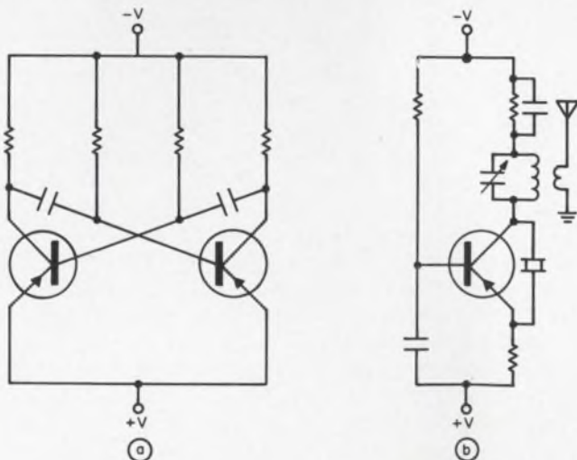
1. Combination of bi-stable multivibrator (a) and RF oscillator (b) results in a super-regenerative, reflex-action detector. Low distortion and high reliability accrue.
