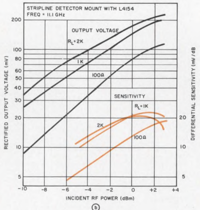
10. The maximum allowable power level may be found with these graphs for waveguide (a), and stripline mounts (b).
