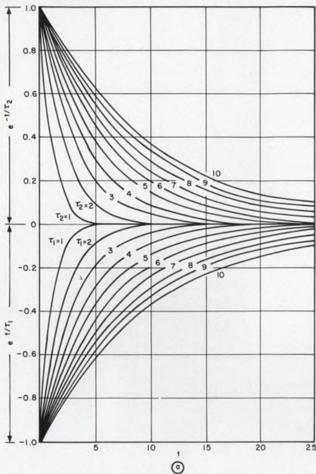
5. This graph permits interpolation of the in-phase overshoot to be made (a). To the plot of the exponential portions of the normalized overshoot voltage, we graphic-
