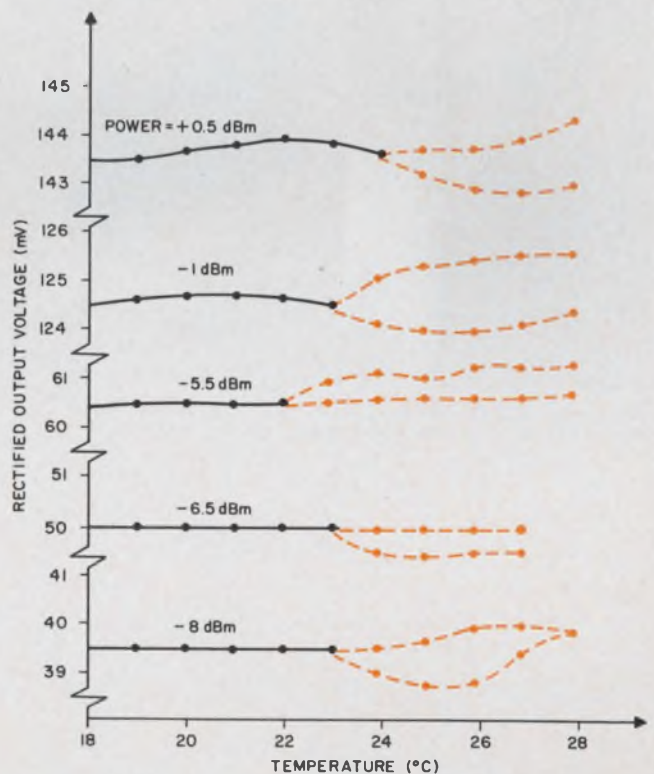
14. The rectified output voltage of an L4154 in X-band clearly shows the effects of temperature instability at varying power levels. The diode apparently switches between two states.
