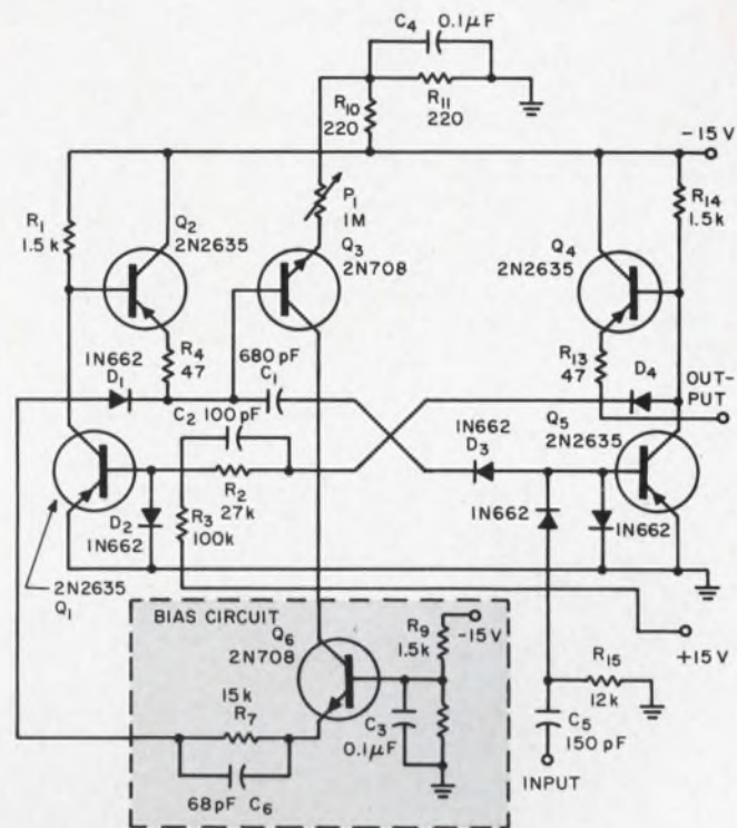
2. More linear operation is possible by adding still another current source and separating the bias and timing functions even more sharply. Pulse width is more stable because of linear timing capacitor discharge.
