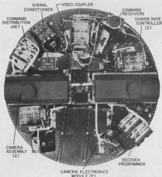
ESSA II is the latest of the TIROS-class weather satellites. Its two cameras are mounted 180 degrees apart on the outer rim. Electronic circuitry is arranged around the baseplate (shown at left). Numbers in parenthesis indicate redundancy.
