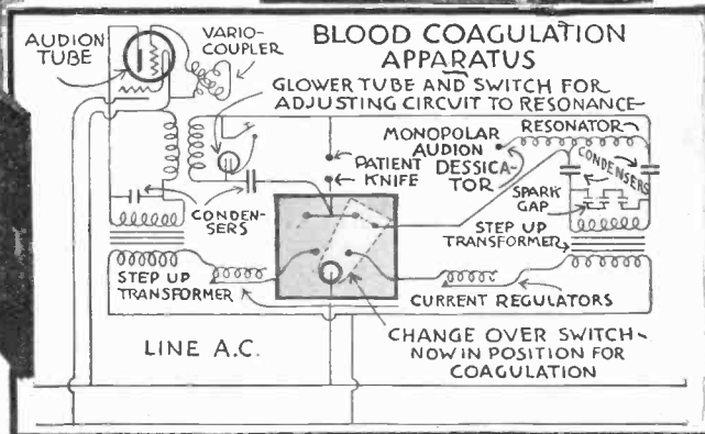
The above diagram shows the circuit of the "radio knife" apparatus. The instrument was developed by Dr. George A. Wyeth and is technically known as the Endotherm. Photos courtesy Wappler Electric Co.
