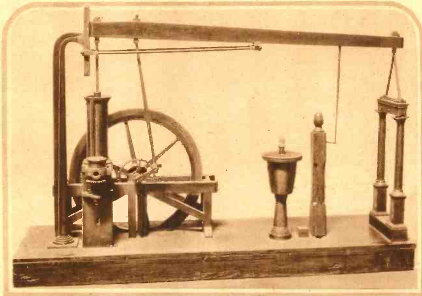
Almost all of the large trans-Atlantic liners owe their operating efficiency to the principle involved and first worked out in the above model. It shows Oliver Evans' original high pressure steam engine working on the compound principle. After the steam had exerted its force in the high pressure small cylinder, it passed over and expended some residual energy in the large low pressure cylinder. Both motions were communicated to the rocker arm which was connected to the pulley wheel.
