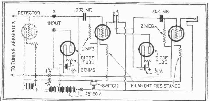
The diode tubes employ a single dry cell to light their filaments. Not only does the tube function as a plain resistance coupled amplifier, but its use allows of a lower "B" battery voltage being employed. The above diagram shows how the amplifier may be connected.
