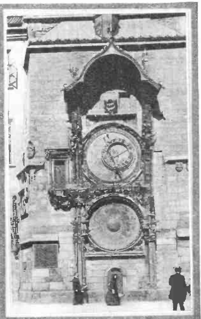
Town Hall clock at Prague, Czecho-Slovakia, was built in 1430. It shows mean time, Sideral time, and position of sun. —Siouka.
