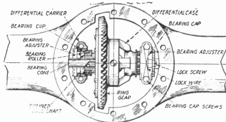
"E" The above illustration shows the remaining adjustments on a differential that are to be reached by removing the rear inspection cover.
