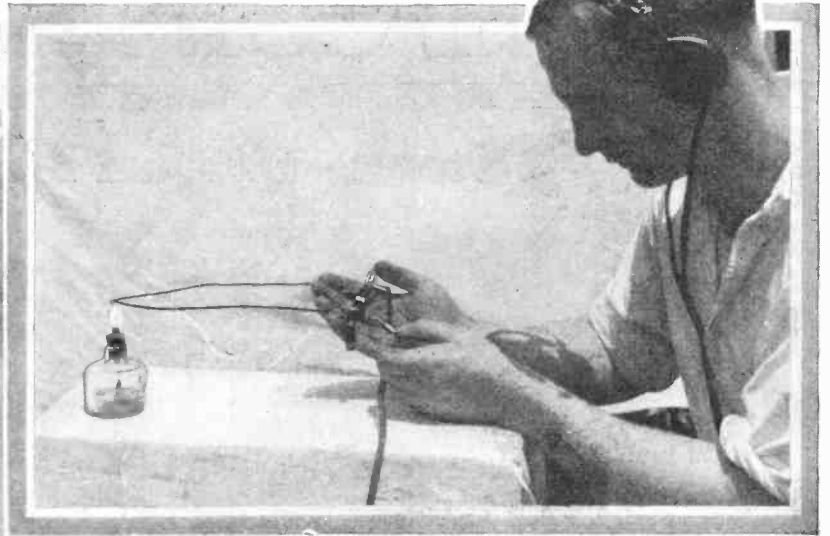
Electricity can be made directly from heat. To perform this experiment, twist the ends of an iron and a copper wire together, connecting the two wires to a pair of radio receivers. If the ends of the wires are heated and one of the phone tips is intermittently touched with one of the wires, thus opening and closing the circuit, a series of clicks will be heard in the telephone. This is the principle of the thermo-couple.
