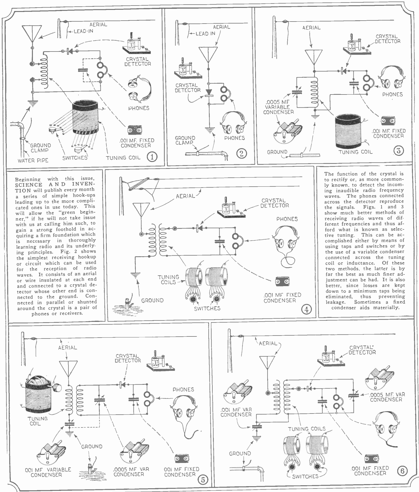
Fig. 4 shows an arrangement whereby much finer tuning can be accomplished and what is known as "interference" obviated to a great extent. It is known as an "inductively coupled" circuit. The radio wave is picked up by the antenna and then traverses the primary circuit, where tuning is accomplished by means of a switch and the necessary taps. By means of the phenomena of induction, the radio frequency currents are induced into the secondary circuit through the inductance. The rest of the circuit, as can be seen, is similar to the single circuit receiver as shown in Figs. 1, 2 and 3. The space between the primary and secondary inductances is what is known as the degree of coupling between the primary and secondary
