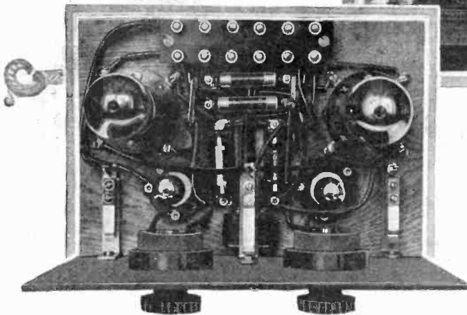
The above photo shows a view of the two step audio frequency amplifier employing the new method of coupling. In the upper right-hand corner is shown a group of New York newspaper men listening attentively to Mr. J. W. Marshall, a Philadelphian, the inventor of the system. Tests show no distortion whatsoever, both on local and distant stations, and with no apparent diminution in volume.
