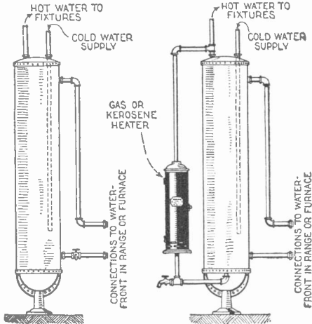
Range boilers can readily be installed by the average layman. The above diagram shows how to do it properly so as to pass the fire underwriters' rules.
