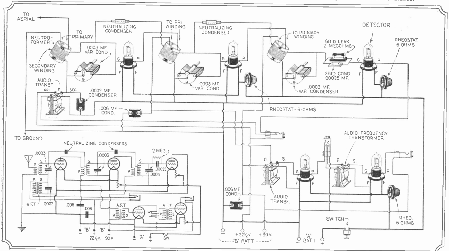
Those who have a four tube reflexed neutrodyne will find that an added stage of audio frequency amplification will vastly improve the volume on distant stations. The diagram shows explicitly how this can best be done. It is best, perhaps, to rewire the set completely for superior results.
