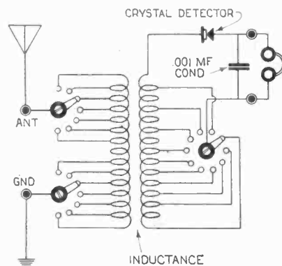
The primary consists of 300 feet of No. 38 S. C. C. wire, tapped at every 20 feet and is wound in a compact coil, 2 inches in diameter. The secondary contains 400 feet of the same wire, tapped at every 40 feet.
