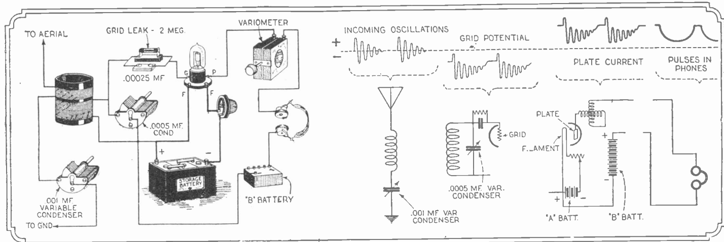
Just what happens in the different parts of a simple regenerative circuit is depicted here. Memorize the diagrams. They will help you in solving and understanding more complicated hook-ups.
