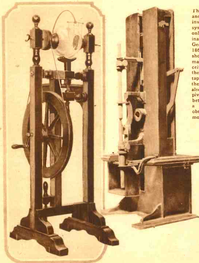
Dr. Franklin's original static machine using a whirling glass globe rotated by a wooden hand wheel, and incorporating a metallic ball to collect the charge is shown at the left above. At the right is a model of an early arc lamp using gravity with a ratchet control to feed the carbons.
