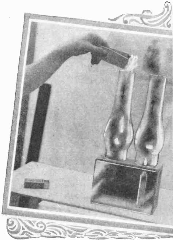
The convection of air currents is shown above. The candle is placed under one of the lamp chimneys and a piece of lighted paper held over the other. The hot air rises above the candle, pulling the smoke and flame of the paper down through the second chimney. Metal conducts heat better than wood. (See right.) Half a rolling pin is covered with metal foil and then with paper, and the paper lighted. The paper will burn while there is wood under it, but will go out over the metal because the metal dissipated the heat, preventing the paper burning.
