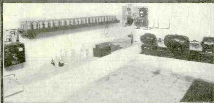
Below: A View of the Extremely Neat Power Room of WKAQ. The Motor-Generators Appear on the Right and the Various Instruments and Apparatus Necessary for the Operation of the Station May Be Seen Around the Wall. This Station Has Been Heard in New England, Nova Scotia, and Many Cities Throughout the United States. The Station Proves to Be An Important Link Between the Island and Distant Places. Lower Right: The Monitoring Set of WKAQ on the Desk, and the Voice Amplifier on the Wall. The Operator Can Check Up On the Outgoing Programs by Means of His Receiving Set.
