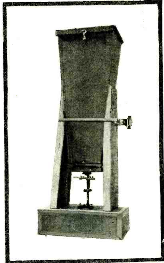
In Picture of Apparatus (Above) Brass Strip Movable Support for Camera is Shown. Light for Illuminating Subject Must Be Directly Under Slide, in Cigar Box. Use a Flat Black Paint Only, on Apparatus.
