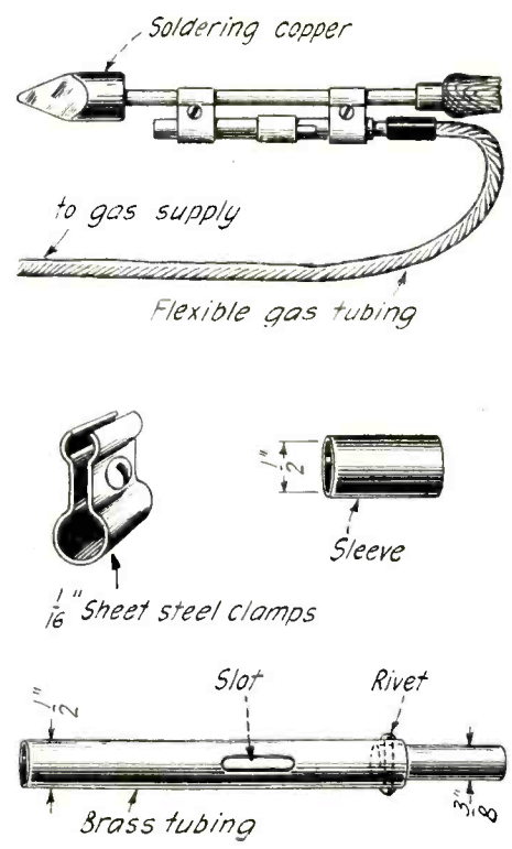
The Burner Used in the Above Heater is of the Bunsen Type. The Sleeve is Placed Over the Slot in the Tube and the Gas Line Attached to the Shank. The Whole is Attached to the Iron with the Clips.—G. A. Luers.
