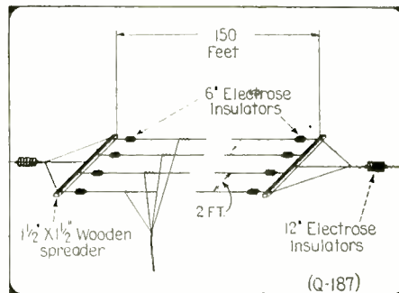
For All Around Use, Where Expense is Not to be Spared, an Aerial Built as Illustrated Above Will Give Excellent Results for Reception. It Should Be Located as High as Possible.
