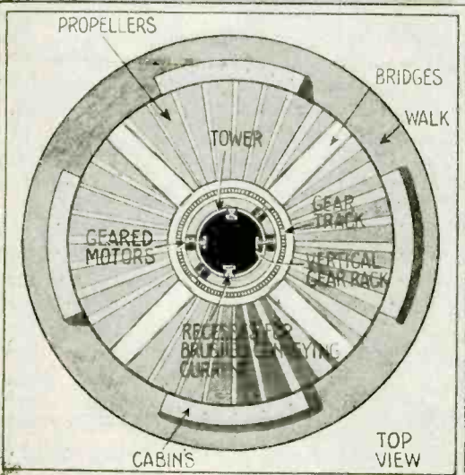
The Above Illustration Shows a Top View of the Revolving Wheel. The Vanes, or Propellers in the Center Forcing the Air Through Help in the Ascent and Operate as a Cushion in the Descent. Coming Down the Tower, the Motors Are Used Only to Break the Speed as the Wheel Nears the Bottom.
