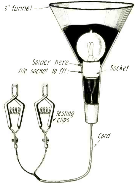
A Trouble Light Can Be Made from a Funnel and Headlight Socket. Solder Socket in After Cord Has Been Drawn Through the Neck of the Funnel. Attach Battery Clips to the Ends of the Cord. A 3-Inch Funnel Will Serve the Purpose Best. It's Not Necessary to Fasten the Cord In.—Stanley Fitch.
