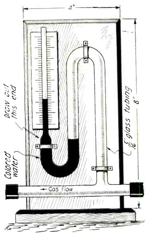
The Above Illustrated Gas Gauge is Simple in Construction. The Bend is Made and the End Drawn Out. The Tee is Then Made. If the Bends are Made While the Glass Rests on a Flat Surface a Neat Product Will Result.—Carlyle Weiss.
