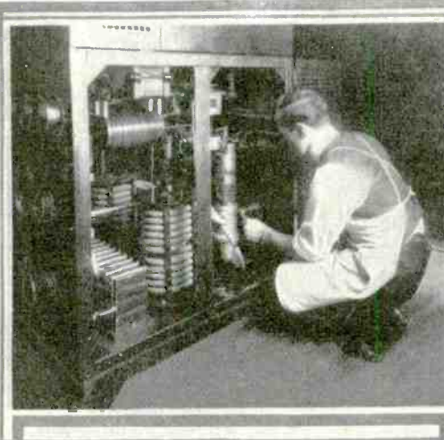
The Inside of the Vacuum Tube Unit is Illustrated, Showing the Water-Cooled Tubes Designed to Operate With a Plate Voltage of 6000 Volts Great Success Has Been Achieved With This Arrangement.
