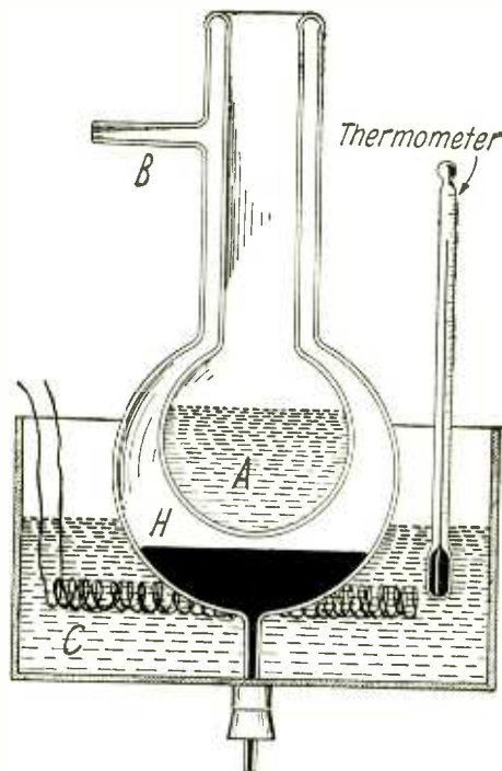
The Above is Apparatus Used by Dutch Chemists to Obtain Mercury Isotopes. The Mercury (H) is Boiled in the Vacuum Envelope of a Thermos Bottle by Immersing Bottle in Electrically Heated Oil. The Lighter Isotope Comes Off First and Freezes Against the Inside of the Bottle Containing Liquid Air. Residue is Then Poured Off and Frozen Product Allowed to Drip Back. Isotopes Obtained Thus Differed One-Half of One Per Cent. in Atomic Weight.
