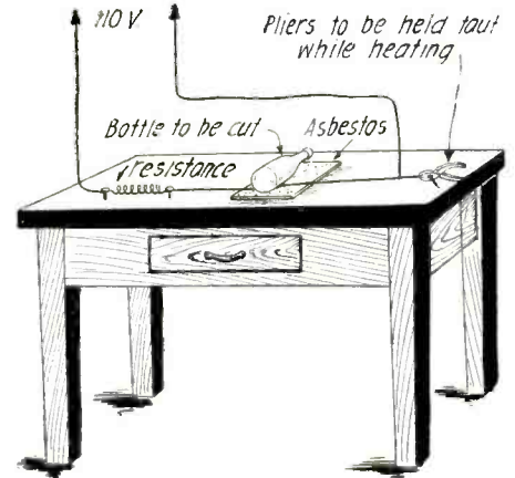
The Heat Through the Resistance Wire (Nichrome or German Silver) Quickly Cuts the Bottle in a Clean Line Where the Wire is Wrapped Around it.—Frank Lindstaedt.
