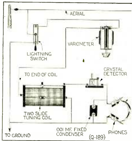
The Necessary Connections for a Lightning Switch Used with a Crystal Receiving Set Are Shown Above. The Variometer Will Allow Reception on Higher Wave-Lengths.
