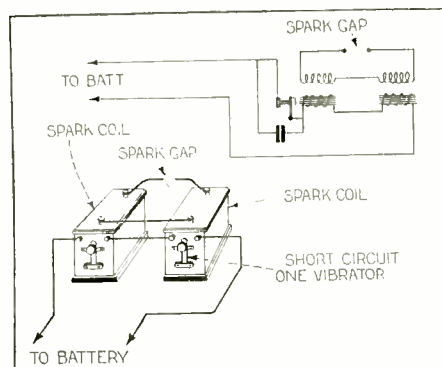
In Connecting the Spark Coils in Series For a Fatter and Longer Spark, as Shown Above, Short-Circuit One of the Vibrators, as Shown.
