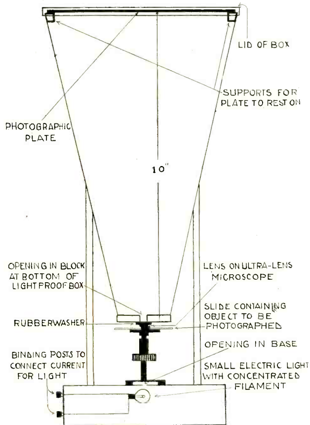
Cross-Section Shows Lightproof Box Taken from Old Enlarging Camera or Constructed by Amateur Supported Over Microscope. Top Must Fit Light-Tight. Microscope and Camera Are Supported on Cigar Box.
