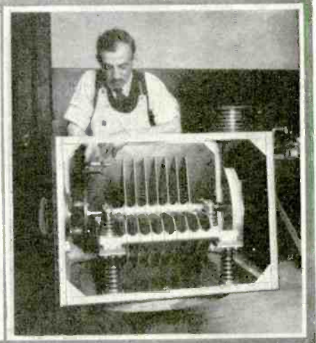
One of the Variable Condensers on the Leviathan's Transmitter, Compared With a Standard Variable Condenser Held by the Gentleman.—Photos, C. W. Tucker.
