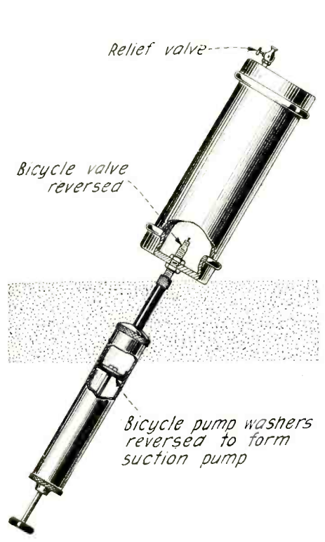
The Best Method of Popping Corn is in a Vacuum. The Device Illustrated Here is Made of a Short Length of Large Pipe. The Corn is Inserted and the Cylinder Heated and the Air Exhausted.—W. E. Dodge.
