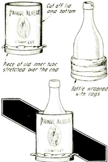
A Force Pump Handy for Cleaning Sink Pipes Can Be Made from a Circular Can and Bottle. Wrap the Bottle with Rags So It Fits Snugly. Place a Piece of Inner Tube Over the Bottom of the Can in Order to Get Tight Contact Over the Sink Strainer and Then Work the Bottle Up and Down Vigorously.—Thos. Barta.
