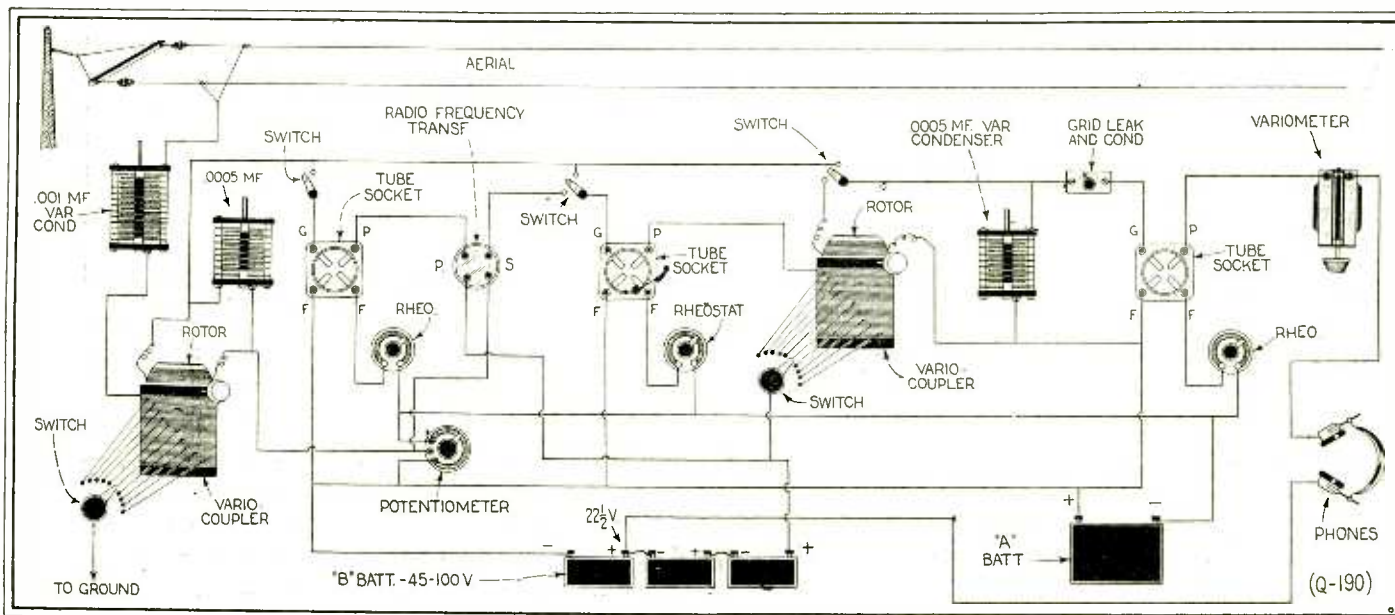
An Excellent Circuit for Tuned Radio Frequency Amplification is Given Above. By Means of the Two 2-Point Switches and the Single-Point Switch, it is Possible to Use One or Two Stages of Radio Frequency Amplification or Both May Be Eliminated and the Detector Used Alone. The First Stage
