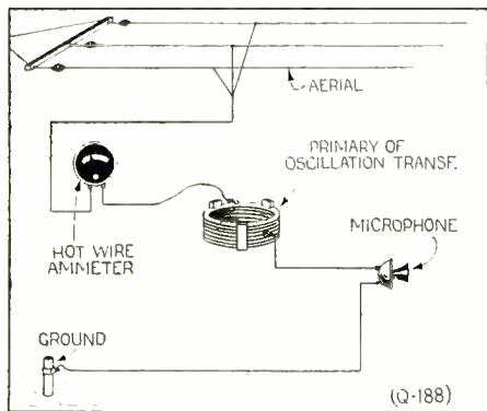
A Microphone Inserted in the Ground Lead of a Loose-Coupled C.W. Transmitter, Will Allow the Transmission of Radiophone Messages. This Method is Satisfactory Only Over Short Distances.
