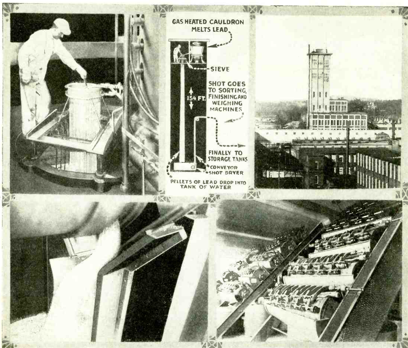
Upper Left: The Sieve From Which a Shower of Lead Drops 154 Feet Into the Water. Upper Center: A Cross-Section View of the Shot Tower. Upper Right: An Exterior View of the Shot Tower. Lower Left: Stream of Shot
