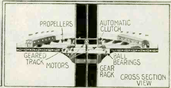
A Cross-Section of the Wheel Shows the Hub Which Rises on the Tower. Motors Attached to it Work Into the Gearways on the Side of the Column, Raising and Lowering the Wheel. Two Other Motors Furnish Power to Drive the Wheel in its Circular Motion. The Wheel Itself Rests on the Hub on Ball Bearings.
