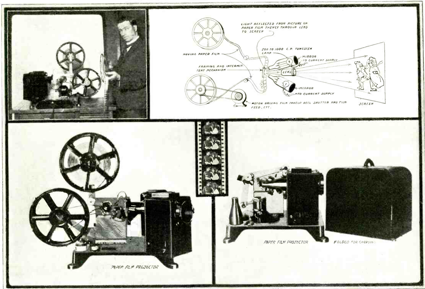
Paper Movie "Films" Are the Latest. The Upper Left-Hand Photograph Shows the Inventor With One of His Projecting Machines Employing Paper "Film" Movies. The Diagram at the Top Shows How Powerful Incandescent
