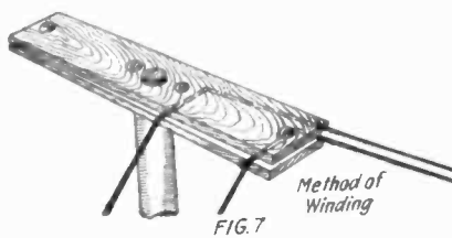
Details of Construction for the Loop Aerial to be Used With the Vacation-time Radio Set, Are Given in the Drawing Above. A Series of Holes Are Drilled Thru the End of One of the Cross Sticks, so That the Aerial May be Pulled Tight and a Nail Inserted Behind the Spreader on This Particular Leg to Hold the Wires Taut.
