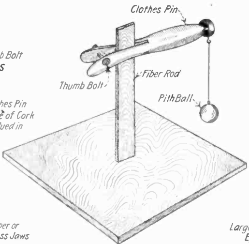
INSULATED STAND
