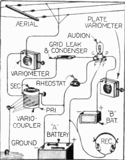
Query 17.—A Short Wave Regenerative Receiving Set, Using Two Variometers and a Variocoupler for Tuning.
