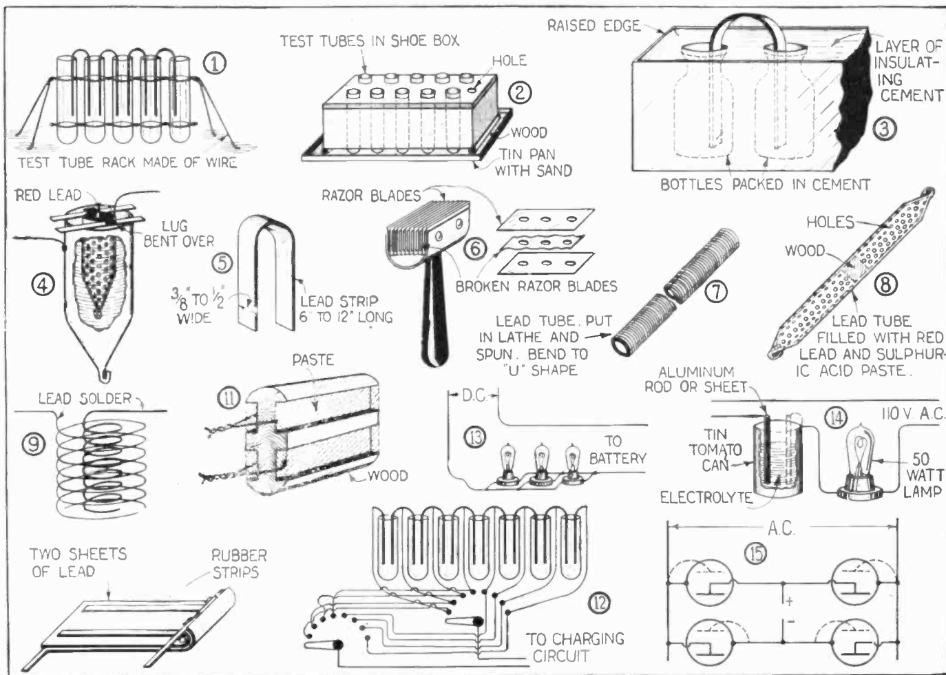
Now That Vacuum Tube Amplifying Receivers Are Coming Into Extensive Use, and in View of the Fact That the Dry "B" Batteries Are Not so Efficient After They Have Begun to Age Somewhat, and Also as They Frequently Give Rise to Noise, Due to Loose Connections or Weak Cells in the Regular Sealed Block Batteries, the Storage "B" Battery is Rapidly Coming into Favor. A Great Variety of Ideas Are Here Illustrated and Described, for Making Your Own Storage Batteries for the Plate Circuits of Vacuum Tube Receiving Sets.
