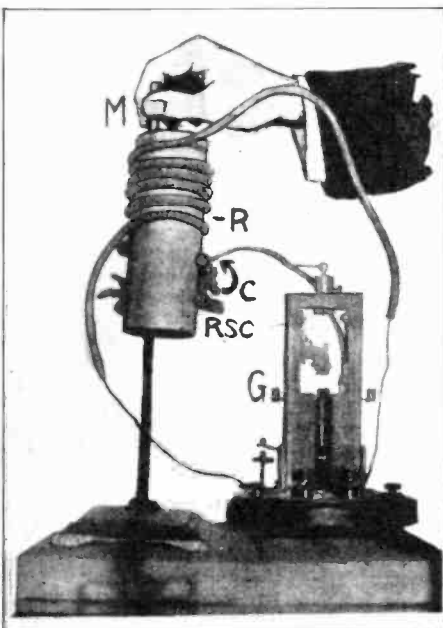
An Interesting Experiment With a Solenoid Made from a Rubber or Glass Tube Coiled Around a Drum. An Electrolyte Fills the Tube and is Connected with a Galvanometer. A Magnet Plunged Into the Solenoid Causes a Current to Flow.
