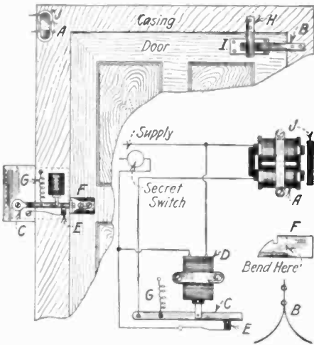
Useful Home-Made Electric Door Opener.
