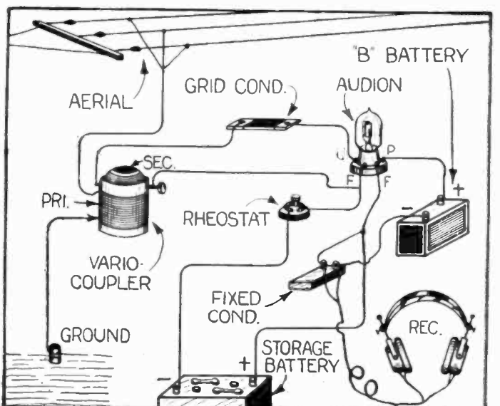
Query 18.—Above is Given the Circuit for a Loose Coupler Used in Connection with an Audion Detector.
