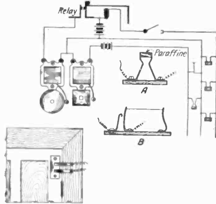
Valuable Burglar and Fire Alarm Circuit.
