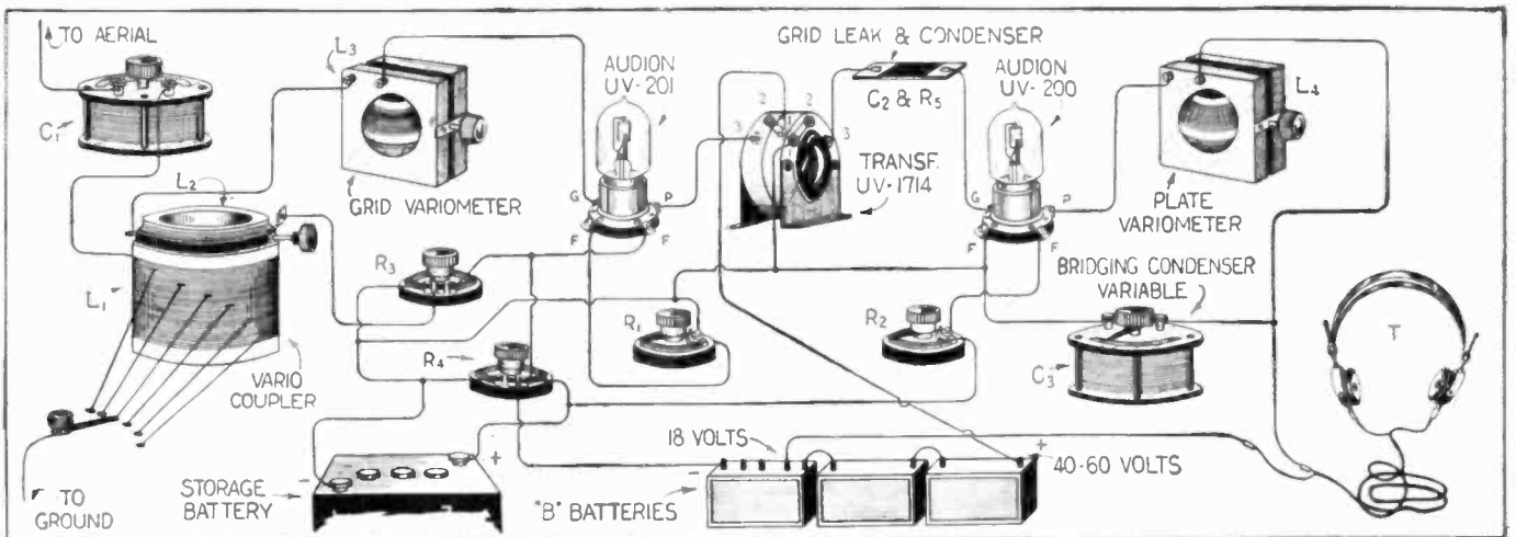
FIG. 1. VARIOMETER-REGENERATIVE CIRCUIT WITH 1-STAGE RADIO FREQUENCY AMPLIFIER
