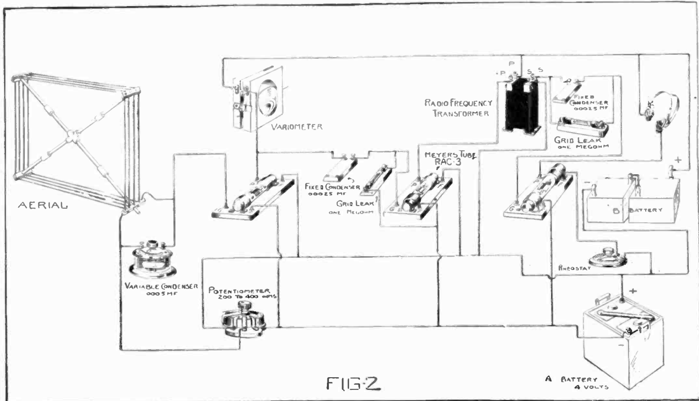
Perspective Diagram Showing All the Connections to the Terminal Posts of the Various Radio Instruments Used in the Vacation-time Radio Receiving Set Here Described by Mr. Lacault. This Set Utilizes a Small Loop Aerial, as the Front Cover Illustration and Diagram Herewith Show, This Loop Being Shunted by a Variable Condenser for Tuning to Different Wave Lengths. The Amplifier Comprises Two Stages of Radio Frequency, With a Radio Frequency Transformer Connected as Indicated in the Diagram. Three Vacuum Tubes Are Used. These Operate on Four Volts Filament Potential, Which May be Supplied by a Two-Cell Storage Battery or Else Dry Cells. The 'Phones Used Should Have 2,000 to 3,000 Ohms Total Resistance for the Set.
