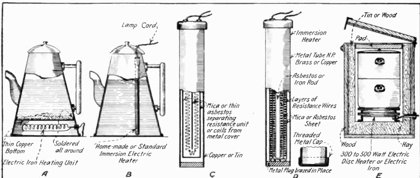
The Illustration Herewith Shows How Home-Made Electric Cooking Apparatus May be Made. At the Left We See an Electric Coffee Pot, While the Center Detail Drawings Show Two Forms of Electric Immersion Heaters, Suitable for Heating Water or for Use in Coffee and Tea Pots. An Electric "Fireless Cooker" is Observed at the Extreme Right.
