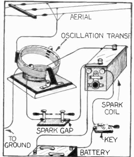
Query 21.—A Circuit Using an Oscillation Transformer in Connection with a Spark Coil and Gap for Spark Transmission is Shown Above.
