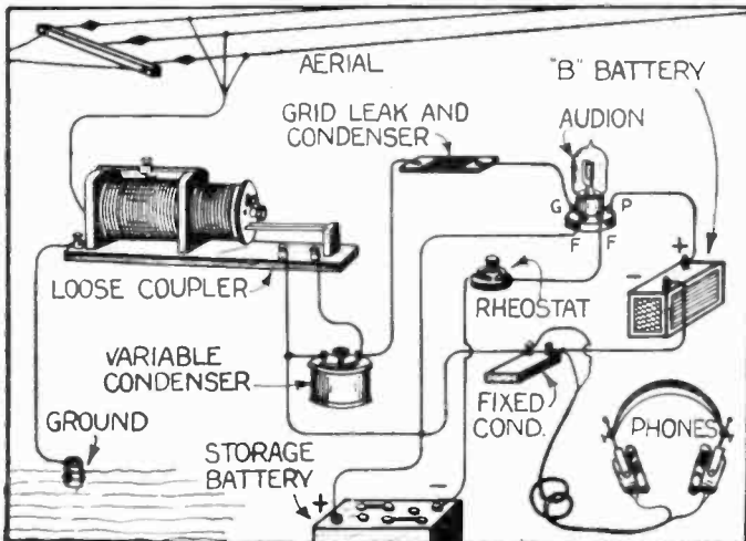
Query 18.—Above is Given the Circuit for a Loose Coupler Used in Connection with an Audion Detector.
