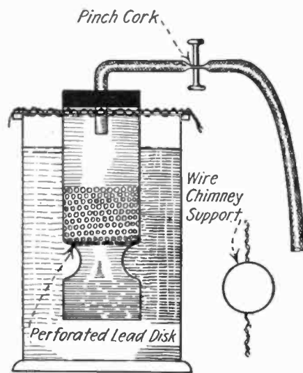
Home-Made Sulfide Generator Made from a Glass Lamp Chimney and a Large Mouthed Bottle. A Perforated Lead Disc Is Placed Inside the Lamp Chimney. Fig. 1.
