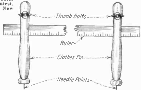
BEAM COMPASS
