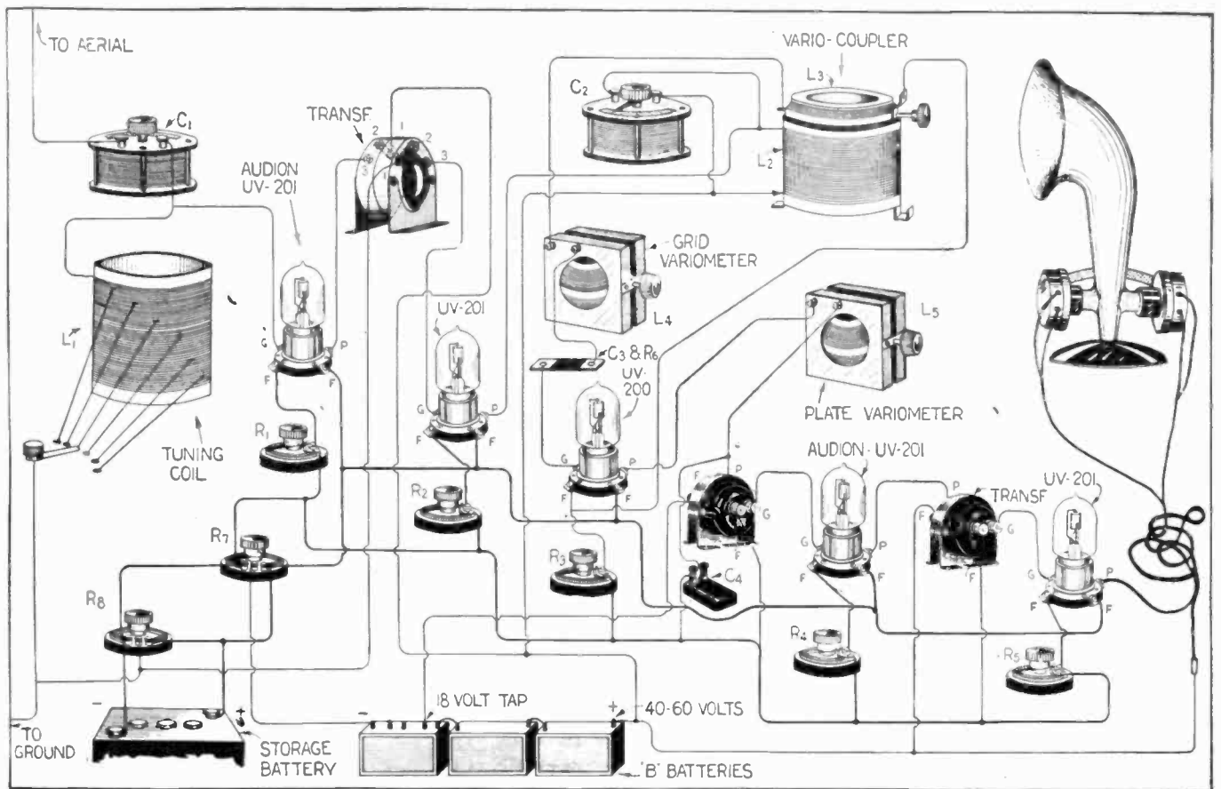
FIG. 2. COMBINED RADIO-AUDIO FREQUENCY AMPLIFIER CIRCUIT (Non-Reradiating)
