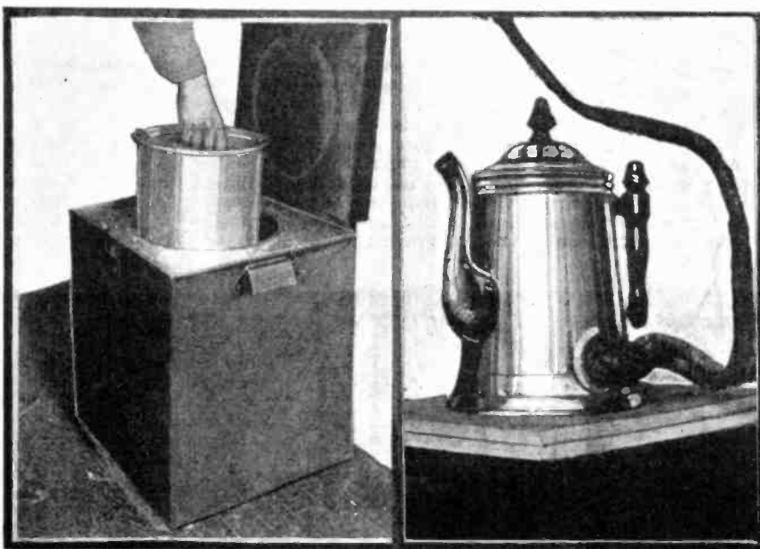
Home-Made Electric "Fireless Cooker."
