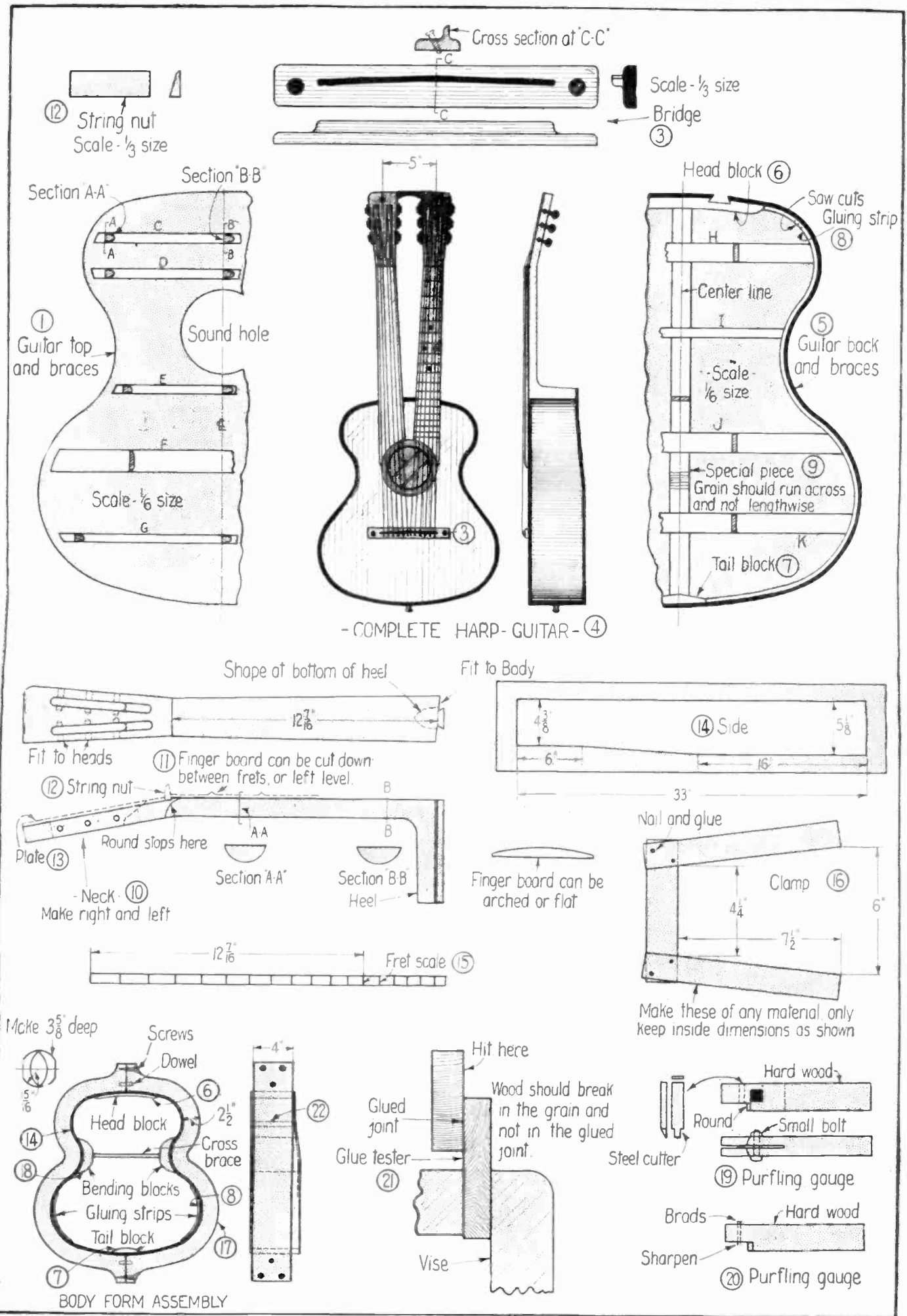
The Accompanying Article and the Illustration Above Explains the Details for Building a Double Neck Guitar.
