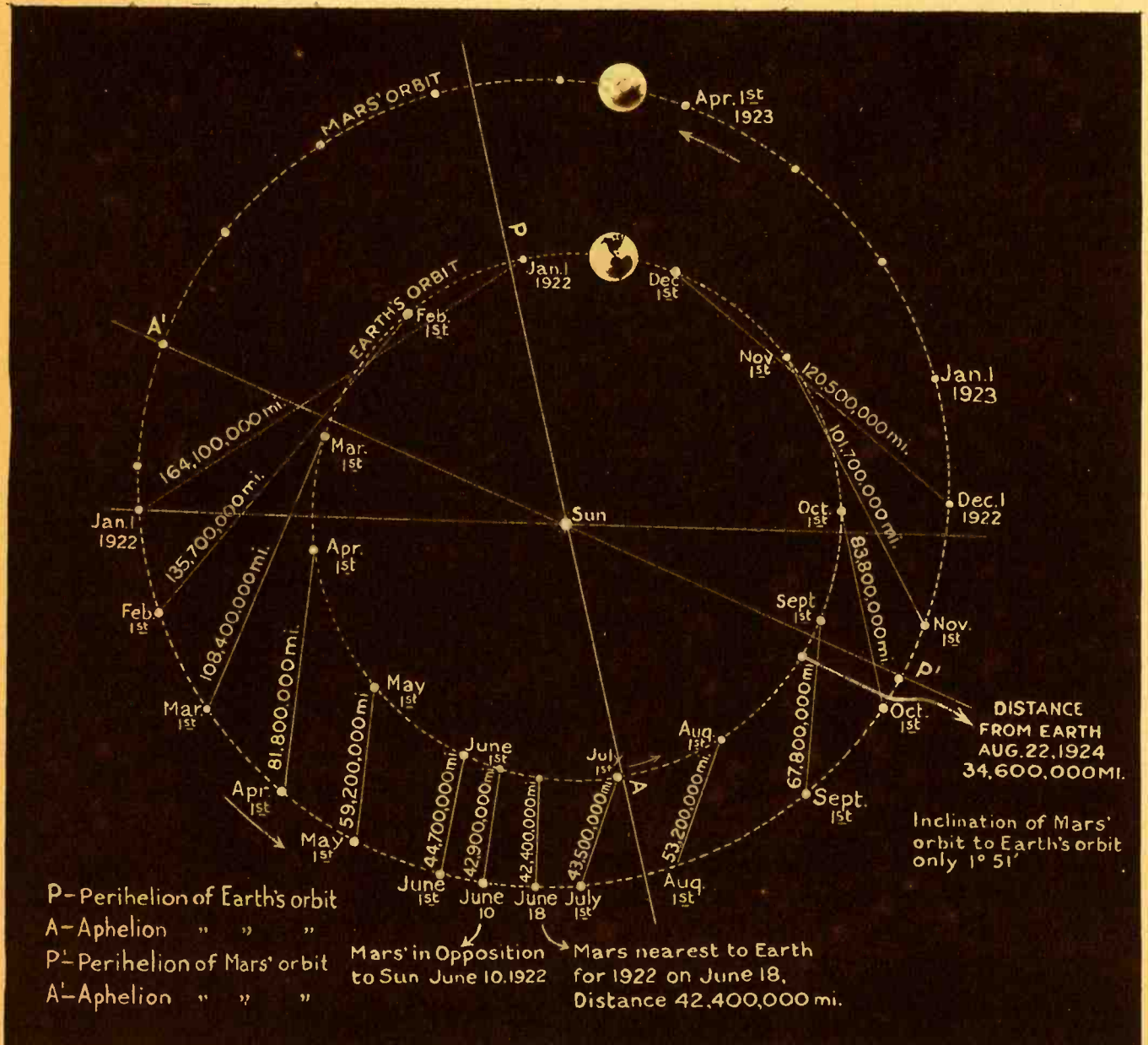
In This Illustration, We See the Two Orbits of Earth and Mars Respectively. It Will be Seen That Mars is on the Outer Track While the Earth is on the Inner. Both Planets Move Roughly at the Same Speed, but Mars Must Traverse a Much Greater Distance Than the Earth in Order to Complete One Revolution Around the Sun. Periodically After a Lapse of Many Years, the Two Planets Pull Very Close Together, the Nearest Distance That They Ever Came Together Being 34,600,000 Miles. This Opposition Will be Reached on August 22, 1924. This Year, on June 18th, Mars and the Earth Will Come Together at a Close Opposition, the Distance Being 42,400,000 Miles, Which is the Nearest the Two Planets Will Approach for the Present Opposition.
