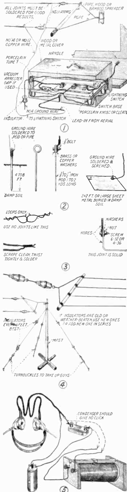
Fig. 1 At Top, Shows How to Install Aerial Grounding Switch Outside Window. Fig. 2 Shows How Ground Rod and Joint is Made. Fig. 3 Illustrates Poor and Good Joints in Wires. Fig. 4 Gives Hints on Aerial Insulators and How to Place Them, While Fig. 5 Depicts Simple 'Phone and Battery Test for Determining the Condition of Condensers, Tuning Coils, Etc.
