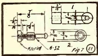
Fig. 7. Details of Binding Posts.
