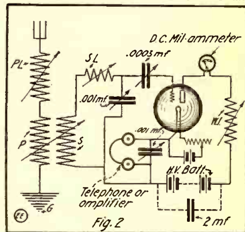
Fig. 2. Audion Amplifier Circuits Employed in Mr. Apgar's Radio Station.
