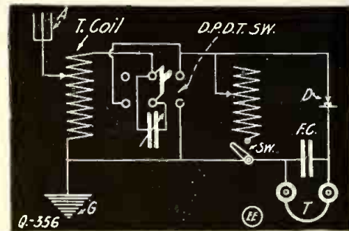
Wireless Receiving Tuning Diagram.
