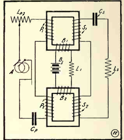
Frequency Changer, Using Transformers Specially Arranged.
