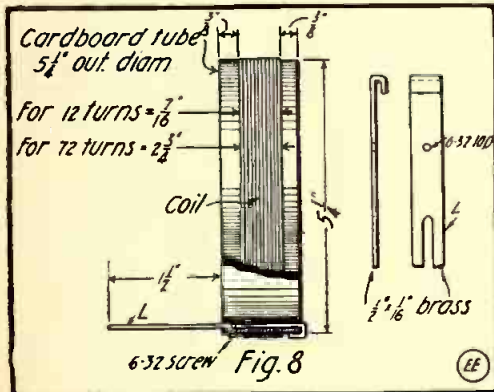
Fig. 8. Inductance Coil Make-Up.
