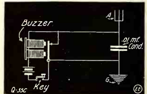
Buzzer Used for Transmitting Radio Signals.
