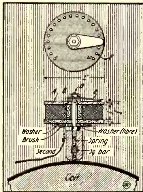
Loading Coil Mounted on Tuner Slider.
