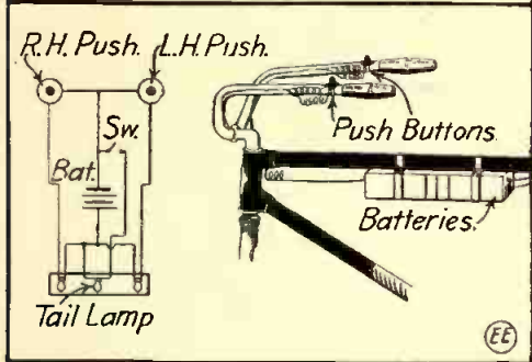
Electric Signal for Tail-End of Bicycles and Motorcycles.
