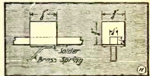
Tuning Coil Slider Made from Wood.
