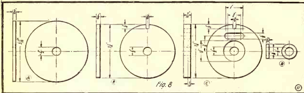
Fig. 8. End Discs of Secondary Coil.
