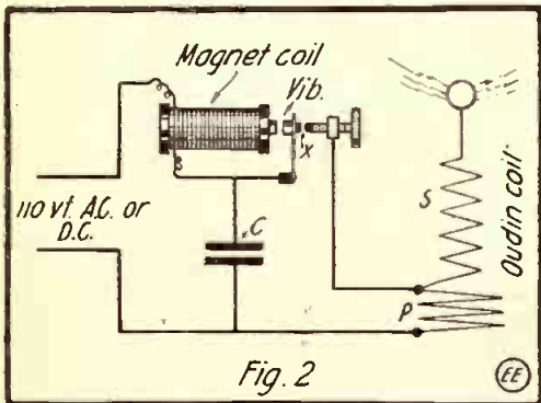
Fig. 2. Collins-Sanchez High Frequency Generating Circuit.
