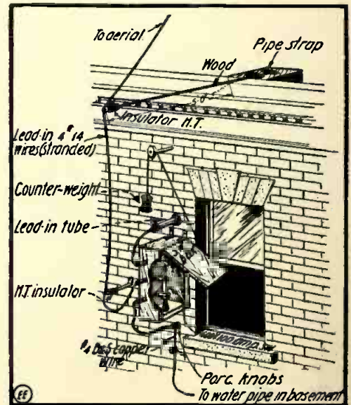
Practical Method of Installing Lightning Switch.
