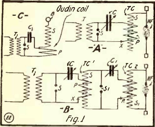
Fig. 1. Diagrams For Oudin and Tesla Coil Hook Ups.
