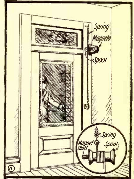
A Magneto Door Bell Saves Batteries.
