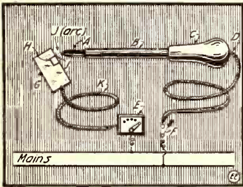
Arc Type Electric Soldering Iron.
