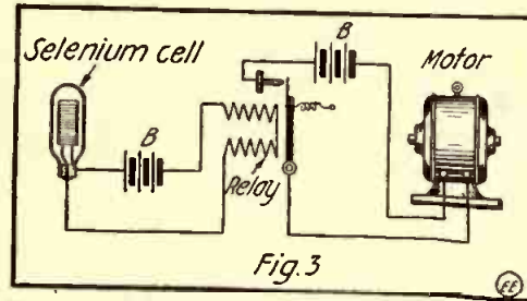
Fig. 3. Standard Connections for Selenium Cell and Relay.
