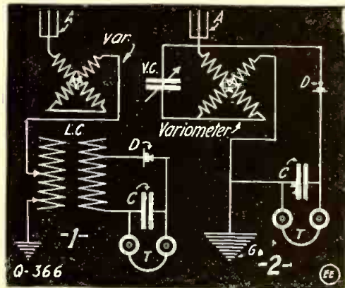
Variometer Hook-Ups.
