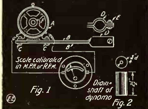
Electric Speedometer for Bicycles.
