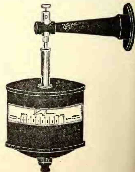
Fig. 5. Electro-Static Type of X-Ray Penetrometer.
