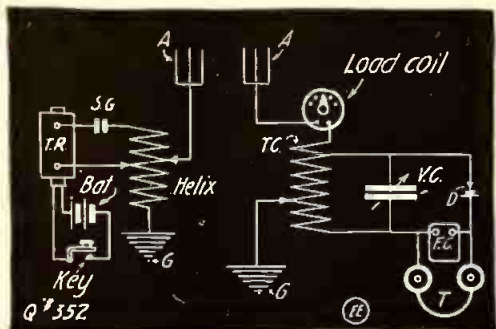
Radio Transmitting and Receiving Hook-ups.
