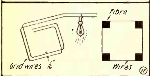
One Type of Electric Insect Destroyer.
