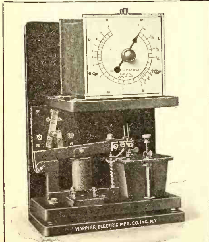
Fig. 8. Serial Timer With Heavy Current Switch for X-Ray Work.
