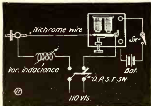
Making Mechanical Waves on Wire Visible.
