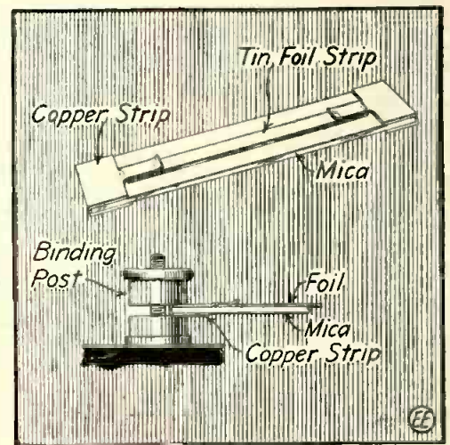
Battery Fuses Made from Tin-Foil and Mica.
