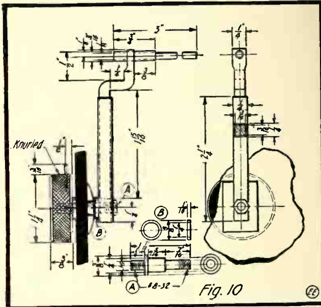
Fig. 10. Arrangement of Secondary Coupling Lever and Knob.
