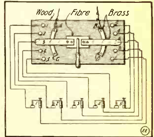
Unique Detector Switch.
