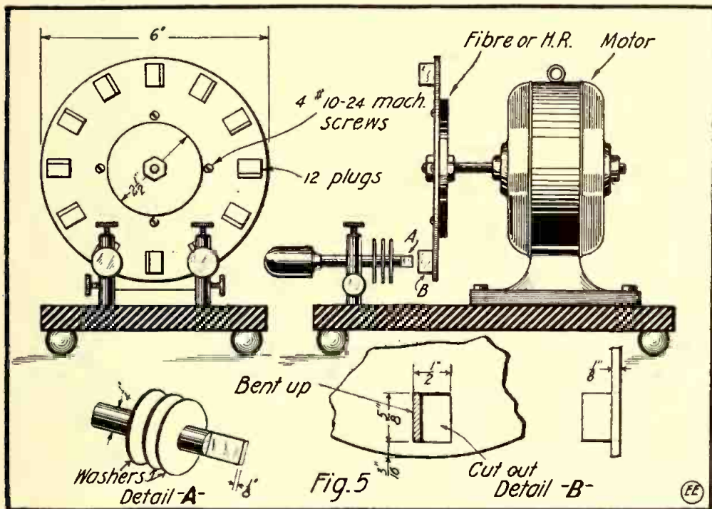
Fig. 5. Details of Rotary Spark Gap for 1/2-Kw. High Frequency Coil.
