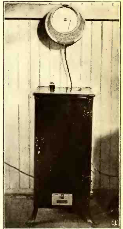
Electric Oven With Automatic Heat Control for Shrapnel Testing by U. S. Government.
