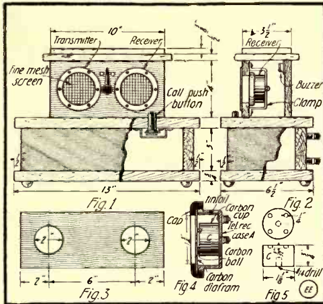
Details of Dictaphone Desk Set.
