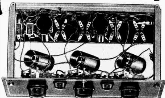
Here you can see the heavy R. F. Coils, the Erla Audio transformers, the heavy socket contacts, the metal frame---and other high grade features in design---found only in the best radio sets made.
