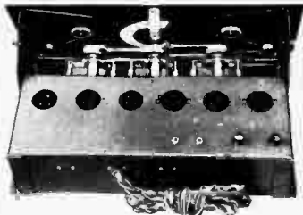
This view shows the substantial metal chassis, the single control mechanism, the six sockets in line and the rugged construction of the Ace single six.
