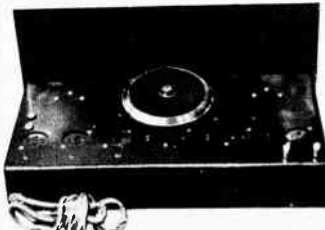
This rear view of the WRIGHT chassis shows the control dial, six sockets in line, the steel chassis shielding and the standard battery cable eliminating unsightly and inconvenient binding posts.
