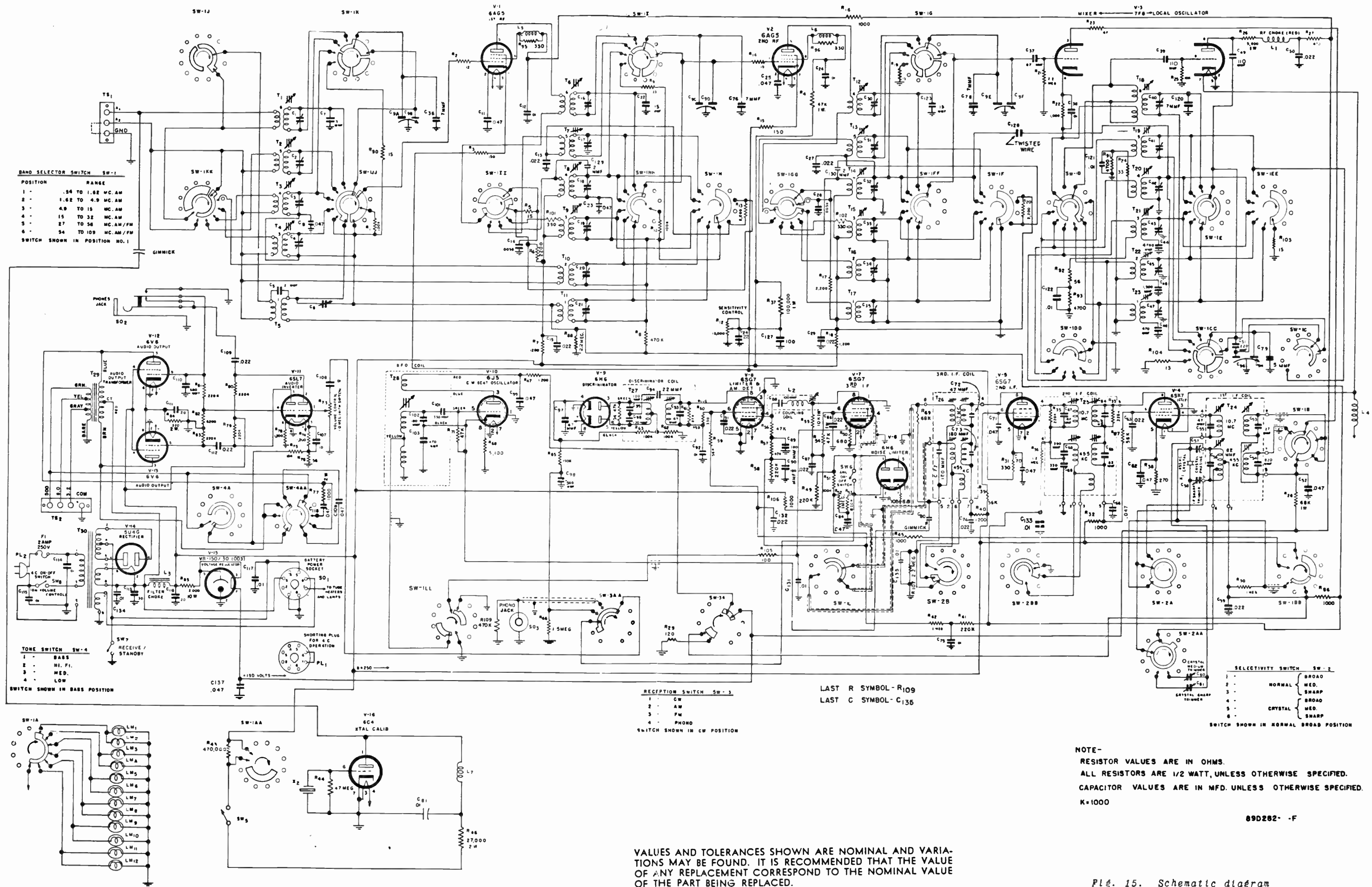
Fig. 15. Schematic diagram
