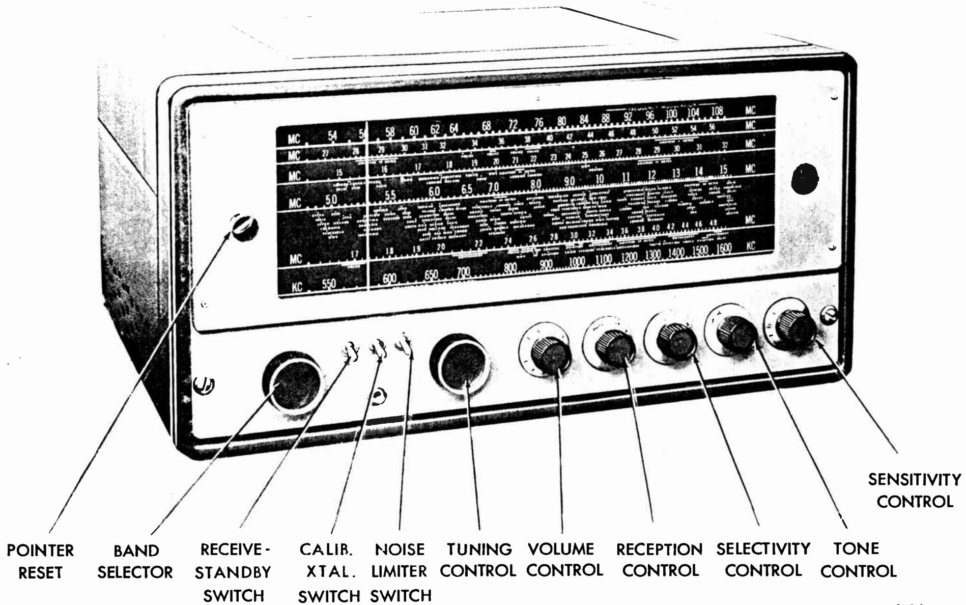
Fig. 1. Radio Receiver Model SX-62A/62AU
