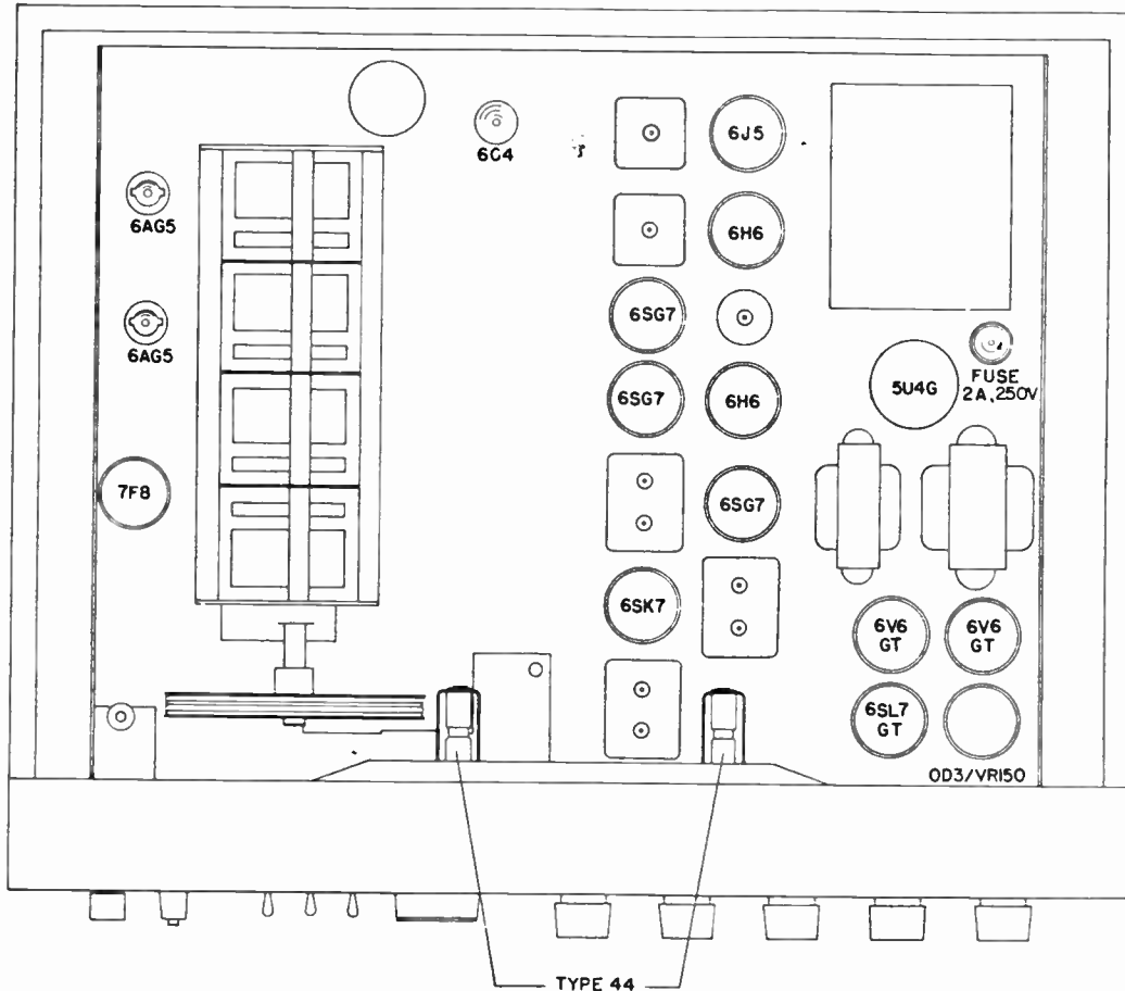
Fig. 6. Top view showing location of tubes and dial lamps
