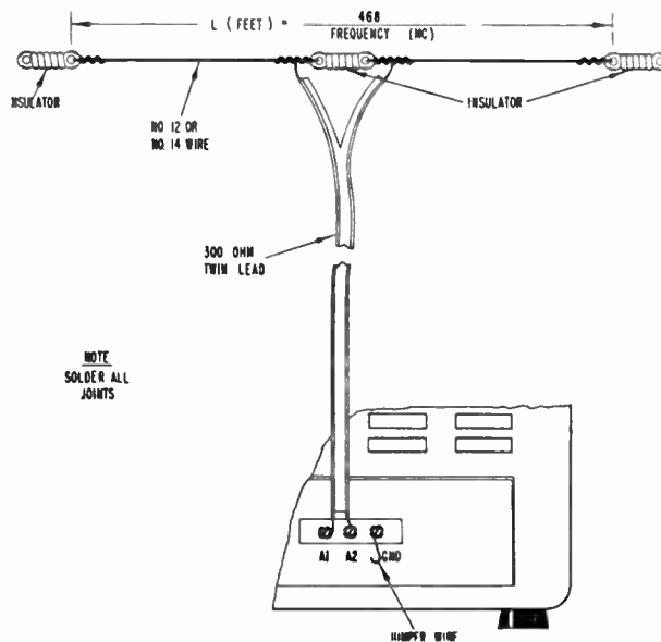
Fig. 5. Doublet Antenna using Twin-Lead Transmission Line
