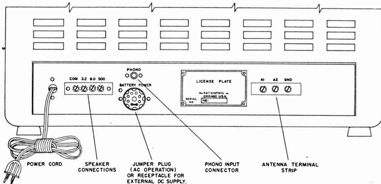
Fig. 3. Rear view.
