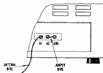
Fig. 4. Single Wire Antenna
