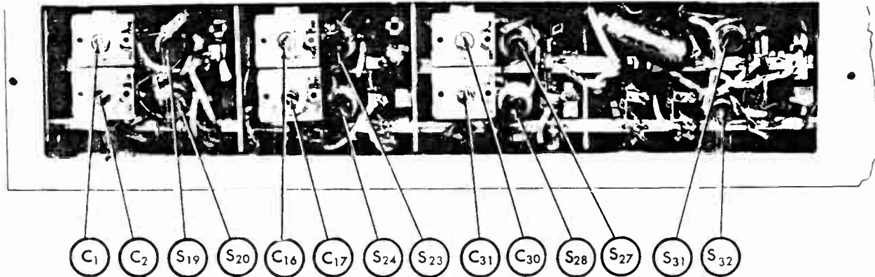
Fig. 10 Alignment adjustments, left side view
