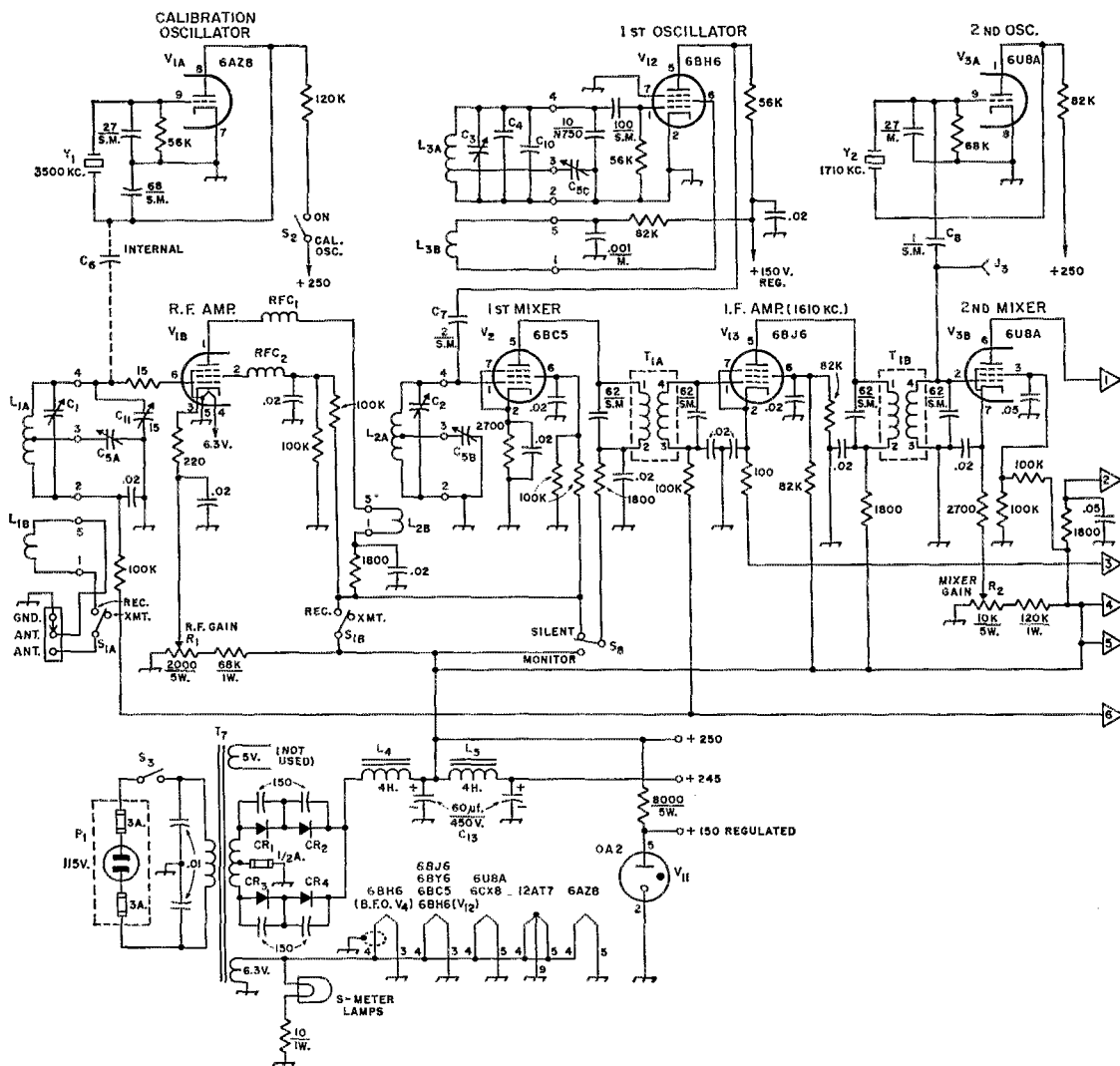
Fig. 1—Circuit diagram of the HBR-13C. Fixed resistors are \frac{1}{2} -watt composition unless otherwise indicated. Fixed capacitors are ceramic except M = mica, SM = silver mica, P = paper or Mylar.
