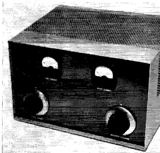
The "Top-Band" linear amplifier. Capable of 200-watt "night" and 345-watt "day" power levels, this compact linear amplifier is suitable for c.w., a.m., and s.s.b. service on 160 meters. The receiver-size wrap-around cabinet is homemade. Cabinet and panel are sprayed with aerosol paint, followed by a coat of clear Krylon enamel.
