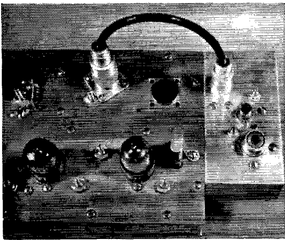
Fig. 1—Top view of the 432-Mc. preamplifier showing fit attached to the converter as a subassembly.
