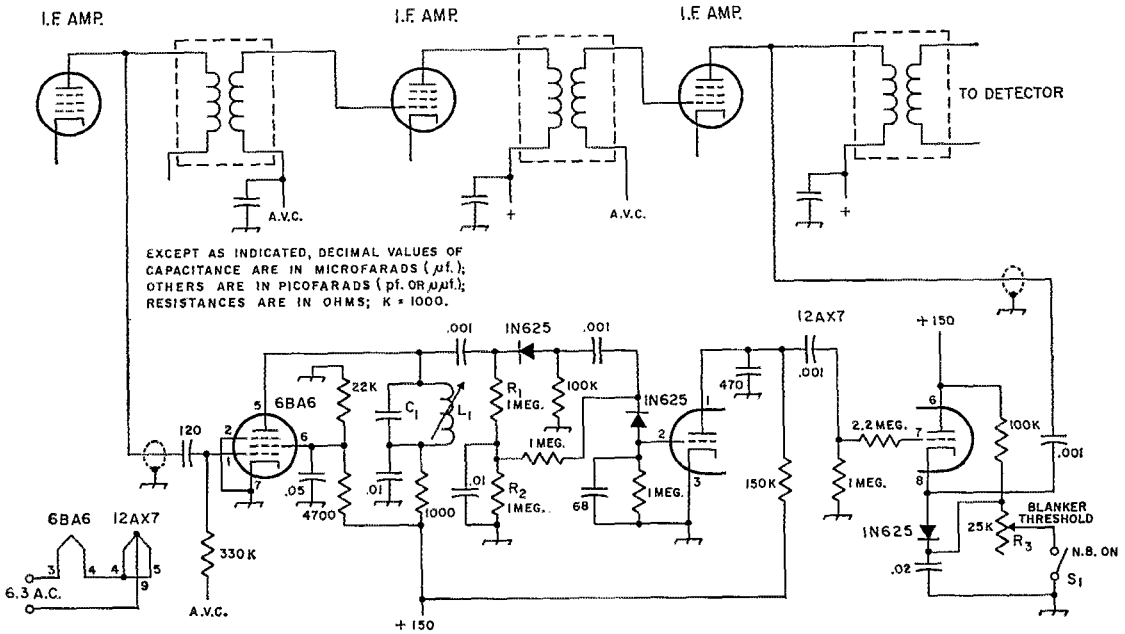
Fig. 2—Schematic diagram of the Drake noise blanker. Capacitors are disk ceramics, and resistors are 1/2-watt.
