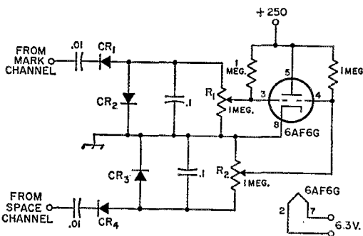
Fig. 1—"Magic-eye" tuning indicator circuit. The display is similar to Fig. 2A when the receiver is properly tuned. Capacitances are in \mu\text{f} ; capacitors may be paper or mylar as convenient. Resistances are in ohms; fixed resistors are \frac{1}{2} -watt.
