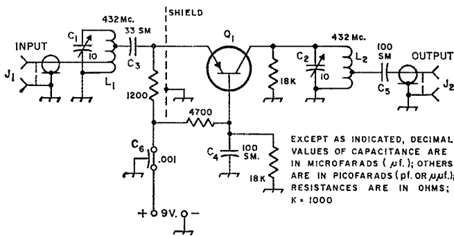
Fig. 2—Schematic diagram of the 432-Mc. preamplifier. 5 M indicates silver mica. Resistors are ¼ watt, carbon.
