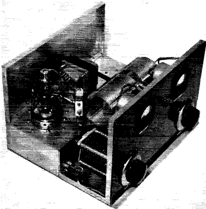
Left-oblique view of the amplifier. The plate-coupling capacitors are supported from the top of the plate choke by a small aluminum bracket. Meter leads are shielded and pass into the subchassis via feedthrough capacitors visible in foreground. The perforated area in the back panel is for a possible addition of a blower, and substitution of a 4-250A at a later date.
