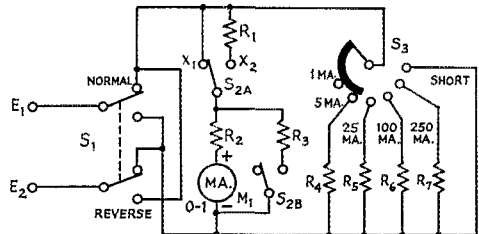
Fig. 2—Circuit of the Multimilliammeter.
