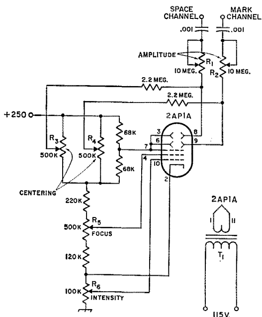
Fig. 3—Oscilloscope indicator circuit. Resistances are in ohms (K = 1000); fixed resistors are 1/2-watt. Capacitances are in \mu f.
