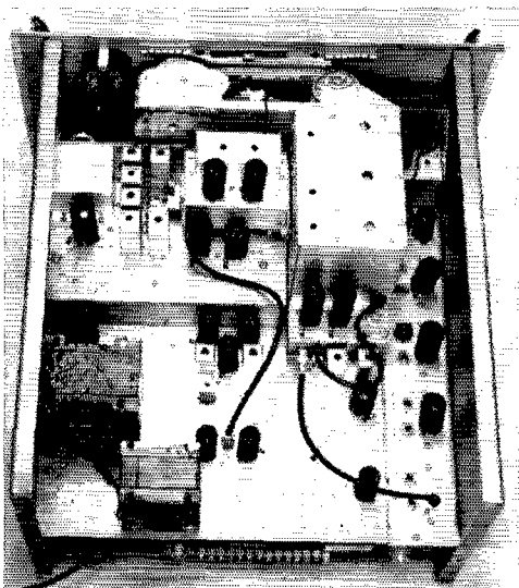
The r.f. stage, first mixers, and the megacycle oscillator are located on the large subchassis to the left. The other large subchassis, at the right, contains the 2-3-Mc. tuner.
