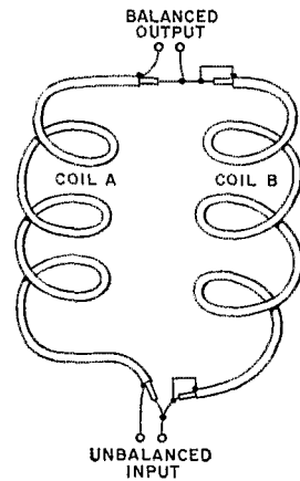
Fig. 1—Two tightly-coupled coils of coax connected to provide an unbalanced to balanced transformation.
