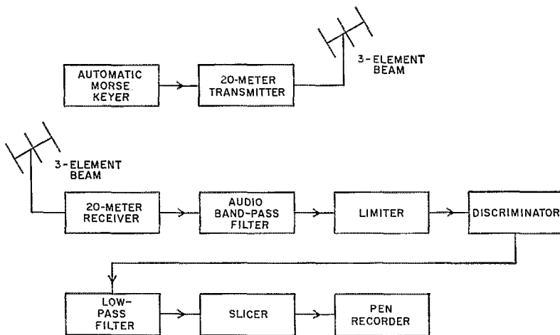
Fig. 1—Block diagram of the weak-signal slow-speed c.w. communication system.
