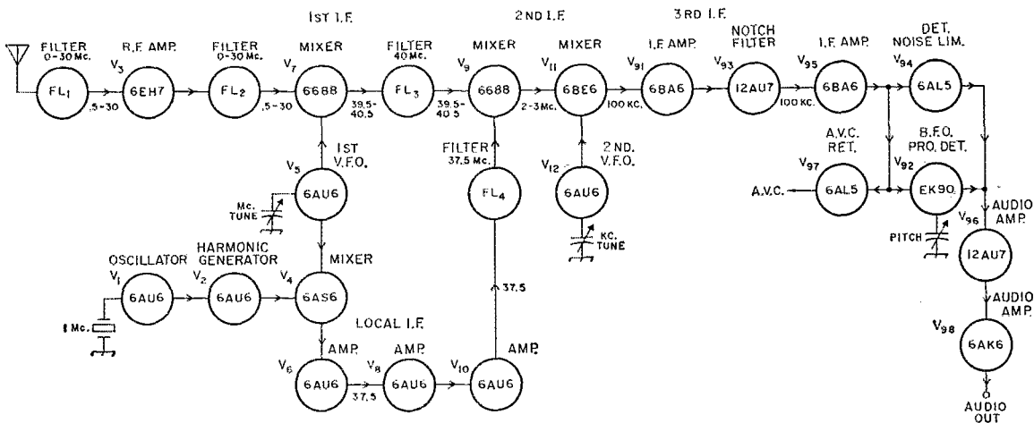
Fig. 1—Block diagram of the Racal RA-71.
