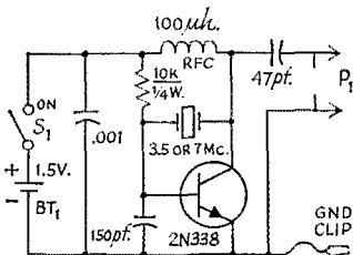
Fig. 1—Circuit of the crystal-oscillator adapter. Capacitors are mica. BT_1 is a penlight cell. P_1 is a plug to fit the transmitter's crystal socket (see text). S_1 is a miniature slide switch.
