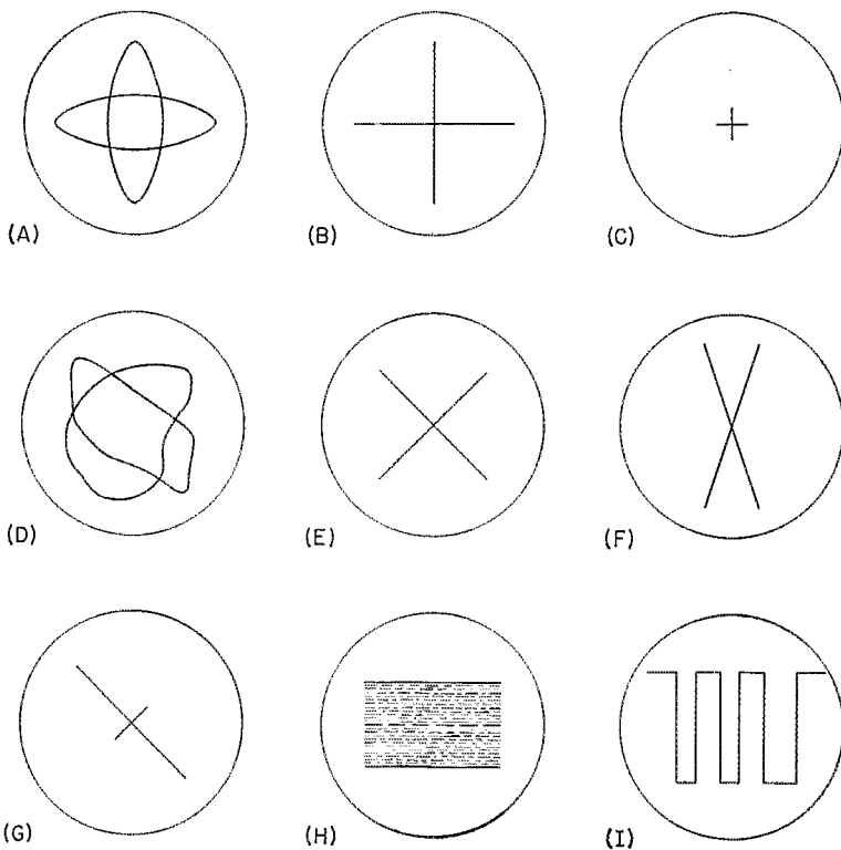
Fig. 4—Scope displays of various types for RTTY signals. See text for explanation.
