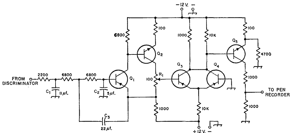
Fig. 2—Circuit of the low-pass filter and slicer. Resistances are in ohms; fixed resistors are ½ watt composition. C 1 , C 2 , C 3 —Good-quality paper; see text. Q 1 , Q 3 , Q 4 —2N404. Q 2 , Q 5 —2N1302.
