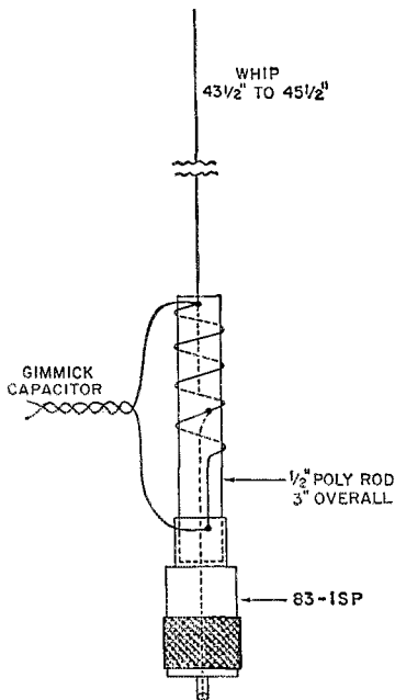
Fig. 1—The 5/8-wave 2-meter whip mounts in a poly rod, inserted in the top of a coaxial plug. Impedance matching coil is wound on the rod, and the line to the transmitter is tapped up one turn from the bottom end. The coil is tuned with a "gimmick" capacitor.
