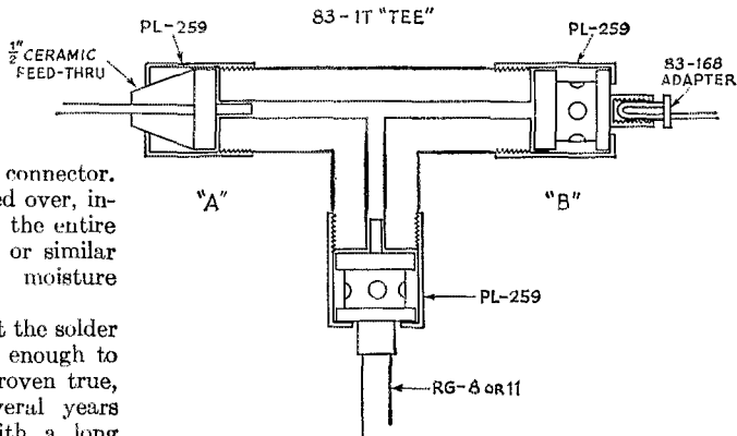
Fig. 1—Assembly of the center insulator constructed from coax connectors.
