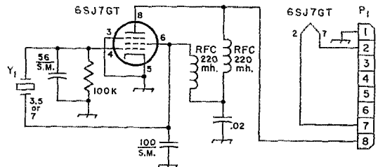
Fig. 3—Circuit for a crystal-oscillator adapter for Collins 32V series transmitters. Resistances are in ohms (K = 1000); decimal values of capacitance are in microfarads (μf.), others are in picofarads (pf.). SM indicates silver mica capacitors. P 1 is an octal plug.
