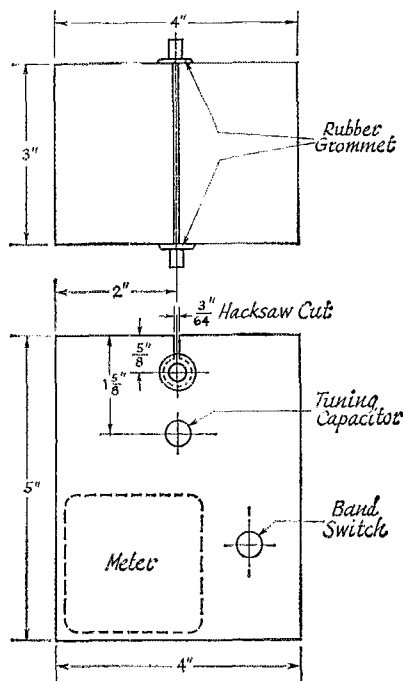
Fig. 2—Sketch showing mounting of ferrite through box and saw cut.
