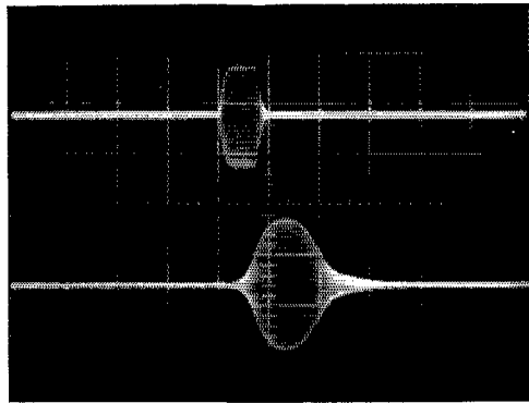
Fig. 1—Oscillograms of (above) 150- \mu second pulse at input to a 1-Mc. i.f. amplifier, and (below) the same pulse at the output of the amplifier. Amplifier bandwidth is 5 kc.; note delay and lengthening.
