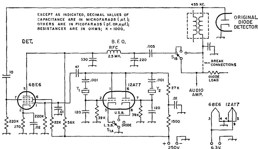
Fig. 1—Circuit of the product-detector adapter. Capacitors of decimal value are disk ceramic; others are mica or NPO ceramic. Resistors are \frac{1}{2} watt.
