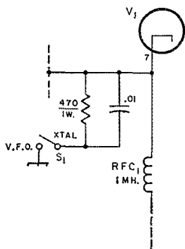
Fig. 4—Adding cathode bias to the crystal oscillator.
