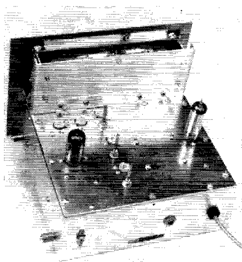
Rear view of the Heath HG-10 v.f.o. The oscillator tube is at the left. Trimmers for setting the various bands are just above the oscillator and in a line at its right.
