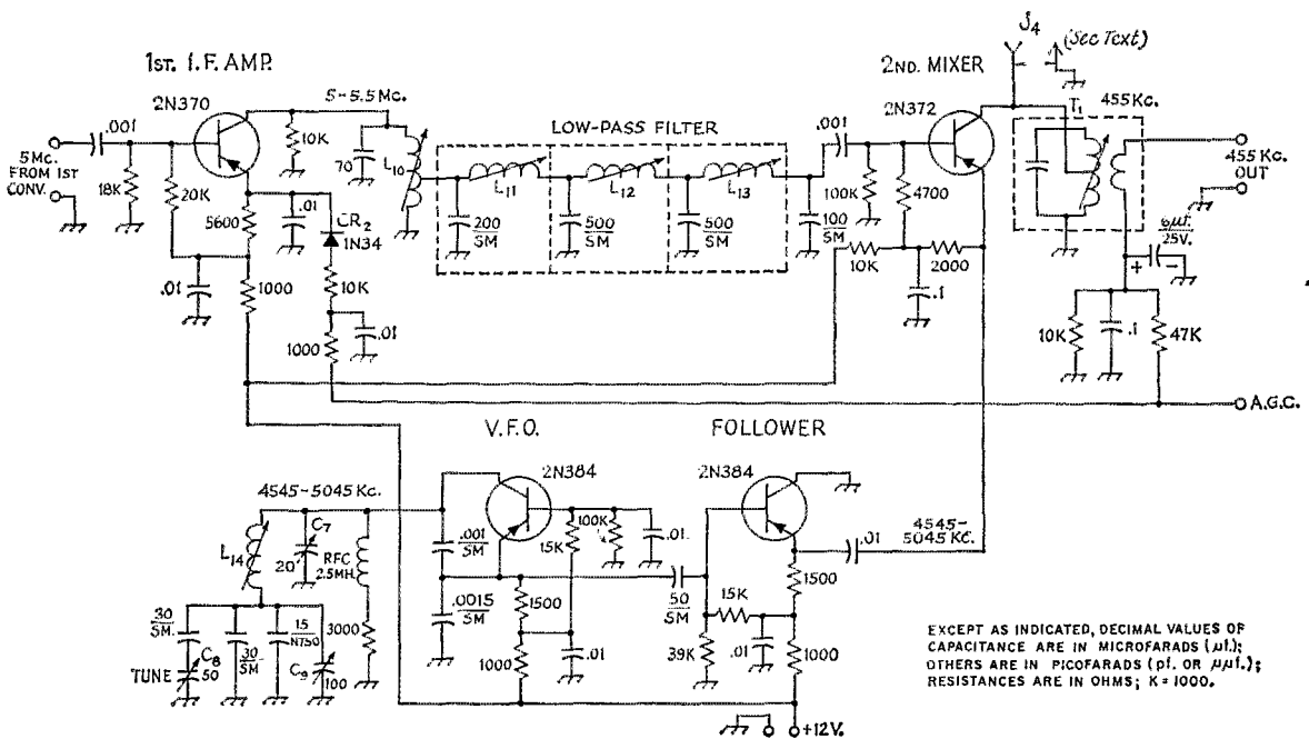
Fig. 2—First i.f. and second frequency-conversion circuits. Resistors are ½ watt. Fixed capacitors of decimal value are disk ceramic or mylar, except SM indicates silver mica; others are mica except SM again indicates silver mica; N indicates negative temperature coefficient, and polarized capacitors are electrolytic. Components not listed below are labelled for text-reference purposes.
