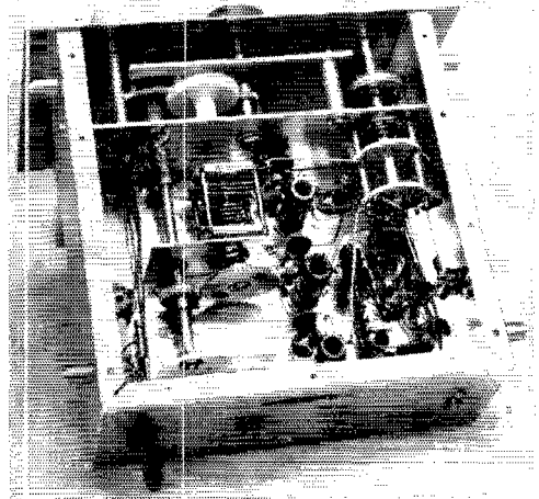
Bottom of the v.f.o., with its cover plate removed. The dial-driven main tuning capacitor is at the left center, with the three coils at its right. At the upper right is the band switch
