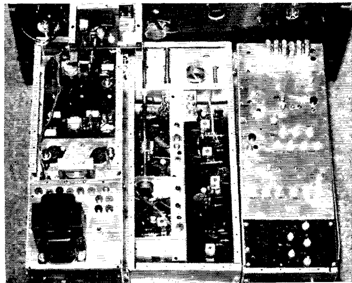
Rear-top view of the TDCS receiver with some of the shielding removed. The audio and power section is to the left. The center chassis is devoted principally to the i.f. circuitry, while the chassis to the right contains the h.f. stages. The v.f.o. compartment has been removed to expose the crystals and slug-tuned coils of the oscillator feeding the first mixer.
