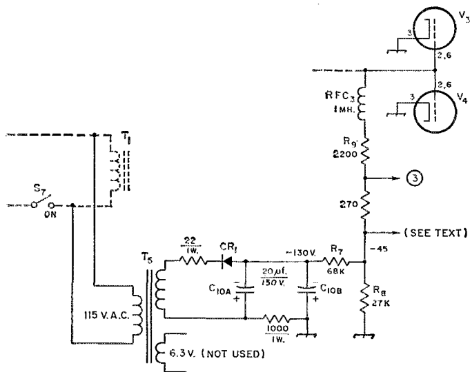
Fig. 1—Bias-supply circuit. Resistances are in ohms and, unless indicated otherwise, resistors are 1/2 watt.
