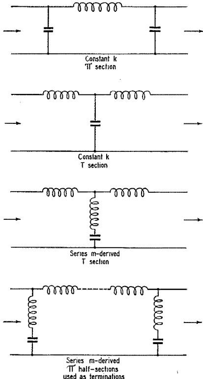
Fig. 9—Types of filter sections discussed in the text. In the lowest drawing, the dashed line between the two coils indicates that additional filter sections may be inserted. In case only one section is desired the two half-sections are simply connected together. The two coils may then be combined into one having twice the inductance of either.
