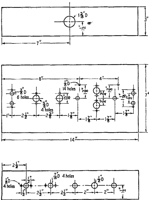
Fig. 4 — Layout drawing of the chassis for the 2-meter transmitter. The large view is looking down at the top of the chassis, with the front wall below and the rear wall above.
