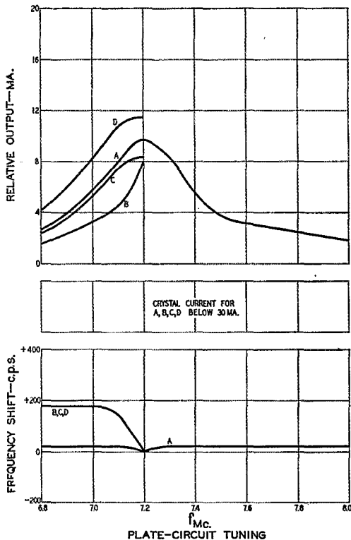
Fig. 5 — Crystal-current, frequency-shift and output data for the modified-Pierce oscillator. Feed-back capacitances ( C_s ) for the various tubes are: 6AG7 = 220 \mu\text{fd.} ; 6F6 = 40 \mu\text{fd.} ; 6V6GT = 50 \mu\text{fd.} ; 6L6 = 60 \mu\text{fd.}
