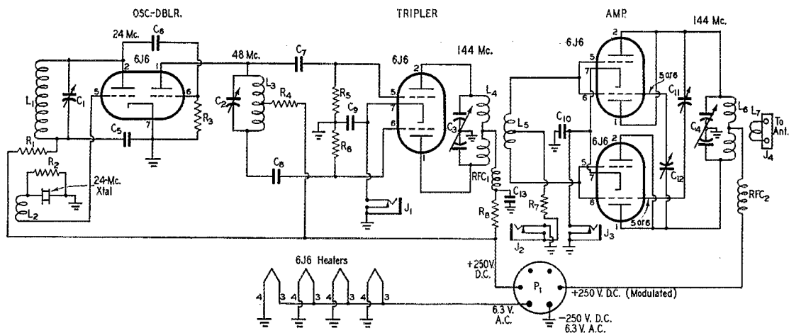
Fig. 3 — Wiring diagram of the 2-meter r.f. unit.
