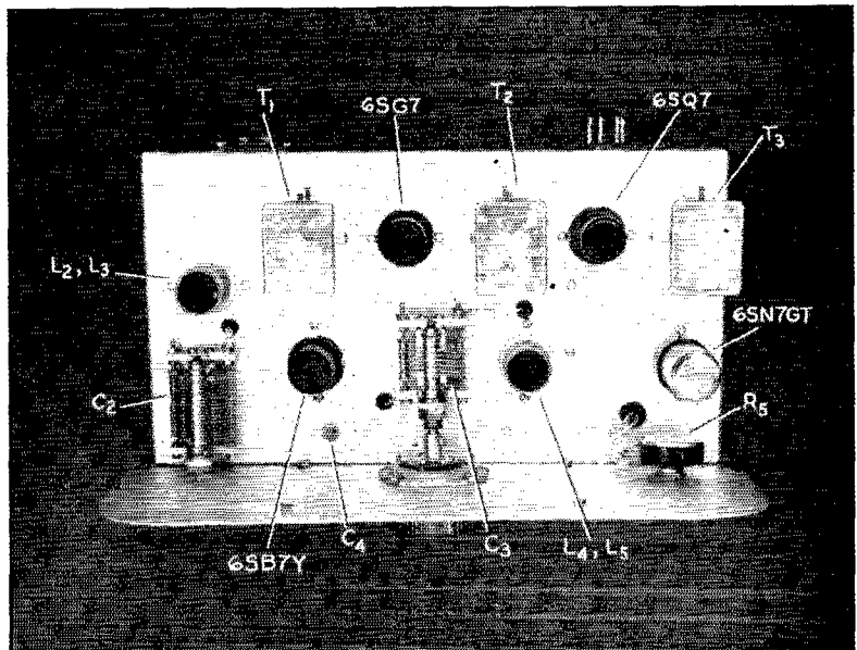
Rear top view of the beginner's superhet receiver showing the placement of parts on top of the chassis.
