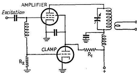
Fig. 1 — The clamp-tube circuit eliminates the need for protective fixed bias in a screen-grid amplifier by reducing the screen voltage when there is no excitation.
