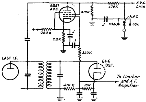
Fig. 2—The a.v.c. system used in the receiver. The 6SJ7 tube picks up the signal from the plate of the last i.f. stage. Delay bias is introduced in the cathode circuit across the 2200-ohm cathode resistor. When a signal develops at the 6H6 detector, some positive voltage is fed back to the grid of the 6SJ7, thus canceling out the delay bias and permitting an a.v.c. voltage to develop. The result is that the S-meter (which is controlled by the a.v.c. voltage) indicates on weaker signals than it would if a more conventional system were used.
