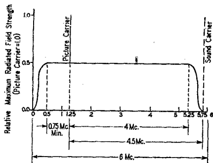
Fig. 1 — The television channel and ideal transmitter frequency characteristic for the picture signal.
