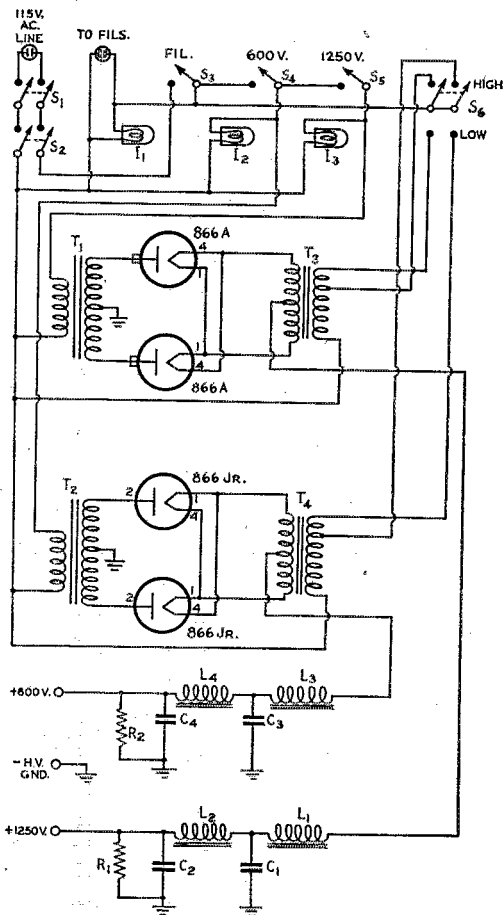
Fig. 4—Circuit diagram of the dual power supply for the medium-power handswitching transmitter, delivering 1250 volts at 550 ma. and 600 volts at 200 ma.
