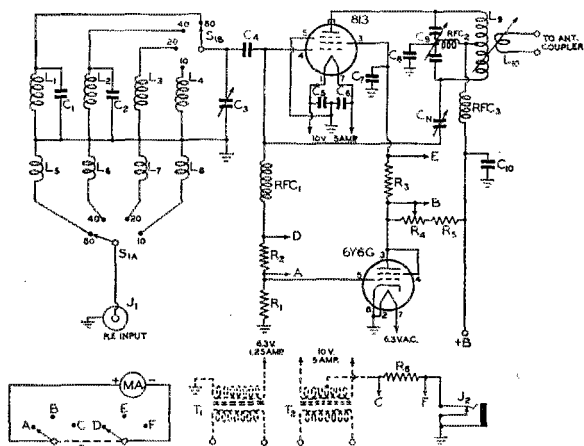
Fig. 1 — Schematic diagram of the 813 amplifier.
