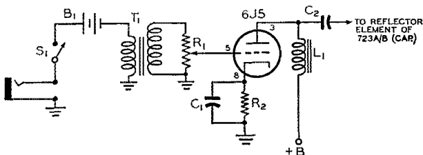
Fig. 5 — Circuit of the unit used for modulating the 723A/B oscillator.
