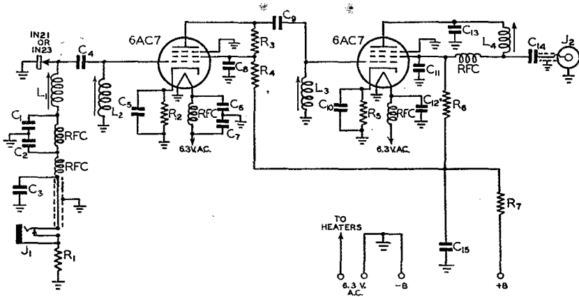
Fig. 2 — Schematic diagram of the 30-Mc. preamplifier.
