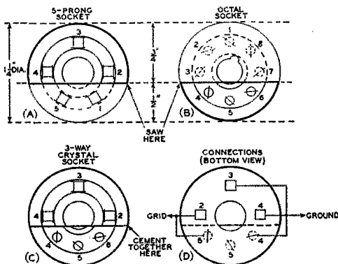
Fig. 4 — Method of constructing a 3-way crystal socket from portions of a 5-prong socket and an octal socket. The two are cut as shown in A and B, and are cemented together as shown in C. The socket connections to permit use of any of the three popular sizes of crystal holders are shown in D.
