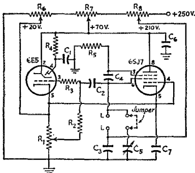
Fig. 1 — A wide-range transitron utility oscillator for the ham shack. The sliders on R_6 , R_7 and R_8 should be adjusted to give the voltages shown in the diagram.
