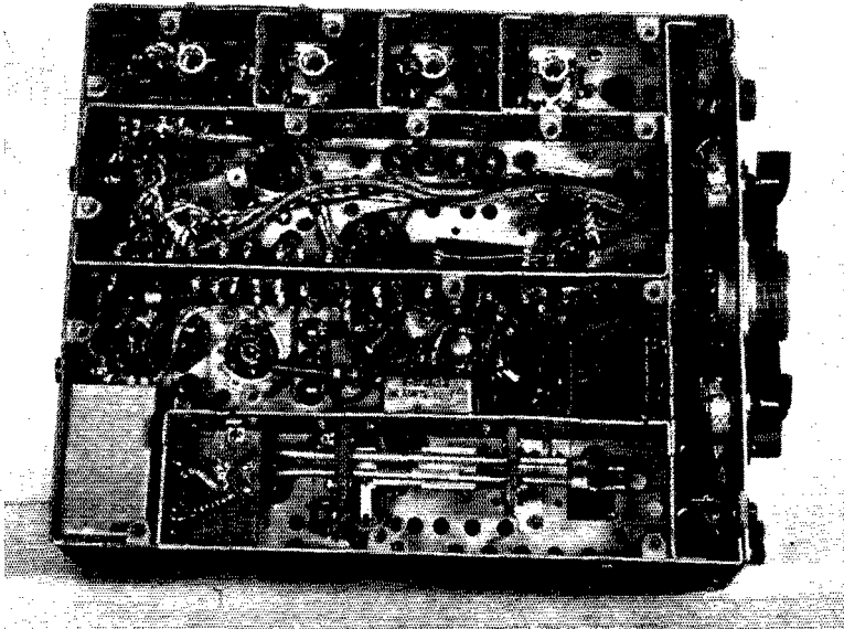
Bottom view of the converted unit. Relays, potentiometers, and other unused parts are removed. The transmitter oscillator line (bottom of photo) has been lengthened and a means of frequency adjustment added. The shielded compartments across the top of the unit are the slug-tuned i.f. stages in the receiver.
