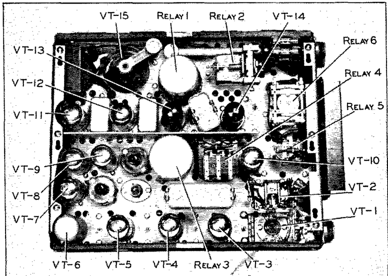
Top view of the BC-645 before conversion. Components mentioned in the text are indicated with designations which correspond to those used on the schematic diagram. Note that the 955 mixer tube, VT-1, is mounted bottom up.
