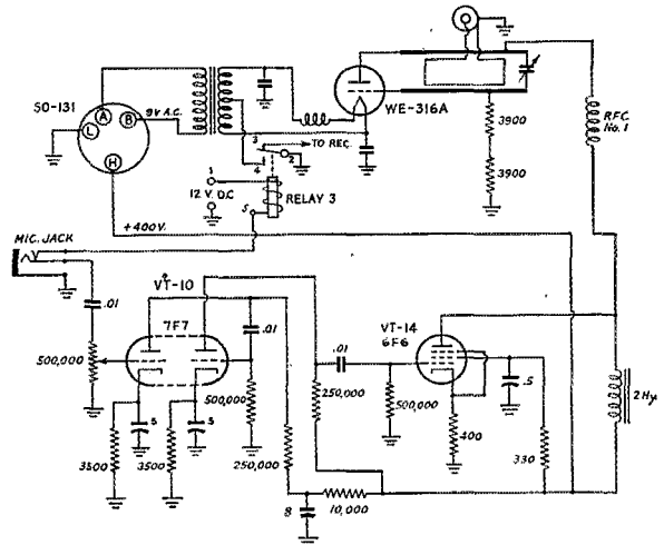
Fig. 3 — Wiring diagram of the oscillator, modulator and speech amplifier used in the converted BC-645. Like other portions of the conversion job these changes involve the use of tubes already in the unit.
