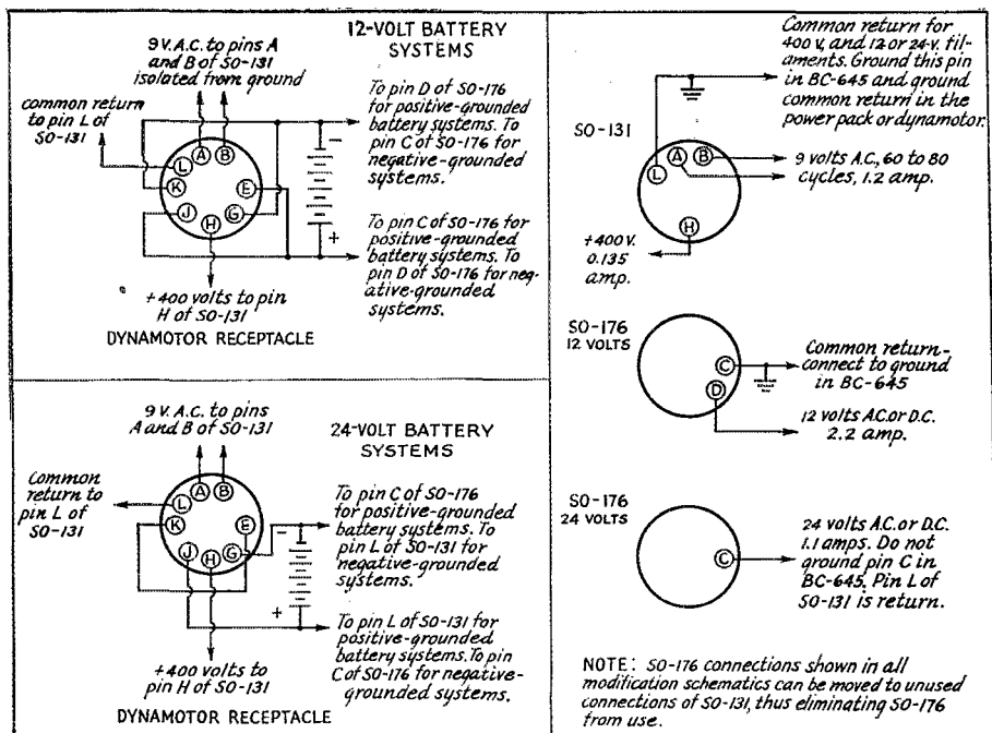
Fig. 5 — Power connections for the converted BC-645. At the left are the connections used for 12- and 24-volt battery operation. At the right are the connections used in a.c. operation.
