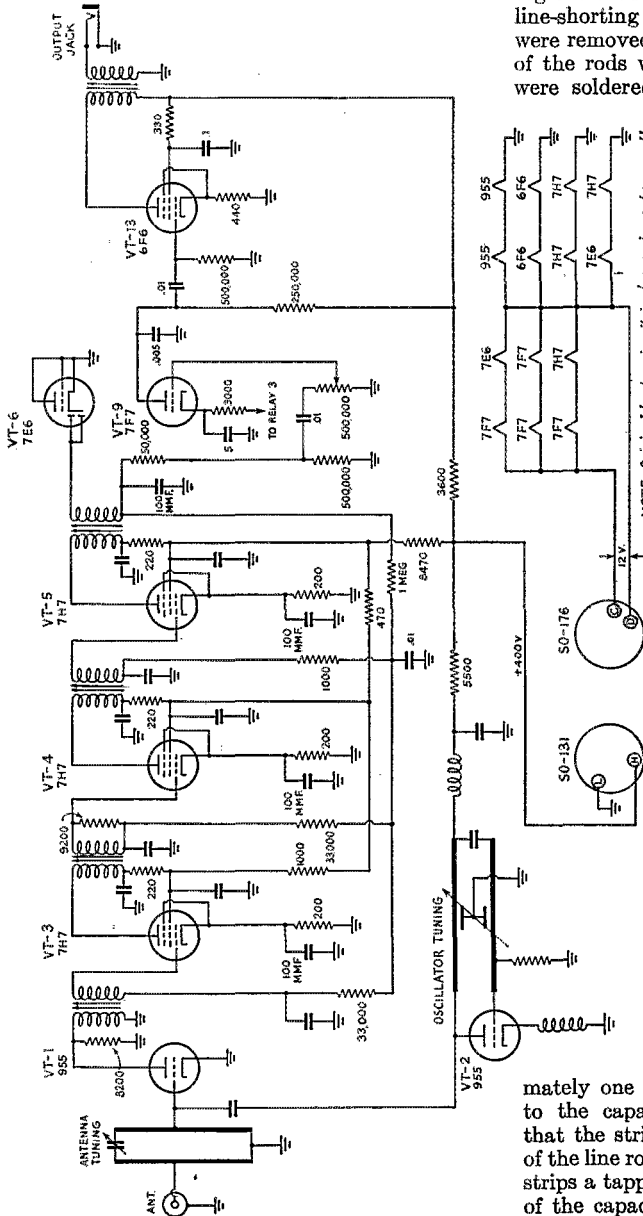
Fig. 2—Schematic of the receiver as converted for 420 Mc. Two stages of audio, employing tubes already in the unit, have been added. The oscillator lines are lengthened (see photo) and a.v.c. is incorporated.
