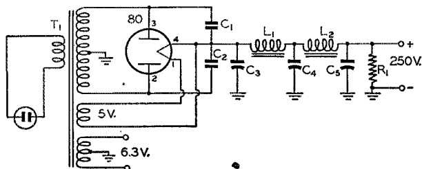
Fig. 2 — Circuit diagram of the receiver power supply.
