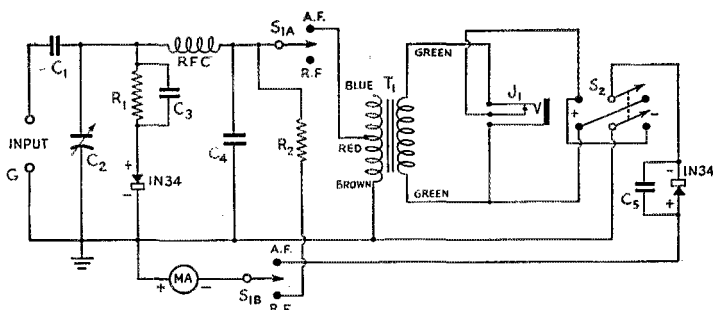
Fig. 1 —Circuit of the direct-reading modulation meter.
