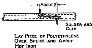
Fig. 3 — A splice between two pieces of 300-ohm Twin-Lead. The "staggered" joint adds strength to the splice.
