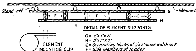
Fig. 3 — The element supports. These mount at right angles to the adder (indicated in cross-section at "F").
