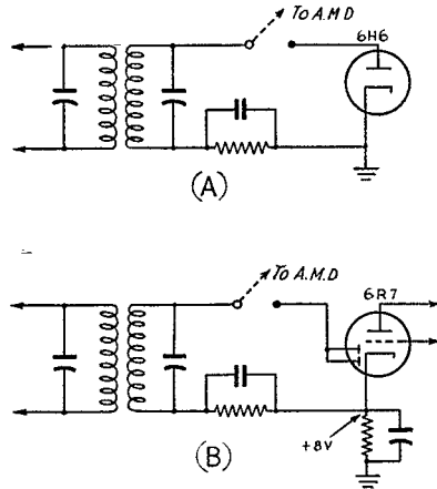
Fig. 6—Diode-detector circuit commonly used in receivers. The circuit at A uses a separate diode rectifier while that at B uses a combination diode-triode tube. In the latter case, the diode plates, in the absence of signal, are given a positive voltage with respect to the chassis by the voltage drop across the cathode resistor. This bias must be compensated in the adjustment of the A.M.D. adapter.
