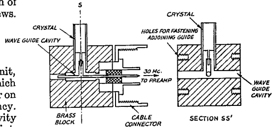
Fig. 2—Cross-section of the crystal mixer.
