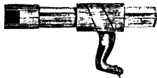
Phantom View showing how tapered shank of Nylon needle fits into tapered hole in Nylon chuck.
