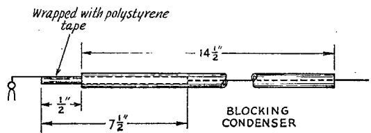
Fig. 4 — Construction of the plate blocking condenser. The inner tube has a diameter of \frac{3}{8} inch and, like the resonant line, should be silver-plated.
