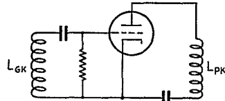
Fig. 1 — Fundamental oscillator circuit.
