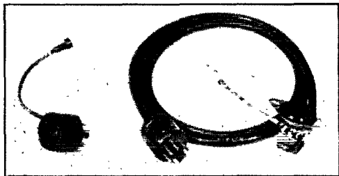
The adapter plug and extension cable. The 6IH6 socket, at the right, should be grounded at a convenient point on the receiver near enough to the second-detector socket to permit joining the pin-jack and prod.
