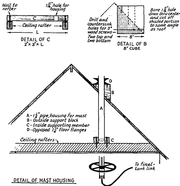
Fig. 1 — Sketch showing the attic housing, with the mast protruding through the operating-room ceiling and automobile steering wheel for turning the antenna. Dimensions of the housing and mast will depend on the individual location.
