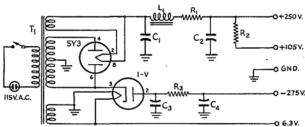
Fig. 2 — Power-supply wiring diagram.
