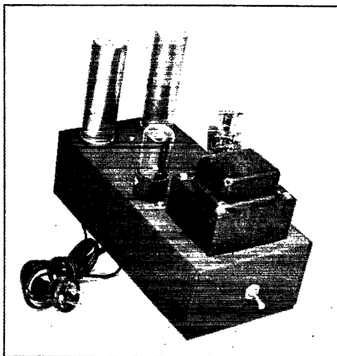
The power supply for the eight-tube receiver. Two rectifiers are required because a separate supply is incorporated for gain-control purposes. The filter choke and the negative-supply filter condensers are mounted under the chassis. At the rear of the chassis is the socket for the power cable.
