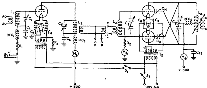
Fig. 1 — Schematic diagram of the 50-148-Mc., driver-amplifier using 35TGs.
