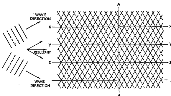
Fig. 9 — The fields of two traveling waves add at any point in space to give a resultant at that point having an amplitude and direction dependent upon the amplitudes and directions of the two component waves. This drawing represents a space distribution for a single instant of time. The two wave components, assumed to have equal amplitudes, are shown at the left, with the direction of propagation indicated. The resultant wave direction is shown by the small drawings between. Along lines such as XX, YY and ZZ the resultant amplitude always is zero, giving rise to standing waves in space.
