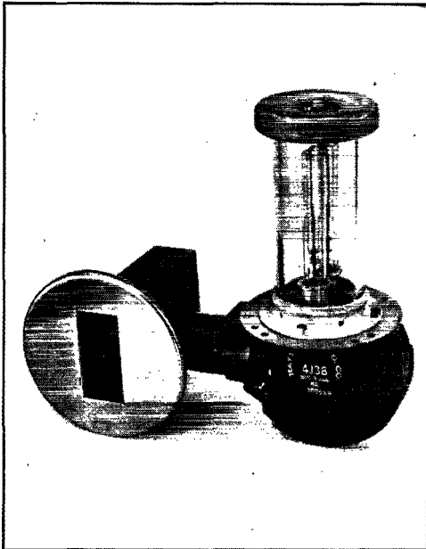
The 4J38 is a high-power "maggie" capable of a peak power output of 850 kilowatts at 3600 megacycles (8.3 centimeters). A pick-up loop in one of the anode cavities connects to a coaxial line which terminates in an antenna in the wave-guide section at the left. The ring at the top of the glass tube enclosing the cathode leads is a corona shield, required because of the high potential (30,000 volts) at which this tube operates. The over-all height is slightly over ten inches.
