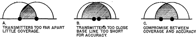
Fig. 8 — Effect of station placement on coverage available to navigators.
