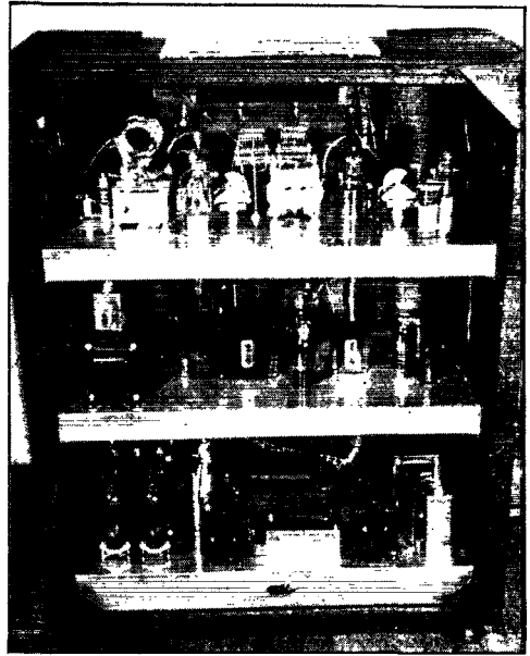
The three chassis of the complete transmitter are mounted on wall brackets along the side of the cabinet. Flexible cables pick up the tuning condensers and other controls on the transmitter chassis.
