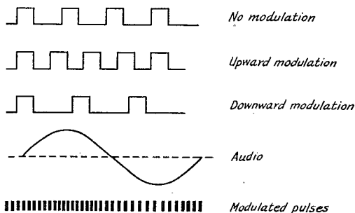
Fig. 2 — A pulse-modulation system using constant pulse length and varying the repetition rate in proportion to the modulation amplitude.
