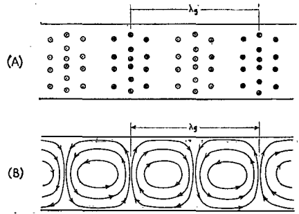
Fig. 13 — Instantaneous distribution of the electric field (A) and magnetic field (B) in a simple form of TE wave traveling through a rectangular guide. This is a view looking down on the wave, the side walls of the guide being represented by the horizontal lines. There is no component of the electric field directed along the guide (left to right) but the magnetic field does have such a component.
