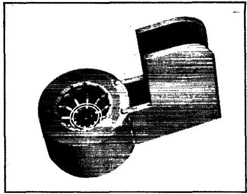
The insides of a 12-cavity 3-cm. magnetron shown actual size. The two rings inside the structure strap alternate cavities. The two fins are part of the cooling surfaces.
