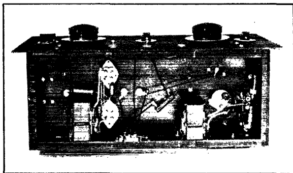
Under-chassis view of the 35TG driver-amplifier. Separate filament transformers are used for the two stages. The driver tube socket with its two filament r.f. chokes is at the right.
