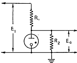
Fig. 1 — Typical simple voltage-regulator circuit for VR-type tubes.
