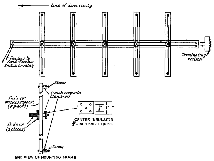
Fig. 1 — The experimental model of the Marconi-Franklin Series-phase Array. Any number of vertical sections may be used. The folded portions should be spaced as closely as possible — the 1/2-inch spacing shown is a convenient form. The array is unidirectional, toward the transmitter end.
