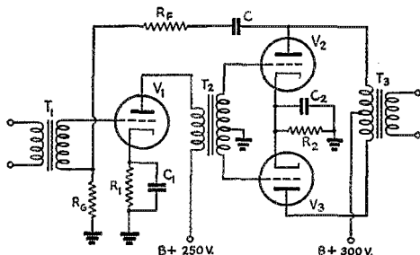
Fig. 5 — Feed-back over two stages in a transformer-coupled amplifier with push-pull output stage.
