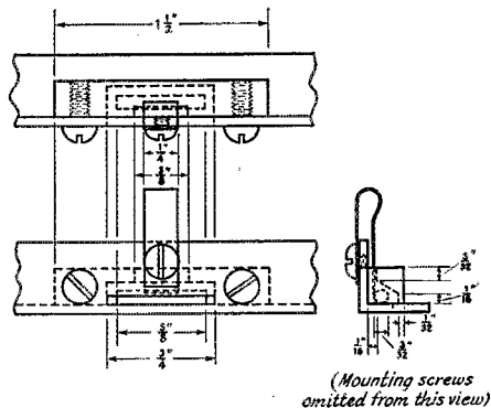
Fig. 8 — Dimension drawing of the puller assembly.
