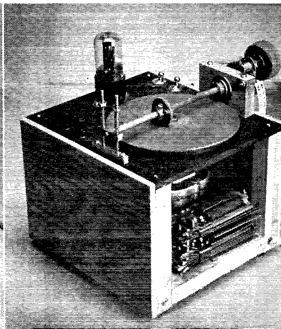
Fig. 11 — The bearing arrangement used allows the driving shaft to follow any wobble in the driving disc.
