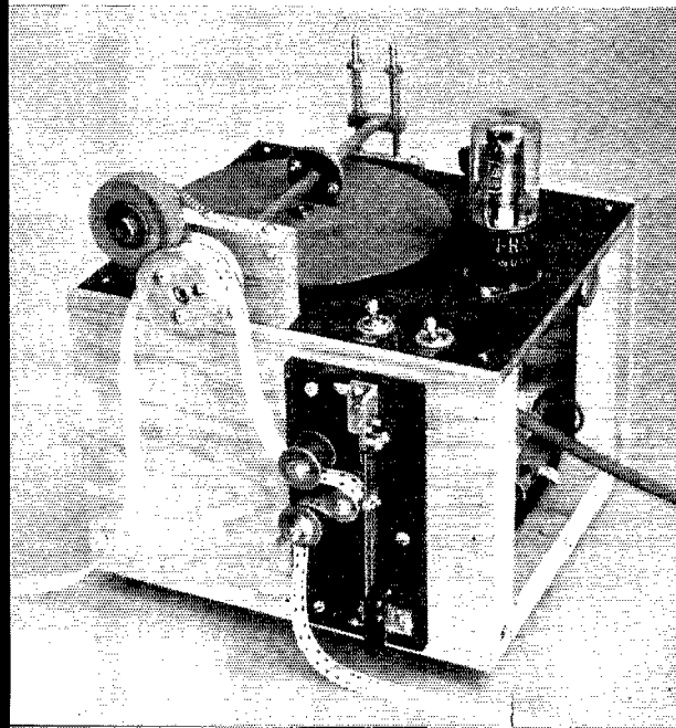
Fig. 10 — Front view of the rebuilt reproducer, showing the revamped tape-pulling system.
