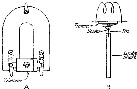
Fig. 2 — Substituting mica trimmers for air condensers in WERS gear. A shows the trimmer applied to the high-C horseshoe tank described in QST for December, 1941. The horseshoe is supported by three stand-off insulators, one at each end and one at the center of the curved portion. For the 112-Mc. band, the horseshoe should have an over-all width of 2 inches and length of 2½ inches. The opening at the center is ½-inch wide, making the width of the conductor ¾ inch. The inductance may be adjusted by changing the position of the trimmer on the horseshoe.
