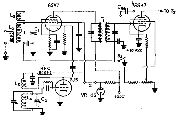
Fig. 1 — Changes to be made: Remove all connections from L_3 , take out C_{15} , run plate lead of i.f. transformer directly to plate connection of 6SA7. All parts not labeled are same as in original circuit.
