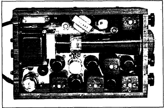
A top view inside the cabinet. The layout of components is described in the text.
