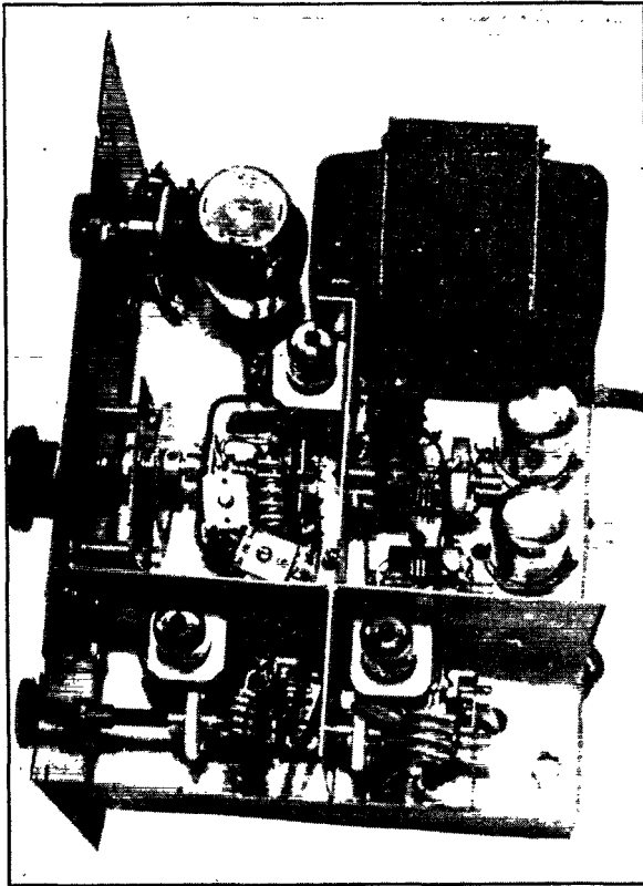
The neat, compact 112-Mc. superhet built by W6ANN. Oscillator is tuned by the vernier dial, center, with r.f. and mixer stages at the bottom of the photo. The two lock-in tubes at the rear are the superregenerative detector and audio stage.
