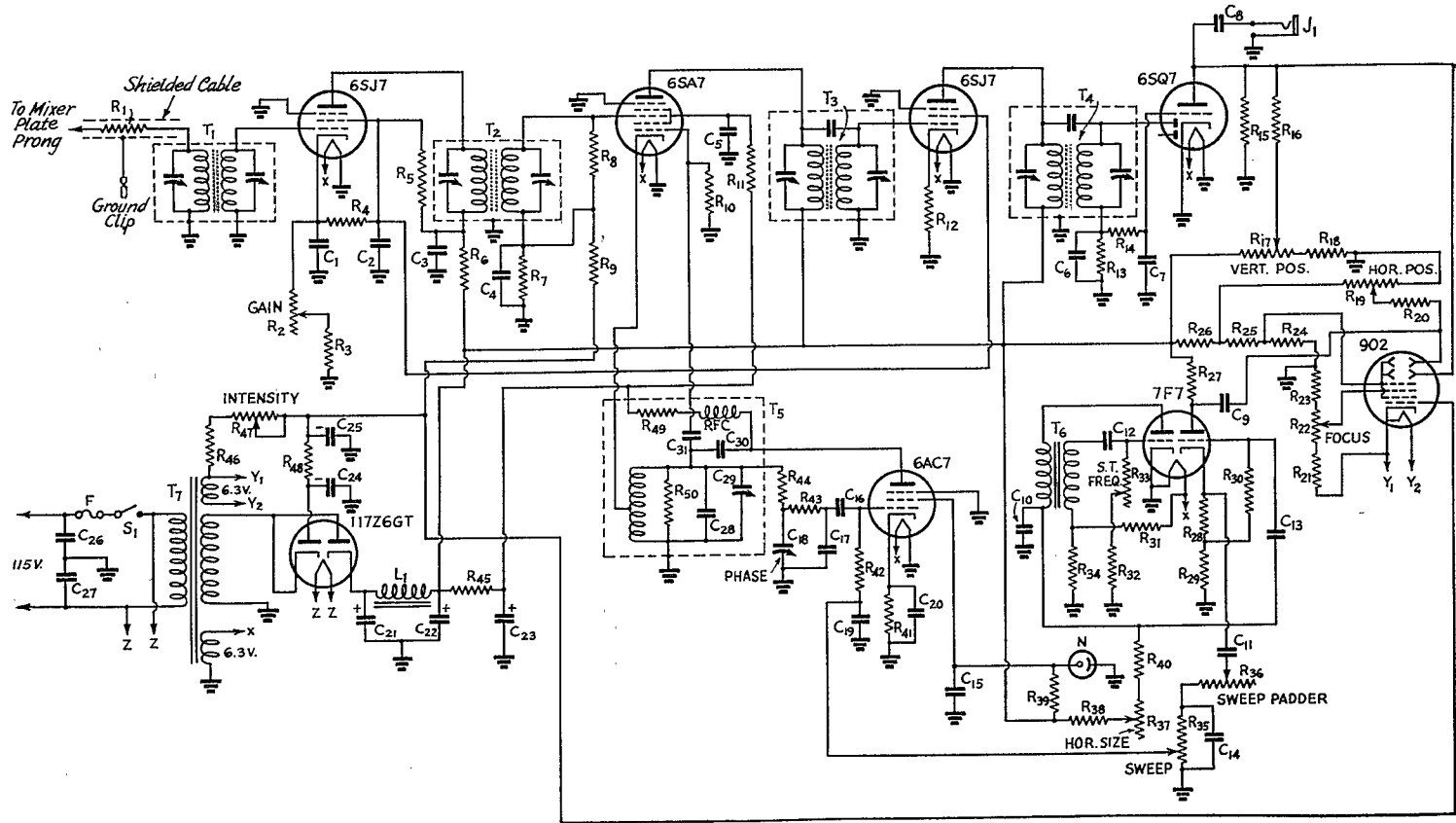
Fig. 1 — Circuit Diagram of the Panoramic Adapter.
