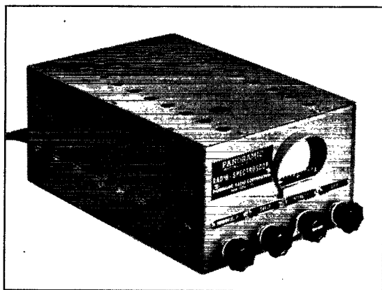
A compactly-built panoramic radio-spectroscope adapter, complete with power supply, which can be used with any communications receiver having an intermediate frequency in the 450-470-kc. region. The cathode-ray tube is the two-inch 902.
