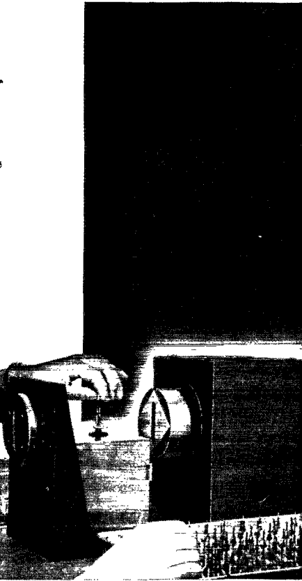
Observation of the stress points on glass bead seals around vacuum tube leads is made with this device. Close-up photo above shows the actual view of a faulty lead. Note the change in polarized light creating distorted shadows which show up stress and strain in beads. Such strain sometimes occurs where metal and glass are sealed together.
