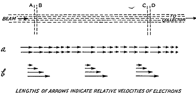
Fig. 2 — Velocity modulation of an electron stream.
