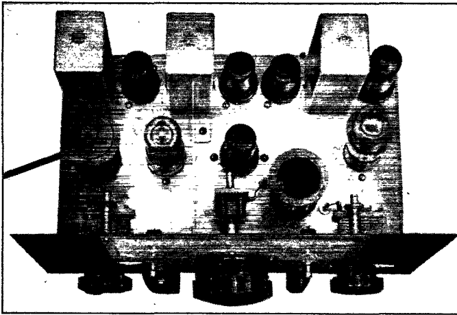
Top view of the seven tube regenerative superhet showing the broadcast-band mixer coil and the novel switch on its top. The new 100- \mu fd. tuning condensers can be seen at the right and left sides of the front panel.
