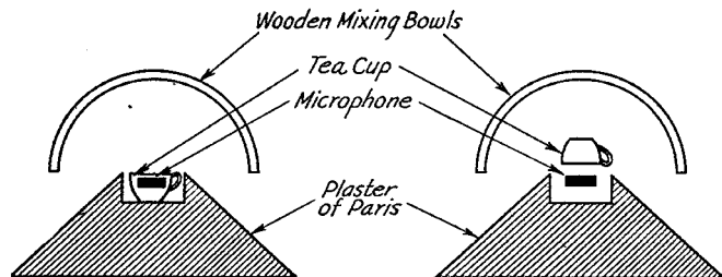
Fig. 2 — Another reflector system suggested by A. G. Redfield of Cambridge, Mass.
