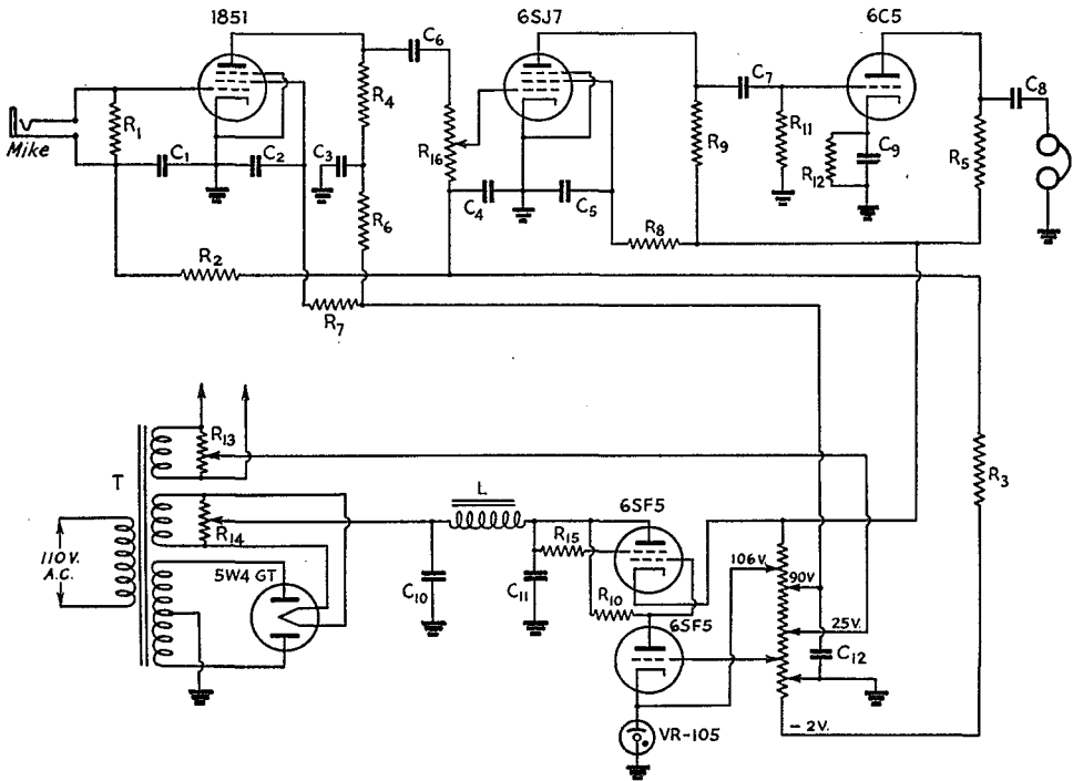
Fig. 3 — Circuit diagram of the high-gain audio amplifier
