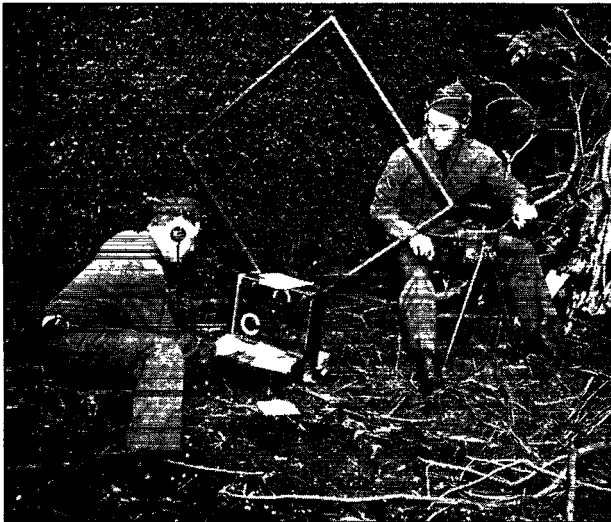
In the field the Signal Corps uses a wide variety of specialized portable equipment, operating from medium frequencies to the ultrahighs. Here a two-man team is seen operating a self-powered set.
