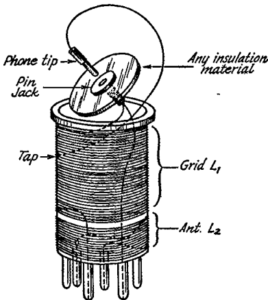
Fig. 2 — Layout of the b.c. band mixer coil.
