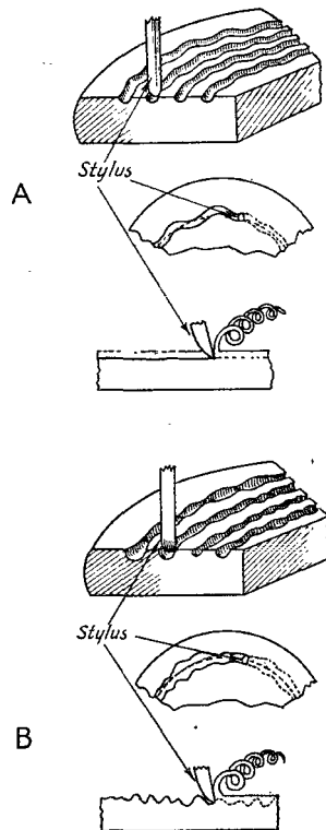
Fig. 3 — (A) Lateral recording, as used in phonographic and most instantaneous recordings. The stylus cuts a groove of constant width and depth but moves from side to side in accordance with the frequency and amplitude of the signal being recorded.
