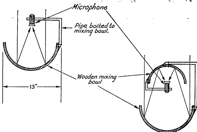
Fig. 1 — Arrangement of "mixing-bowl" acoustic reflectors used by B. C. Barbee of Jackson Heights, L. I.
