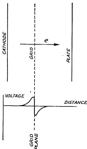
Fig. 1 — Voltage induced in grid by a moving electron, the mechanism by which transit-time effects arise.
