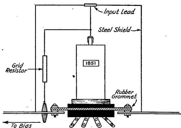
Fig. 4 — Sketch showing method of assembling the 1851 stage of the high-gain audio amplifier.
