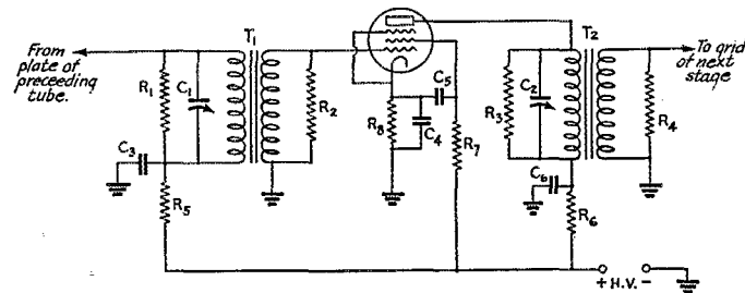
FIG. 4—THE CIRCUIT OF A SATISFACTORY I.F. STAGE
