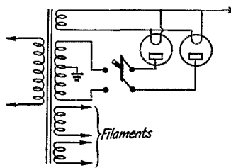
FIG. 5—SWITCHING THE PLATE WINDING ON A COMBINATION TRANSFORMER SO TUBES CAN BE HEATED BEFORE APPLICATION OF PLATE POWER
