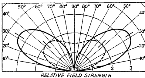
FIG. 4—COMPUTED RADIATION CHARACTERISTICS IN THE VERTICAL PLANE FOR A SINGLE HALF-WAVE ANTENNA (DASHED) AND A 2-SECTION FLAT-TOP (SOLID) BOTH AT A HEIGHT OF THREE-EIGHTHS WAVELENGTH ABOVE GROUND
