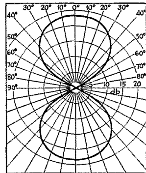
FIG. 5—MEASURED HORIZONTAL RADIATION PATTERN OF SINGLE-SECTION FLAT-TOP ANTENNA
