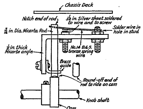
FIG. 2—AUXILIARY CAM SWITCH
