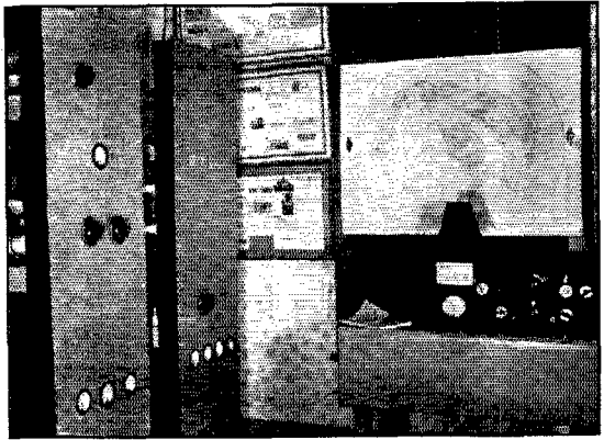
W9RCQ Wm. G. Baird, Jr., W9RCQ, E. St. Louis, Illinois, worked 276 stations in 56 sections, rolling up a score of 30,912. Behind the panels is an 80Z oscillator, 100TH buffer-doubler and 150T final. A kilowatt is pushed in on 7 and 14 Mcs. The crystal is keyed for break-in. A rotary beam is the radiator on 14 Mc., a doublet on 7 Mc. The receiver is an NC101X, an SW3 being available for portable and standby use.
