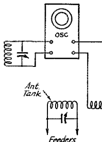
FIG. 3—USING AN OSCILLOSCOPE WITHOUT SWEEP CIRCUIT FOR MEASURING MODULATION
