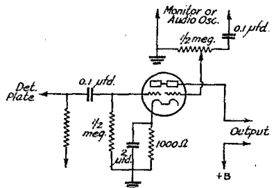
FIG. 5—USING A TWIN TRIODE FOR INTRODUCING THE MONITOR SIGNAL INTO THE RECEIVER OUTPUT
