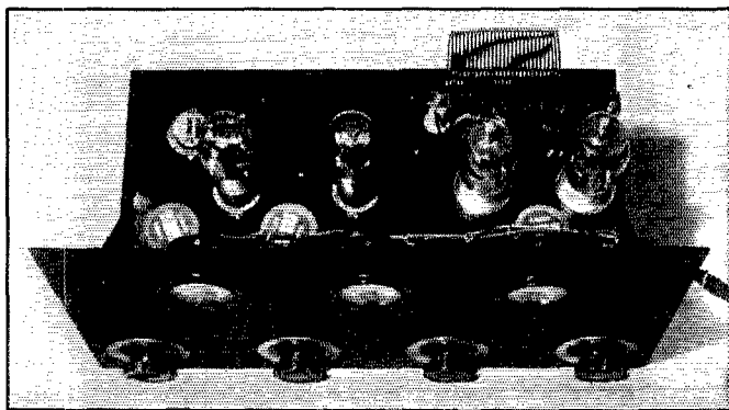
THE BEAM-TUBE R.F. UNIT USING 6L6G TUBES IN THE OSCILLATOR AND BUFFER STAGES, AND A PAIR OF RK-39'S IN THE PUSH-PULL FINAL AMPLIFIER
