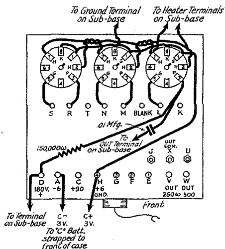
FIG. 4—REVISED WIRING OF THE PRE-AMPLIFIER WITH 6CS METAL TUBES
