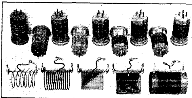
COMPLETE SET OF COILS FOR ALL FIVE BANDS
