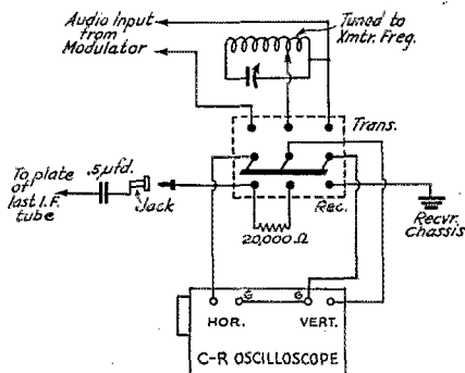
FIG. 1—SWITCHING CIRCUIT TO USE THE CATHODE-RAY OSCILLOSCOPE FOR CHECKING BOTH TRANSMITTER AND RECEIVED SIGNALS
