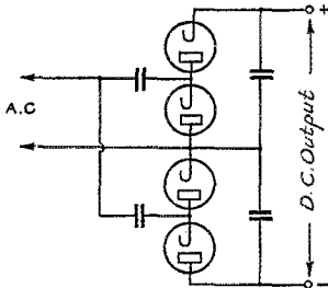
FUNDAMENTAL CIRCUIT
