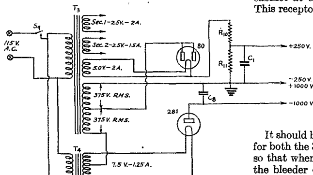
FIG. 3 — CIRCUIT OF THE POWER SUPPLY UNIT. THE TWO SEPARATE HALF-WAVE RECTIFIERS ARE SUPPLIED BY THE ONE TRANSFORMER SECONDARY
