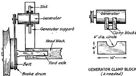
TOP VIEW SHOWING METHOD OF SUPPORTING GENERATOR
