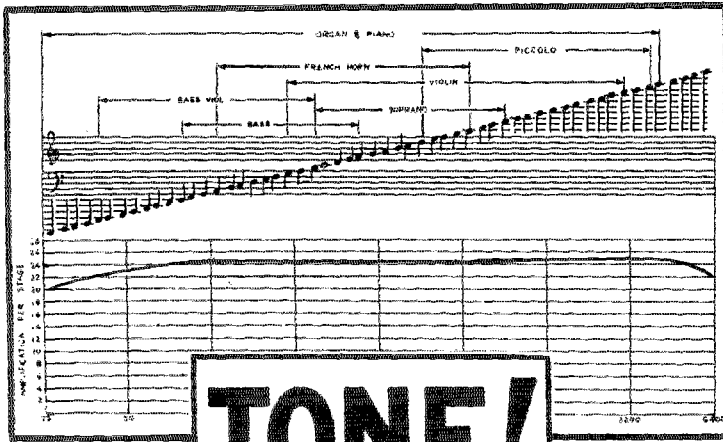
Curve of Type "A" or Sangamo Straight Audio Transformer showing uniformity of amplification at all available frequencies.
