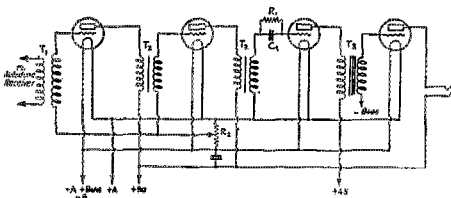
FIGURE 2. THE CONNECTIONS OF THE AMPLIFIER ILLUSTRATED IN FIGURE 1
