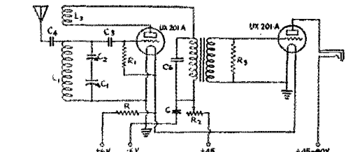
FIG. 4. THE SIMPLE WIRING OF THE TWO-TUBE SET
