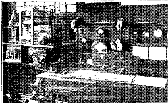
AMATEUR STATION 6b4FT, OWNED AND OPERATED BY GEORGE NEELEMANS, TRAFFIC MANAGER OF THE RESEAU BELGA AT BRUSSELS, BELGIUM, is one of the most widely known amateur stations in the world. The circuits is a Meeny, with two 150-watt Mullard valves. An Esco motor generator supplies 1100 volts for them. The antenna is a half-wave Zeppelin working on 32 meters. All instruments are Westons, and the receiver is a Grebe CR-18. These, with the Esco m. g. and the Vibronlex key 6b4FT, to use the words of its owner "rather a Yank station in appearance!"
