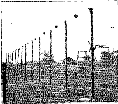
A MULTIPLE TUNED ANTENNA FOR SHORT WAVES
