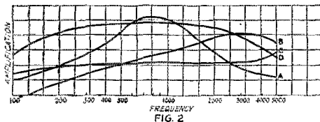
CURVES OF REPRESENTATIVE TRANSFORMERS UNDER NORMAL CONDITIONS
