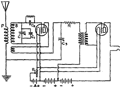
FIG. 1. THE CR-18 CIRCUIT C—Maximum of 130 \mu fd. C1—Vernier of 3 \mu fd. maximum capacity. C2—40 \mu fd. CR—226 \mu fd. R—25,000 ohms. R1—10 ohms.
