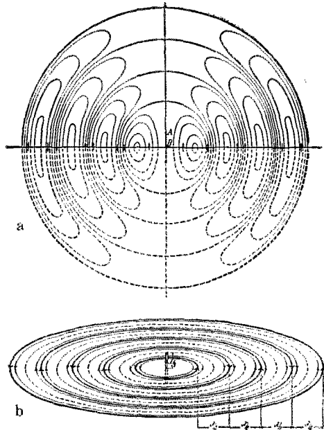
FIG. 1. THE FIELDS ABOUT A VERTICAL HERTZIAN ANTENNA a—The electrical field, sometimes mis-called the static field. b—The magnetic field. Both are present at the same time and place; both are expanding with the speed of light.—Zenneck-Seeling "Wireless Telegraphy".
