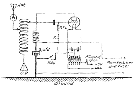
FIG. 3 WHEN USING A COUNTERPOISE
