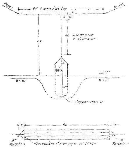
THE "NUMBER TWO" ANTENNA Fundamental to earth 262 meters FIG. 8
