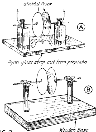
FIG. 8 AIR CONDENSERS FOR USE AT HIGH FREQUENCIES
