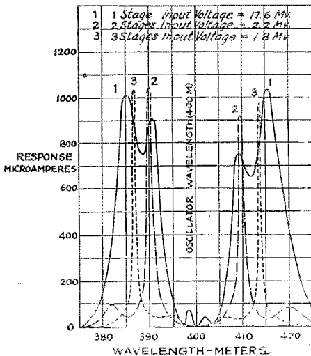
FIG 6 WAVELENGTH-RESPONSE CURVES Constant Input Voltage GR Transformers
