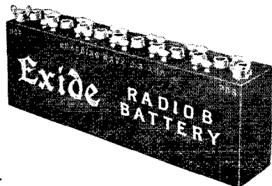
Famous Exide "B" battery for smaller sets. 24-volt, 4000 milliamper hours capacity. $10.00 f. o. b. Philadelphia.
