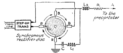
CIRCUIT USED TO "MUFFLE" COTTRELL PRECIPITATOR.
