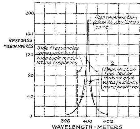
FIG. 5 WAVELENGTH-RESPONSE CURVES Constant Input Voltage GR Transformers 3 stages.
