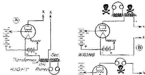
FIG. 5 MEASURING WITHOUT A MILLIAMETER OR GALVANOMETER GOOD FOR A.C., PARTLY FILTERED R.A.C. OR UNFILTERED GENERATOR
