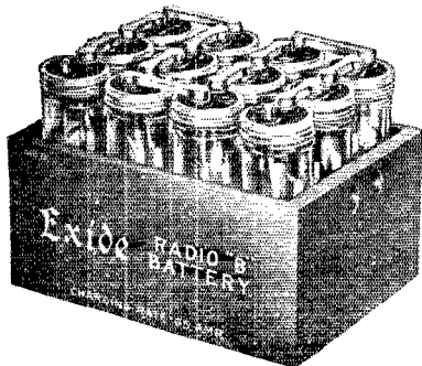
New 24-volt Exide "B" battery in glass jars. 6000 milliamper hours capacity. Also made in 48-volt size. Prices $12.00 and $23.30 respectively, f. o. b. Philadelphia.
