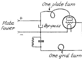
Series-feed Hartley cut down.
