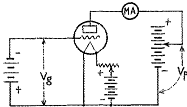
FIG. 3 FINDING THE AMPLIFICATION CONSTANT \mu
