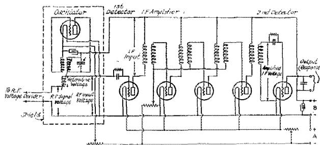
FIG. 1 CIRCUIT DIAGRAM
