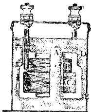
Cross section view of the Receptrad Super-Heterodyne Transformer, type 1716.
