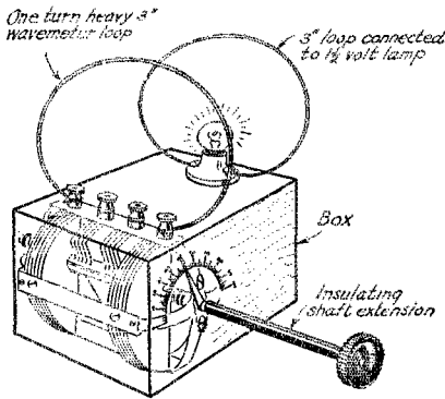
FIG. 5 A 5-METER WAVEMETER
