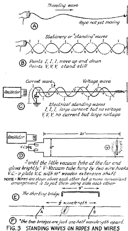
FIG. 3 STANDING WAVES ON ROPES AND WIRES
