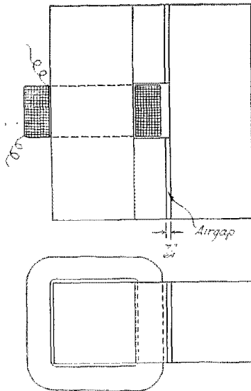
FIG. 5 30 HENRY CHOKE COIL
