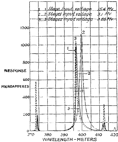
FIG 7 WAVELENGTH-RESPONSE CURVES Constant input Voltage DX Transformers
