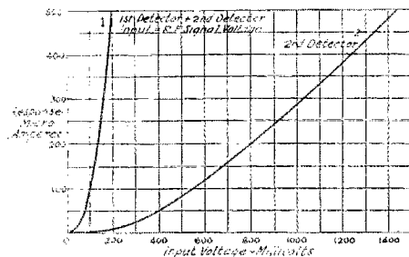
FIG 2 INPUT - RESPONSE CURVES
