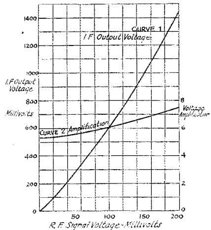
FIG 3 FIRST DETECTOR
