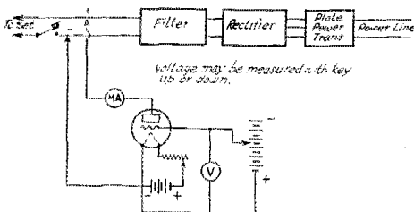
FIG. 4 MEASURING PLATE VOLTAGE OF SENDING SET
