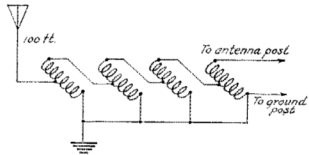
STATIC DRAIN COIL SYSTEM
