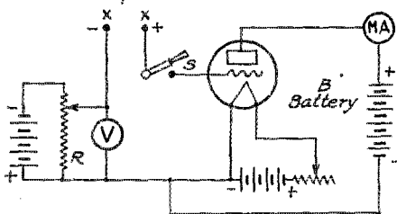
FIG. 2 A ZERO-PLATE-CURRENT METHOD
