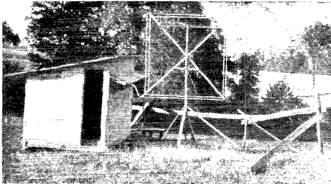
THE RECEIVING HOUSE WITH ITS LOOP This station was described in part one of this article.
