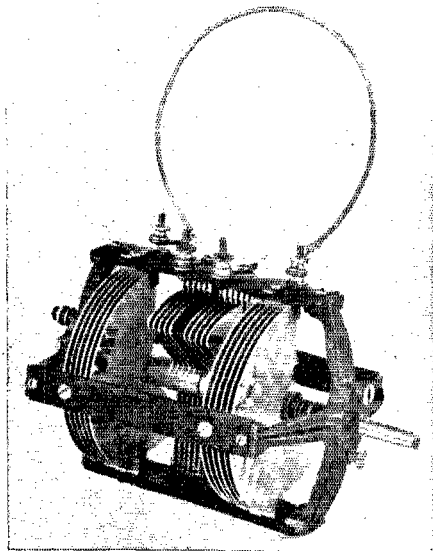
THE 5-METER WAVEMETER
