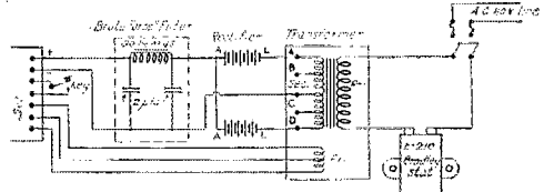
FIG. 4 HOW TO CONNECT THE TRANSFORMER, RECTIFIER AND FILTER TO THE SET
