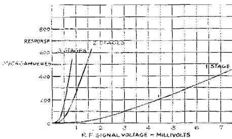
FIG. 4 INPUT-RESPONSE CURVES
