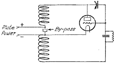
Ordinary Series-feed Hartley
