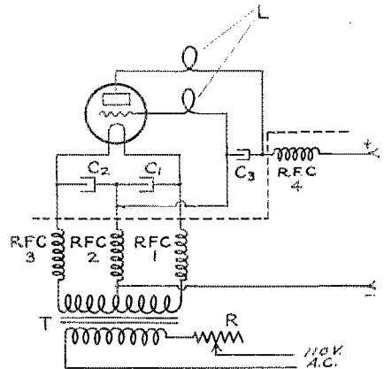
5 METER OSCILLATOR CIRCUIT
