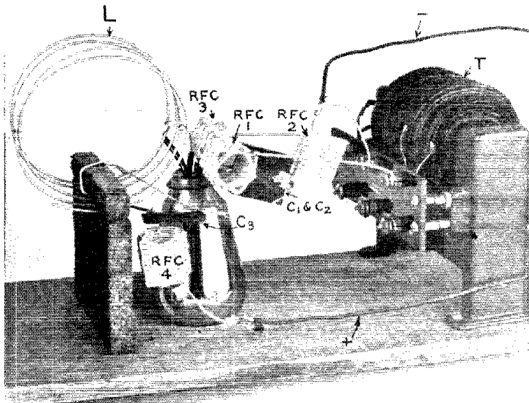
DETAIL OF THE OSCILLATOR, SHOWING CHOKES AND CONDENSERS.
