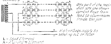
HOW TO CONNECT THE RECTIFIER JARS
