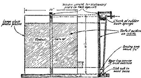
VARIABLE CONDENSER Suggested by F.C. Beckley I.A.E.L. FIG. 4
