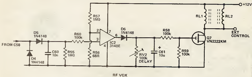
Fig 4. The circuit diagram for the RF metering.
