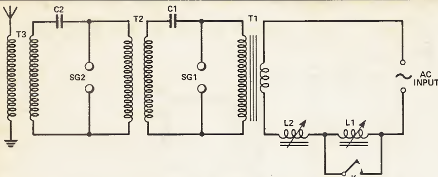
Fig. 4 The circuit of the Poldhu transmitter. The AC input supplied by a 25kW Mather and Platt alternator delivering 2000V at 50Hz was stepped up to 20000V by the transformer, T1, and fed to the primary of the oscillation transformer, T2, via C1 which then discharged across the spark gap, SG1. The secondary of T2 in turn charged C2 via the primary winding of T3. C2 then discharged across the second gap, SG2, exciting the serial and earth system via the secondary winding of T3. Keying was effected by short circuiting one (or both) of the variable choke coils L1, L2. The wavelength of the transmitter was calculated to be about 366m.
