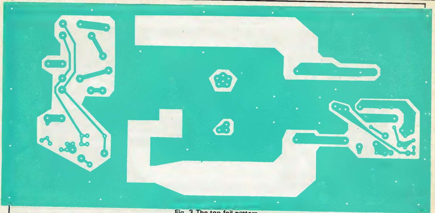
Fig. 3 The top foil pattern.
