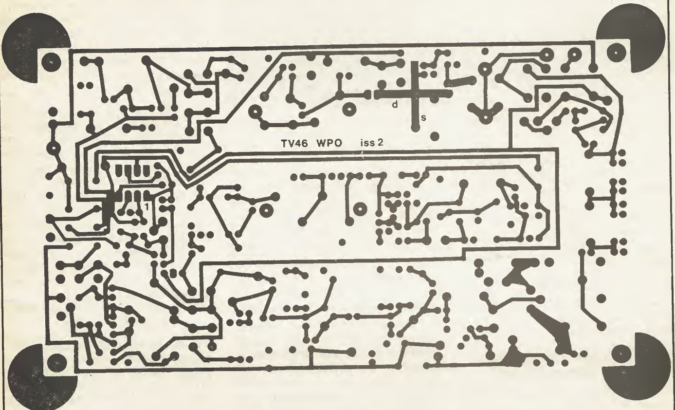
Fig. 2 The foil pattern for the transverter.
