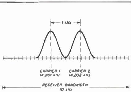
Fig. 7. Two carriers close to one another will produce a beat note that is directly related to their frequency separation. In this case, they are 1 kHz apart, thus you'll hear a 1000-hertz tone when they are both on.
