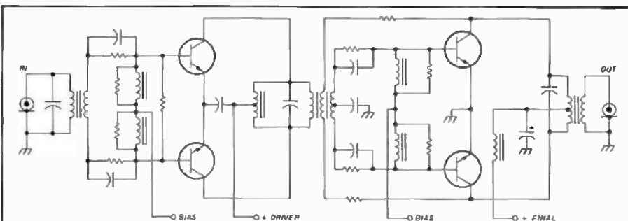
Fig. 10. The push-pull circuitry of this driver and final amplifier stage bears a slight resemblance to that found in older rigs, but note the lack of tuning capacitors; it's all done by impedance matching.
