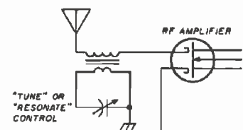
Fig. 4. The receiver rf amplifier, or input stage, is tuned by a front-panel control for better rejection of out-of-band signals and noise.
