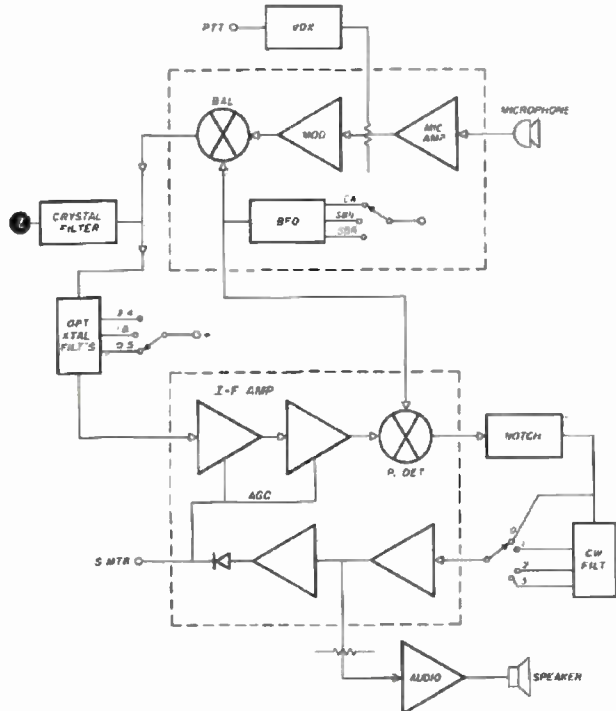
Fig. 8. A modern transceiver is a joy to use, but that convenience does not come easily. This block diagram of the Ten-Tec OMNI-D shows what it takes to pack all those marvelous functions into one neat box.
