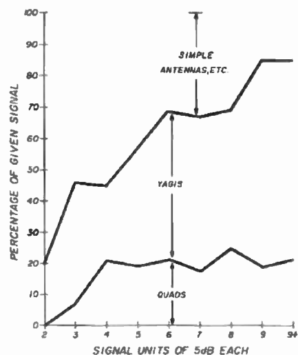
Fig. 3. Percentage of two types of beam antennas giving a stated signal strength.
