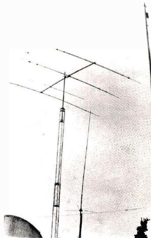
View of author's antenna farm. Mast at right supports an inverted V antenna now used for the 7-MHz band. It is the predecessor of the ATB-34 tribander in the background. Antenna in the center is a collinear vertical used for 2 meters.
