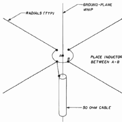
Fig. 5. Inductive match for ground-plane antenna.
