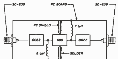
Fig. 4. The Test filter was built up on a section of PC board. Coaxial receptacles and a shield plate were soldered to the board, as were the ground ends of the inductors.
