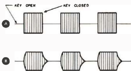
Fig. 2. A quick rise-time when you close your key looks nice on paper, A, but the sudden transition from rising to the steady "on" condition is similar to a square wave, which is full of harmonic energy and causes key clicks near your signal. A small amount of delay in the turn-on and turn-off, B, will soften the transition, and eliminate the clicks. If you go too far in softening the waveform, the code will run together and be impossible to copy.
