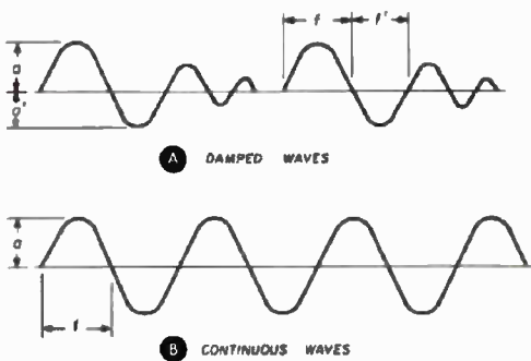
Fig. 3. Spark transmitters put forth a damped wave, as in A. Note that the amplitude, a , a' , changes, as does the frequency, f , f' , when the energy in the circuit dissipates. In modern oscillator circuits that use tubes or transistors, the energy is replenished so that the amplitude and frequency remain constant — or continuous, B. Therefore, it is called a continuous wave , even though you are keying the transmitter in a dot or dash sequence.
