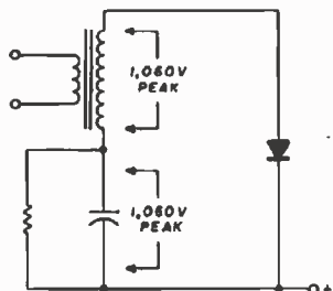
Fig. 8. Redrawn and simplified version of Fig. 3 showing how the diode PIV is actually 2.82 \times E_{rms} .
