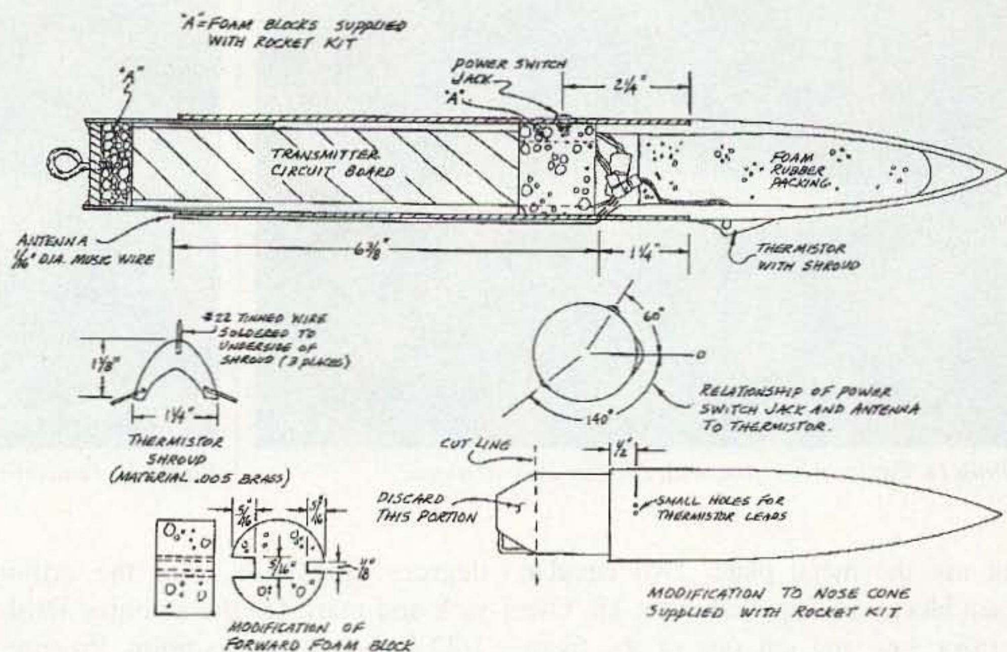
Fig. 6. Rocket assembly.
