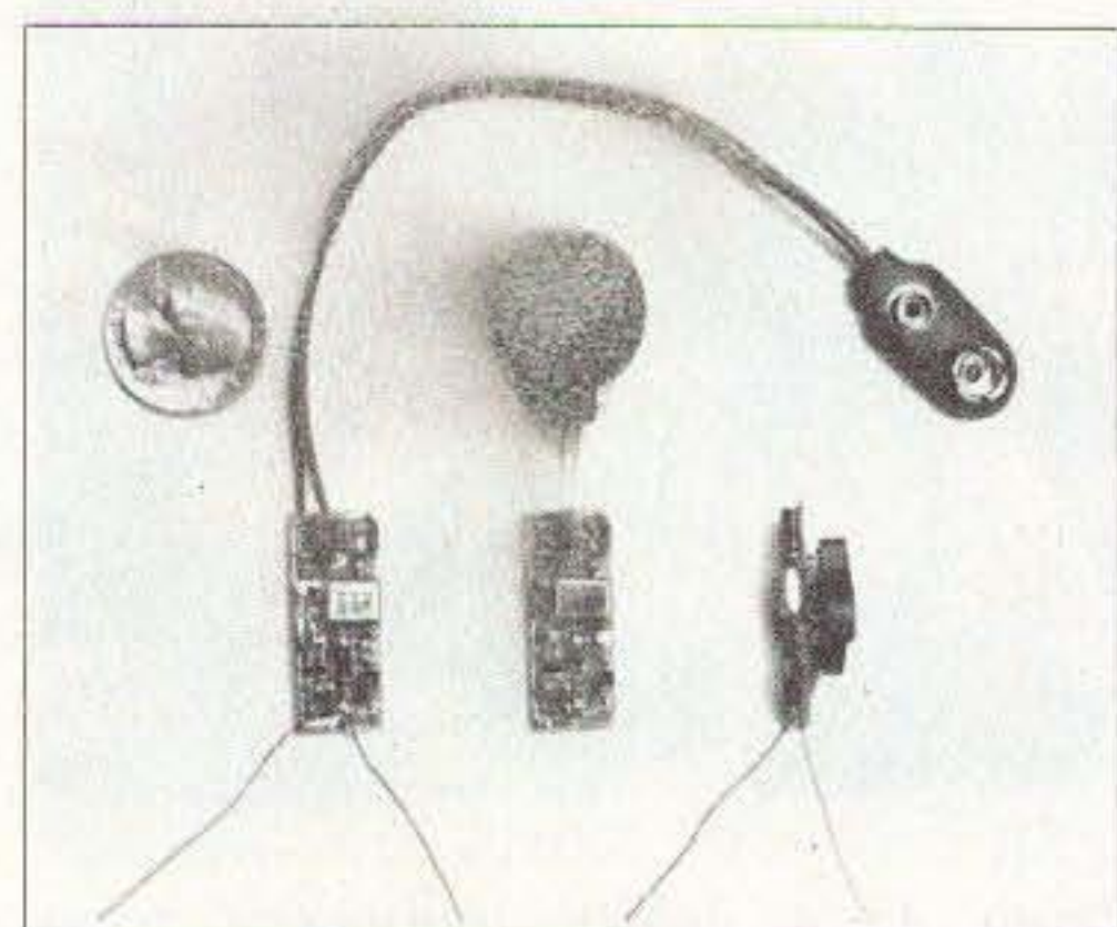
Photo C. Whether for sport or for covert tracking, the biggest part of a tiny hidden transmitter is sometimes the battery. These transmitters, designed by Ken Bauer of Airtek, were featured in previous "Homing In" columns.
