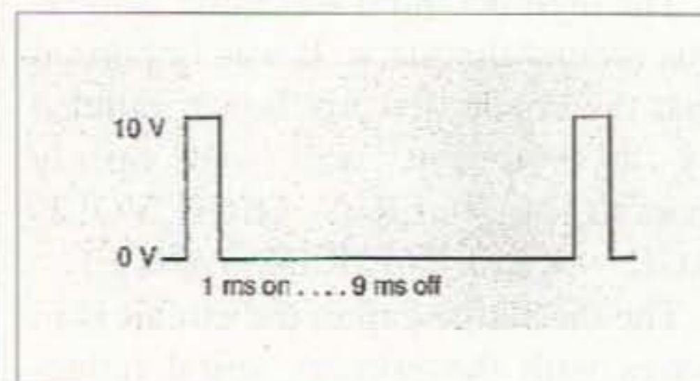
Fig. 1 An example using a 10 V DC pulse with a 10% duty cycle, applied to a 1-ohm resistor.
