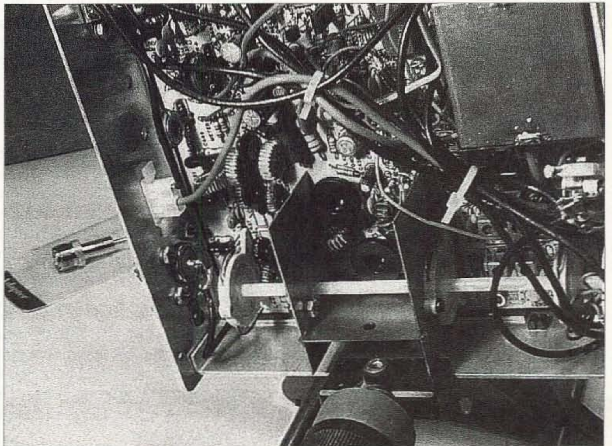
Photo A. The bottom PC board for the HW-9. In the bottom center you'll see the two black heat sinks for the final transistors. On the left of the finals you'll see the two empty slots for the filters. These open locations would be filled with the correct inductors needed.
