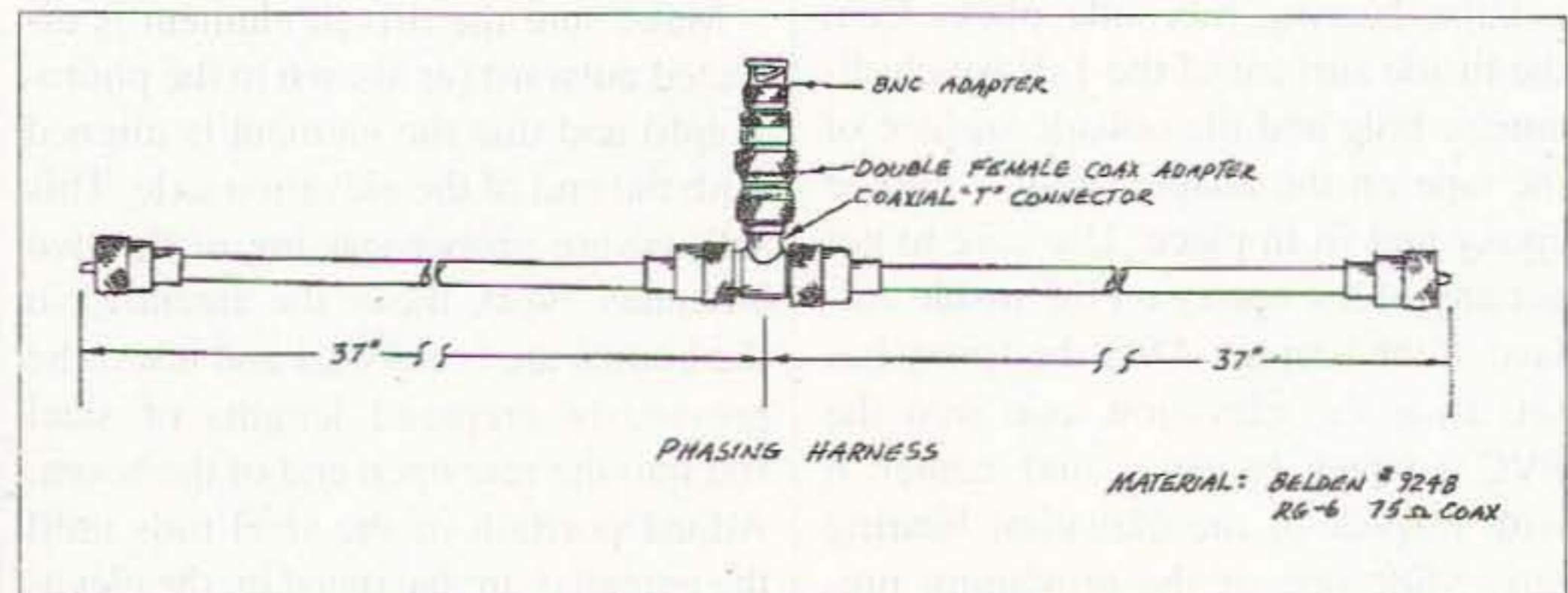
Fig. 5. Phasing harness.
