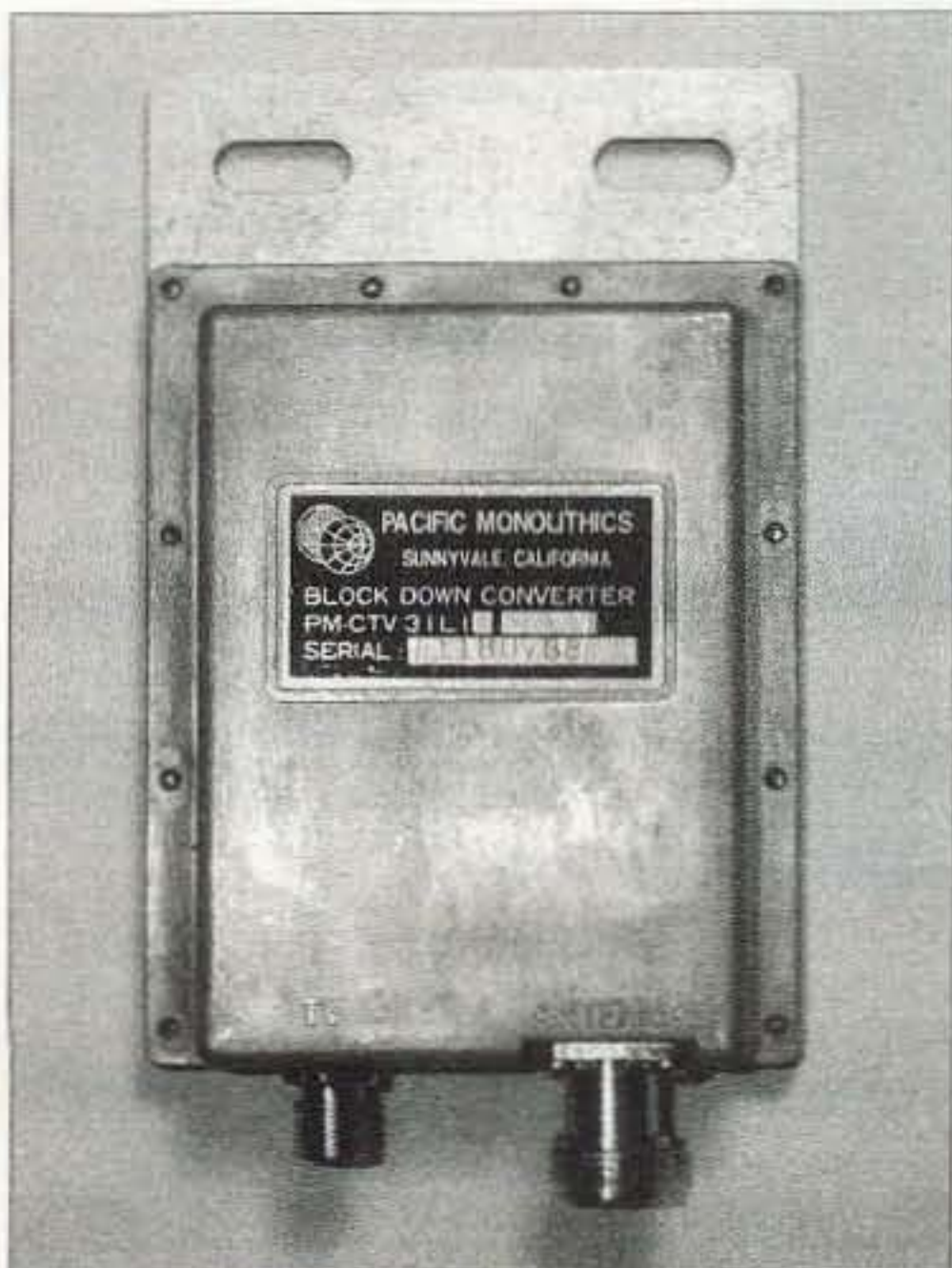
Photo C. Another alternative downconverter, from Pacific Monolithics.
