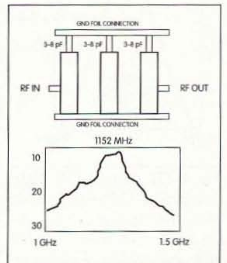
Fig. 3. PC board filter for 1296 MHz constructed from PC board traces and three small-value variable capacitors.
