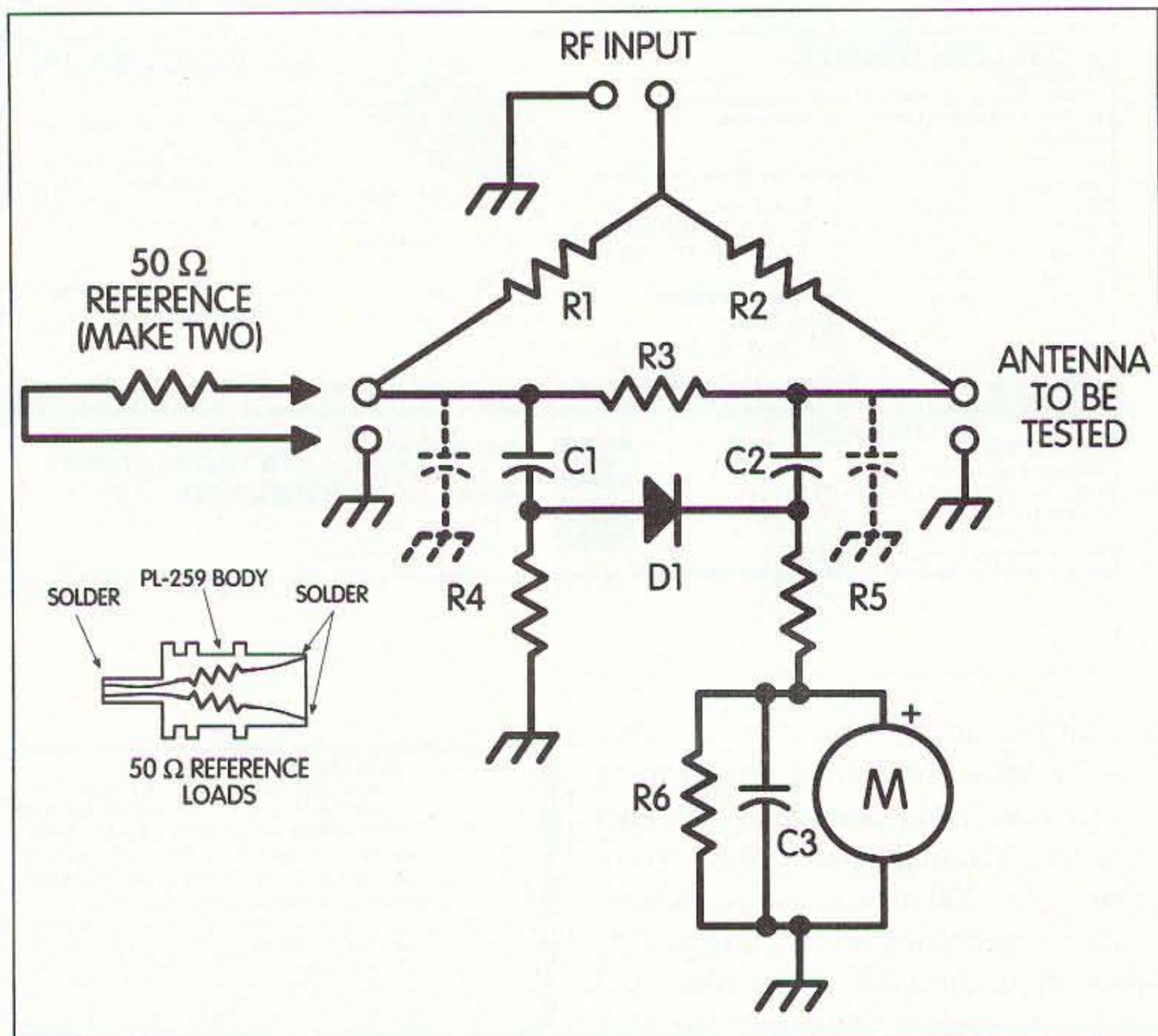
Fig. 3. RF impedance bridge.
