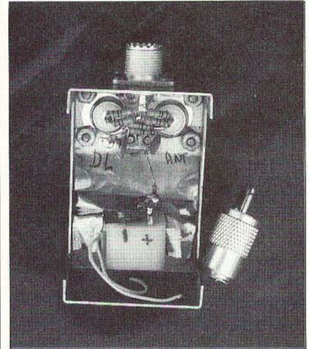
Photo B. Inside view of the RF bridge.
