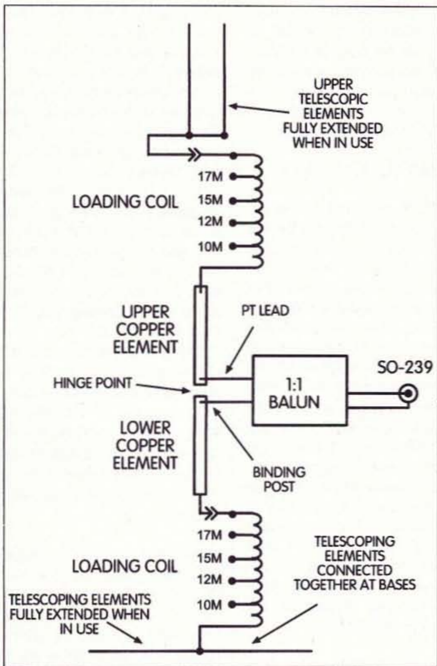
Fig. 3. Complete diagram.
