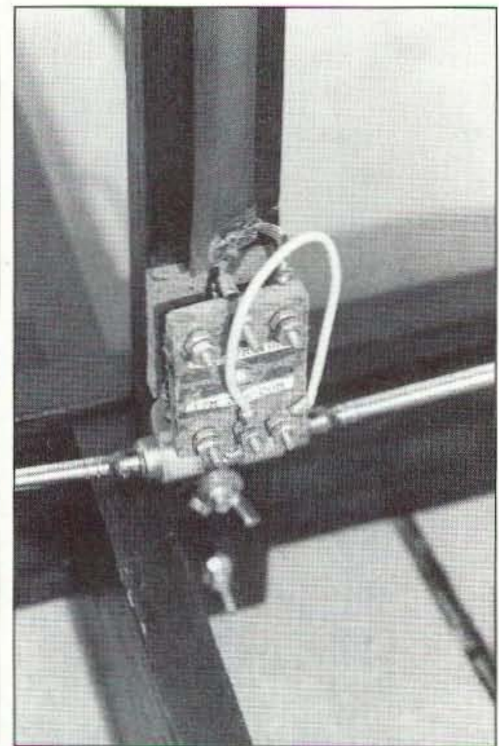
Photo E. Lower loading coil, showing #6-32 hardware with jumper for band changing. Lower elements horizontal when in operation.
