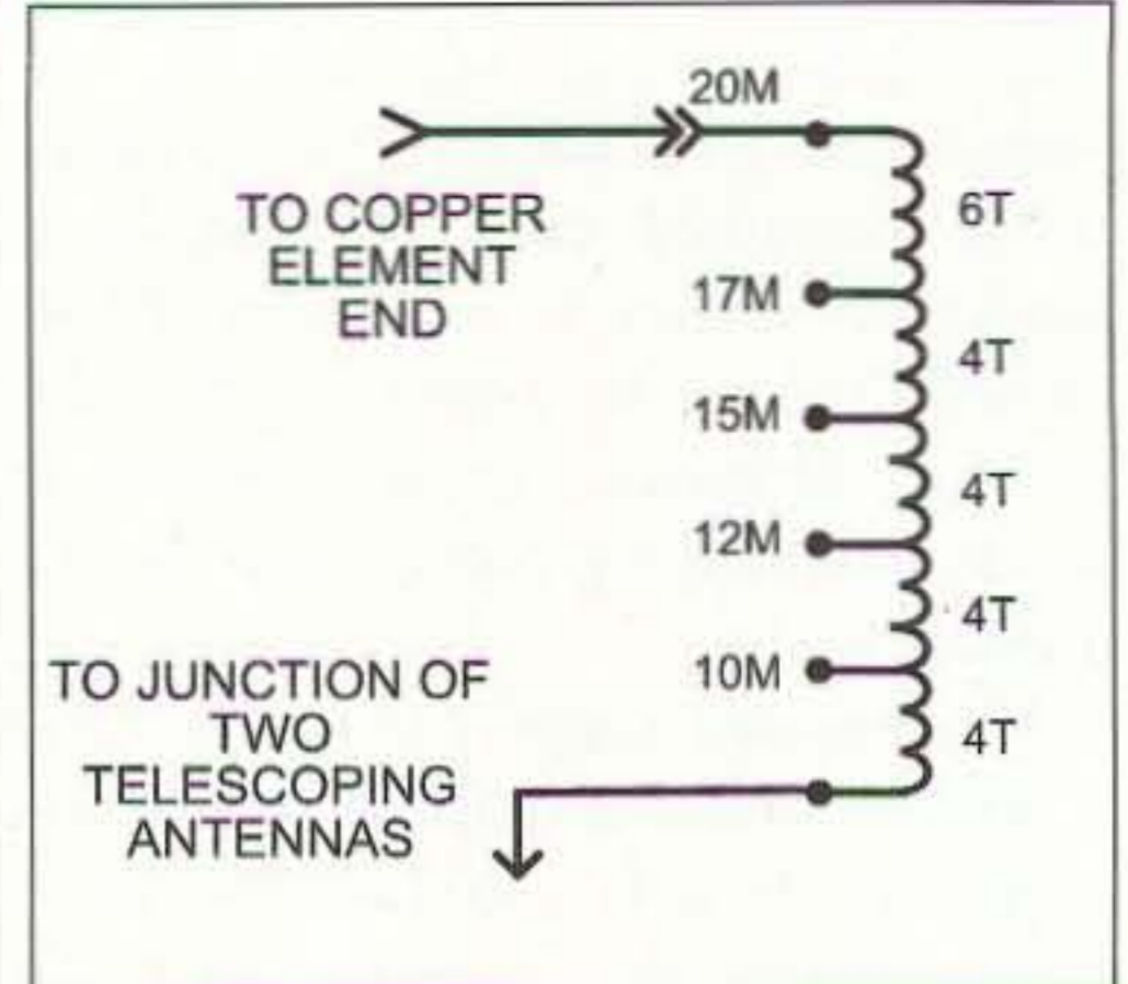
Fig. 2. Loading coils (two required). #18 Formvar wire wound on Amidon powdered iron toroid T-106-6.
