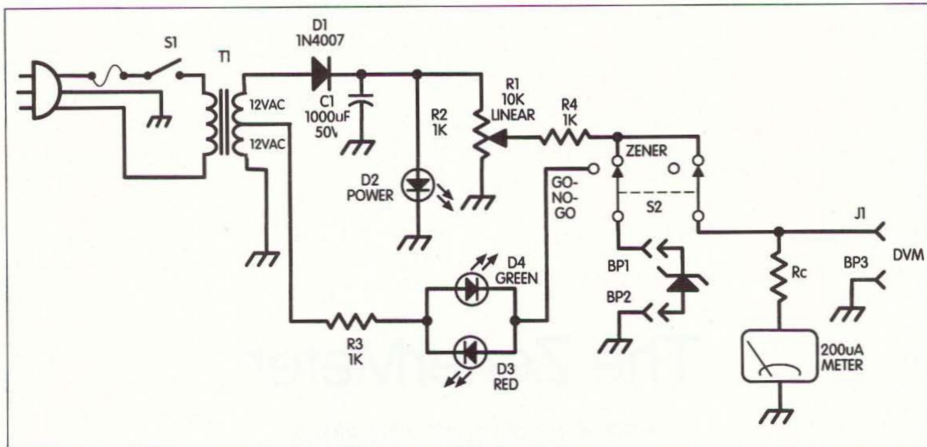
Fig. 1. Schematic.
