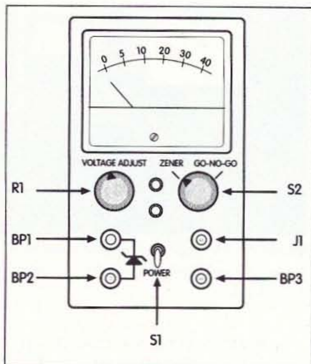
Fig. 2. Front-panel layout.
