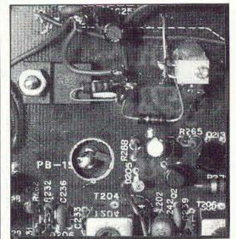
Photo E. The added LM317 IC and potentiometer provide power regulation and control. Below the IC is a hole for access to the SO-239 output connector.
