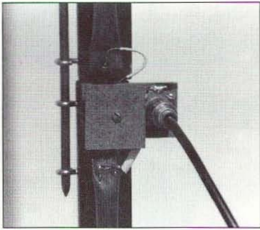
Photo C. Feedpoint in operation.
