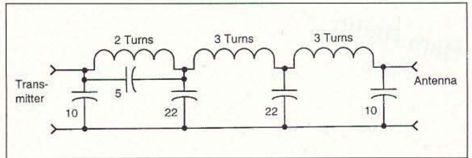
Fig. 1. Schematic of a simple low-pass filter for two meters. Capacitance values are in picofarads.
