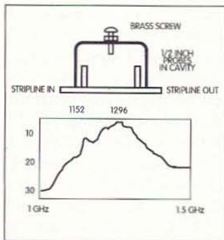
Fig. 1. Copper pipe cap filter for 1296 from standard plumbing fitting. Add a brass screw and two half-inch probes on either side of the center line, tied to PC board stripline traces.
