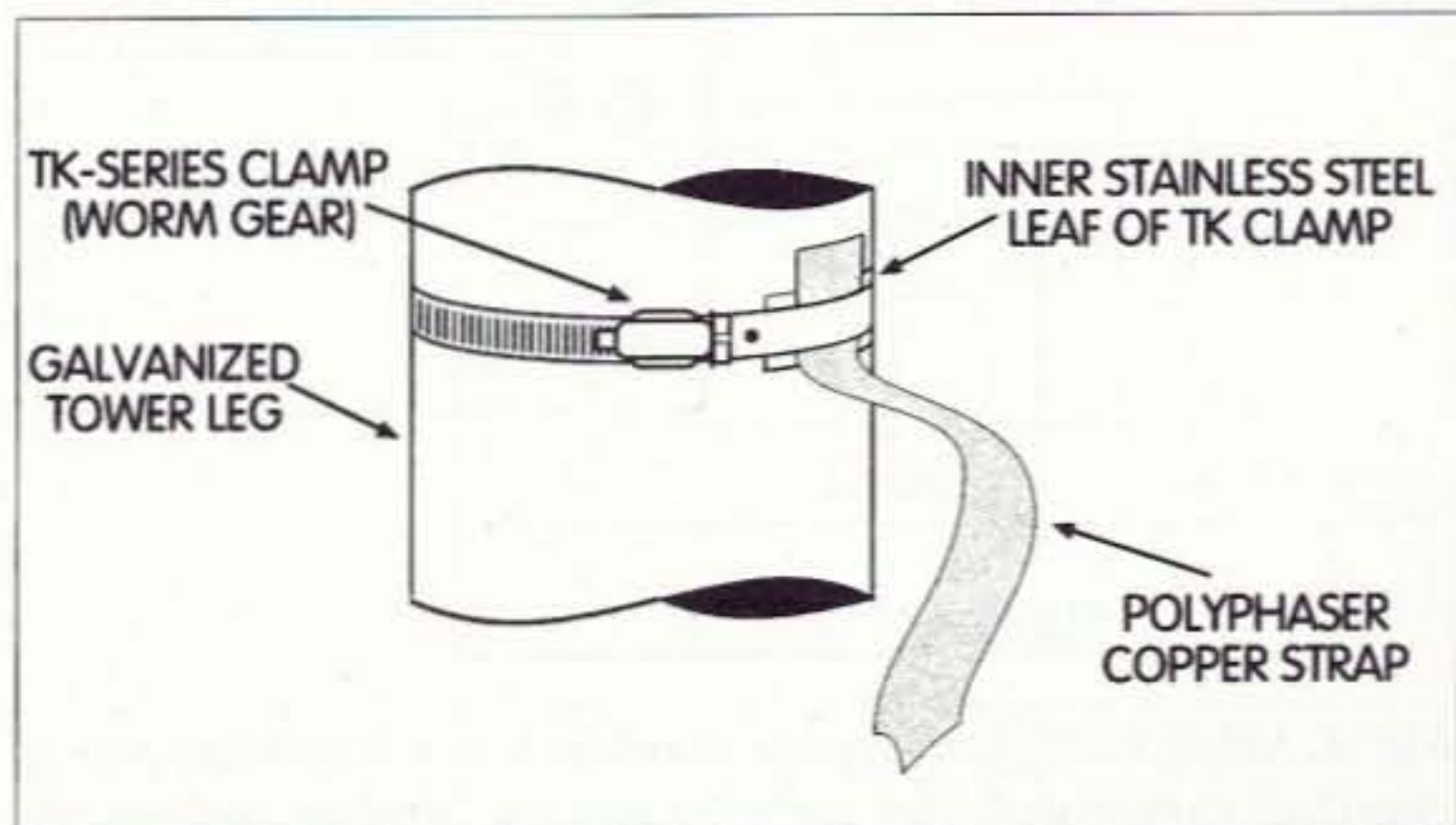
Fig. 2. Closer view of the TK clamp mechanics.
