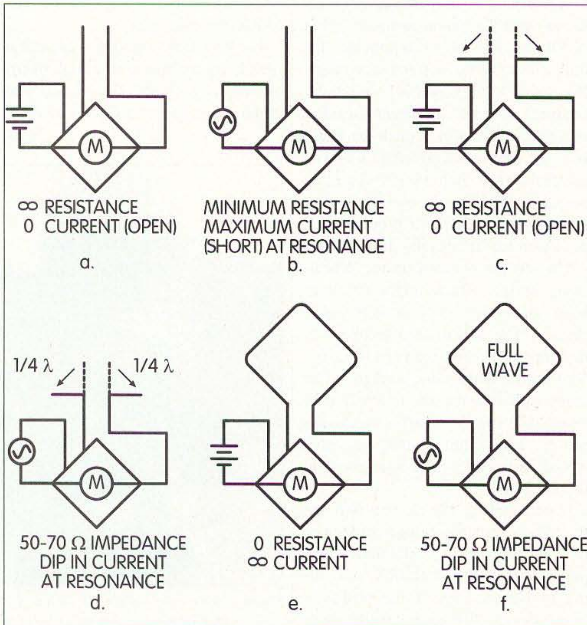
Fig. 2. Simple RF bridge.
