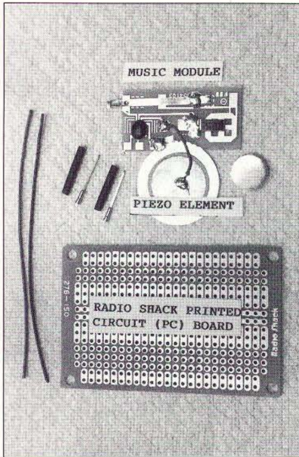
Photo A. Original parts kit.
