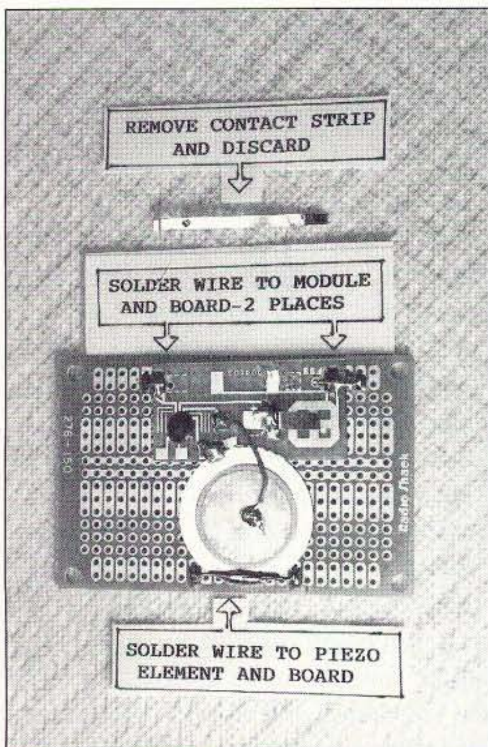
Photo B. Module mounted onto board.
