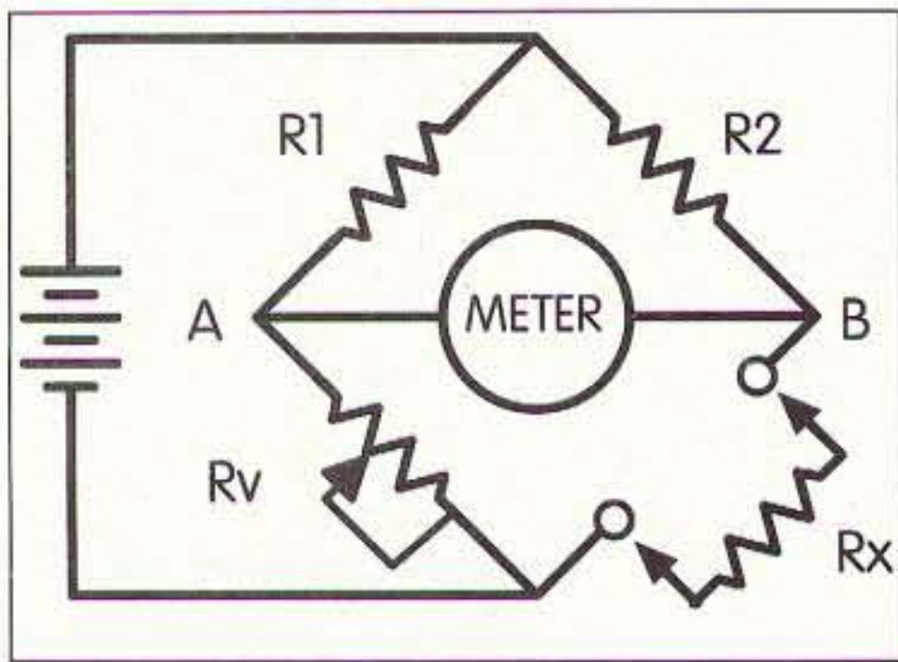
Fig. 1. Basic DC Wheatstone bridge.
