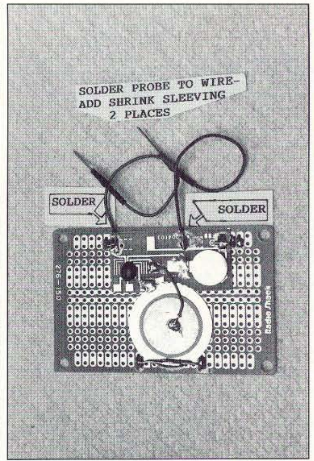
Photo C. Prepare and install test leads.
