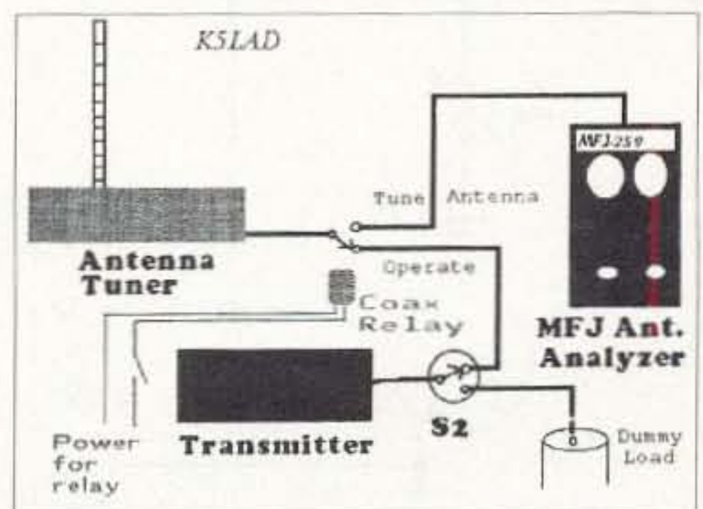
Fig. 1. Note that you can't feed the rig into the analyzer, frying it.
