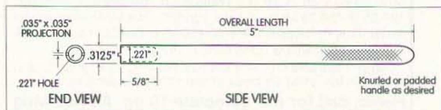
Fig. 1. End and side mechanical views of the Slotted-Nut-Tool© used for 1/8" miniature panel phone jacks. For the 3/32" Slotted-Nut-Tool, the hole (shown as .221") is bored to .144".
