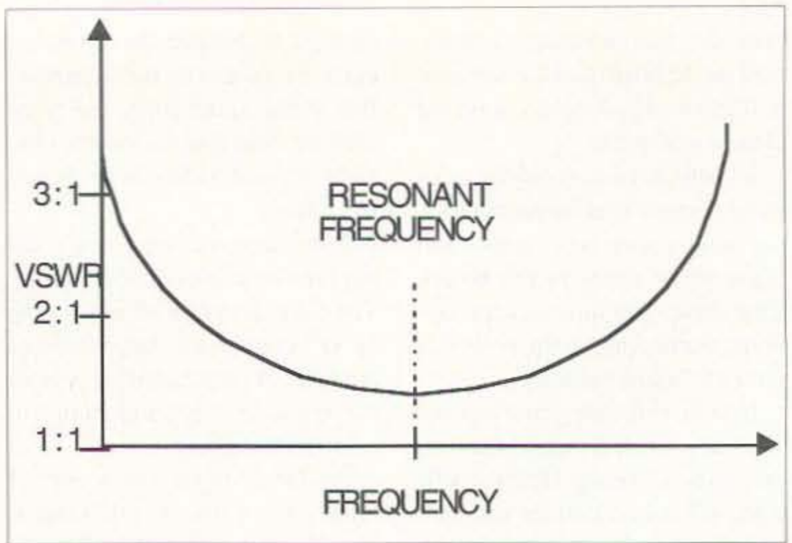
Fig. 1. VSWR vs. frequency curve.
