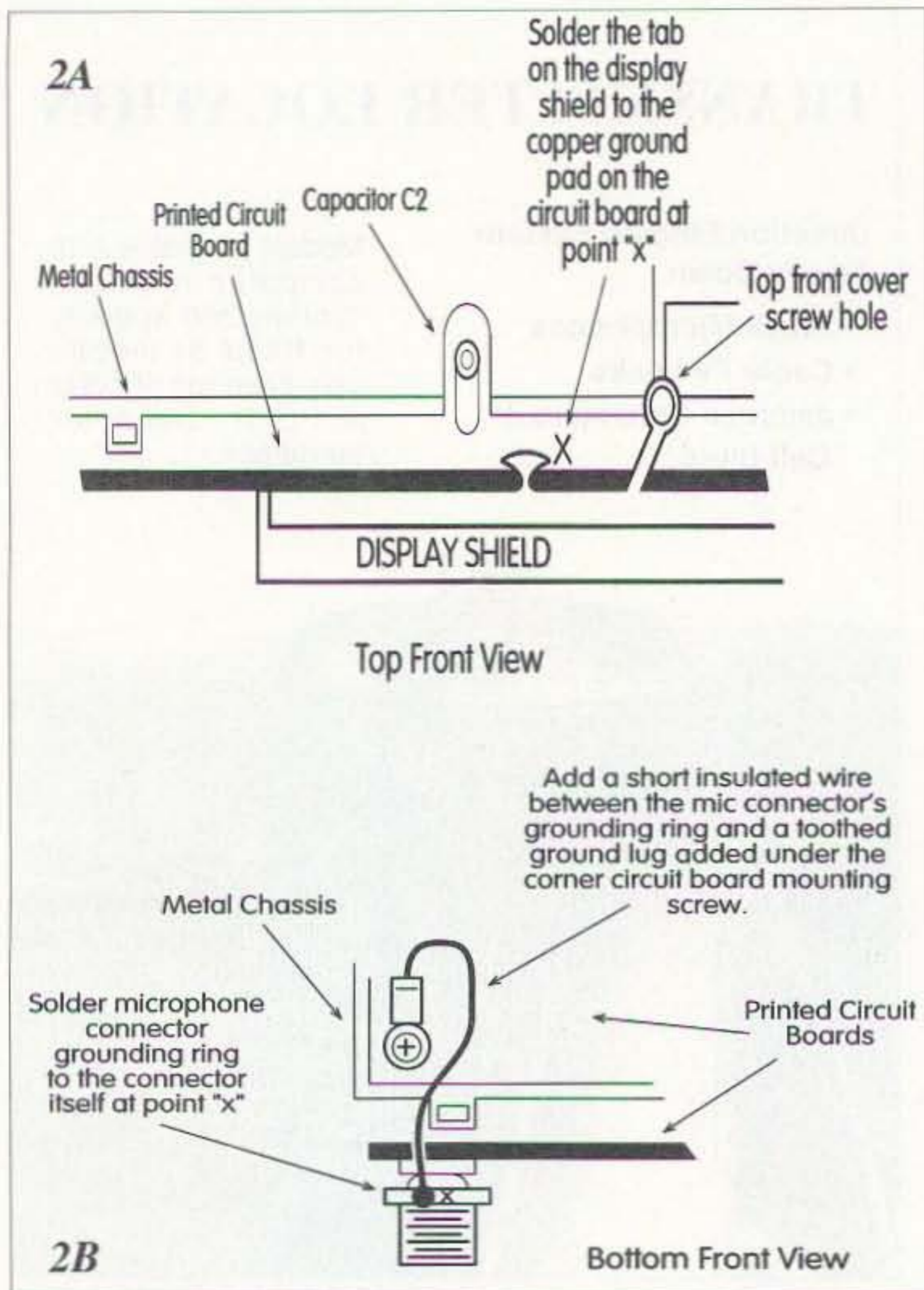
Figs. 2A & 2B. Alinco DR-1200T anti-static modification.
