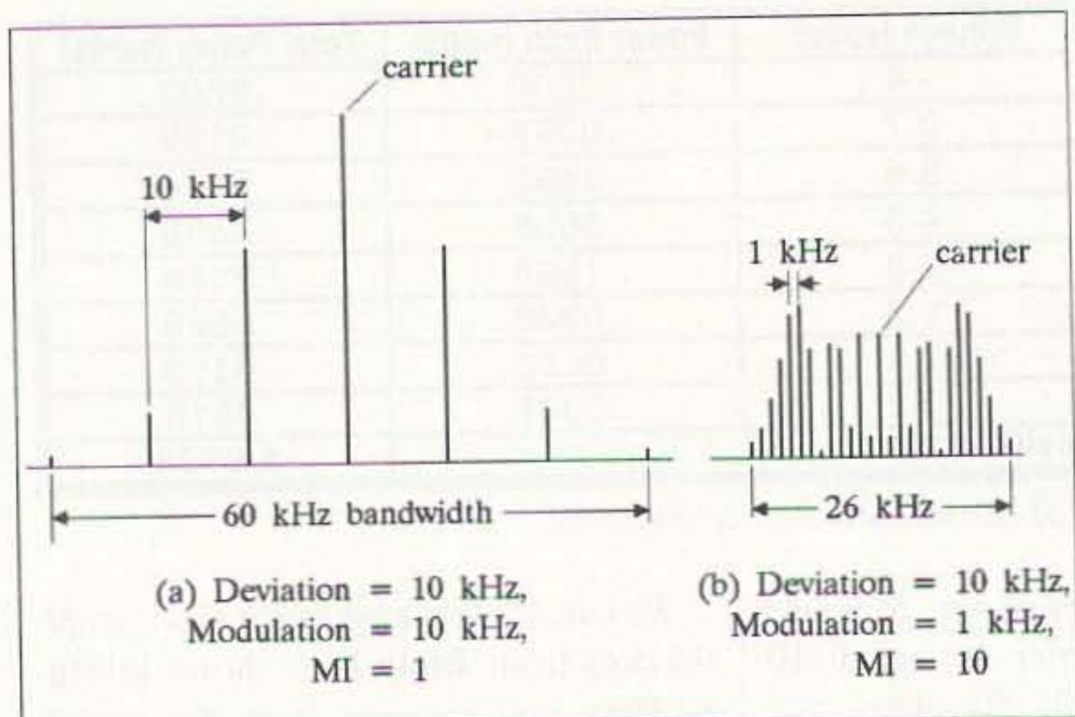
Fig. 2. FM, same deviation, different modulation index.
