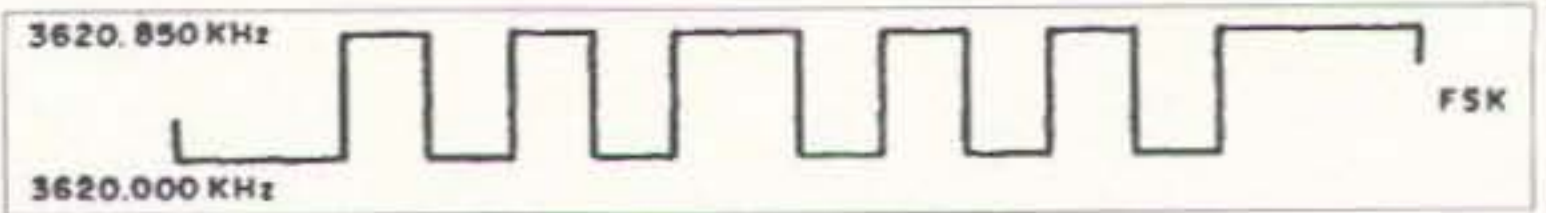
Fig. 2. In FSK, a carrier is shifted in frequency to correspond to MARK and SPACE.
