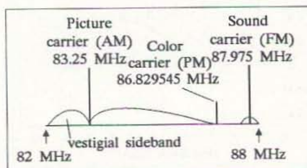
Fig. 3. TV channel 6 spectrum.
