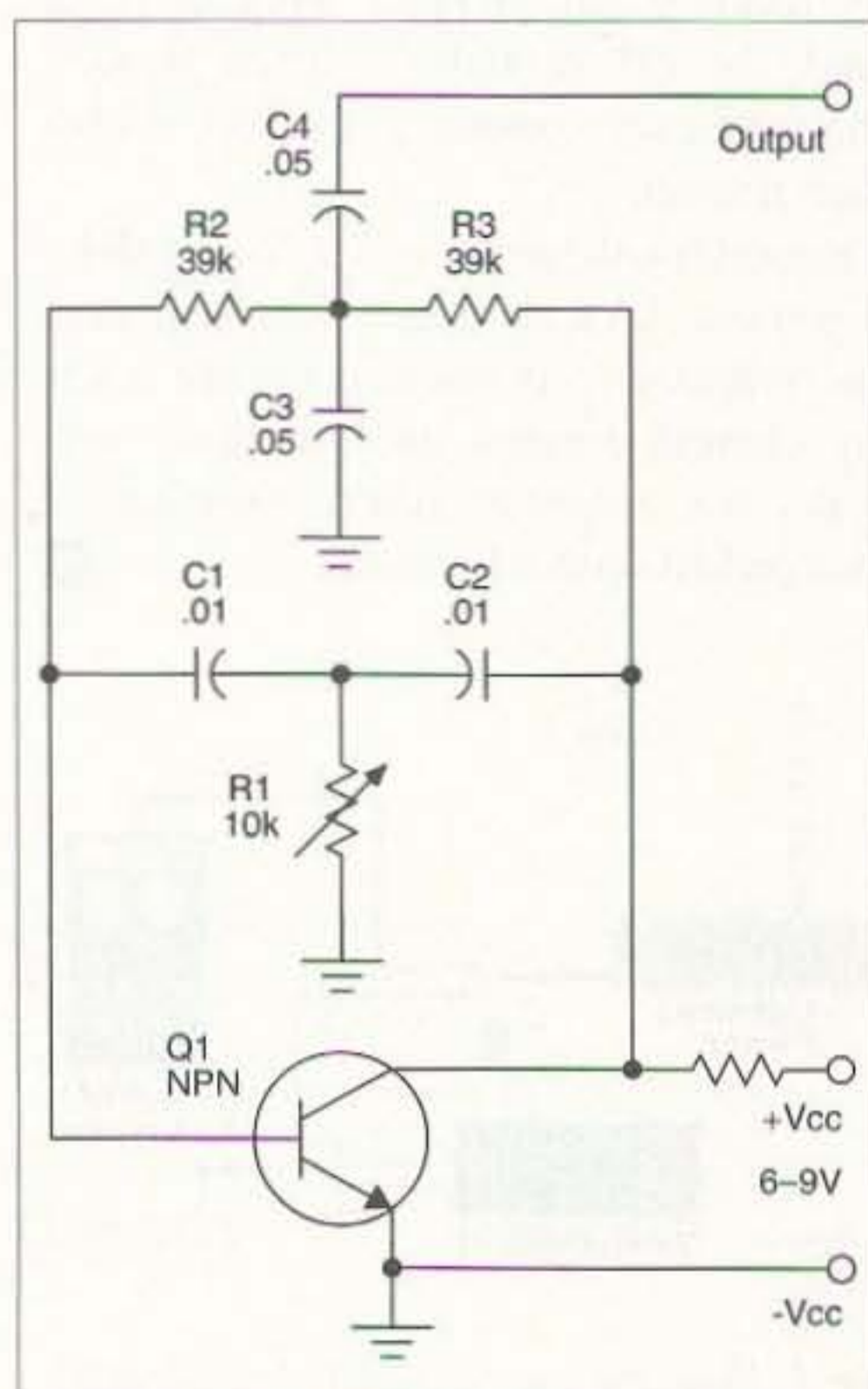
Fig. 1. Basic circuit for the Twin-T.
