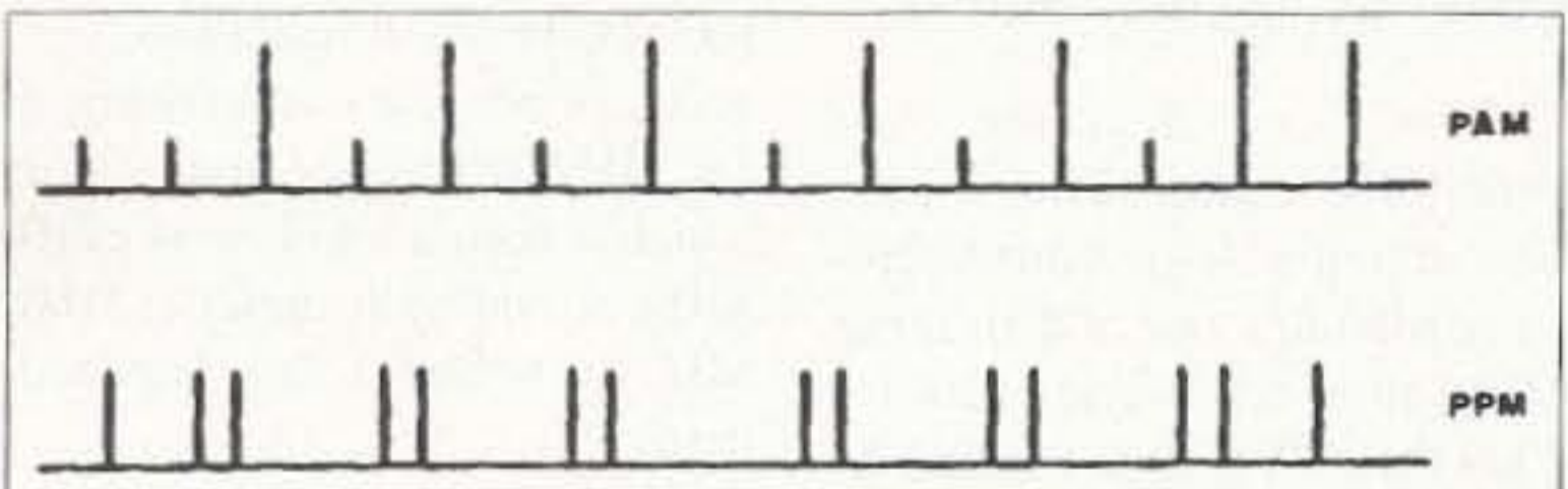
Fig. 4. Pulse Amplitude Modulation (PAM), or Pulse Position Modulation (PPM).
