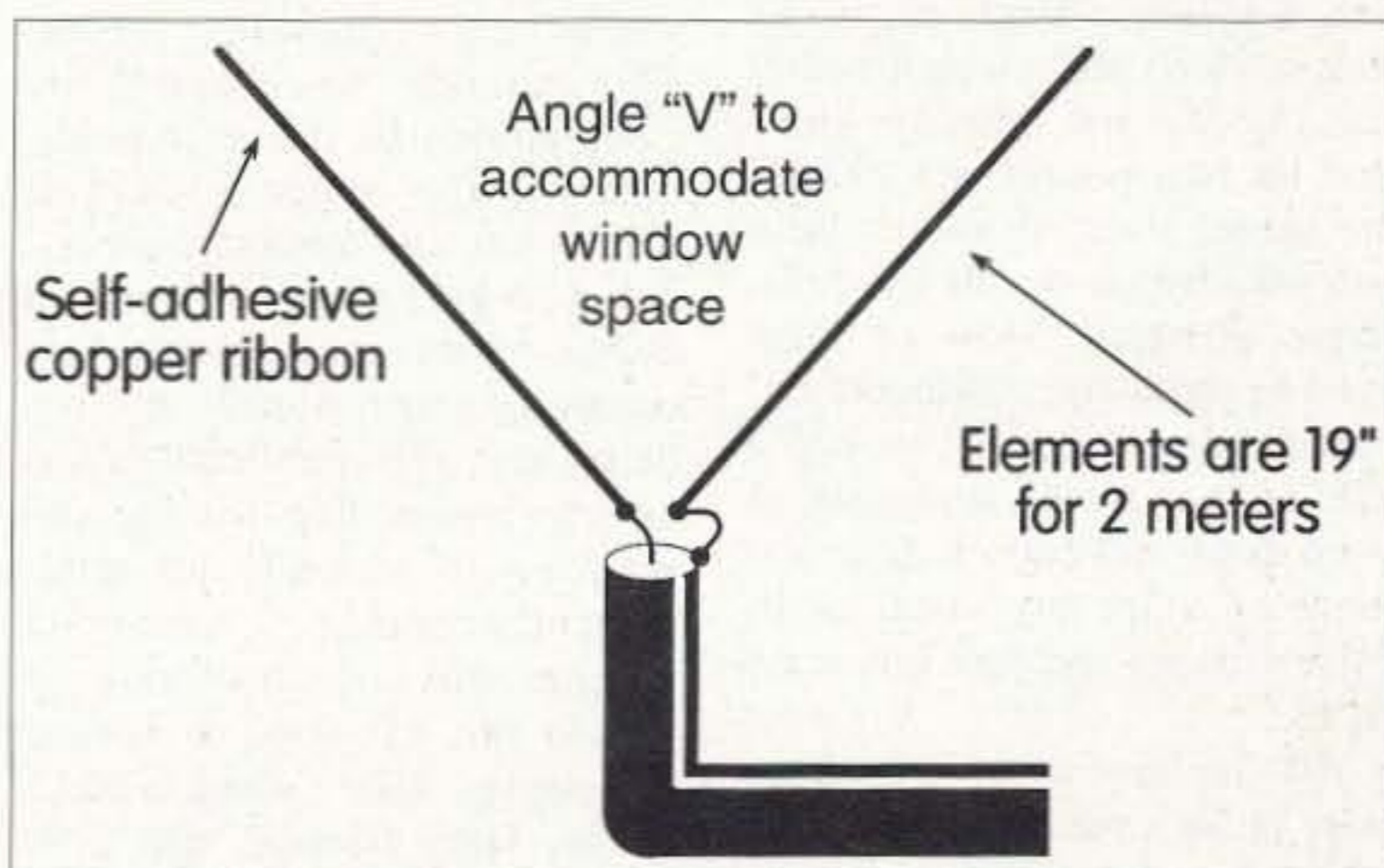
Fig. 3. N6MUJ's "Sticky Antenna."
