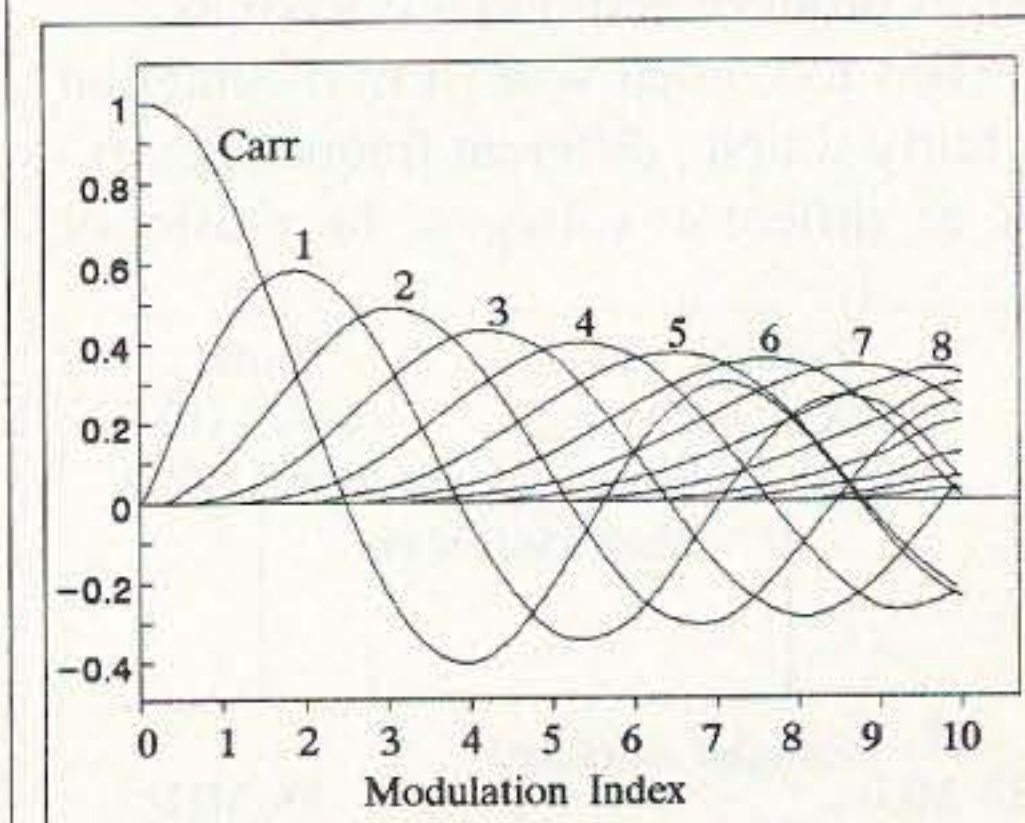
Fig. 1. FM carrier and sideband amplitudes.
