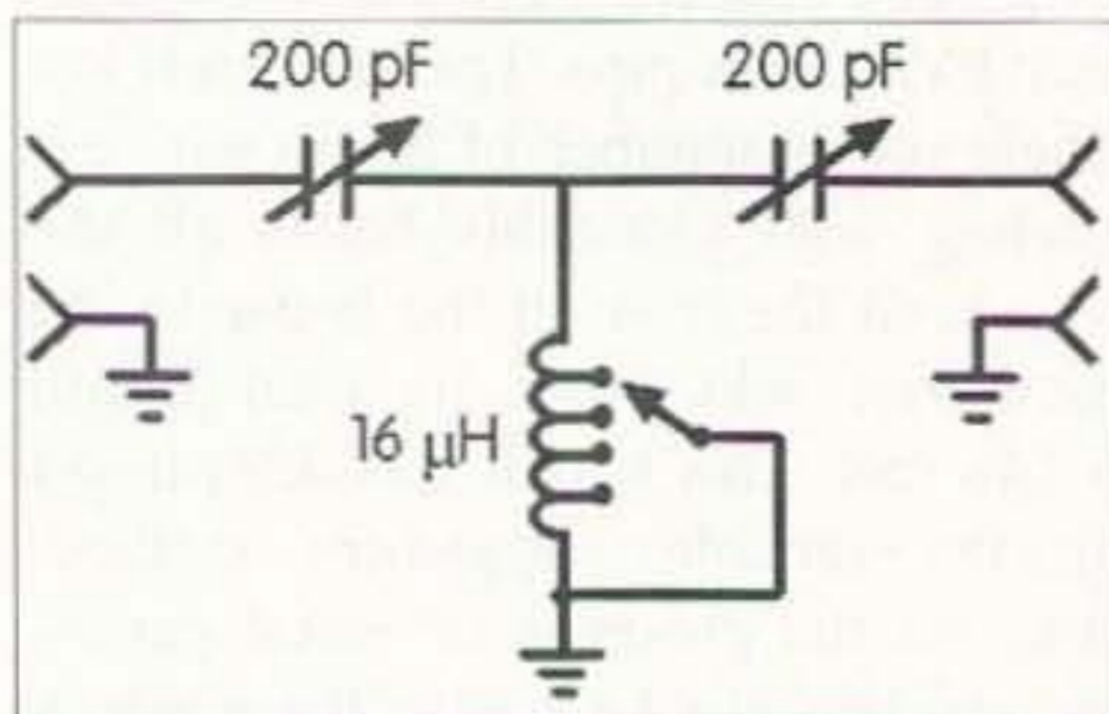
Fig. 1. The T-match.
