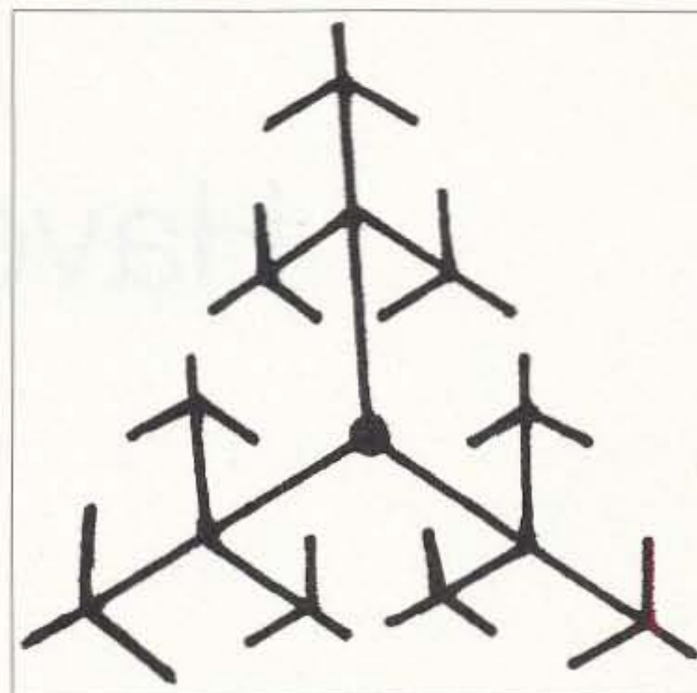
Fig. 1. The fractal pattern of the radial ground counterpoise, called a "third-order ternary dendrite."
