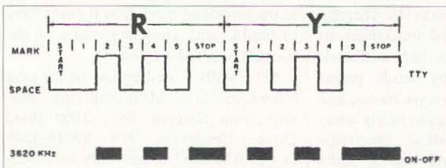
Fig. 1. On-off keying.
