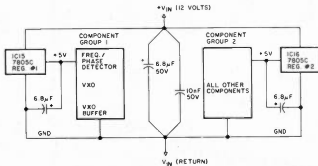
Fig. 5. Power supply.
