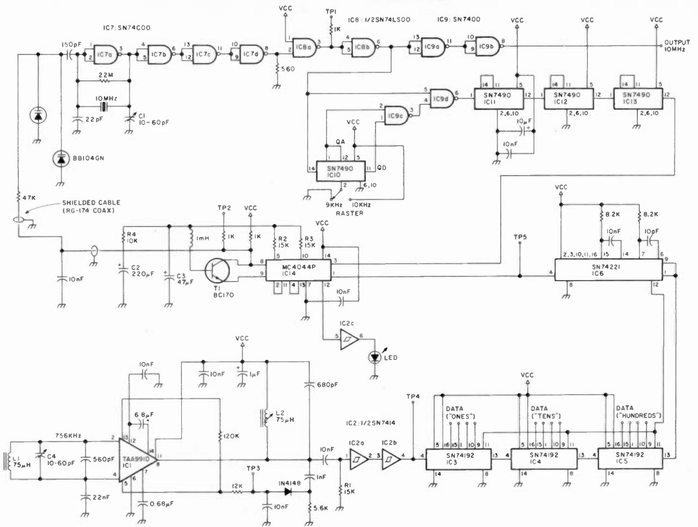
Fig. 2. Schematic diagram.
