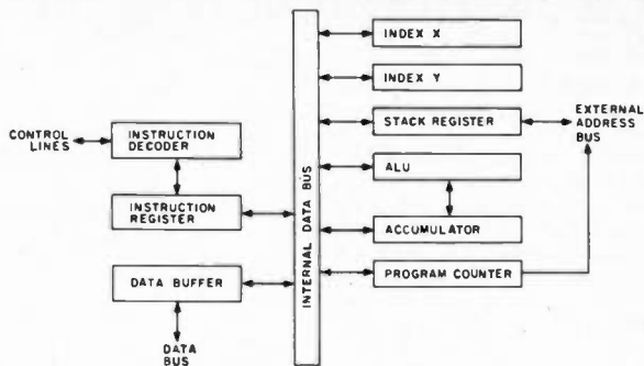
Fig. 3. 6502 block diagram.
