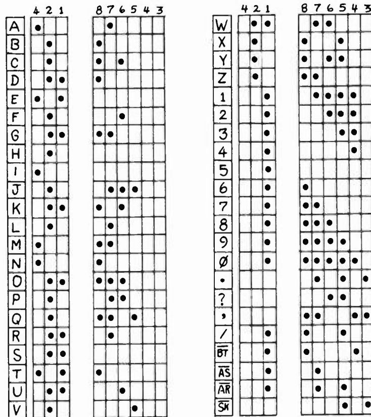
Fig. 2. Placement guide for diodes in the diode matrix. The first column refers to the CD5422 down-counter. The second column is for the CD4021 shift register. A dot indicates that a diode is to be placed in the appropriate line. All diodes are silicon switching types such as 1N914s or 1N4148s. The use of germanium diodes such as 1N34s is not recommended.
