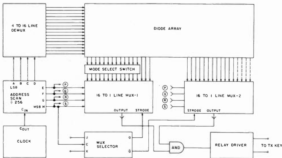
Fig. 4. Block diagram of the "improved" CQ Sender with different modes.
