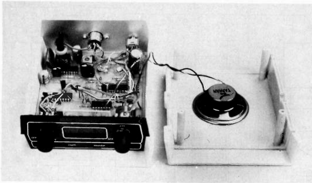
Photo B. Virtually all the circuitry is accommodated on two PC boards.
