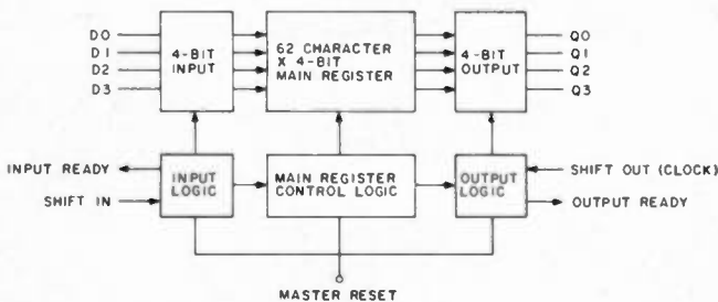
Fig. 1. The Fairchild 3341 MOS FIFO buffer block diagram.
