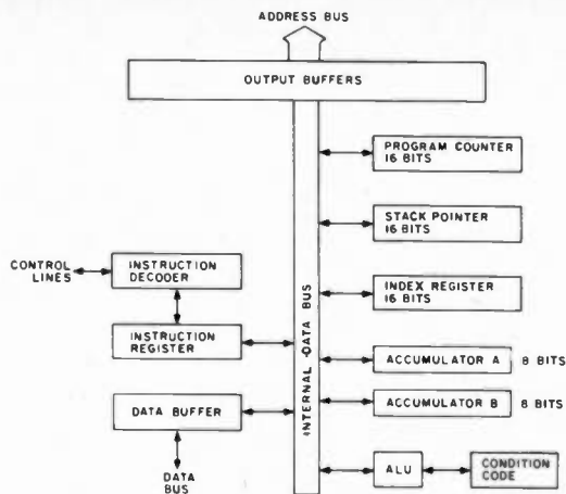
Fig. 2. 6800 block diagram.
