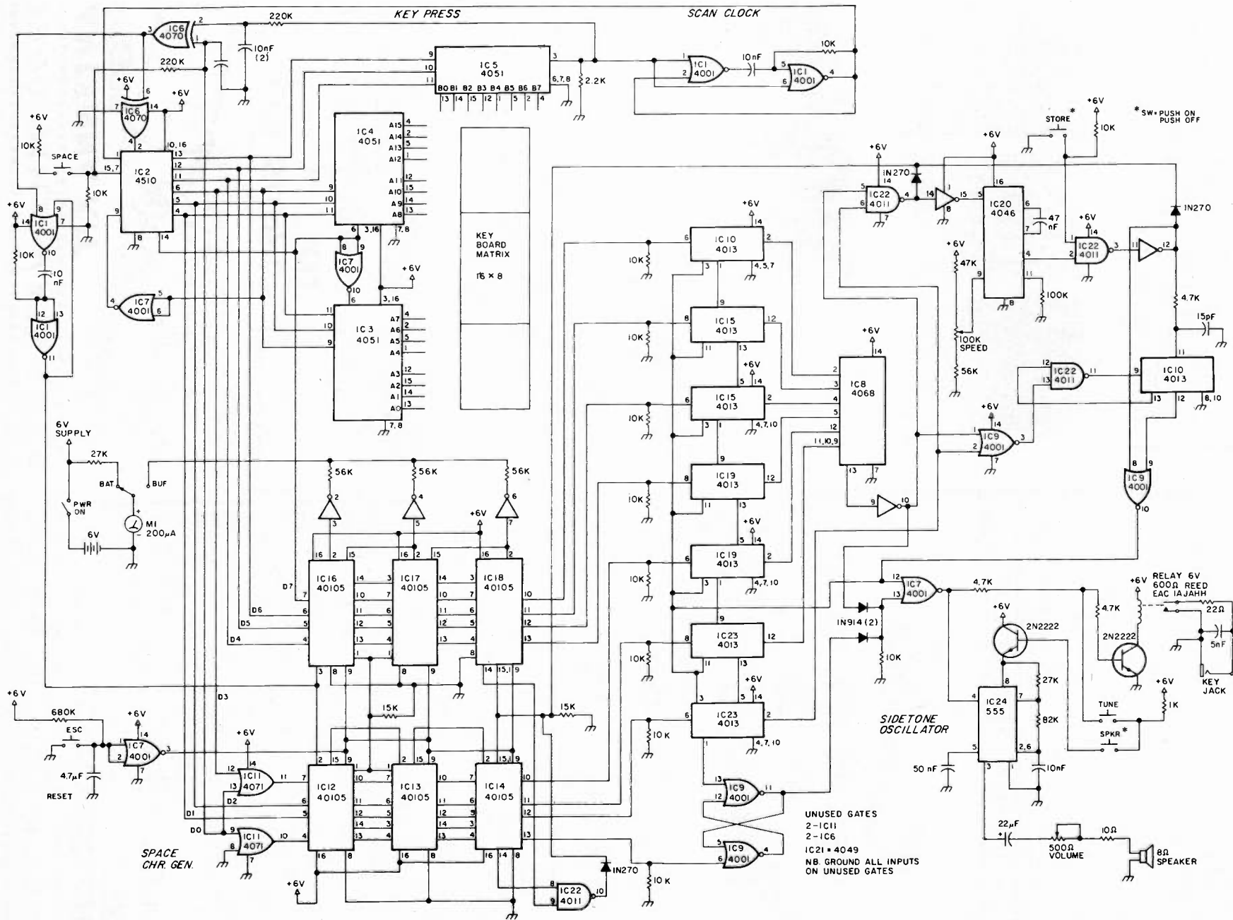
Fig. 1. QRP schematic.
