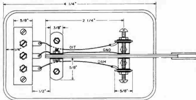
Fig. 4. Top view of the completed key. The dimensions were measured on one of the models, but need not be exact.
