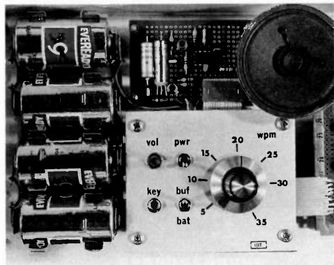
Photo C. Control panel, speaker, batteries, and sidetone/relay board.
