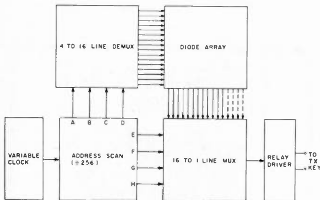
Fig. 1. Block diagram of CQ Sender.
