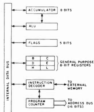
Fig. 1. 6800 block diagram.
