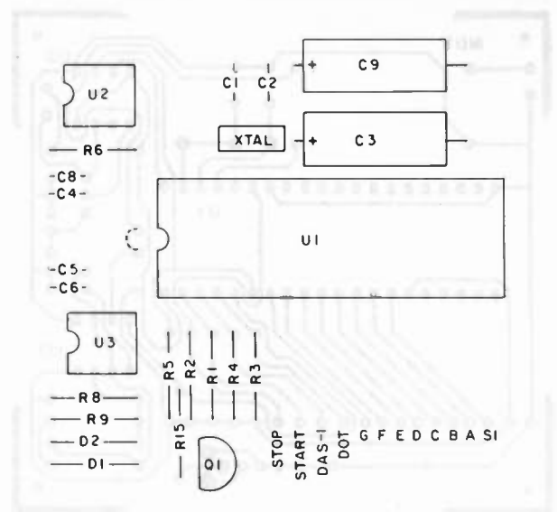
Fig. 4. Circuit board showing parts placement.
