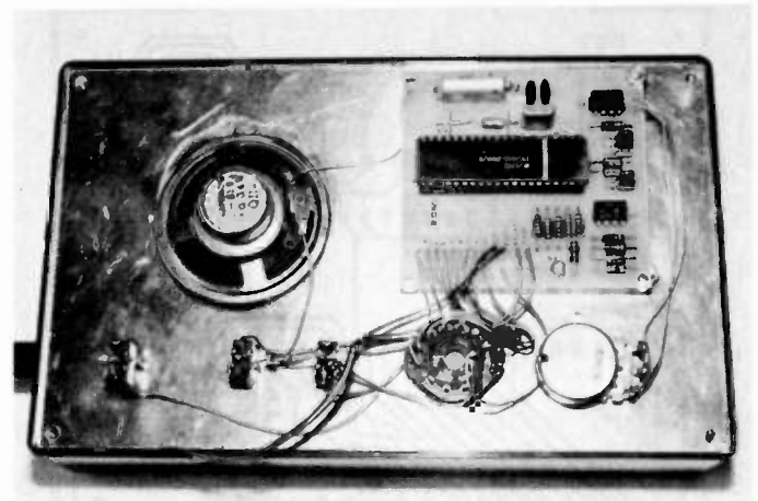
Photo B. The inside top panel of the CPP1.
