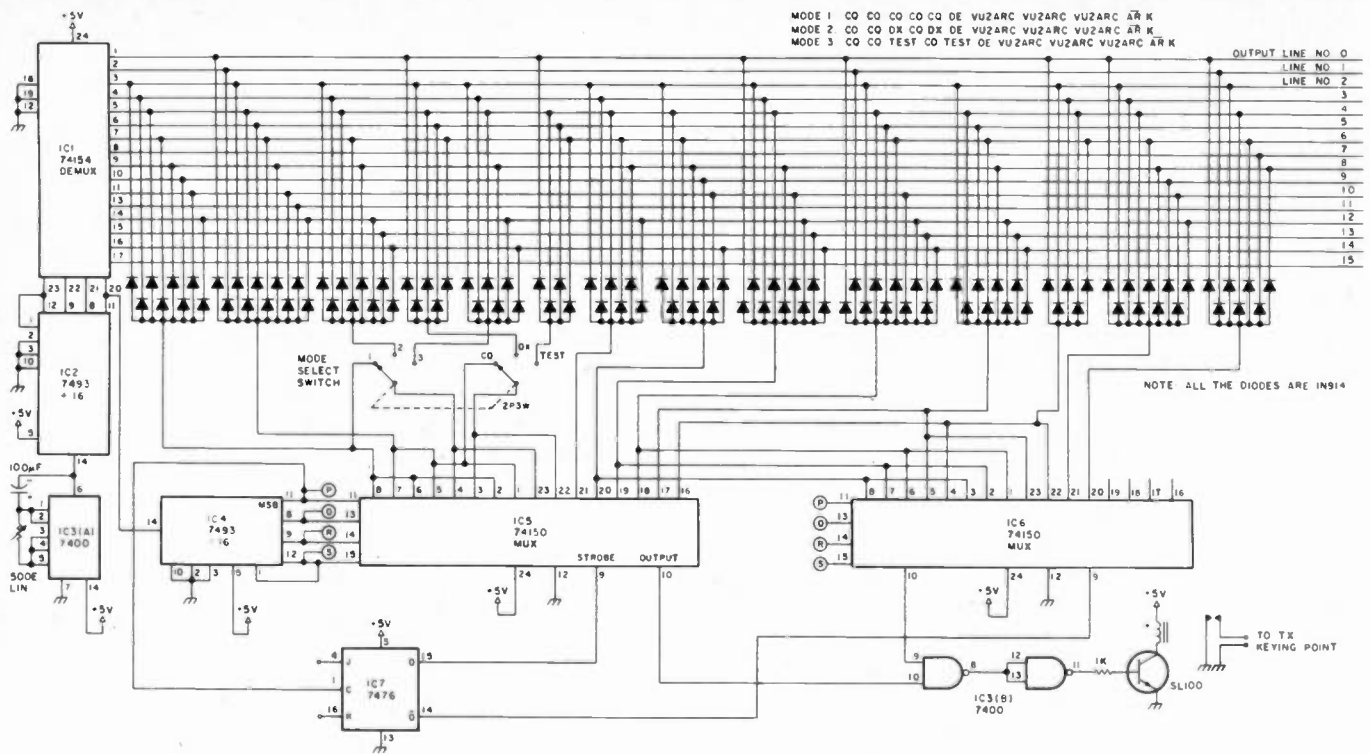
Fig. 3. Improved CQ Sender with different modes.
