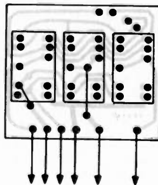
Fig. 7. Parts placement for the display PCB.
