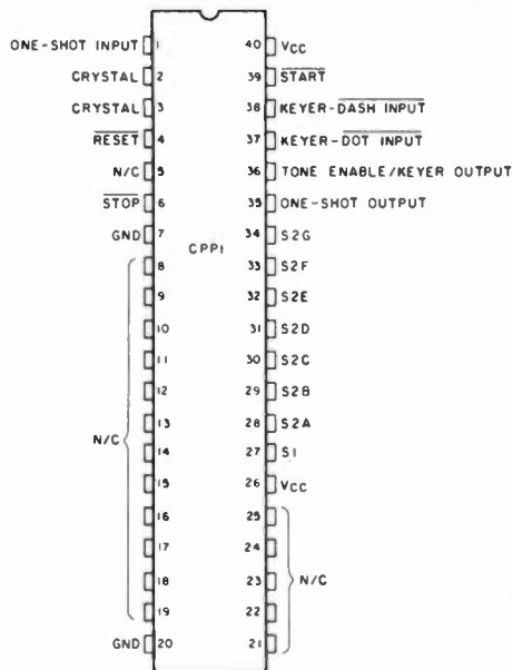
Fig. 2. Pin description.
