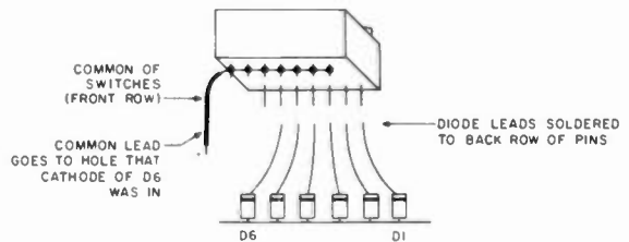
Fig. 2. End view (parts omitted for clarity).
