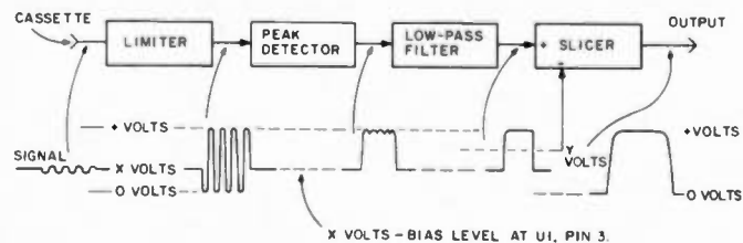
Fig. 1. Cassette memory keyer block diagram.
