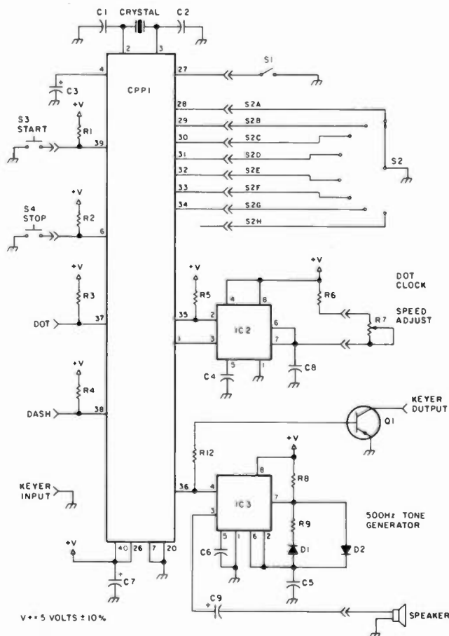
Fig. 1. Schematic.
