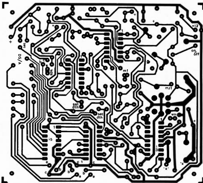
Fig. 3. PC board for the depth sounder.
