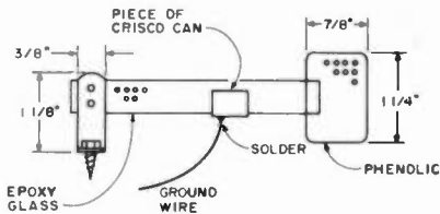
Fig. 3. Details of paddle-arm assembly.
