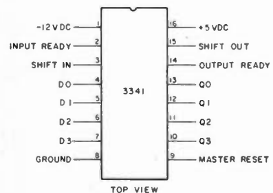
Fig. 3. 3341 connection diagram.
