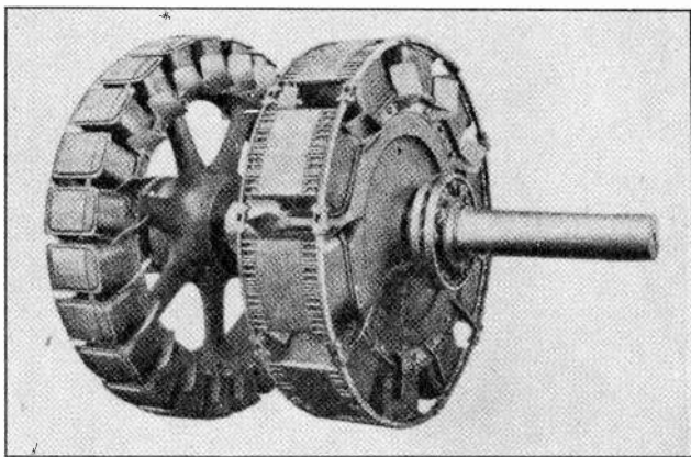
Fig. 11. Double rotor of a frequency changer motor-generator set. The ten-pole rotor operates on 25 cycles and the 24-pole rotor produces 60-cycle energy. Courtesy of Allis-Chalmers Mfg. Co.
