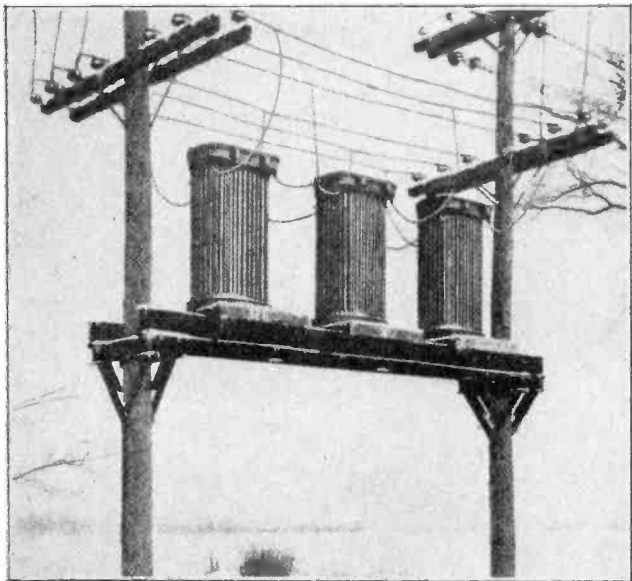
Fig. 6. Bank of three power transformers mounted on a neat platform between two strong poles.
