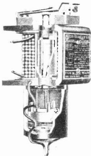
Fig. 17. Sectional view of a magnetic overload-relay and dash pot. When the core is lifted the rod above it forces open the spring contacts which break the circuit to the holding magnet. (Courtesy Allen Bradley Co.)
