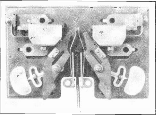
Fig. 7. Excellent view of thermal overload-relay such as used on automatic controllers manufactured by the General Electric Co. Note the current setting pointers and also the resetting cord on this device. (Courtesy General Electric Co.)
