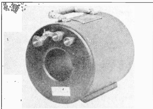
Fig. 4. Portable current transformers of this type are very convenient when making tests on lines or electric machines with portable ammeters and wattmeters. (Photo Courtesy General Electric Co.)
