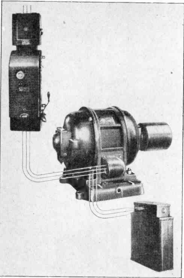
Fig. 7. Static condensers can be connected direct to the terminals of individual induction motors as illustrated in the above view. The condenser then supplies the magnetizing current to the motor and corrects the lagging power factor at its source. (Courtesy G. E. Company.)
