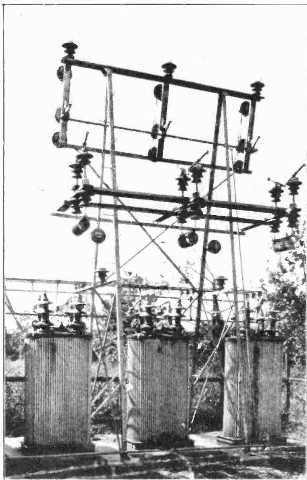
Fig. 2. Small outdoor transformer substation with transformers located on a base on the ground, and choke coils, fuses, and disconnect switches on the steel tower above them.
