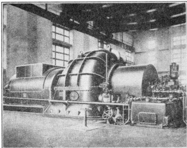
Fig. 6. Large steam-turbine-driven alternator. The turbine with its control mechanism is on the right. This alternator is enclosed in the air-tight casing at the left. This unit is typical of hundreds of great steam-driven generators in use in modern power plants throughout this country. (Photo Courtesy General Electric Co.)
