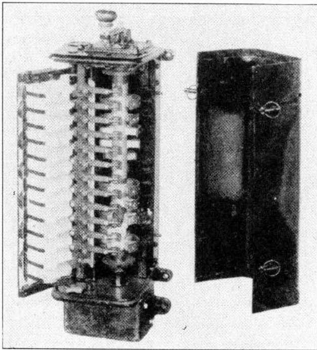
Fig. 13. This view shows an A. C. drum controller with the cover removed. Note the rotating segments, stationary contact fingers, arc barriers, and blow-out coils. (Courtesy General Electric Co.)
