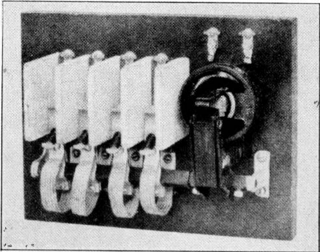
Fig. 7. Photo of contactor panel of an A. C. motor controller. These contacts and their connections require frequent attention by the maintenance electrician.
