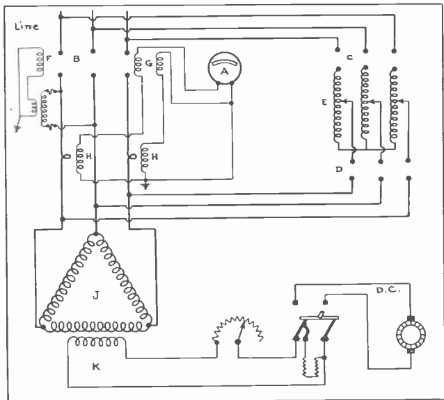
Fig. 7. Diagram of connections for a large synchronous motor with a compensator for starting at reduced voltage. Also note the protective device connected with a circuit-breaker in the line leads.
