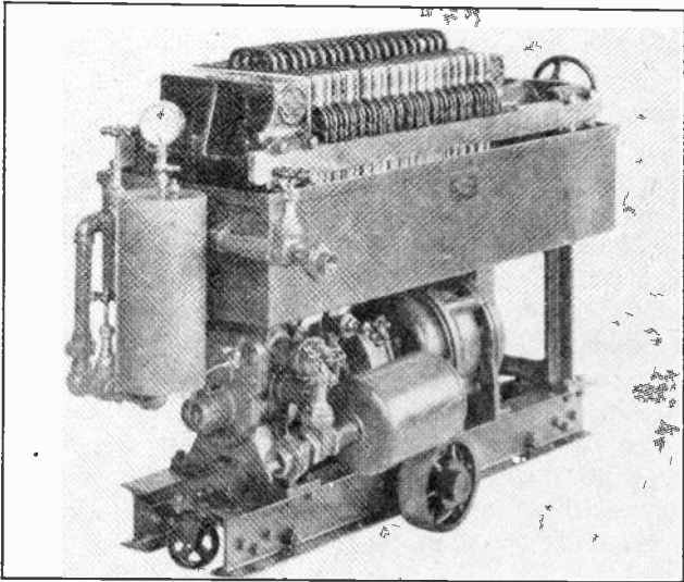
Fig. 10. This photo shows a filter press for cleaning and removing the moisture from insulating oil. Note the motor-driven pump mounted underneath the filter press. (Photo Courtesy General Electric Co.)
