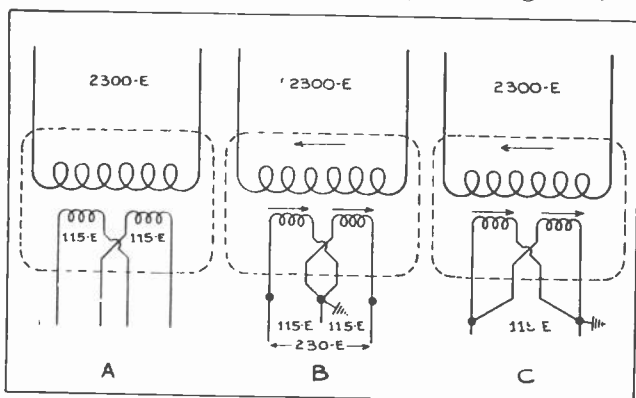
Fig. 2. A shows a single-phase transformer with the secondary winding in two sections. Note the manner in which the leads are crossed inside of the tank. B secondary windings connected for 115 and 230-volt service. C secondary windings connected in parallel for 115-volt service.
