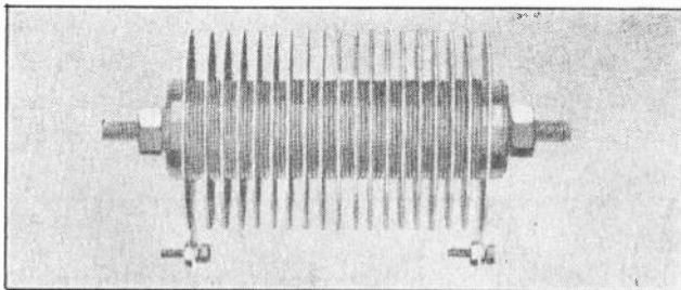
Fig. 10. Single unit of a copper oxide rectifier, consisting of a number of copper disks coated with copper oxide and clamped into one series group. Current can only pass through these devices in one direction. (Courtesy of Westinghouse Elec. & Mfg. Co.)
