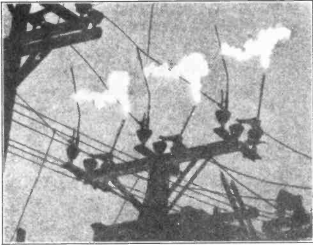
Fig. 13. This night photo of an air break switch opening under load shows the arcs which are drawn from the arcing horns just as the switch opens. Courtesy of Hi-Voltage Equipment Company.
