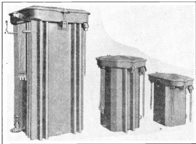
Fig. 8. This view shows three different sizes of common power transformers. Note the cooling flanges or ribs in the tanks of the two larger ones. (Photo courtesy General Electric Co.)
