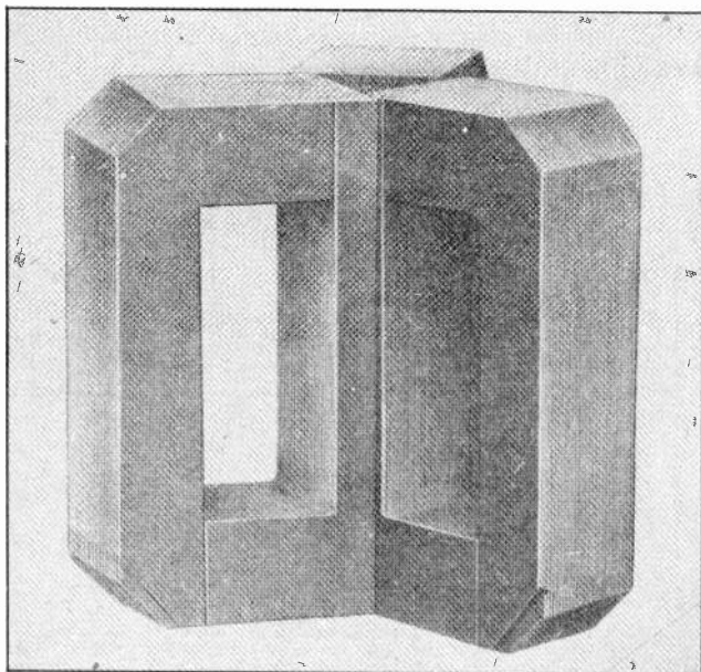
Fig. 3. The above photo shows a complete core of the three-sided type for a distributed core transformer. (Photo courtesy General Electric Co.)
