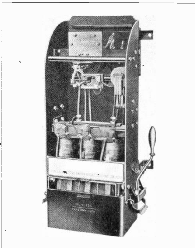
Fig. 1. This photo shows a front view of a three-phase, auto transformer starter or compensator used for starting squirrel-cage motors at reduced stator voltage. (Photo courtesy General Electric Co.)
