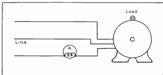
Fig. 3. Ammeter connected to measure the current in one phase of a three-phase motor.
