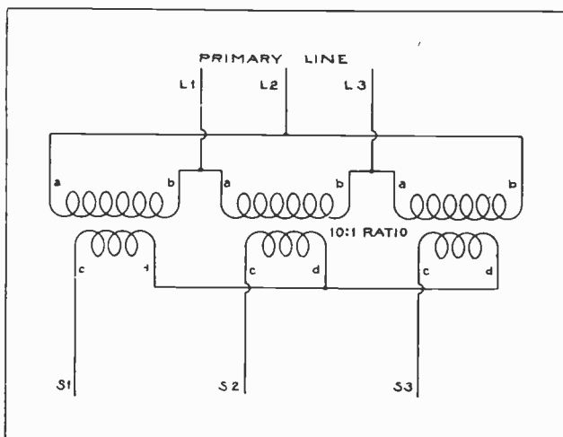
Fig. 11. Three-phase transformer bank connected delta-star. Observe carefully the methods of making the connections shown in each of the diagrams in this section.
