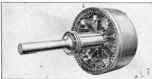
Fig. 11. Phase wound rotor of a large slip-ring induction motor. This rotor has heavy bar windings which are not shorted together like those of a squirrel-cage rotor, but instead have connections brought out from each phase to the slip rings.
