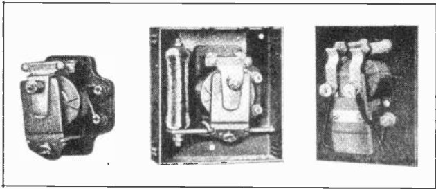
Fig. 18. Three different types of A. C. relays used with motor controllers. (Courtesy Cutler Hammer Mfg. Co.)
