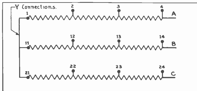
Fig. 16. The above sketch shows a common method of marking resistance units for use with drum controllers.
