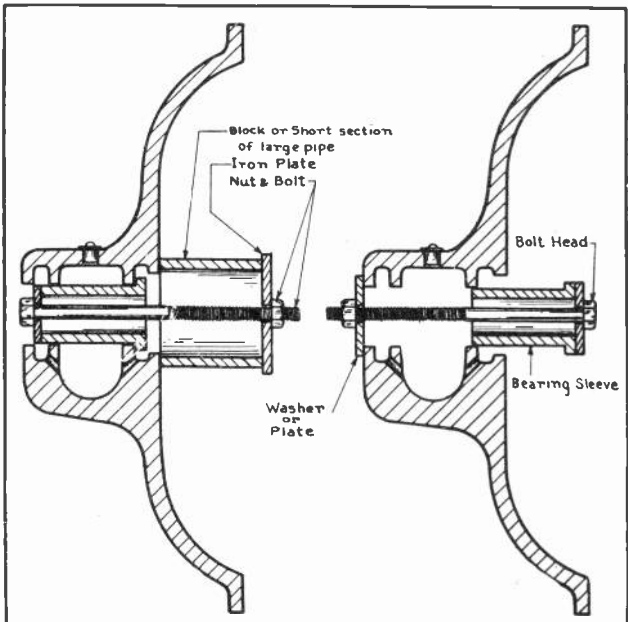
Fig. 3. The sketch on the left illustrates a convenient method of removing a sleeve bearing; and on the right is shown the method of replacing the bearing.
