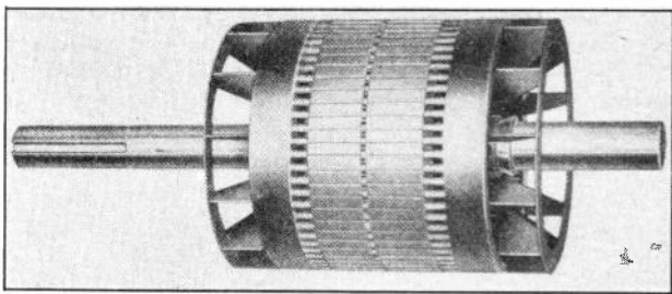
Fig. 7. Squirrel-cage rotor from an A. C. induction motor. Note the manner in which the bars are imbedded in the core slots and also note the ventilating fans at the ends of the rotor.
