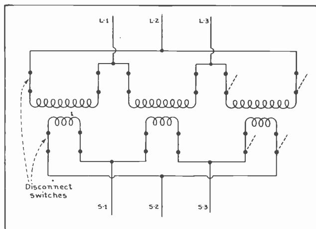
Fig. 14. This diagram shows a convenient method of arranging a bank of transformers with disconnect switches to quickly change over to open-delta operation in case of trouble on one transformer.
