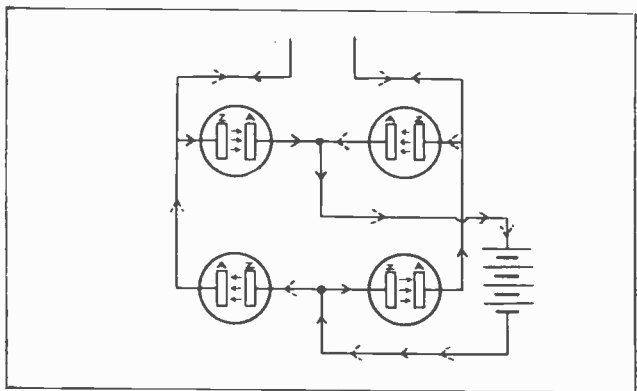
Fig. 3. Full-wave, electrolytic rectifier using four cells connected in a "bridge" circuit.
