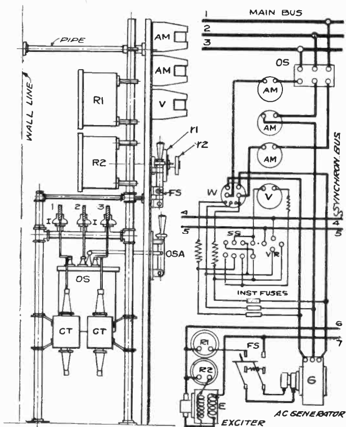
Fig. 2B. Side view and wiring diagram of the panel shown in Fig. 2A.
