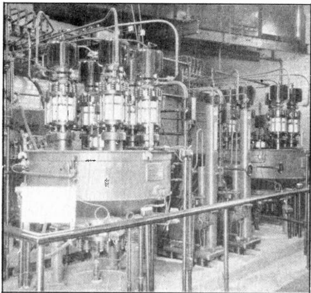
Fig. 5. This photo shows an excellent view of two 500-kw., 600-volt mercury arc rectifiers. Note the insulators on the tank supports and also the insulating bushings through which the anodes enter the tank at the top. The vacuum pumps and a number of pieces of auxiliary equipment can be seen between the two units and in the background of the photo. (Courtesy General Electric Co.)
