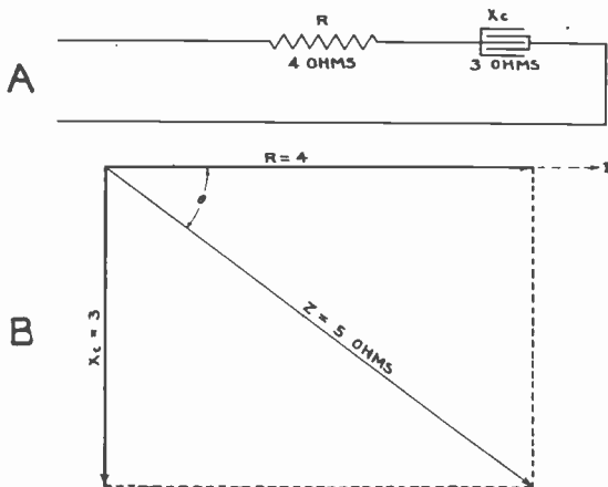
Fig. 9. "A". This circuit has a resistance connected in series with a Condenser. "B". The vector diagram shows the method of determining the impedance and angle of lead between the current and voltage for a circuit such as shown at "A".
