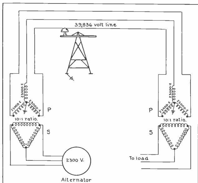
Fig. 12. This diagram illustrates the method and advantage of using star-delta and delta-star transformer connections with transmission lines.
