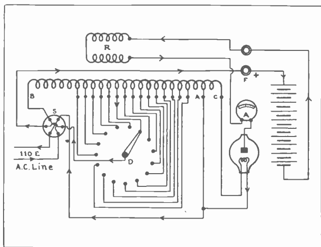
Fig. 7. Wiring diagram of a Tungar type bulb rectifier showing the taps on the auto transformer winding for varying the charging voltage.
