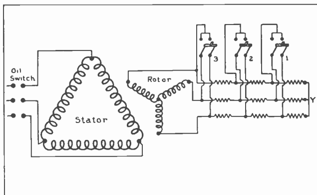
Fig. 14. Connection diagram of slip-ring induction motor with knife switches used to cut out the starting or speed control resistance step by step.
