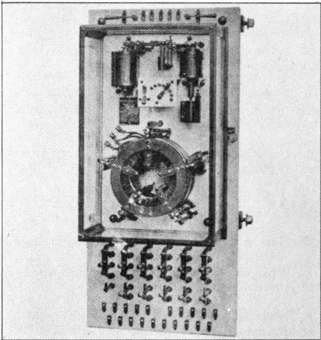
Fig. 16. Automatic voltage regulator for controlling the voltage of several alternators in parallel. (Photo Courtesy General Electric Co.)
