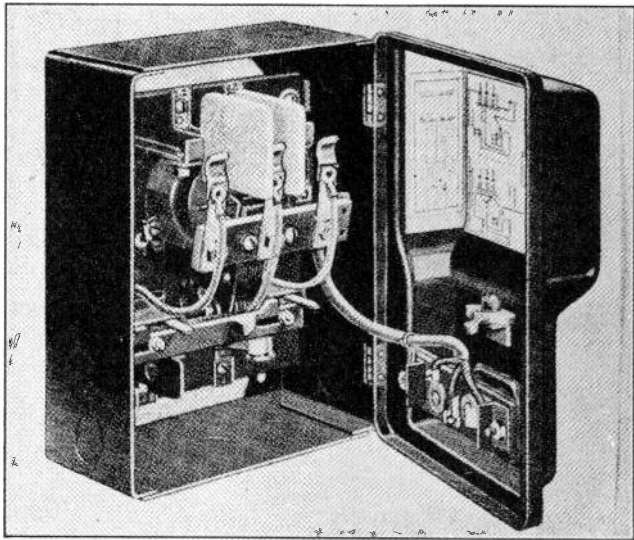
Fig. 3. This view shows a complete across-the-line starter for a three-phase, A. C. motor. The mechanism is enclosed in a safety cabinet with push button control attached to the cabinet cover. (Courtesy Allen Bradley Co.)
