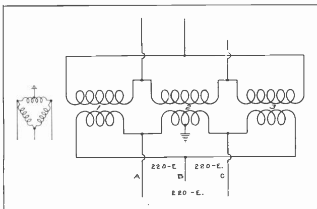
Fig. 15. This sketch shows the method of grounding the secondary circuit of a bank of transformers on which the secondary is connected delta.
