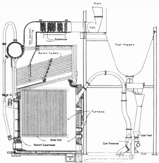
Fig. 7. Diagram of a modern power plant boiler using pulverized coal for fuel. Note the coal hopper, pulverizer, furnace feed tube, and also the economizer which is located above the boiler.
