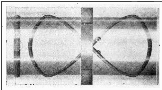
Fig. 5. Phantom view of sleeve bearing, showing oil grooves and oil ring slot.
