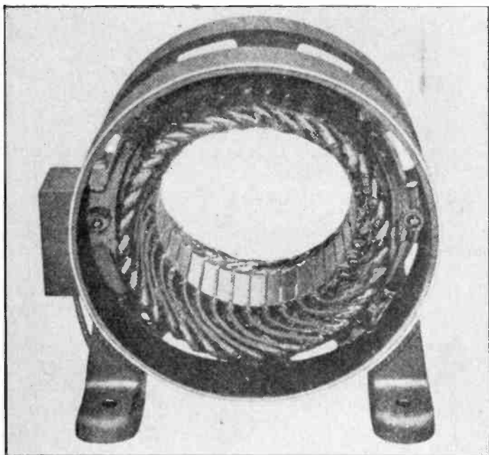
Fig. 6. This view shows a stator of an induction motor with the end shields and rotor removed. When A. C. is applied to the winding a revolving magnetic field is set up around the inside of the stator core.
