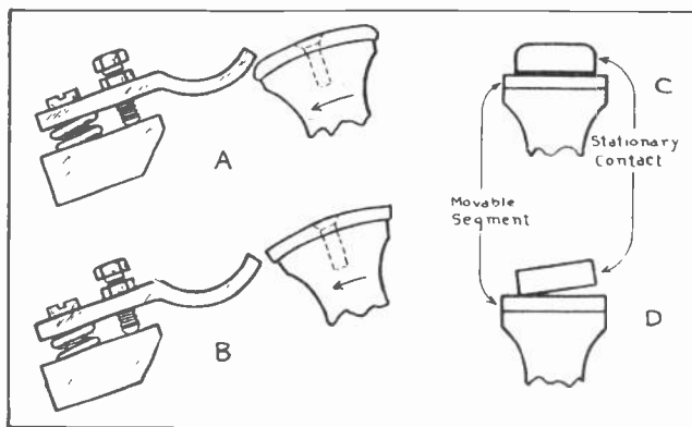
Fig. 21. At "A" is shown the proper shape and position of the segment and contact finger of a drum controller. At "B" is shown the wrong position and unrounded corners of these contacts. At "C" and "D" are shown the right and wrong positions of the stationary contact on the movable segment.
