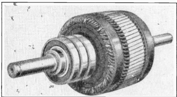
Fig. 10. Wound rotor of a variable speed slip-ring motor. This rotor has windings of insulated copper wire similar to those in D. C. armatures.
