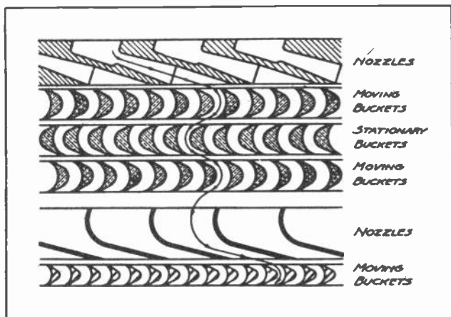
Fig. 12. This sketch illustrates the operating principles of a steam turbine. Note the nozzles and stationary and moving blades or buckets. Courtesy of Elliott Company.
