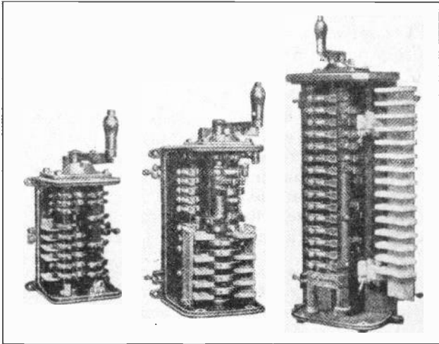
Fig. 14. Three drum controllers of different types and sizes showing the variety of arrangements that can be made with their contacts and segments. (Courtesy Cutler Hammer Mfg. Co.)
