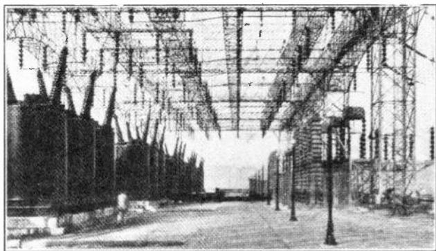
Fig. 14. View of large oil switches and lightning arresters underneath the bus and switching structure of a 220,000-volt outdoor substation. Courtesy of Philadelphia Electric Company.
