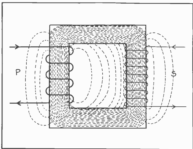
Fig. 17. This sketch illustrates the operating principle of a simple transformer and shows the manner in which the primary flux passes through the core and induces voltage in the secondary winding.
