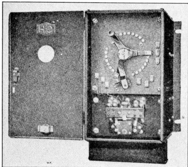
Fig. 7. Three-phase resistance starter of the face plate type. When the rheostat armature is rotated, resistance is cut out of all three phases at once. (Courtesy Cutler Hammer Mfg. Co.)
