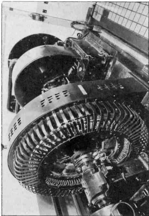
This Westinghouse generator is driven by an airplane engine on break-in run, to develop power to make more airplane engines. It is one of many such synchronous machines connected to a common bus in a plant of the Ford Motor Company.
