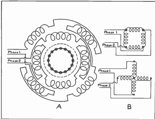
Fig. 2. A. This diagram shows the connections of the stator windings of a two-phase induction motor. At B are shown two schematic diagrams illustrating different methods of connecting two-phase windings.
