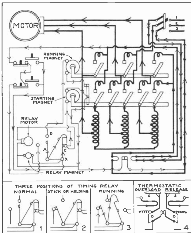
Fig. 5. This diagram shows the complete circuits of an automatic controller with magnetically-operated contactors in the starting and running circuit, and a motor-operated timing relay to regulate duration of the starting period. Trace all parts of this circuit carefully with the accompanying explanation.
