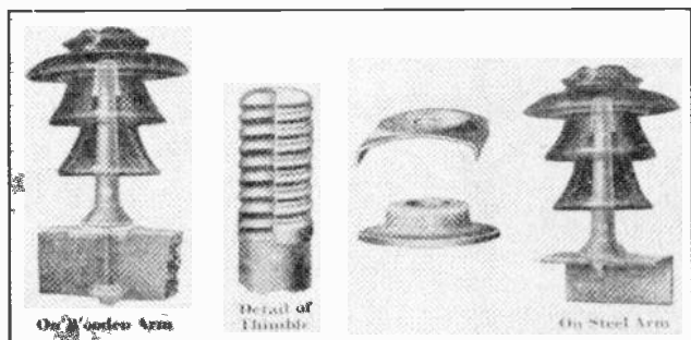
Fig. 15. Above are shown the methods of mounting insulators on pins and attaching the pins to wood and metal cross arms, and also the soft lead thimble which enables the insulator to be securely tightened on the pin without damaging the threads in the porcelain. Courtesy of Ohio Brass Company.
