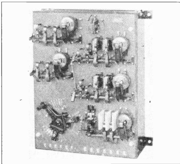
Fig. 8. This photo shows a front view of an automatic, panel type controller with a hand-operated, speed-regulating rheostat. (Photo courtesy General Electric Co.)
