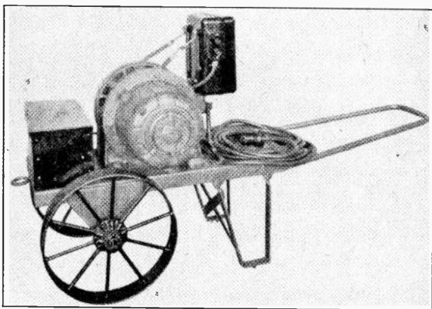
Fig. 23. Portable A.C. induction motor particularly adapted for use on farms and for driving portable machinery. (Courtesy G. E. Company)
