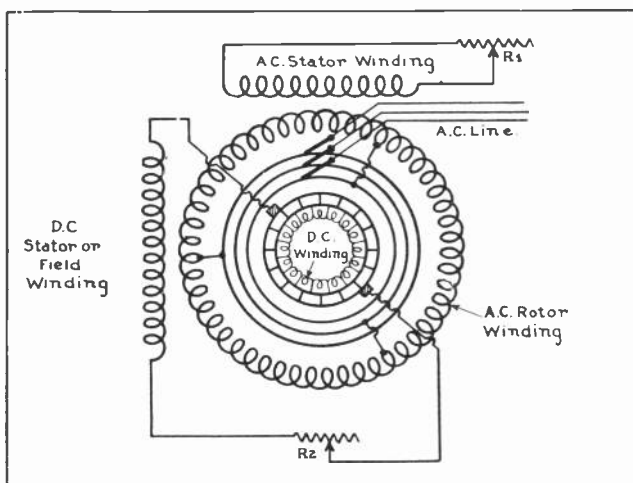
Fig. 19. Diagram showing the connections of the armature and field of a Fynn-Weichsel motor. Note that both the stator and armature have two separate windings.
