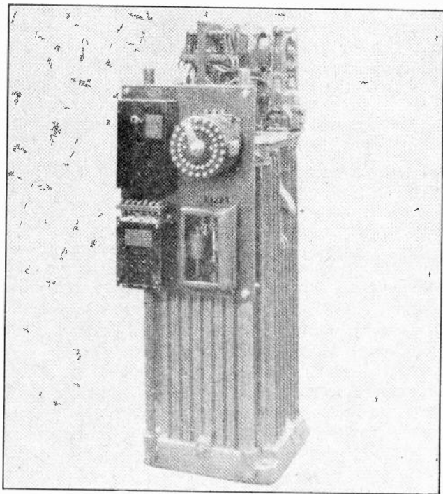
Fig. 9. This photo shows a single-phase regulator enclosed in its tank and equipped with the operating motor and control relays. (Photo Courtesy General Electric Co.)
