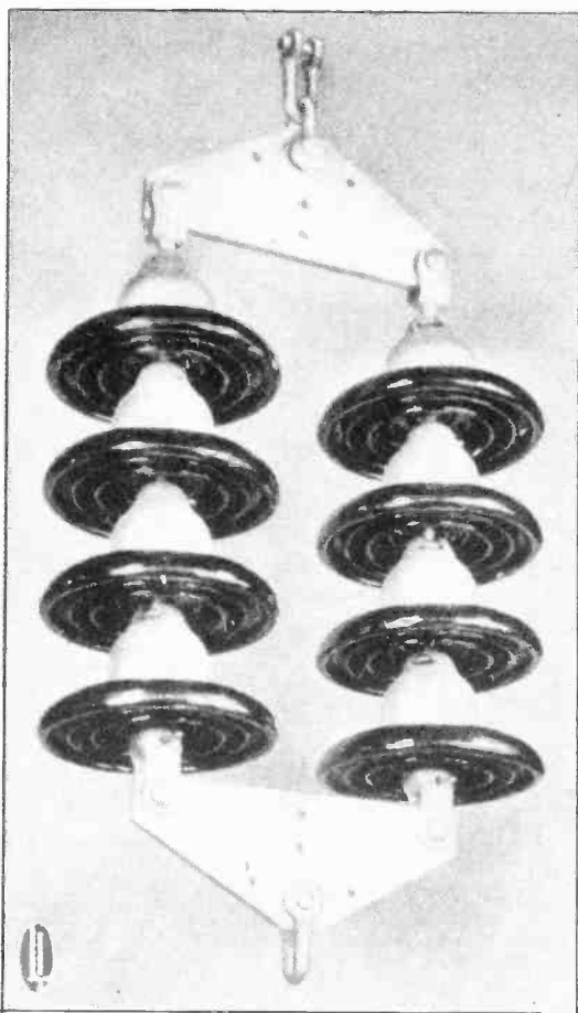
Fig. 27. Two strings of strain insulators fastened together with evener bars to take the strain of a very heavy conductor span. Courtesy Lapp Insulator Co., Inc.
