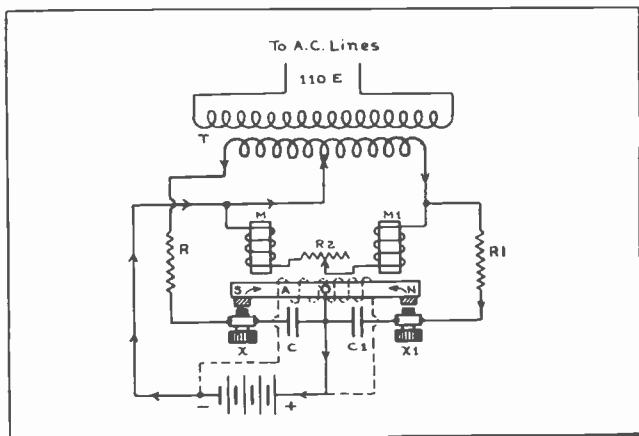
Fig. 1. The above diagram shows the parts and connections of a simple mechanical rectifier of the vibrating type. The synchronous operation of the contacts delivers pulsating D.C. to the battery circuit.
