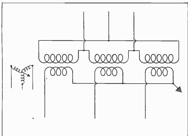
Fig. 16. This sketch shows the location of the ground connection on a bank of transformers with the secondary connected star. Read carefully the explanation of the advantages of this system which are given in the accompanying paragraphs.
