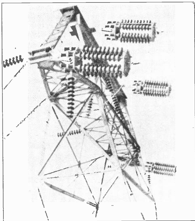
Fig. 28. Extra heavy strain tower with six strings of insulators grouped together on evener plates for each conductor. Note the heavy coil springs on the left evener plates to allow the heavy tension of these 3800-ft. river spans to equalize on all six insulator strings. Courtesy Lapp Insulator Co., Inc.
