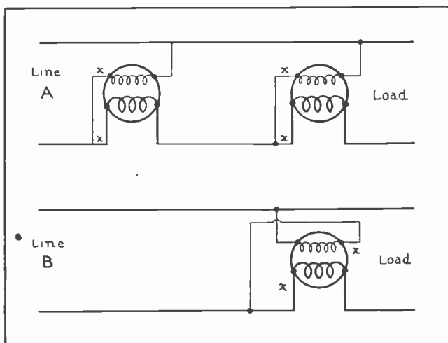
Fig. 5-A. Above is shown the method of connecting wattmeters to a single-phase circuit to locate the proper terminals of the potential and current coils.
