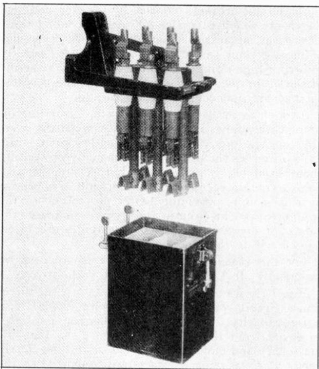
Fig. 1. View of a three-pole, 3300-volt, 200 ampere oil switch with oil tank removed to show contacts. Courtesy of G. E. Company.
