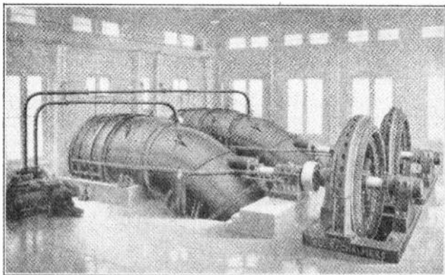
Fig. 8. This photo shows 2600-h. p. synchronous motors driving low-pressure, screw type water pumps. (Photo courtesy Allis-Chalmers Mfg. Co.)
