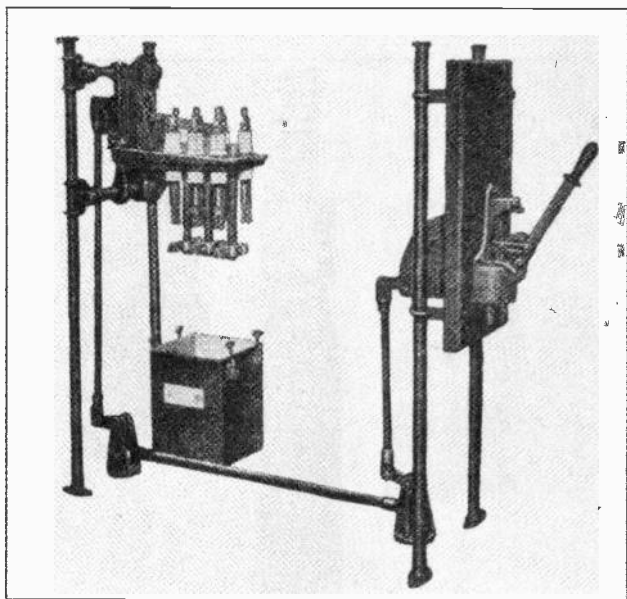
Fig. 2. This figure illustrates the method of obtaining remote mechanical control for an oil switch located several feet back of the switchboard. Courtesy of G. E. Company.
