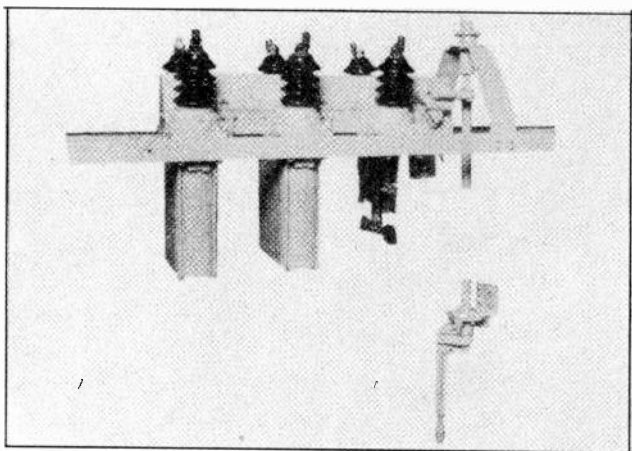
Fig. 5. 15,000-volt, 400-ampere, triple-pole oil switch with one tank removed. Note that the pole elements of this switch are each enclosed in a separate tank. Courtesy of G. E. Company.
