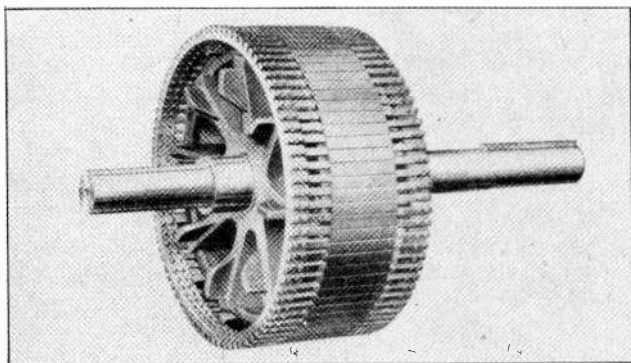
Fig. 9. This photo shows an excellent view of a squirrel-cage rotor using square bars which are riveted to heavy end rings.
