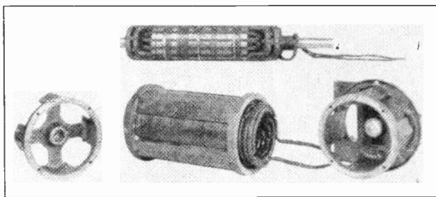
Fig. 7. This photo shows the stationary, primary, and rotating secondary windings of an induction voltage regulator. (Photo Courtesy General Electric Co.)
