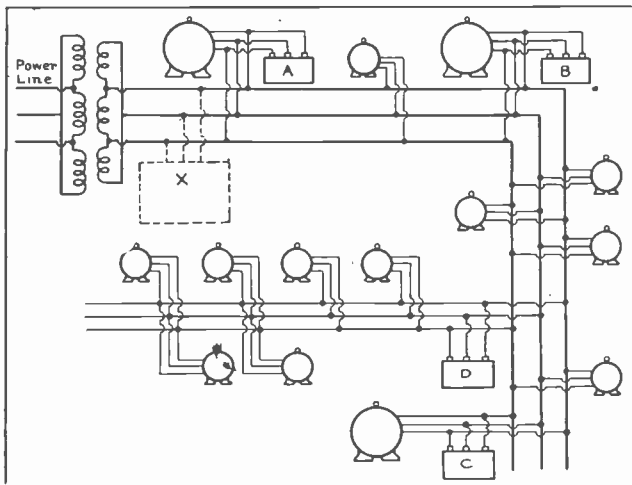
Fig. 8. This diagram illustrates the manner in which condensers can be connected to individual large motors and also at load centers to correct the power factor for a group of small motors.
