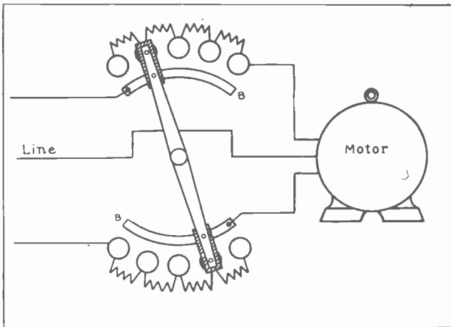
Fig. 9. Diagram showing the connections and circuit through a three-phase resistance type starter.
