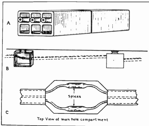
Fig. 5. "A" shows underground conductors run in tile ducts. "B". This sketch shows the arrangement of man holes and cable ducts underground. "C". Cables spread apart and supported in racks on the walls of man holes allow working room for making splices, tests, etc.
