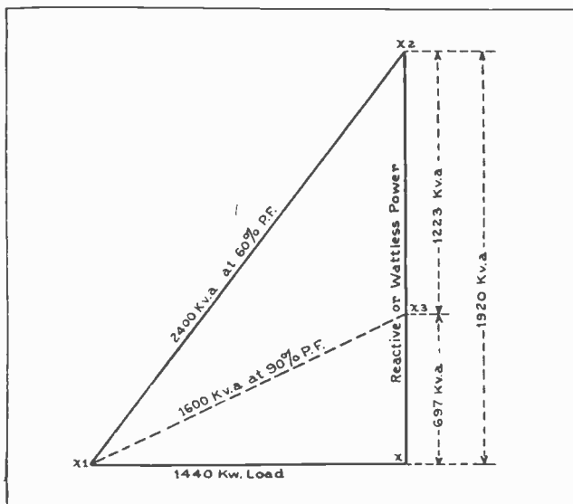
Fig. 9. The above sketch shows the simple method by which power factor problems can be solved graphically by drawing to scale the lines representing the various factors in the problem. Study this diagram very thoroughly with the accompanying explanations.
