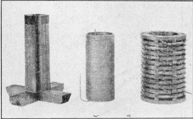
Fig. 4. This view shows a partly assembled core of the distributed type and the primary and secondary windings which are ready to be placed on the core. (Photo courtesy General Electric Co.)
