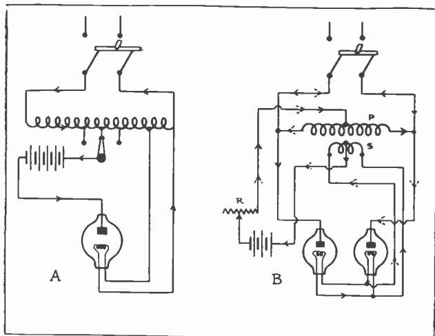
Fig. 5. A shows a circuit of a simple half-wave rectifier of the bulb type, and B shows the circuit of a full-wave rectifier using two bulbs. Trace each of these circuits very carefully.
