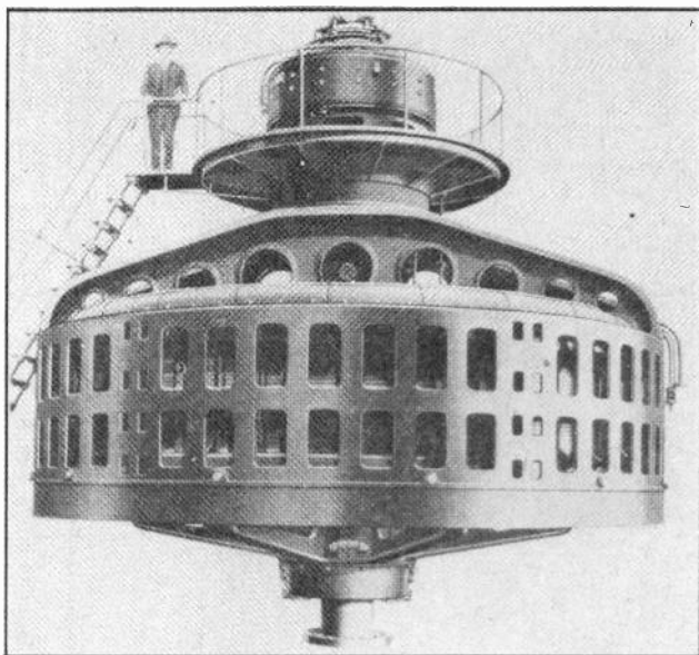
Fig. 4. Large vertical type alternator for water-wheel drive. The stator core and windings of this machine lay in a horizontal position just inside the lower frame work, and the field poles revolve on the vertical shaft within the stator. (Photo Courtesy Allis Chalmers Mfg. Co.)
