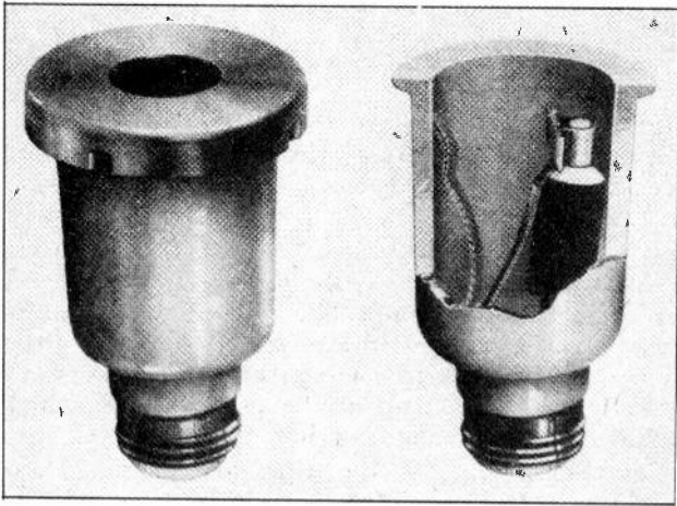
Fig. 9. Convenient plug type thermal relay for protection of circuits to small motors and other equipment.
