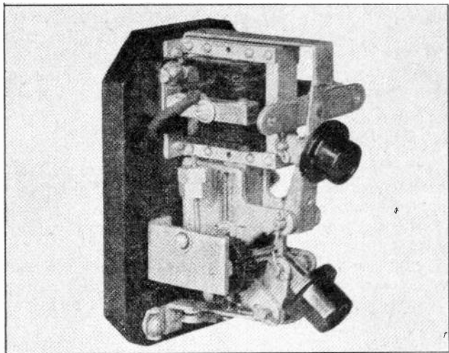
Fig. 8. Push button station with cover removed to show contacts and relay magnet.
