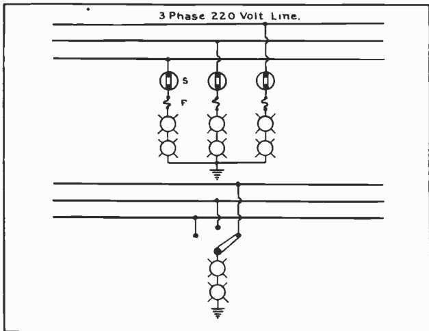
Fig. 8. Two methods of connecting lamps to serve as simple ground detectors on three-phase power circuits.
