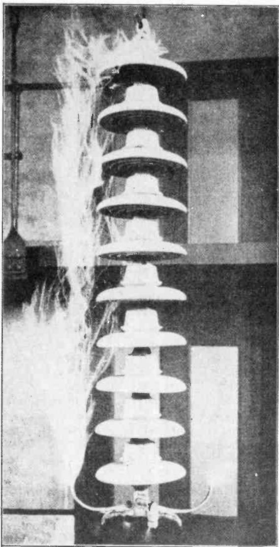
Fig. 1. This very interesting photograph shows an actual flashover or high-voltage arc on a string of 10 suspension insulator units. This flashover was made with 500,000 volts in a test laboratory, but similar flashovers occur on line insulators in service, due to lightning. Courtesy Ohio Brass Co.
