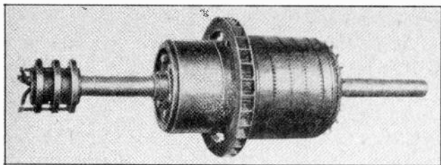
Fig. 16. Armature of a BTA motor showing the commutator, slip-rings, and ventilating fan. (Courtesy G. E. Company.)
