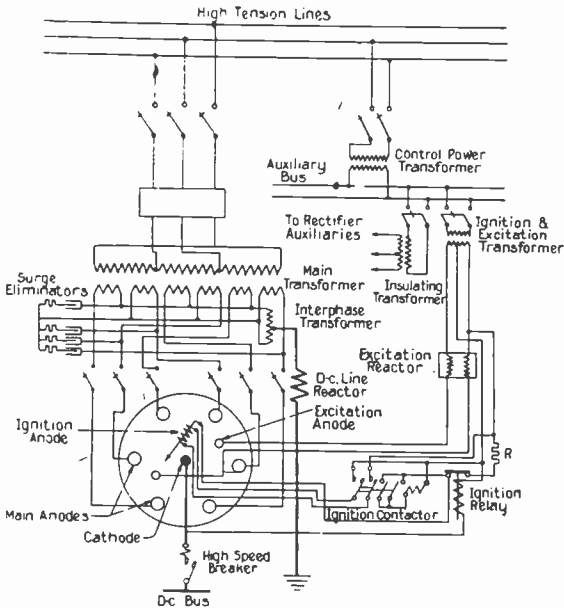
Fig. 11. Wiring diagram of a six-phase rectifier showing transformer connections and auxiliary control circuits. (Courtesy American Brown Boveri Co.)
