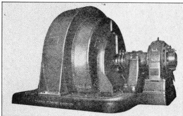
Fig. 1 5000-kv-a., 2300-volt, enclosed-type, synchronous condenser. The exciter for this machine is shown on the right. (Photo courtesy G. E. Company).
