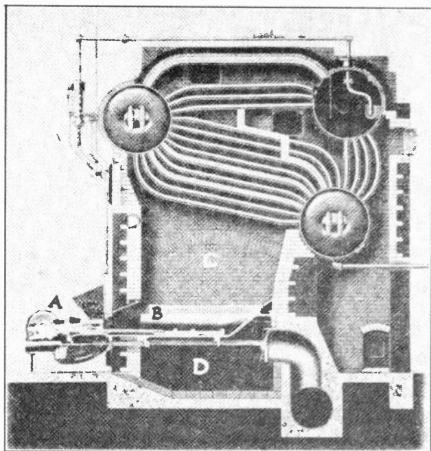
Fig. 6. Sectional view of a water tube boiler with an automatic stoker to feed the coal to the burners or combustion chamber "C".
