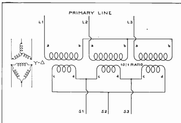
Fig. 10. Three-phase transformer bank with the primary connected star and the secondary delta. This connection is called "star-delta."
