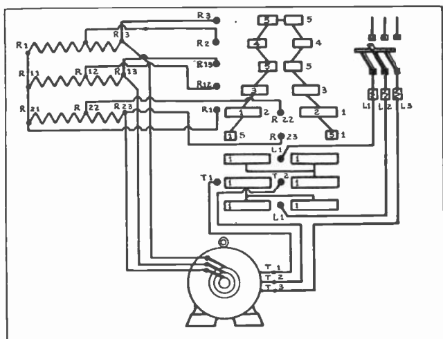
Fig. 15. Circuit diagram of a simple drum controller for starting and reversing three-phase, slip-ring motor. Trace the circuit carefully with the accompanying explanation.
