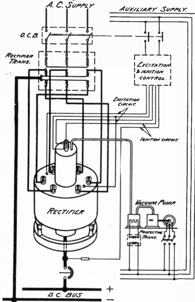
Fig. 9. Wiring diagram showing the power and auxiliary circuits for a six-phase mercury arc power rectifier. (Courtesy American Brown Boveri Co.)
