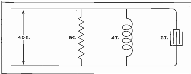
Fig. 14. Note the amount of current in each of the branches of the above circuit and compare sketch with Fig. 15, while determining the total current in this circuit.
