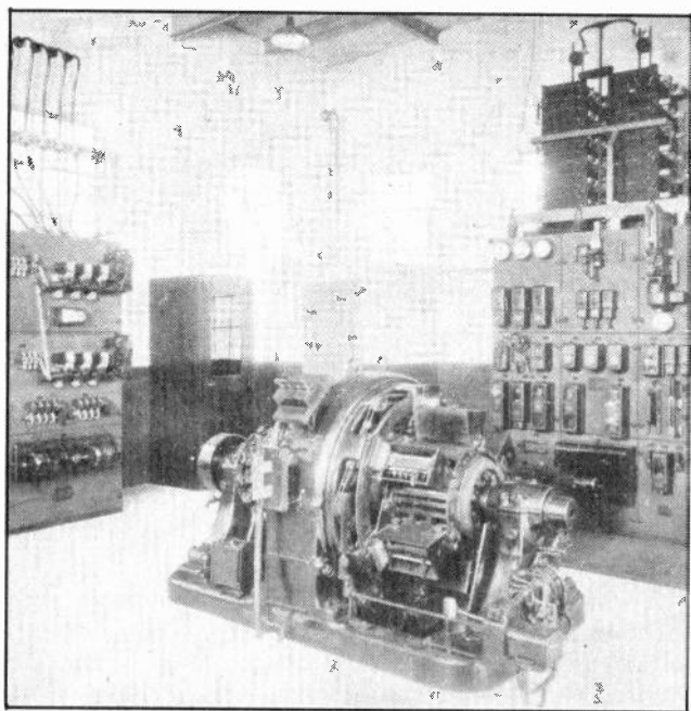
Fig. 5. This photograph gives an excellent view of the inside of an automatic converter substation. The converter is shown in the foreground, the starting panel at the left, and the main switchboard with the automatic control relays and circuit-breakers in the right background. Courtesy of General Electric Co.
