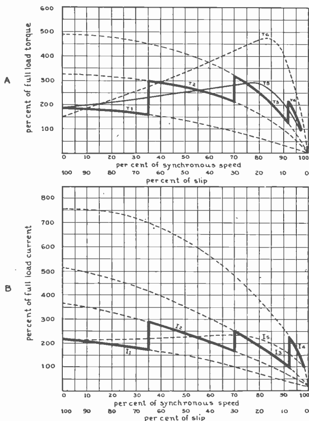
Fig. 15. "A" shows the torque curves of a slip-ring induction motor as the resistance is cut out of the rotor circuit and the motor comes up to speed. "B" shows the current curves of the same motor and corresponding to the various steps of the torque curves. Study these curves very carefully with the accompanying explanation.
