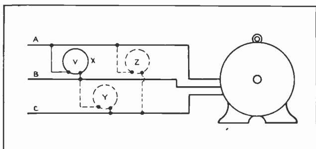
Fig. 4. This diagram shows three different connections for a voltmeter used to measure the voltage of each phase of the three-phase line to this motor.
