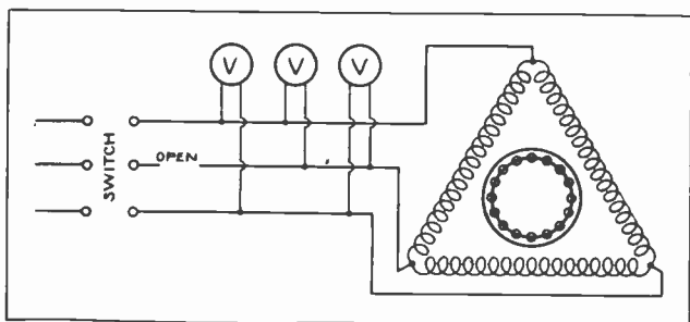
Fig. 3. Sketch illustrating wrong method of testing for an open phase. Ammeters provide a more dependable indication.
