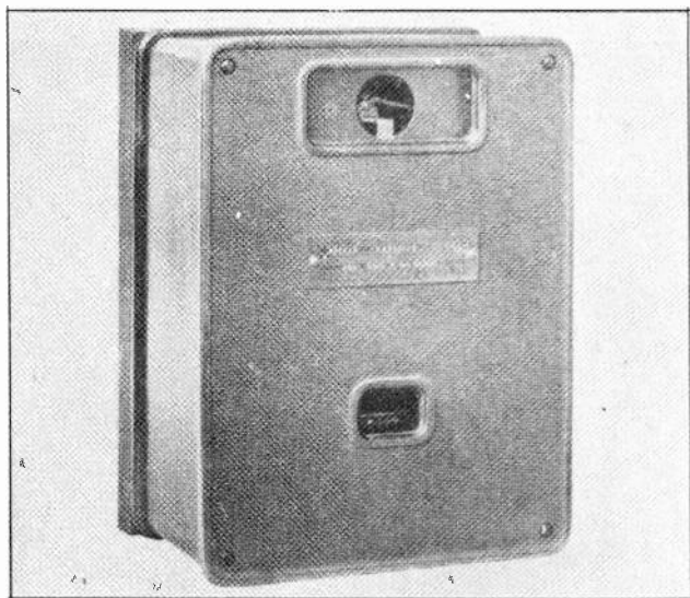
Fig. 24. Photo of a polyphase reverse-power relay for A. C. circuits in substations and power plants. Photo Courtesy of G. E. Company.
