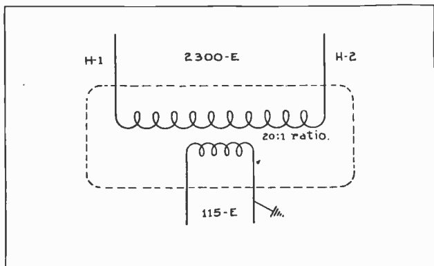
Fig. 1. The above sketch shows a schematic diagram of the primary and secondary windings of a single-phase transformer. This transformer has a step-down ratio of 20:1 and one side of the secondary is grounded, as is common practice.
