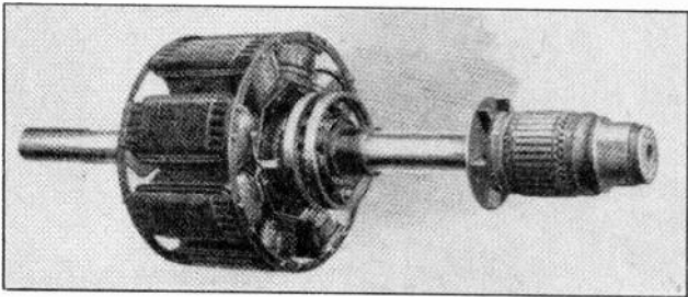
Fig. 3. This view shows the construction of the rotor or revolving field of an alternator similar to the one shown in Fig. 2. Examine its construction carefully and note the position of the collector rings and exciter-armature on the shaft.
