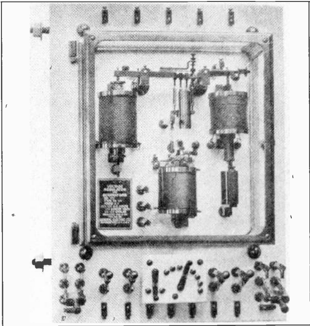
Fig. 15. This photo shows an automatic voltage regulator of a type similar to the one for which the wiring was shown in Fig. 10, and shows the arrangement of the solenoids and relays on the panel. (Photo Courtesy General Electric Co.)
