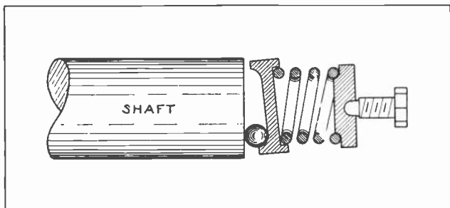
Fig. 12. Diagram showing ball and spring oscillator to cause converter armature to move endwise and promote even wear on the commutator.
