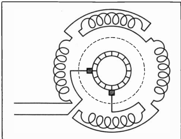
Fig. 21. Stator and armature connections for a series A. C. motor of the universal type which can be operated on either D. C. or A. C.
