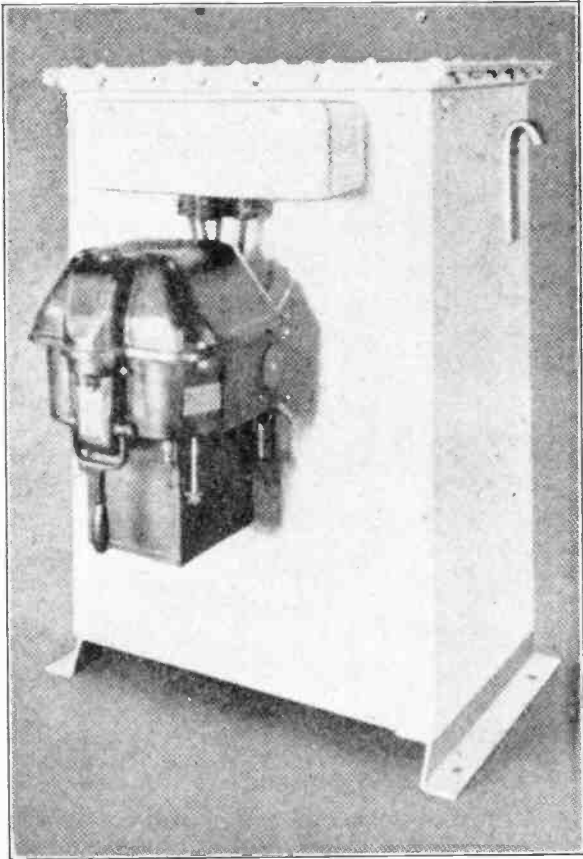
Fig. 6. This photo shows a static condenser enclosed in a moisture-proof metal tank and equipped with an oil switch for breaking the circuit between the condenser and the line. These condensers are made for both indoor and outdoor service. (Courtesy Electric Machinery Mfg. Co.)
