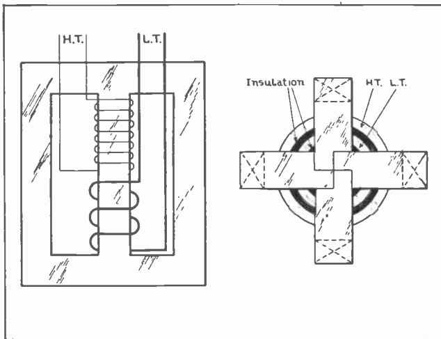
Fig. 2. The diagram on the left shows a transformer with a shell-type core, and on the right is shown the top view of a transformer with a distributed-type core. This view shows the top edges of the coils and insulation, while the sketch on the left shows a schematic diagram of the coils in their position on the core.
