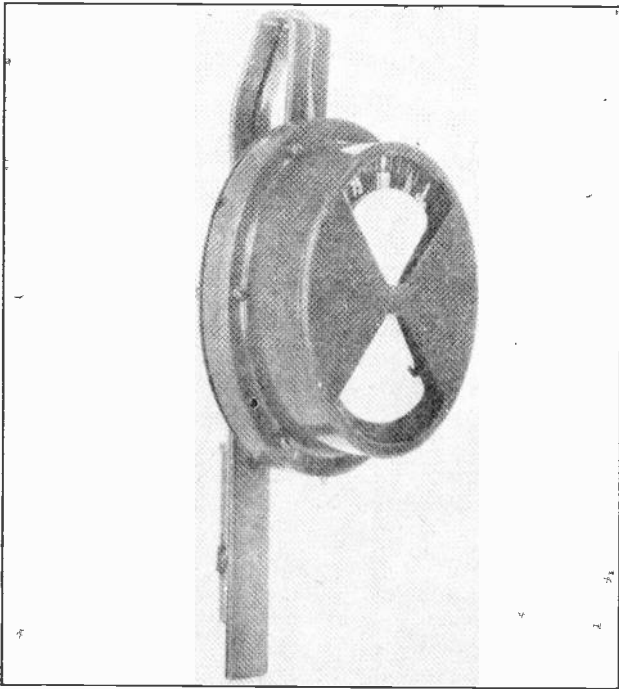
Fig. 14. This photo shows a temperature-indicating device for use with pole type transformers. This device is called a thermotest and indicates both excessive temperatures and overload of a transformer on which it may be installed.
