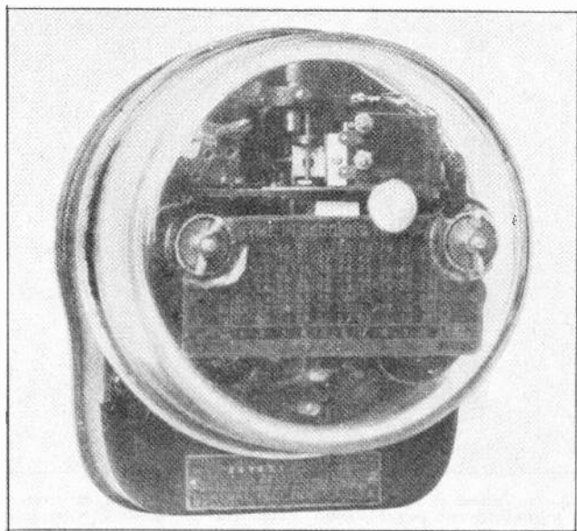
Fig. 23. Modern induction type overload relay such as very extensively used in A. C. power plants and substations. Courtesy of G. E. Company.
