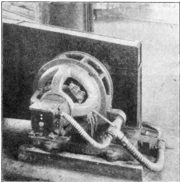
Fig. 2. Induction motor installation, using rigid conduit to bring the wires up to the motor, and flexible conduit to attach to the motor to allow it to be moved slightly for belt adjustment. Courtesy of G. E. Company.
