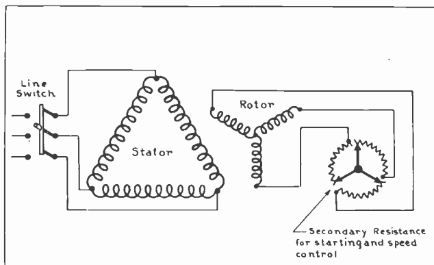
Fig. 13. The above diagram shows the connections of the stator and rotor of a slip-ring induction motor, and also the variable resistance used in the rotor circuit for starting and speed control.
