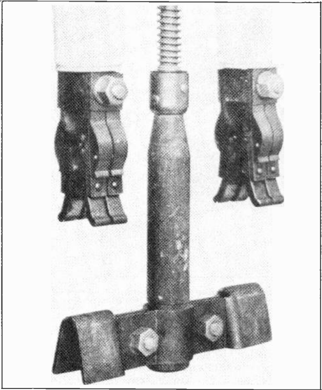
Fig. 3. Close-up view showing the details of construction of stationary and movable contacts of an oil switch. The upper stationary contacts are supported on porcelain bushings and the lower movable contact on a wooden insulating rod. Courtesy of G. E. Company.
