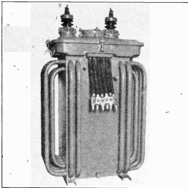
Fig. 10. This transformer is equipped with cooling tubes to allow the oil to circulate outside of the tank and give off its heat more rapidly to air.
