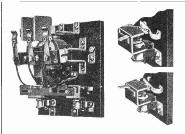
Fig. 2. This view shows on the left another type of an across-the-line starter, the mechanism being removed from the cabinet to show its construction. Also note the thermal overload-relays shown at the bottom of the panel on the left and in larger views on the right. (Courtesy Allen Bradley Co.).
