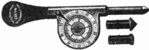
Fig. 10. Revolution counters or speed indicators of the above type are very convenient for checking the speeds of motors and generators.
