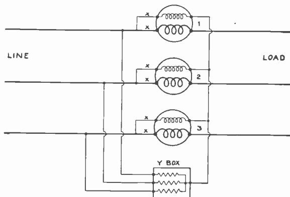
Fig. 11. Meter connections for a "three wattmeter method" for measuring the total power in a three-phase circuit. The Y Box shown in this diagram is explained in the accompanying paragraphs.
