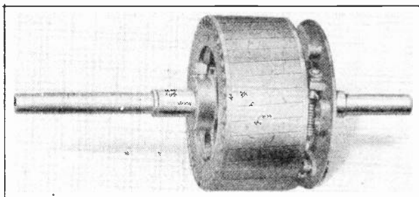
Fig. 12. Small squirrel-cage rotor such as used in single-phase induction motors. Note the centrifugal switch mechanism on the right end.
