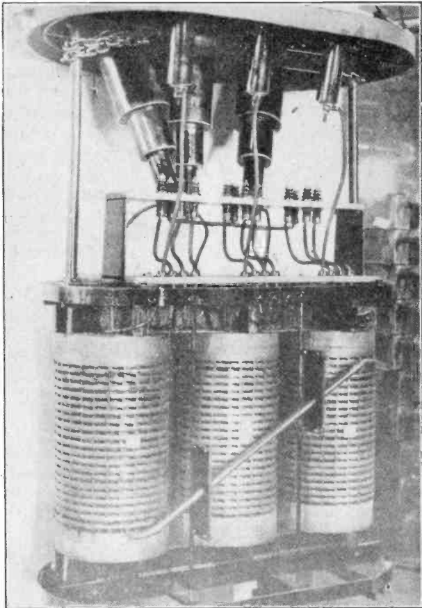
Fig. 15. This view shows the core and windings of a high voltage, three-phase transformer and also the lower ends of the insulating bushings through which the high voltage and low voltage leads are taken from the tank.
