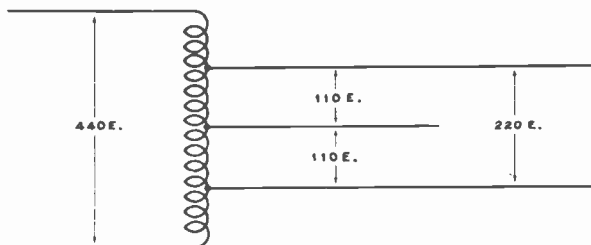
Fig. 4. Auto transformer connection for obtaining both 110 and 220 volts from a 440-volt line.
