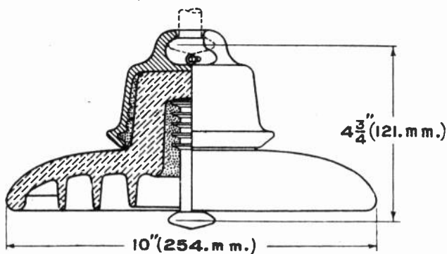
Fig. 22. Sectional view of a suspension type insulator unit showing how the metal cap and pin are securely cemented to the porcelain insulator disk. - Courtesy Ohio Brass Co.
