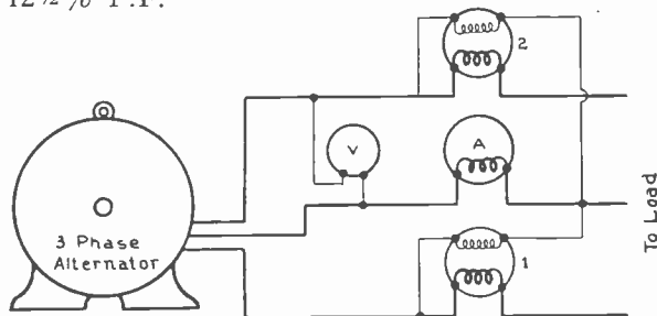
Fig. 13. Voltmeter, ammeter, and wattmeter connected to measure the voltage, current, and power output of a three-phase alternator.
