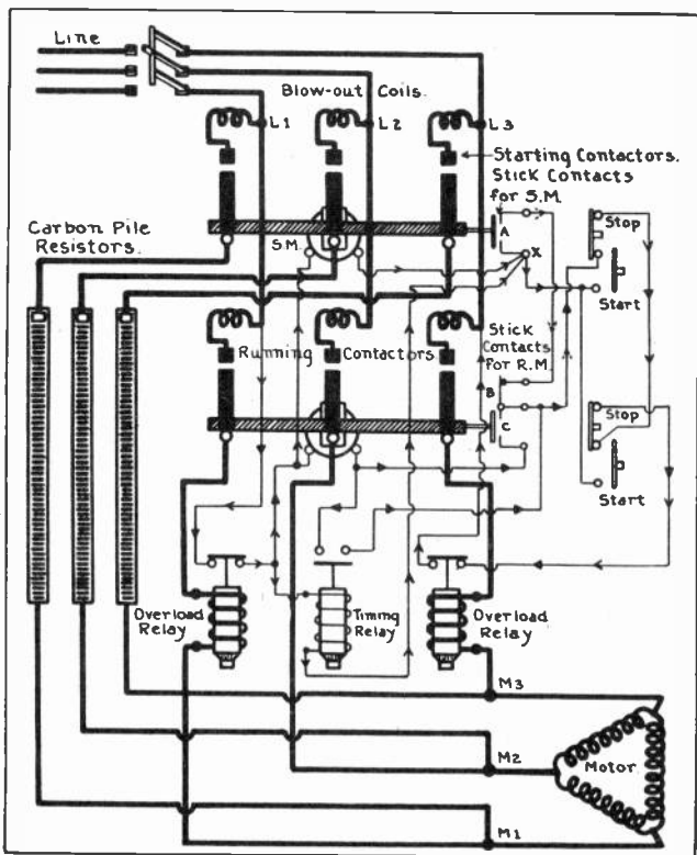
Fig. 15. Diagram showing wiring of an automatic, three-phase, carbon pile starter. Note the main power circuit traced in heavy lines from the line switch to the motor and also the auxiliary control circuits traced in light lines.
