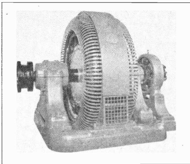
Fig. 4. This photo shows a 2000-h. p., 2300-volt, synchronous motor which operates at 100% power factor. The D. C. exciter-generator is shown on the right-hand end. (Photo courtesy General Elec. Co).
