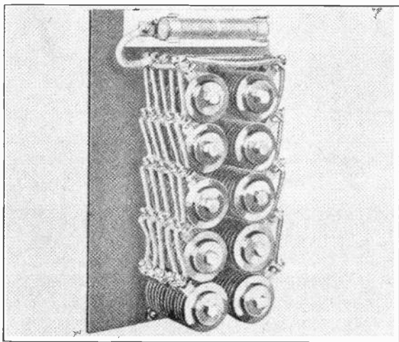
Fig. 11. Copper oxide rectifier consisting of a number of units connected in series and parallel to obtain increased voltage and current capacity. (Courtesy Westinghouse Elec. & Mfg. Co.)
