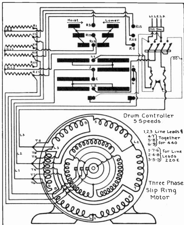
Fig. 17. Wiring diagram of a speed-regulating controller connected to a slip-ring motor. Carefully trace the circuits both to the stator and rotor of this machine.
