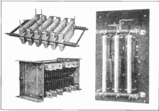
Fig. 8. This photo shows several types of resistance units used with A. C. motor starters. On the upper left are shown non-inductive, coil-wound resistors; on the lower left grid type resistors; and on the right edge-wound resistors made of strips of resistance metal wound edgewise around non-combustible cores.
