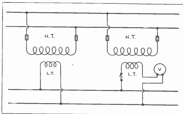
Fig. 4. This diagram illustrates the method of using a voltmeter to test the polarity of a transformer secondary before connecting it in parallel with another.
