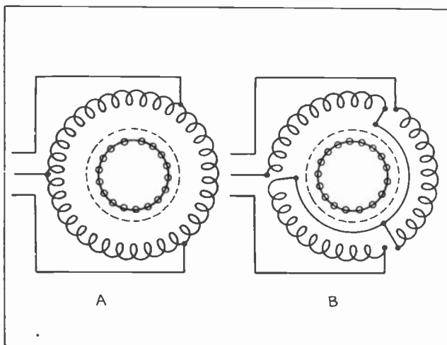
Fig. 3. A shows a delta-connected stator winding for an induction motor. The sketch at B shows a star-connected winding.
