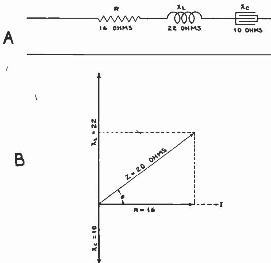
Fig. 10. "A". Resistance, inductance, and capacity connected in series in an A. C. circuit. "B". Note how the capacity reactance is subtracted from the inductive reactance, as the two neutralize each other in the circuit.
