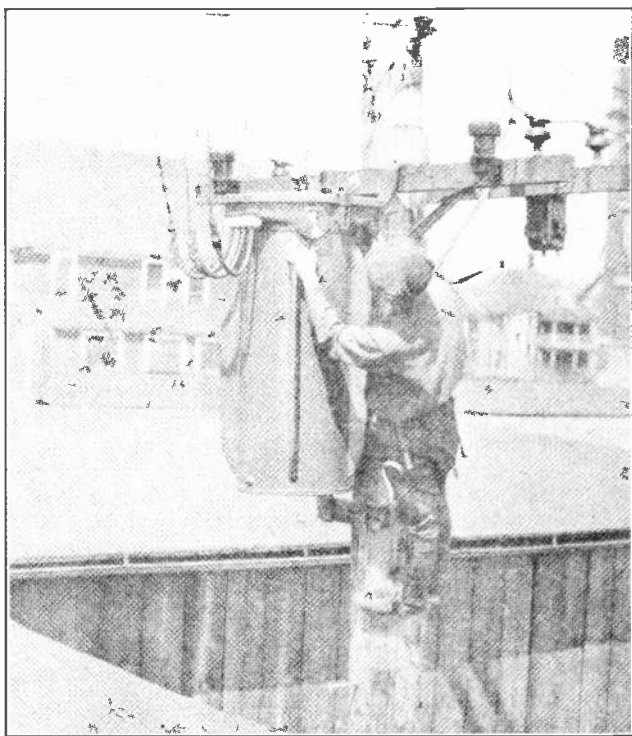
Fig. 6. This photo shows a pole type transformer and the method of making primary and secondary connections. Also note the thermometer temperature indicator near the hand of the electrician.
