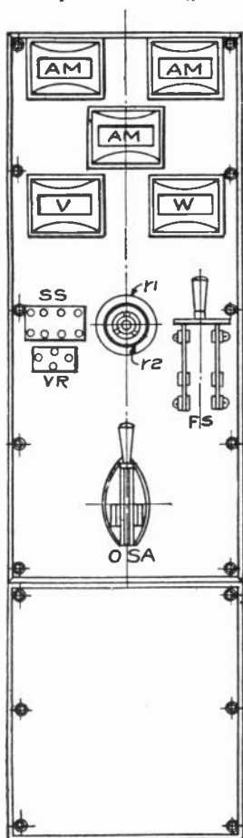
Fig. 2A. This figure shows the front view of a single panel of an A. C. switchboard. See Fig. 2B for the side view, and the wiring diagram.
