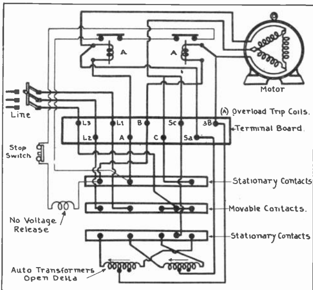
Fig. 4. Wiring diagram of a three-phase Westinghouse compensator using open-delta-connected auto transformers, and a stop switch in series with the no voltage release.
