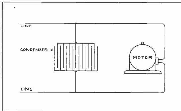
Fig. 7. A condenser connected in parallel with a motor will cause lagging voltage or leading current, and will neutralize effects of induction produced by the motor.
