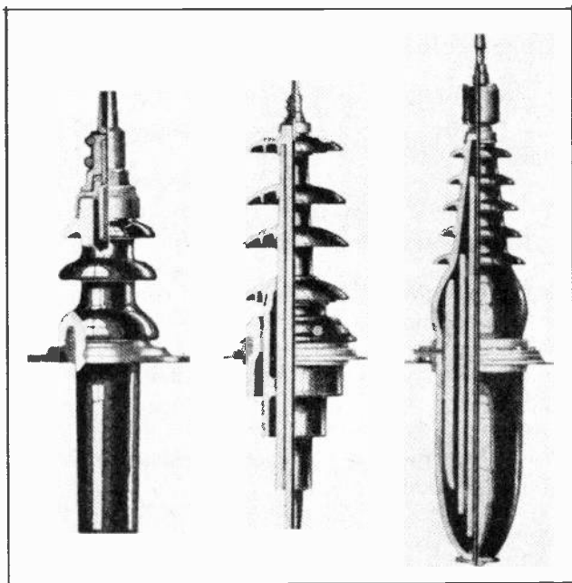
Fig. 30. Three different types of insulator bushings used for transformers and oil switches where the high-voltage conductors enter the metal tanks. Courtesy Ohio Brass Co.
