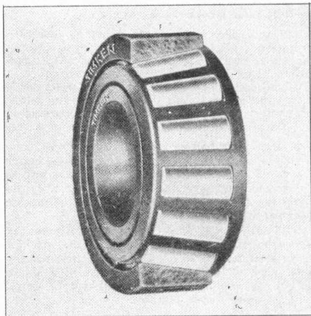
Fig. 2. Cutaway view of a Timkin tapered roller bearing such as commonly used in high grade motors.
