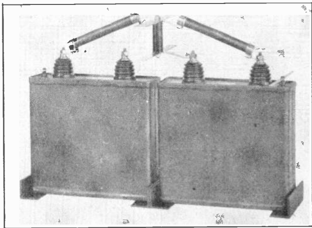
Fig. 3. Two single-phase condenser units connected together with discharge resistors in their circuit. (Courtesy G. E. Company).
