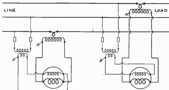
Fig. 10. Connections for two wattmeters on a three-phase circuit, using instrument transformers to reduce the voltage and current to the meters.
