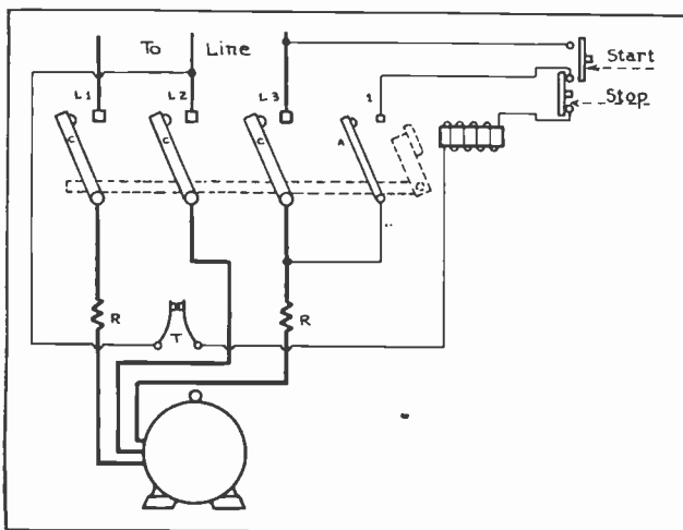
Fig. 5. Circuit diagram showing the connections for a simple across-the-line starter with the contactors operated by an electro-magnet which in turn is controlled by the stop and start buttons. Also note the thermal overload contacts, T, which are operated by expansion from the heat of resistors, R.
