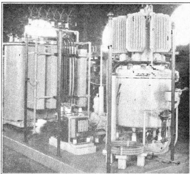
Fig. 4. The above photo shows a 600-kw., 575-volt, mercury arc power rectifier with the transformer and auxiliaries at the left. Note the cooling fins for radiators on the anodes. (Photo courtesy American Brown Boveri Co.)
