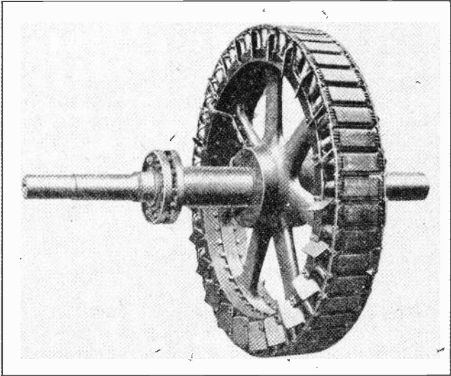
Fig. 3. Revolving field or rotor of a large slow-speed synchronous motor. Note the squirrel-cage damper winding attached to the pole faces and also the slip rings through which the D. C. is passed to the revolving field poles.
