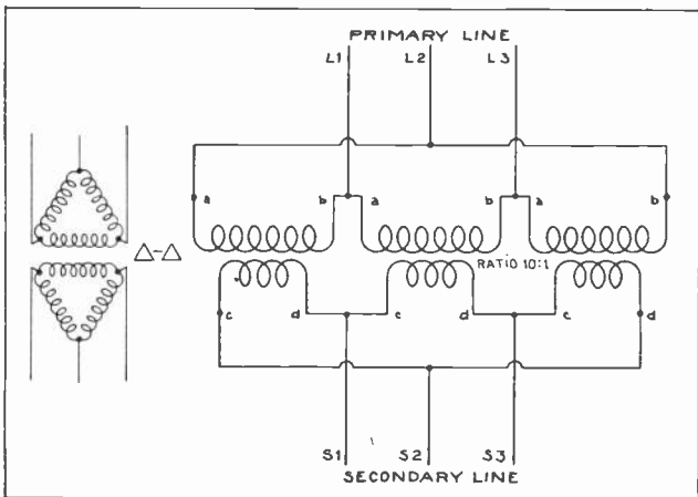
Fig. 9. Connection diagram for a three-phase bank of transformers connected delta-delta. Compare the large diagram with the small schematic sketch at the left and also with the explanation given in these paragraphs.
