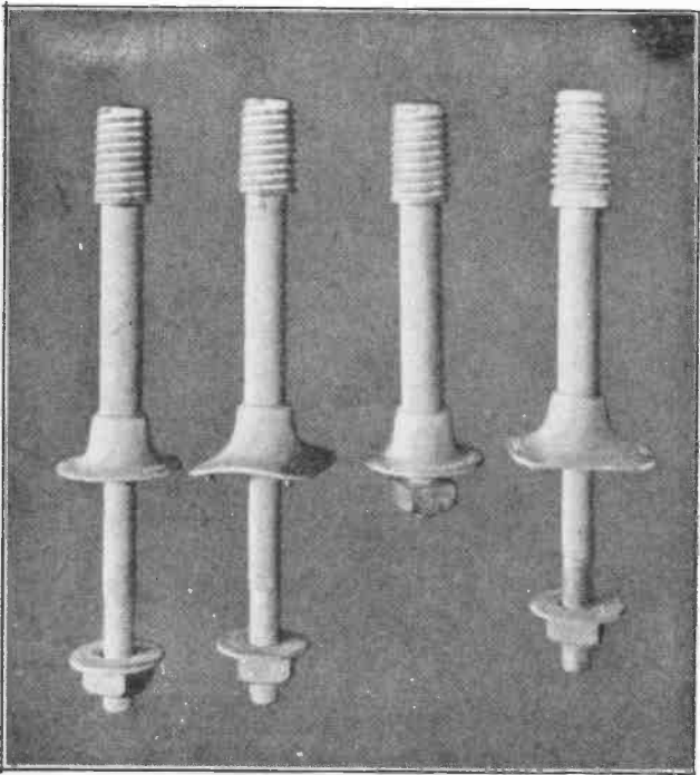
Fig. 14. Several styles of insulator pins used for attaching pin type insulators to wood and steel cross arms. Courtesy of Ohio Brass Company.
