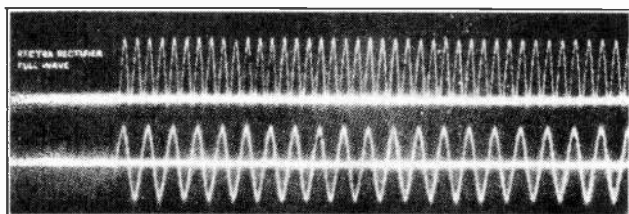
Fig. 13. Photo taken from an oscillograph record, showing the alternating current wave below and the rectified, pulsating D.C. wave above. (Courtesy Westinghouse Elec. & Mfg. Co.)
