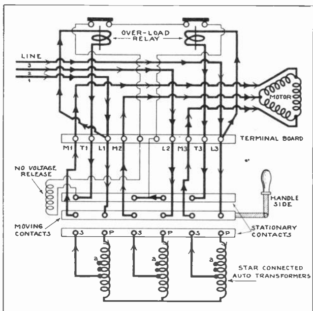
Fig. 3. Wiring diagram of a manually-operated compensator used for starting three-phase, squirrel-cage motors. Carefully trace the starting and running circuits with the accompanying explanation and also note the overload protective circuit.
