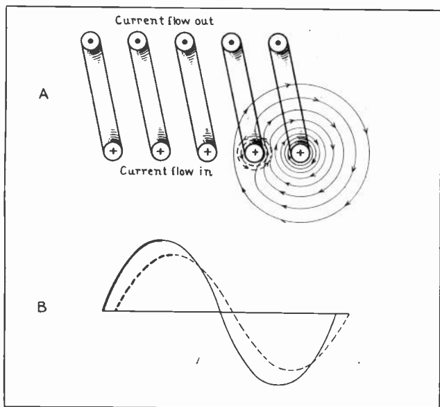
Fig. 2. The above diagram illustrates the manner in which the counter-voltage of self-induction is built up in an inductance coil.
