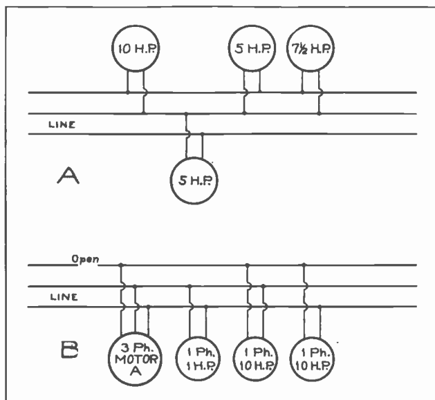
Fig. 2. Unbalanced voltage on three-phase circuits can be caused by unbalanced loads as at "A," or by an open on the line side of a polyphase motor as at "B."
