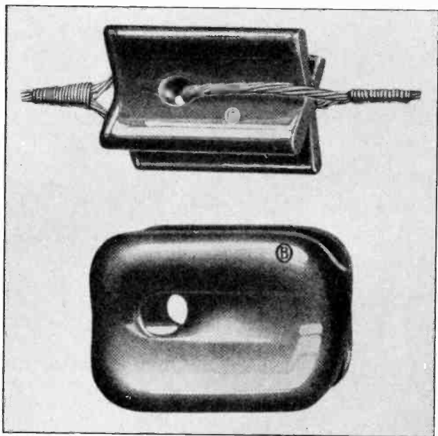
Fig. 29. Two types of small porcelain strain insulators for use on guy wires and low-voltage conductors. Courtesy Ohio Brass Co.
