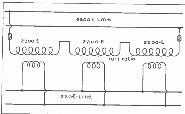
Fig. 5. Transformer primaries are sometimes connected in series to a line of higher voltage as shown above. The secondaries can then be connected for parallel operation.
