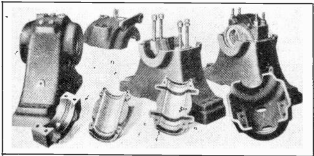
Fig. 8. Pedestal type sleeve bearings, showing parts of one bearing and housing disassembled.
