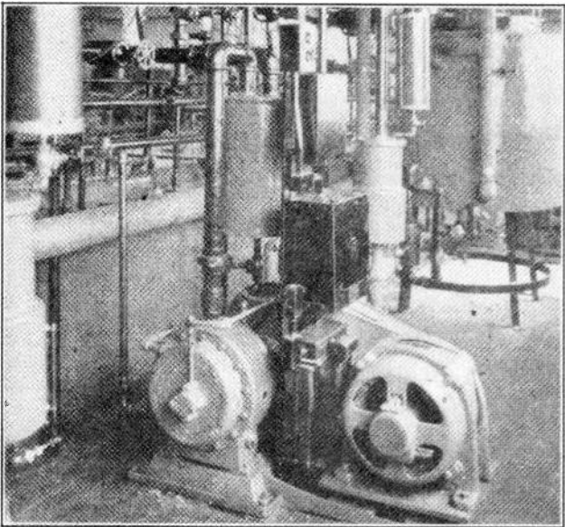
Fig. 3. This view shows a motor, push button control and a static condenser for power factor correction, all wired in conduit. Courtesy of G. E. Company.
