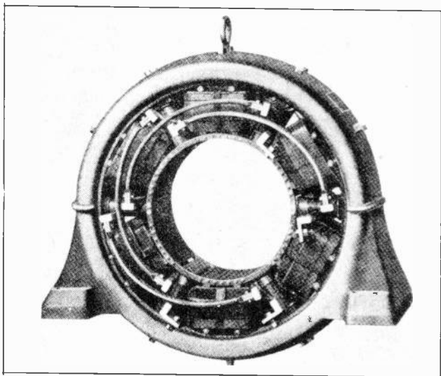
Fig. 3. Side-view of the field of a synchronous converter. Note the squirrel-cage damper winding in the faces of the main poles. Also the interpoles located between the main poles. (Courtesy Allis-Chalmers Mfg. Co.)
