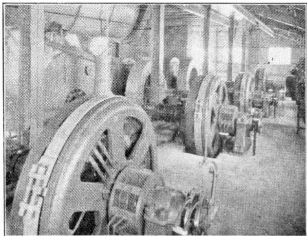
Fig. 11. This photo shows four large low-speed super-synchronous motors operating at 2200 volts and driving machines in a cement mill. (Photo courtesy G. E. Company.)
