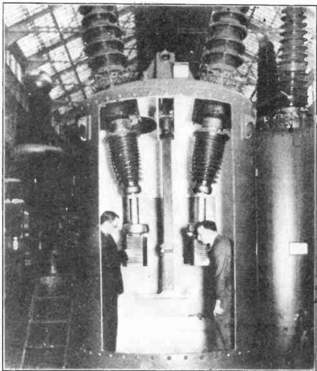
Fig. 9. This unique photograph clearly shows the inside of a large high-voltage oil switch equipped with Deion grids on the stationary contacts. Note the size of the contacts, insulators, and tanks required for handling the currents of high-voltage power lines. Courtesy of Westinghouse Elec. & Mfg. Co.
