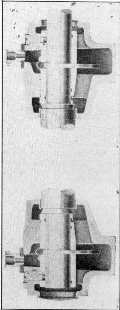
Fig. 4. Sectional views of two sleeve bearings, clearly showing the oil wells, oil rings, filler cups, etc.
