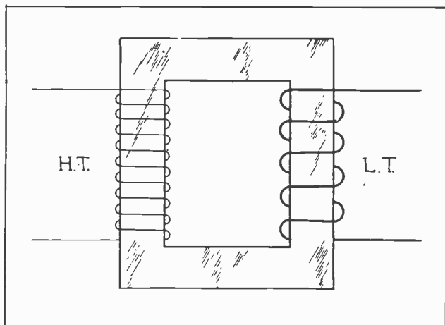
Fig. 1. This sketch shows the core and windings of a simple transformer. The winding on the left with the greater number of turns is the high tension winding, and the one on the right the low tension winding.
