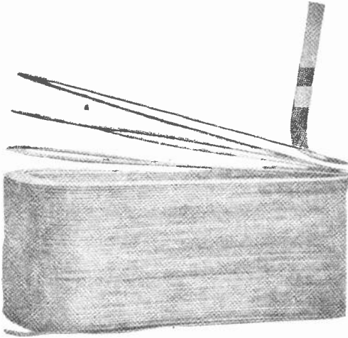
Fig. 11. Field coil which is wound with thin copper strip, making a coil which is very compact and easily cooled.
