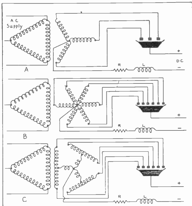
Fig. 10. The above diagrams show three different types of transformer connections which are commonly used with three-phase and six-phase mercury arc rectifiers.
