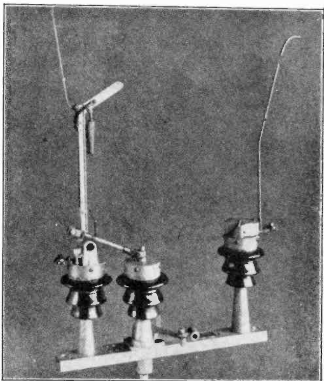
Fig. 12. This is another view of the same air break switch shown in Fig. 11. In this figure the switch is shown open. Note the movement of the center insulator by comparing the two views. Courtesy of Hi-Voltage Equipment Company.
