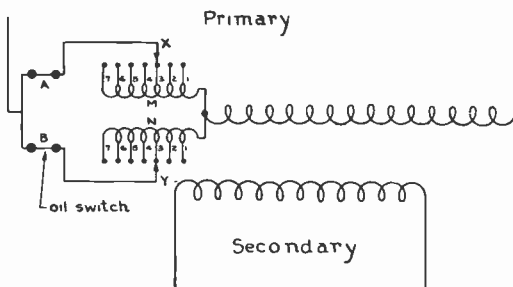
Fig. 1. This diagram shows a method of arranging adjustable connections on the primary of a tap-changing transformer.
