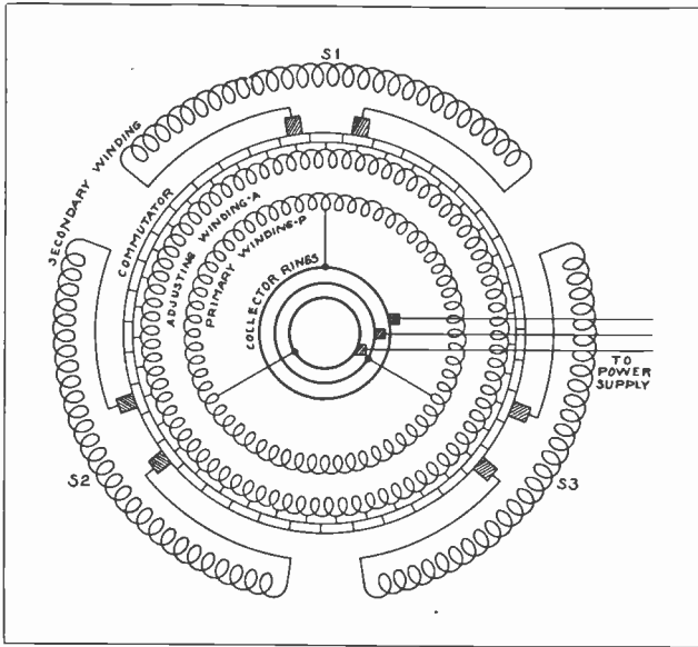
Fig. 15. This diagram shows the connections of the armature and stator windings of a BTA variable speed A. C. motor. Examine the diagram carefully while reading the accompanying explanation.
