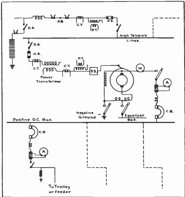
Fig. 4. Single line diagram of a synchronous converter substation, showing main step-down transformer, converter, and auxiliary equipment.
