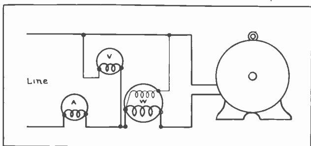
Fig. 1. This sketch shows the method of connecting the meters to measure voltage, current, and power of a single-phase motor.
