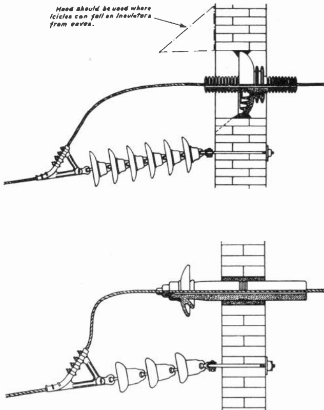
Fig. 26. The above diagrams show methods of using strain insulators to attach line conductors to the walls of substation buildings and keep the strain from the conductor where it enters the building through wall type insulator bushings. Courtesy Ohio Brass Company.
