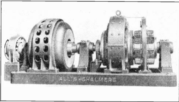
Fig. 7. 1000-kw. motor-generator set with an A. C. synchronous motor and exciter on the left, and the D. C. generator on the right. Courtesy of Allis-Chalmers Mfg. Co.
