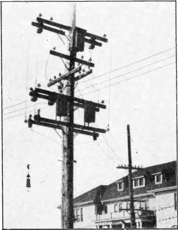
Fig. 3. Group of transformers mounted on heavy cross arms on an extra heavy pole.
