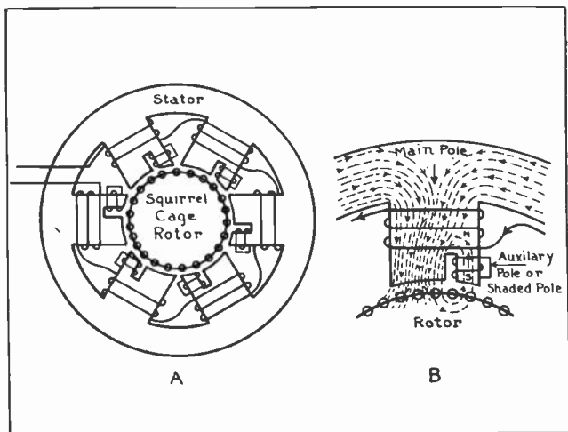
Fig. 16. The above two sketches show the construction and illustrate the principles of the shaded-pole type induction motor.
