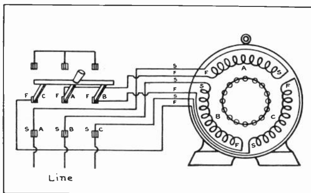
Fig. 19. This diagram shows the method of using a three-pole, double-throw switch for star-delta starting of squirrel-cage induction motors.
