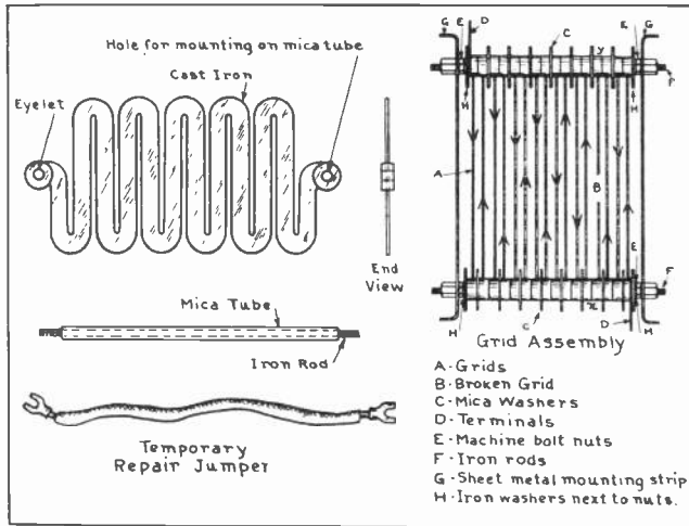
Fig. 12. Sketches showing construction of iron grid type secondary resistors for slip-ring motors. Also note the jumper used for making temporary repairs to open circuited units.
