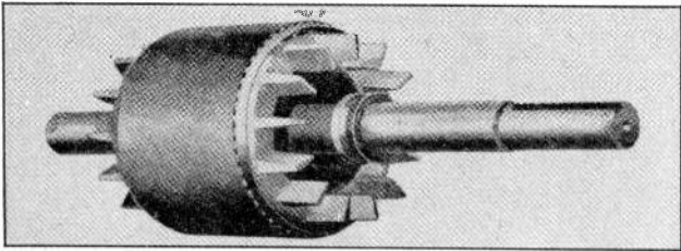
Fig. 13. Complete rotor of the double squirrel-cage type. Note that there are no open slots around the rotor core, the bars being cast into the rotor.
