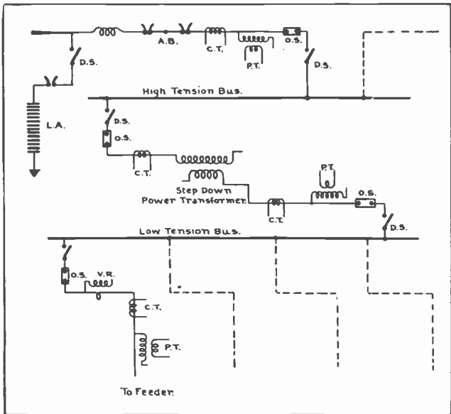
Fig. 1. Single line diagram of a distribution substation with one main power transformer for reducing the voltage from the transmission line. Trace this diagram carefully and familiarize yourself with each part from the explanations given on these pages.
