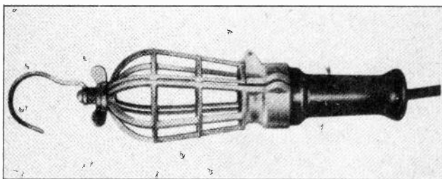
Fig. 11. Convenient trouble lamp with hook, guard, and insulating handle.
