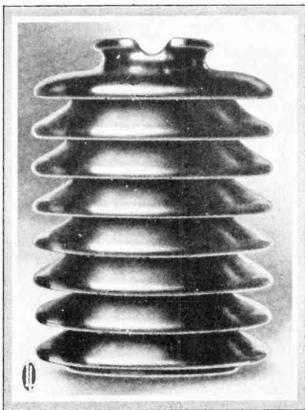
Fig. 19. Large special fog type pin insulator having a number of extra skirts to prevent flashover in districts subject to heavy salt fogs, mist, dirt, etc. Courtesy Lapp Insulator Company, Inc.
