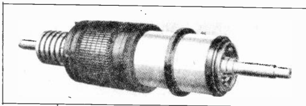
Fig. 4. Photo of converter armature clearly showing the armature winding, slip rings and commutator. A.C. enters at the slip rings and D. C. is taken off from the commutator when this armature is revolved at synchronous speed in the flux of D. C. field poles. Courtesy Allis-Chalmers Mfg. Co.)
