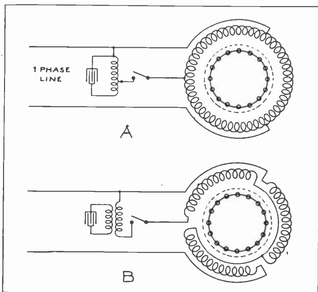
Fig. 14. The above two diagrams show the connections for two different types of single-phase, split-phase motors which use condensers and transformers to obtain the split-phase currents for their stator windings.
