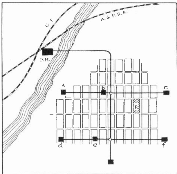
Fig. 2. This diagram shows how a power plant should be located near a convenient source of fuel supply and condenser water. Transmission and distribution lines then carry the energy from the power plant to the substations and consumers.
