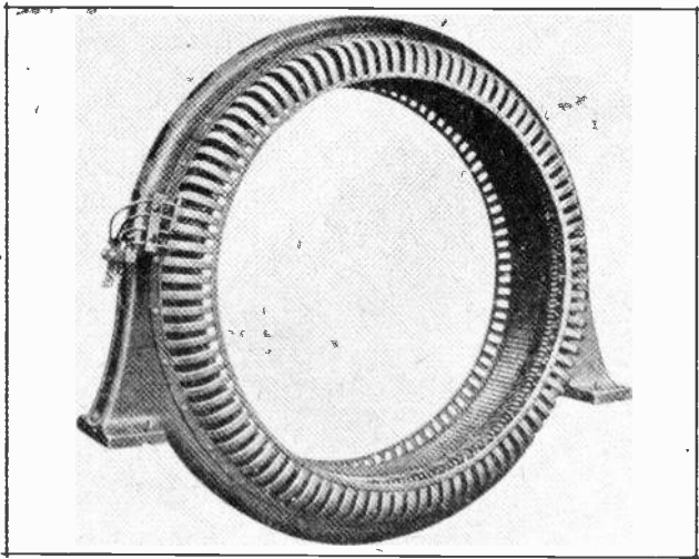
Fig. 2. Above is shown the stator of a large synchronous motor. You will note that the stator, frame, core, and windings are the same as those used for alternators.
