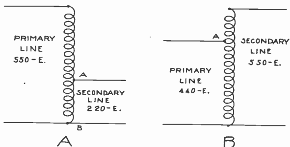
Fig. 3. A shows a step-down auto transformer. Note the reduction obtained in the voltage between the primary and secondary lines. B shows a step-up auto transformer to increase the secondary voltage.
