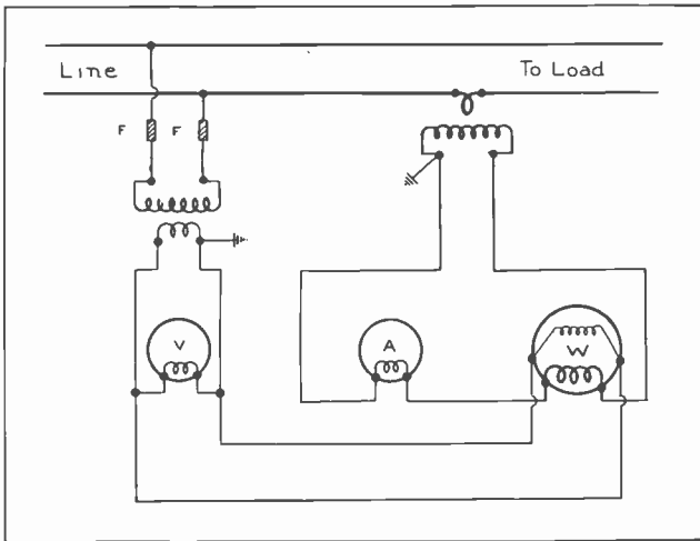
Fig. 2. When meters are used to measure the energy of high voltage lines instrument transformers are used to reduce the voltage and current to the meters.
