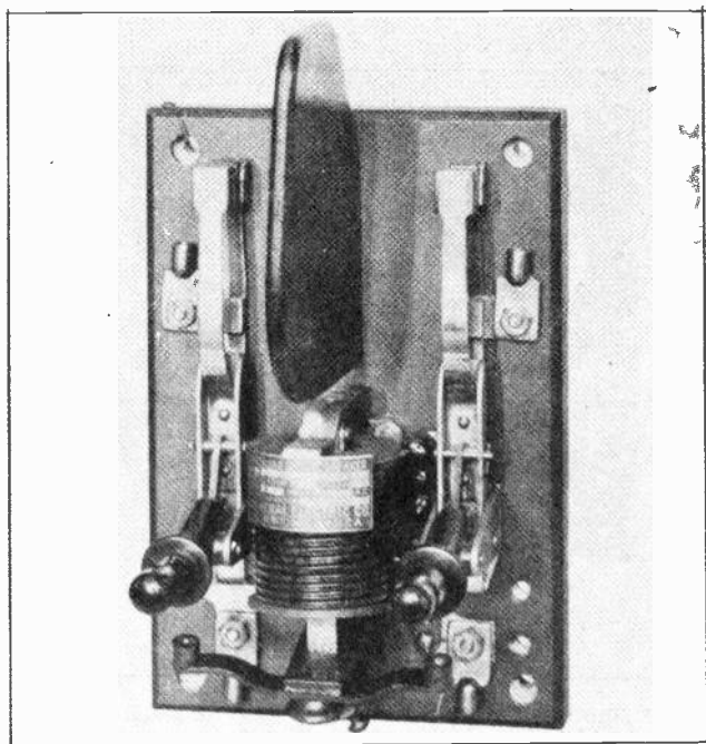
Fig. 6. Small air circuit-breaker for use on circuits of 600-volts and loads up to 100 amperes. Note the flash barrier placed between the two poles of the breaker. Courtesy of G. E. Company.
