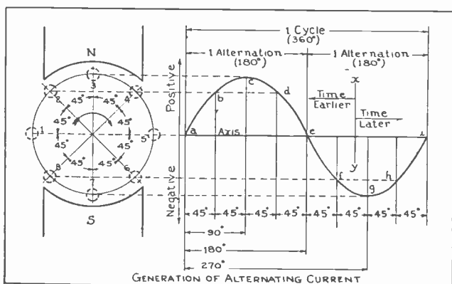
Fig. 6. The above diagram illustrates the manner in which alternating voltage is produced in a simple two-pole generator. The sine curve shows the variations and reversal of voltage for one revolution of the armature. Study this diagram very carefully with the accompanying explanation.
