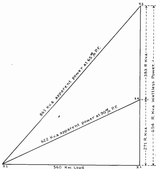
Fig. 10. This diagram also shows the reduction obtained in the apparent power and wattless power by improving the power factor of a system. By carefully measuring the top section of the vertical line in the diagram we can find the size of the condenser required to correct the power factor.
