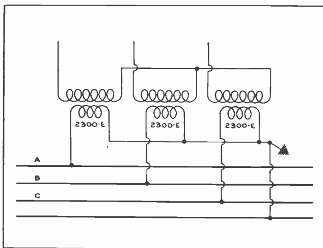
Fig. 17. Connections for three-phase, four-wire service from the star-connected secondaries of a three-phase bank of transformers.
