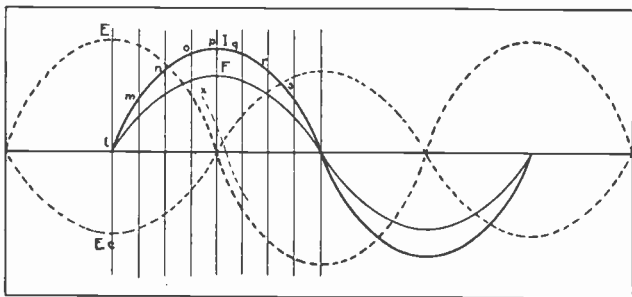
Fig. 5. Curves for a single-phase circuit in which the current and voltage are approximately 90^\circ out of phase with each other, due to inductance in the circuit.
