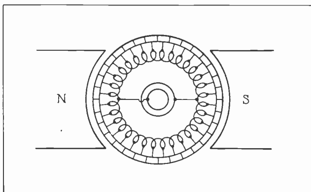
Fig. 5. Diagram of the armature connections for a simple two-pole, single-phase, synchronous converter. Note that the slip ring connections are taken at points 180 electrical degrees apart on the winding.
