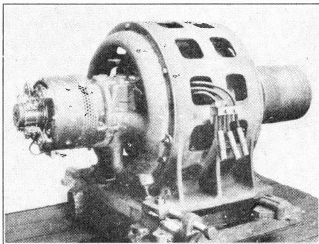
Fig. 2. This photo shows a 125 kv-a. alternator of the horizontal belt-driven type. Note the D. C. exciter-generator which is direct connected to the left end of the shaft. (Photo Courtesy Allis Chalmers Mfg. Co.)
