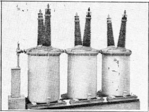
Fig. 7. Large outdoor oil switch for use in three-phase, 150,000-volt circuits. Courtesy of Condit Electric Mfg. Co.
