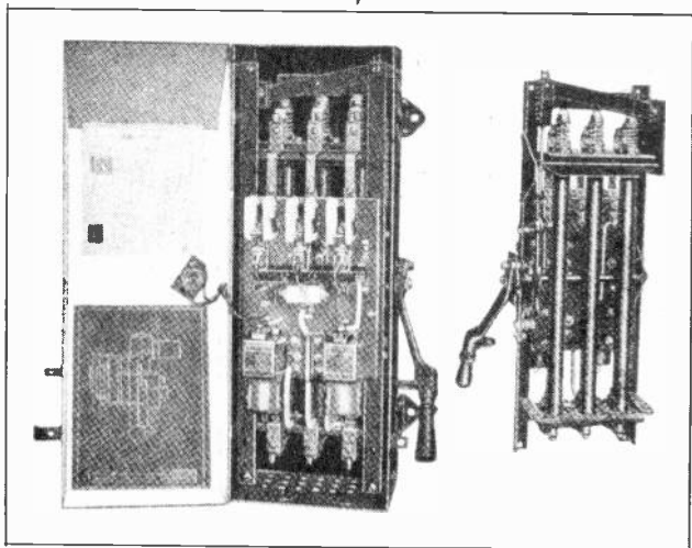
Fig. 12. On the left is shown a complete three-phase resistance starter of the carbon pile type for A. C. motors. On the right is shown the starter mechanism and tubes of carbon disks removed from the cabinet for a rear view. (Photo courtesy of Allen Bradley Co.)
