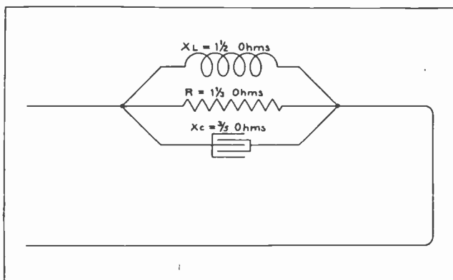
Fig. 13. This sketch shows inductance, resistance, and capacity connected in parallel. The method of determining the impedance of such a circuit is thoroughly explained in this lesson.
