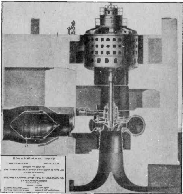
Fig. 11. Excellent sectional view of a large hydro-electric generator unit. Note the casing and runner of the water wheel and also the draft tube through which the water discharges to the tail race. The valve controlling the water flow through the wheel or turbine is shown on the left. The main part of the generator is set down in the concrete so that just the top of the unit and its exciter project above the operating floor. Courtesy Wm. Crampton & Sons Co.
