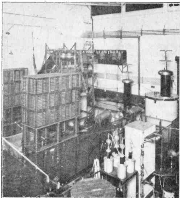
Fig. 16. The above photo shows a high voltage test room at the plant of the General Electric Company. Transformers in this room are capable of producing over one million volts and an enormous arc produced by this voltage can be seen above the sphere gap and condenser slightly to the left of the center of the picture.
