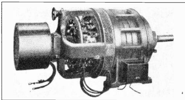
Fig. 17. This photo shows the completely assembled BTA motor. The brush-shifting wheel can be seen on the upper corner of the frame and the slip-rings are enclosed in the housing at the left end of the shaft. (Courtesy G. E. Company.)
