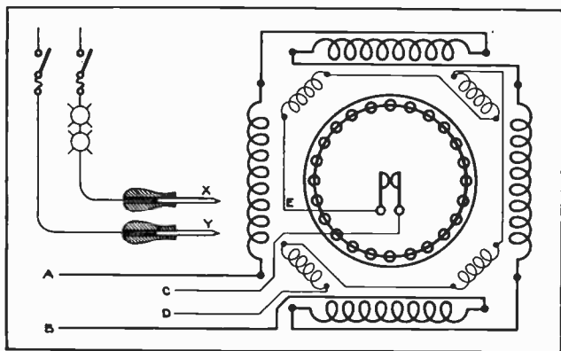
Fig. 5. Diagram illustrating connections and methods for convenient trouble tests on single-phase split-phase A. C. motors.
