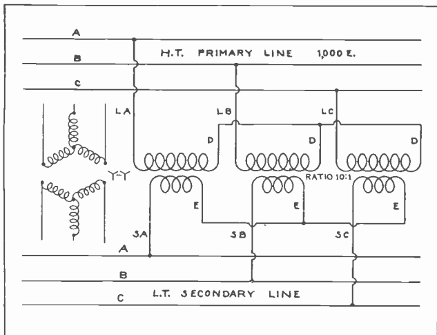
Fig. 8. Connection diagram for a bank of three transformers connected star-star.
