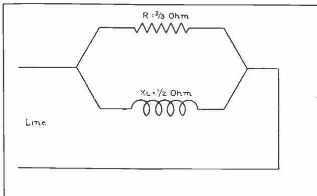
Fig. 11. Resistance and inductance in parallel. The impedance for this circuit can be determined by the formulas given on this page.
