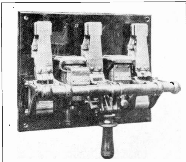
Fig. 7. Three-pole, 500-ampere, 250-volt A. C. air-breaker. Note the intermediate and arcing contacts and also the series overload trip coils. Courtesy of G. E. Company.
