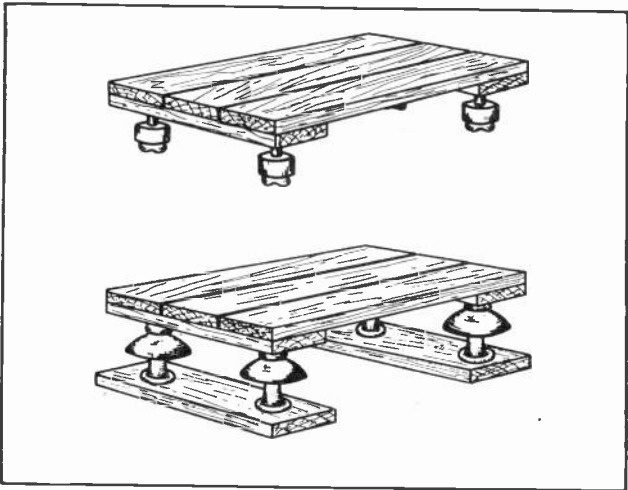
Fig. 9. The above sketch show two types of insulated stools or platforms for safety in working around live wires. These are very simple and inexpensive to make.
