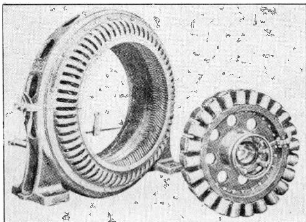
Fig. 1. Above are shown the complete stator of an A. C. generator on the left and the revolving field or rotor on the right. The field coils on the rotor are excited with direct current and revolved within the stator to generate alternating current in its windings.
