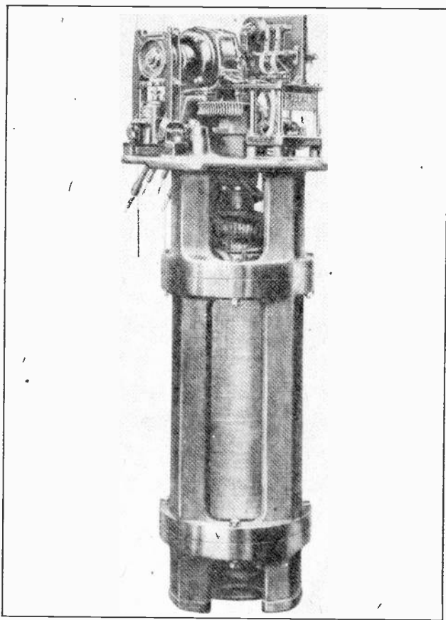
Fig. 8. Complete stator and rotor of a single-phase voltage regulator with the operating motor attached. (Photo Courtesy General Electric Co.)
