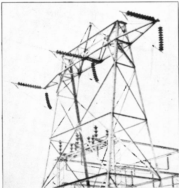
Fig. 25. This photo shows a heavy strain tower with strain insulators supporting the tension of the conductor span, suspension insulators supporting the conductor loops which run down to a substation, and pedestal type insulators in the background supporting high-voltage air break switches. Courtesy Ohio Brass Co.
