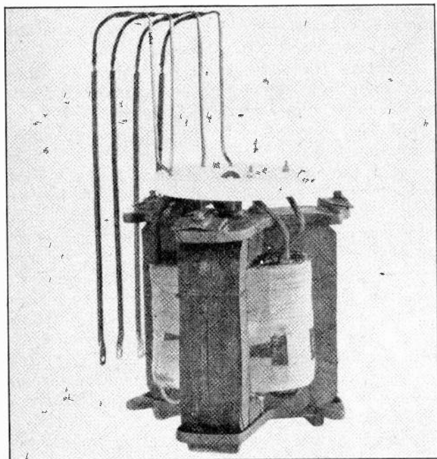
Fig. 5. Complete transformer core and windings. Note how the legs of the core are assembled to form complete magnetic paths around the coils. (Photo courtesy General Electric Co.)
