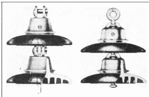
Fig. 21. Suspension insulators which can be fastened together in long strings to insulate high-voltage conductors. Note the two different types of fasteners used for attaching these insulators together. Courtesy of Ohio Brass Co.
