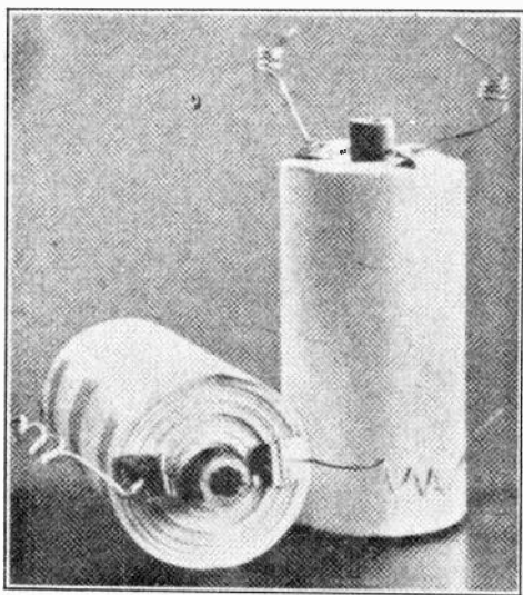
Fig. 4. Roll-type condenser units in which the long strips of metal foil and insulating paper are rolled into one compact condenser element. (Courtesy Electric Machinery Mfg. Co.)
