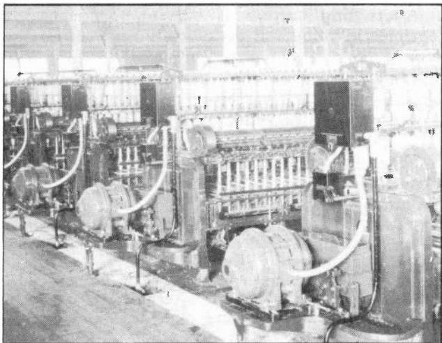
Fig. 4. This view shows a number of A. C. motors being used for individual drive on machines in a textile mill. Thousand of factories and industrial plants use electric motors in this manner for driving their various machines and equipment. (Photo courtesy G. E. Company)
