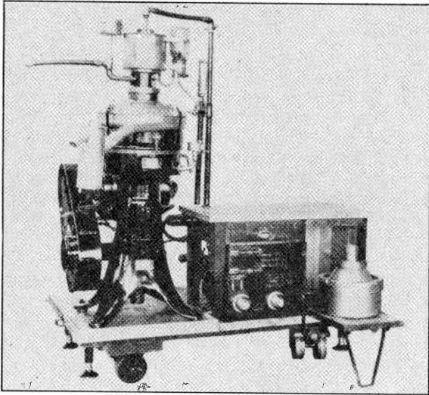
Fig. 11. Motor-operated centrifugal oil purifier which separates water and dirt from the oil by revolving them at high speeds. (Photo Courtesy General Electric Co.)
