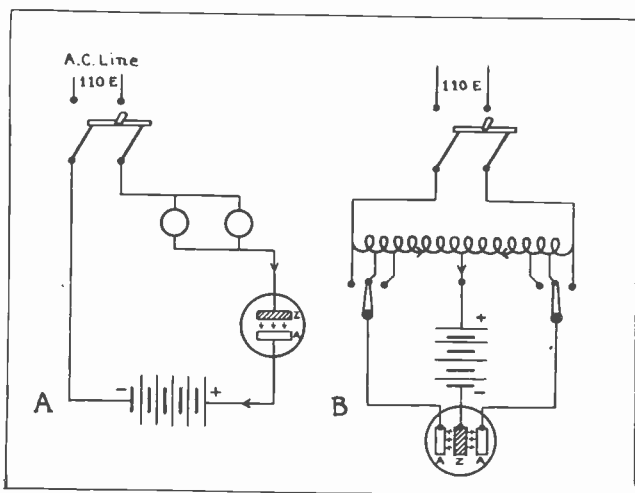
Fig. 2. A shows a half-wave, electrolytic rectifier and B shows an electrolytic rectifier of the full-wave type. Current can only pass through these devices in one direction.
