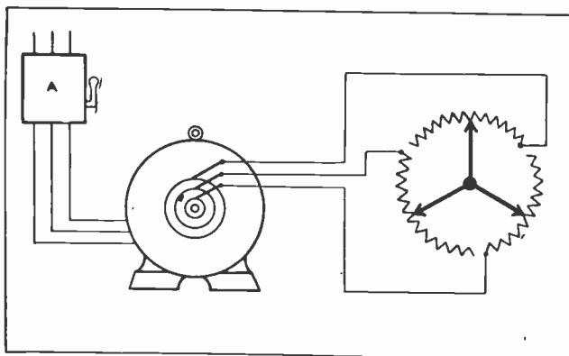
Fig. 10. Diagram showing the connections of a resistance starter in the secondary or rotor circuit of a slip-ring motor. The line switch at "A" is used to energize the stator circuit.
