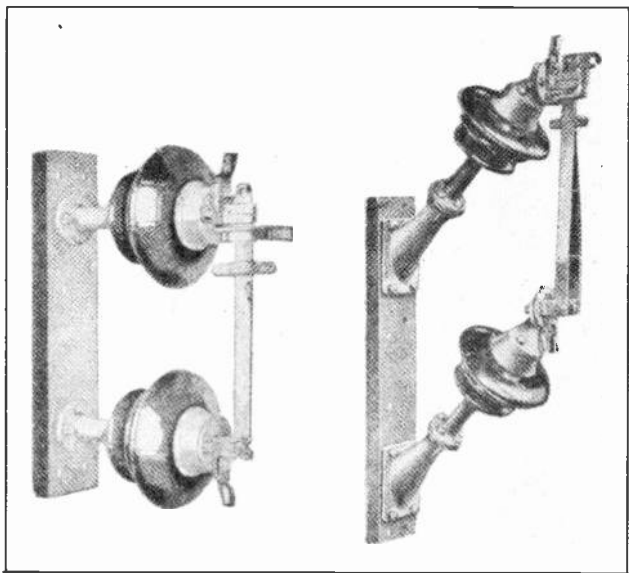
Fig. 10. Two types of disconnect switches for operation by means of a switch hook or pole having an insulated handle.
