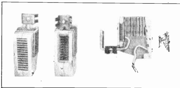
Fig. 10. This photo shows several views of Deion arc quenchers. The sectional view on the right shows the manner in which these devices are placed over the contacts, to quickly extinguish the arc when it passes up into the metal blades. (Courtesy Westinghouse Elec. & Mfg. Co.)
