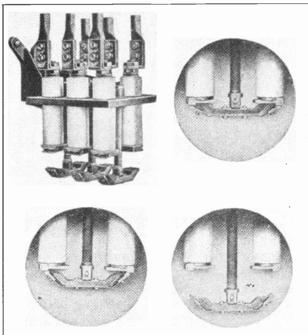
Fig. 4. At the upper left is shown the mechanism of a different type oil switch, and in the three other views are shown the steps or movement of the contacts during the opening of a switch of this type.
