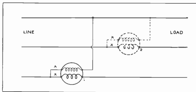
Fig. 9. The above diagram shows the manner of connecting one wattmeter in two different phases of a three-phase system in order to measure the total power.
