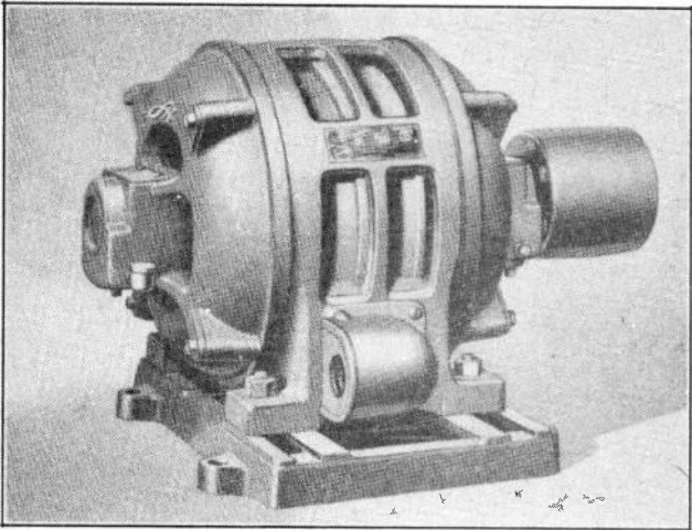
Fig. 1. This photo shows a modern polyphase induction motor. The three phase leads from the line are connected to the stator leads in the connector box shown on the side of the frame.
