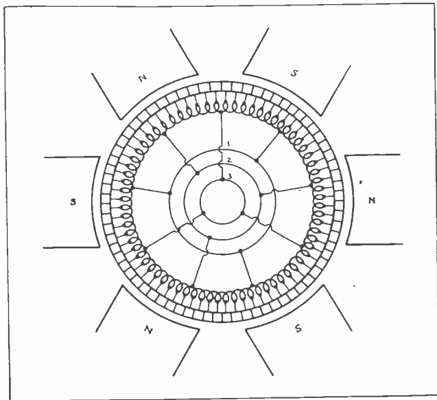
Fig. 6. Diagram of armature connections for a six-pole, three-phase, synchronous converter. The slip ring connections for each phase are taken at points 120 electrical degrees apart.
