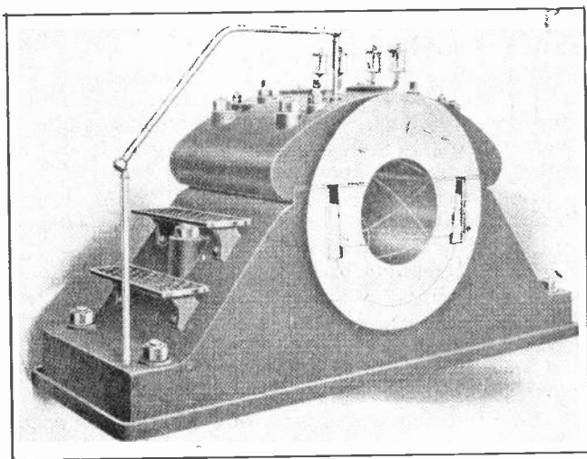
Fig. 7. Very large special sleeve bearing for use with steam engines. Note the adjustable sections in the sides of the bearing to prevent pounding due to bearing slack and engine thrust.
