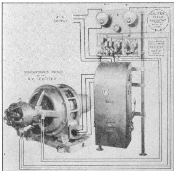
Fig. 12. This photo-diagram shows the arrangement of the connections between a synchronous motor and its exciter, and the controller and instruments used with it. On an actual installation these wires would, of course, be run in conduit or B.X. The three-phase line circuit through the compensator to the stator of the synchronous motor is shown by the heavy lines. The exciter and field circuits are shown by the lighter lines. (Courtesy General Electric Co.)
