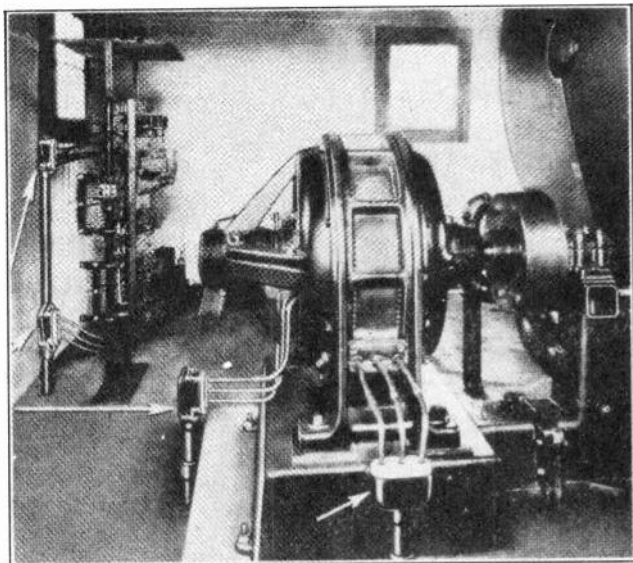
Fig. 1. This photo shows a very neat installation of the wiring to a slip ring motor and its controller. Courtesy of Crouse Hinds Co.
