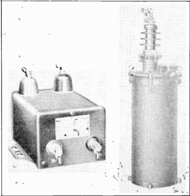
Fig. 5. At the left is shown a small potential transformer with the high-voltage terminals on the top and the low-voltage terminals on the end. Note the polarity markings on the case. On the right is shown a large oil-insulated power-type current transformer.
