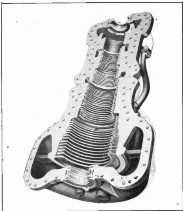
Fig. 14. One-half of a steam turbine casing showing a series of stationary blades between which the movable blades or buckets revolve. Courtesy of Allis-Chalmers Mfg. Co.
