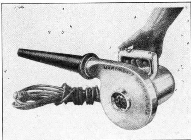
Fig. 26. Convenient portable electric blowers of the type shown above are often used for cleaning dust from electrical machines.
