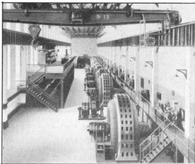
Fig. 18. Interior view of one of the power plants at Niagara Falls showing horizontal type water-wheel-driven alternators manufactured by Allis-Chalmers Mfg. Co. Also note the operating gallery and switchboard on the elevated platform at the left.
