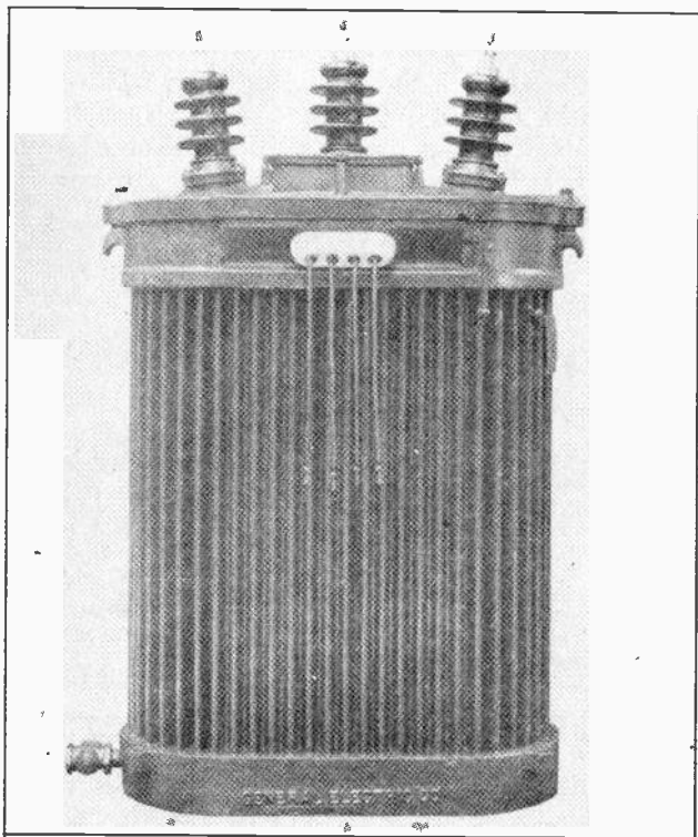
Fig. 9. Three-phase power transformer for high voltage operation. Note the large insulating bushings and also note the manner in which the entire tank is corrugated to provide a greater heat-radiating surface.
