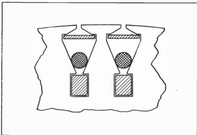
Fig. 14. This sketch shows the slot and bar construction of double squirrel-cage rotors using iron "choker bars" to change the resistance of the field and outer circuits.
