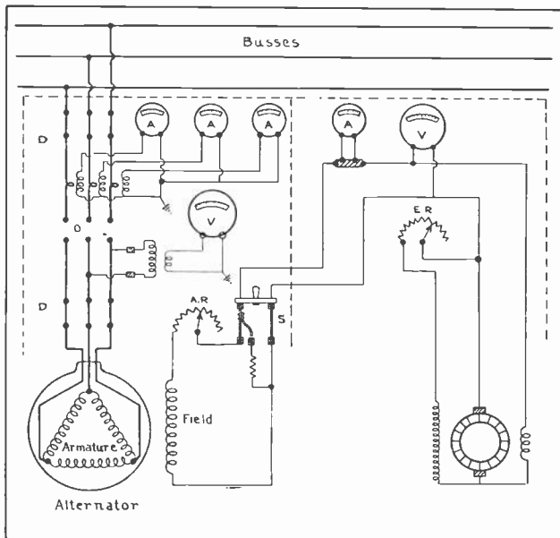
Fig. 6. This diagram shows the wiring and arrangement of a three-phase alternator, and the meters and equipment commonly used on the switchboard panels.
