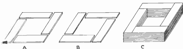
Fig. 12. A core type transformer core may be constructed with alternate layers of laminations as shown above.
