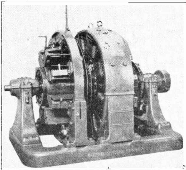
Fig. 2. D. C. end of a large synchronous converter showing brush-lifting mechanism, and flash barriers around the brushes. (Courtesy General Electric Co.)
