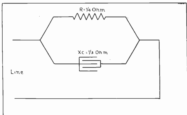
Fig. 12. Resistance and capacity in parallel in the A. C. circuit. Practice using the formulas given on these pages for determining the impedance of such circuits
