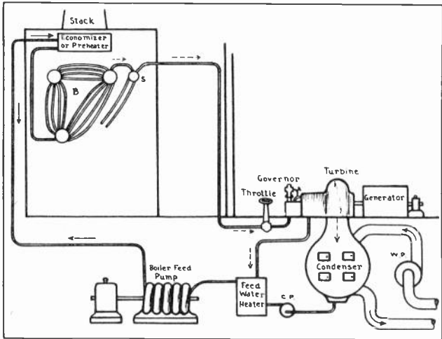
Fig. 9. This simple diagram illustrates the steam cycle or method of recirculating the boiler feed water in a modern power plant.
