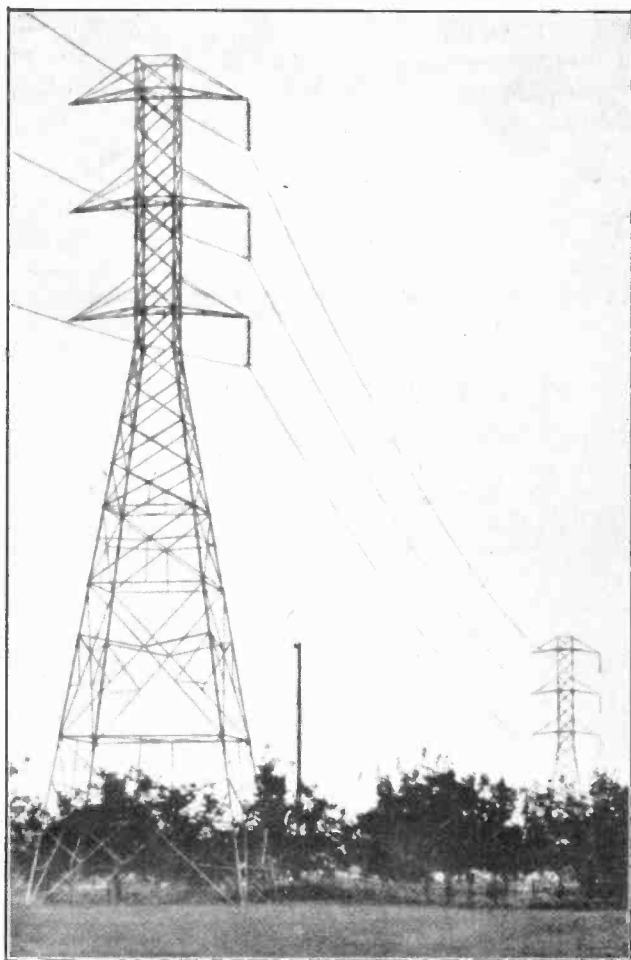
Fig. 23. 220-kv. line on which each conductor is supported by a string of 14 suspension insulator units. Note the arrangement of the three conductors on one side of the towers allowing space for another three-phase line to be put on the opposite side of the towers in the future.
