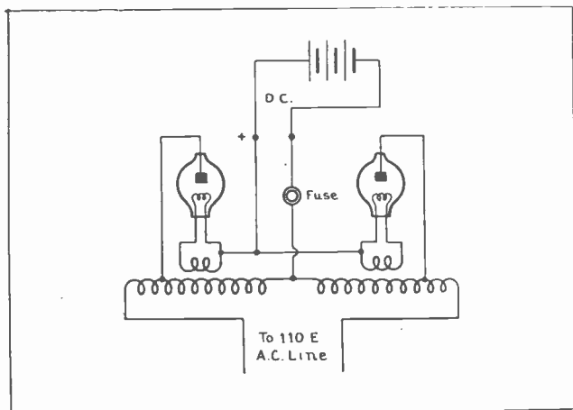
Fig. 9. This diagram shows the circuit of a full-wave Rectigon charger of the type made by Westinghouse Electric & Manufacturing Company. By carefully tracing this circuit you can get a very good idea of the principle of its operation.
