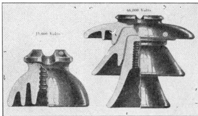
Fig. 13. The above photo clearly shows the shape and construction of both small and large pin type insulators of the type used on high-voltage lines. Courtesy of Ohio Brass Co.
