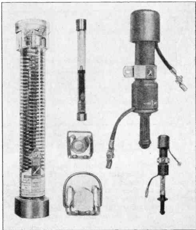
Fig. 19. The above views show high-voltage fuses of the liquid filled type both in normal and open condition, and also shows clips for mounting them. On the right are fuses of this type in waterproof housings for outdoor use. Courtesy of Schweitzer & Conrad, Inc.
