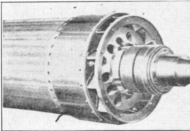
Fig. 13. End-view of high speed field rotor showing shield ring over the coil ends and also showing ventilating blades and slip rings.
