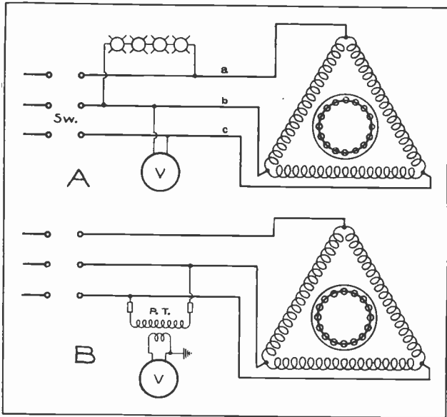
Fig. 1. The above sketches show connections for voltage tests on leads of three-phase squirrel cage motors.
