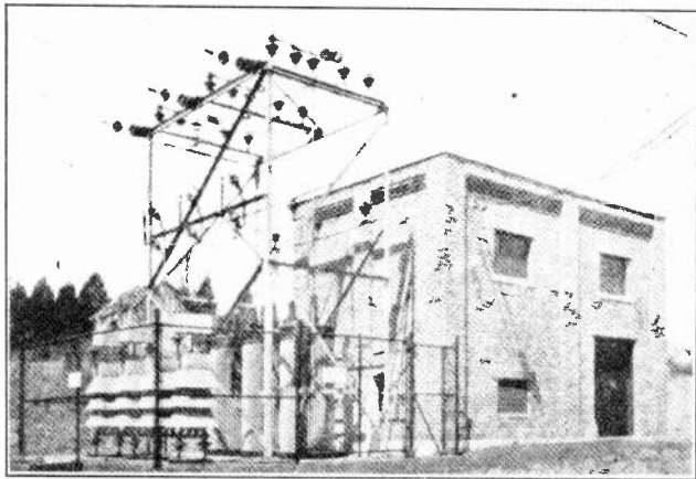
Fig. 13. Exterior view of a modern substation showing incoming line, choke coils, fuses, disconnects, lightning arresters, and power transformers outside of the building. The synchronous converters are located inside of the building.
