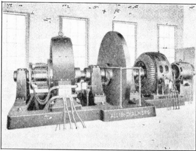
Fig. 8. Motor-generator set with large flywheel for carrying heavy momentary overloads in steel mill work and other classes of severe service. Courtesy of Allis-Chalmers Mfg. Co.
