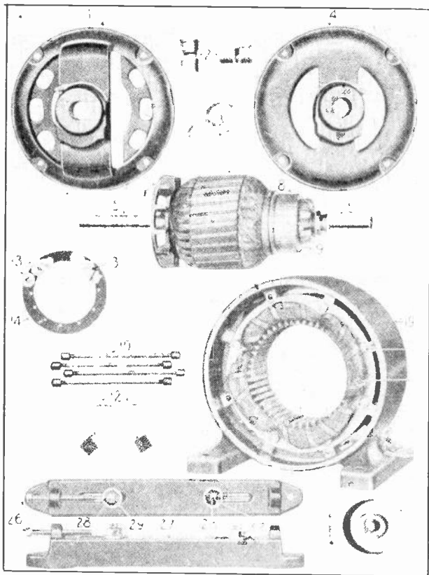
Fig. 19. Disassembled view showing important parts of an A. C. single-phase repulsion motor.
