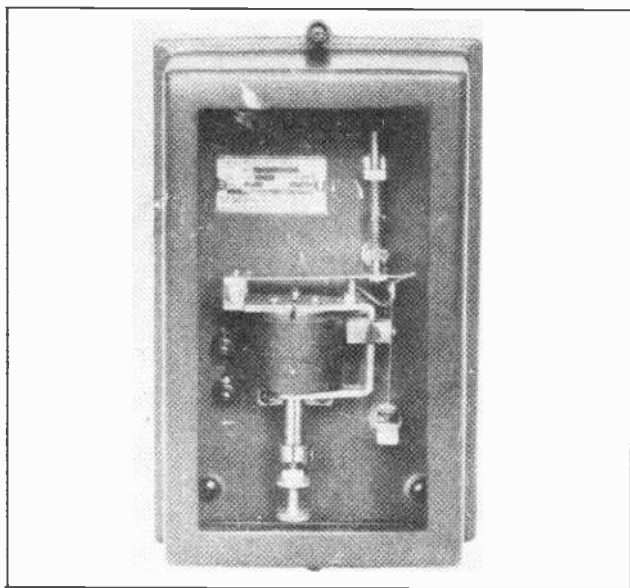
Fig. 21. Photo of a high-voltage cutout relay clearly showing the coil and contacts. Courtesy of G. E. Company.
