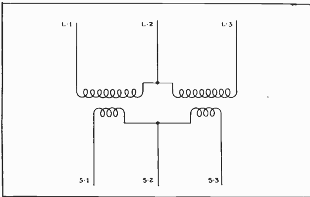
Fig. 13. Connections for using two single-phase transformers to provide three-phase service by what is called the "open-delta" connection.
