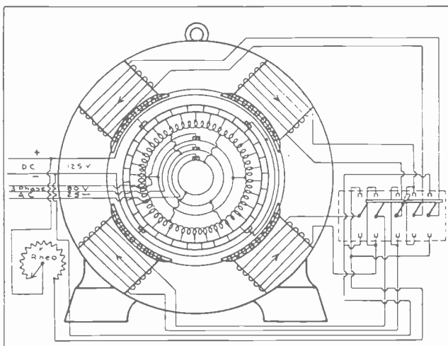
Fig. 11. Wiring diagram showing armature and field connections, and also the field break-up switch and rheostat for a four-pole, three-phase converter. Trace out the field circuit both with the switch in the upper and lower positions and note that the polarity reverses when the switch is changed.
