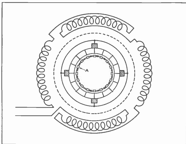
Fig. 20. This diagram shows the connections and arrangement of the short-circuiting device of a repulsion-induction motor. The short-circuiting mechanism at "A" lays around the inside of the commutator bars and short-circuits them all together when the machine comes up to speed.
