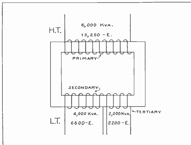
Fig. 20. Diagram of a transformer which is equipped with three windings. The high tension winding in this case is the primary, and the low tension winding is divided into two sections, called the secondary and tertiary windings.
