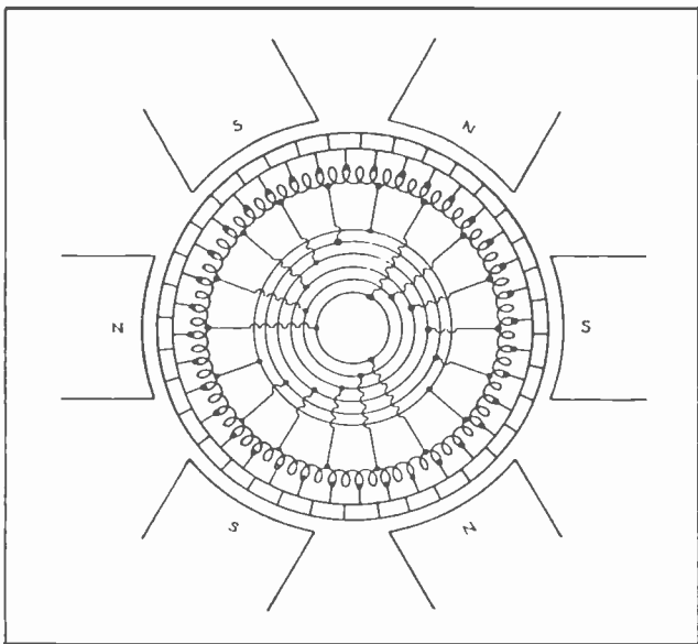
Fig. 7. Diagram showing the armature connections for a six-pole, six-phase, synchronous converter. The connections of the different phases of this winding are made 60 electrical degrees apart.
