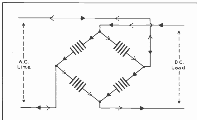
Fig. 12. Connection diagram of a full-wave, copper oxide rectifier with four units connected in a "bridge" type circuit.
