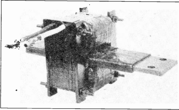
Fig. 3. Bus-bar type current transformer for use with large bus bars on switchboards. (Photo Courtesy General Electric Co.)
