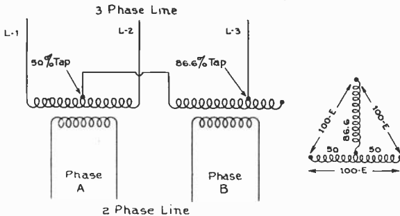
Fig. 2. The Scott transformer connection shown above is often used to change three-phase energy to two-phase or vice versa.
