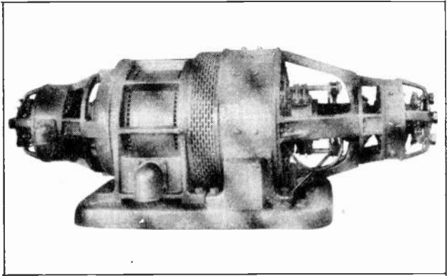
Fig. 9. Compact type of motor-generator set used for operating D. C. elevator motors. Courtesy of G. E. Company.
