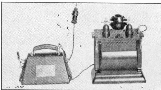
Fig. 9. Portable oil testing outfit consisting of high voltage transformer oil test cup and voltage adjuster. (Photo Courtesy General Electric Co.)
