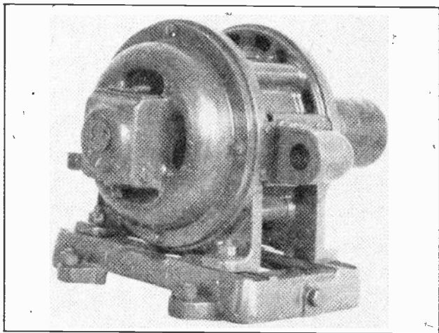
Fig. 4 Common type of 5-h. p. A. C. induction motor. Motors of this type are used by the thousands in factories and industrial plants throughout the country. (Photo courtesy General Elec. Co.)
