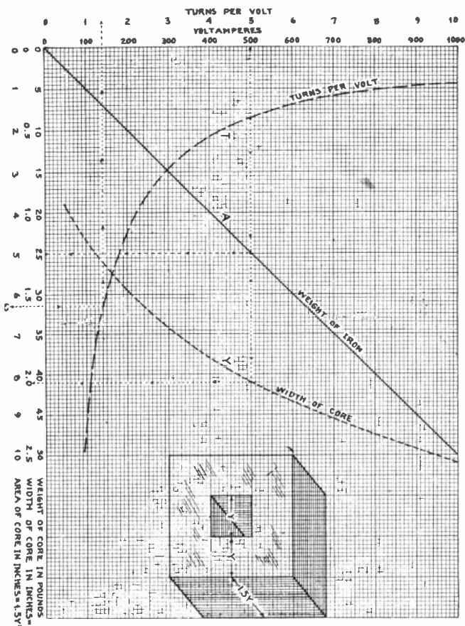
Fig. 10. Transformer design chart.
