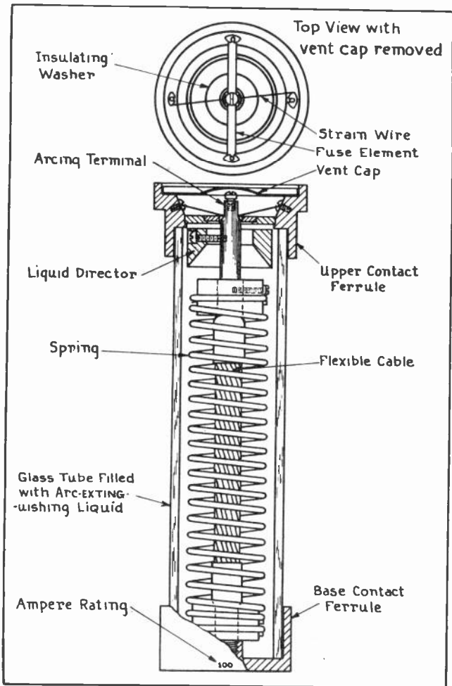
Fig. 18. The above sketch shows the principal parts of a high-voltage fuse of the liquid filled type. Examine each part carefully and compare with the explanations given on these pages. Courtesy of Schweitzer & Conrad, Inc.
