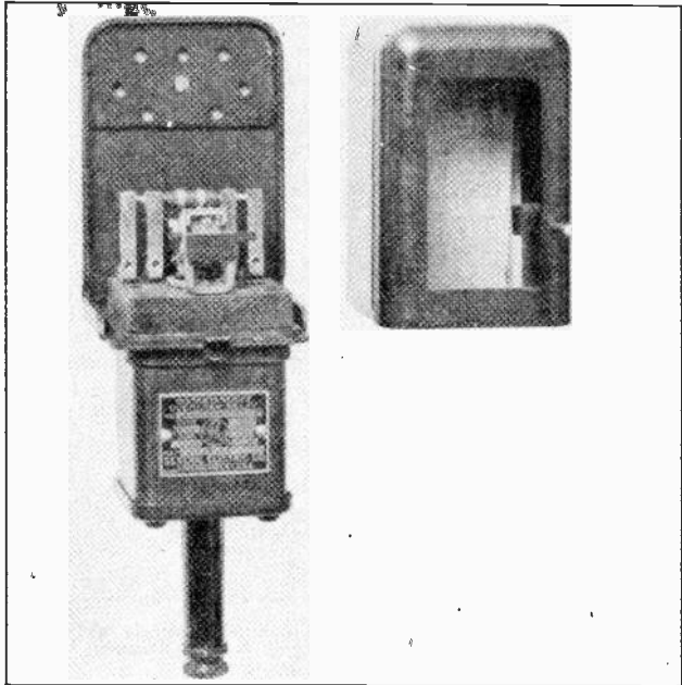
Fig. 22. This view shows an instantaneous operating overcurrent relay with contacts for closing three circuits. Courtesy of G. E. Company.
