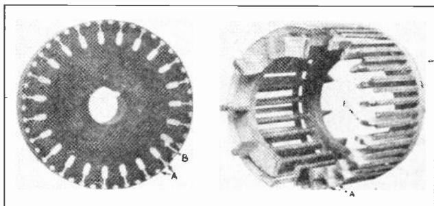
Fig. 12. This figure shows two views of a double squirrel-cage rotor. On the left is a sectional view and on the right the core iron has been eaten out by acid, clearly showing the construction and shape of the double squirrel-cage. (Photo courtesy General Electric Co.)
