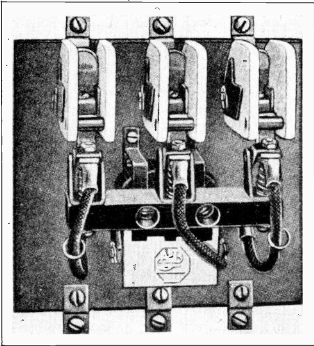
Fig. 1. Contactor mechanism of a magnetically operated across-the-line starter for A. C. motors. (Courtesy Allen Bradley Co.)
