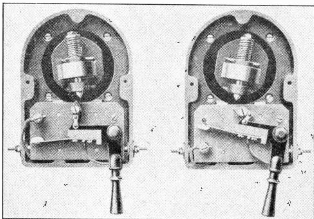
Fig. 13. Two views of a centrifugal overspeed switch showing two possible arrangements of the contact for either an open or closed circuit system.
