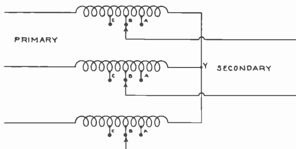
Fig. 5. Three-phase auto transformer in which each winding has several taps so that the secondary voltage can be varied.
