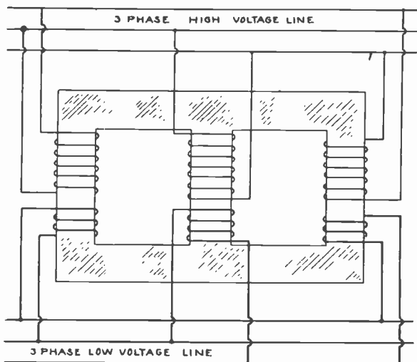
Fig. 7. The above sketch shows the primary and secondary windings of a three-phase transformer. Both primary and secondary are connected delta to the line wires.
