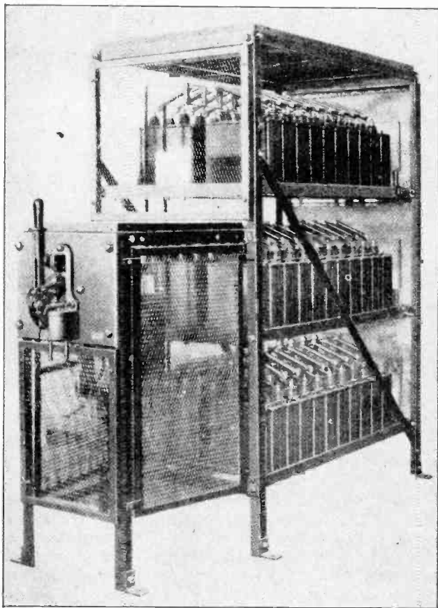
Fig. 2. 300-kv-a., three-phase, 2500-volt, capacitor or static condenser, used for improving power factor. (Courtesy General Electric Co.)
