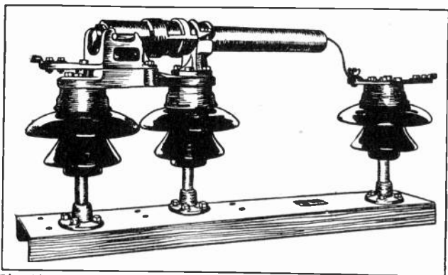
Fig. 16. Expulsion type high-voltage fuse. The fuse strip is violently blown out of the tube or barrel, thus quickly interrupting the circuit when this fuse blows. Courtesy of Hi-Voltage Equipment Co.
