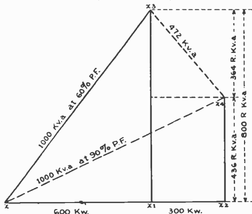
Fig. 11. This diagram shows the graphic solution of a problem in which the synchronous motor is used for mechanical power purposes as well as power factor correction. The figure should be easily understood by referring to the explanations in the accompanying paragraphs.
