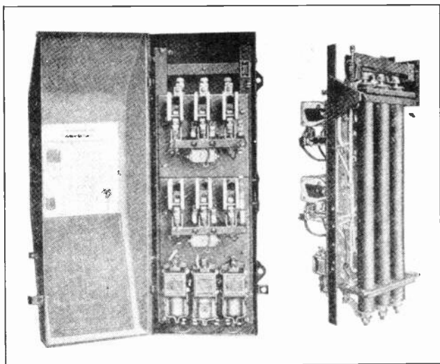
Fig. 14. Front and rear views of an automatic, three-phase, carbon pile starter. The magnetically operated contactors cut the resistance out of the motor circuit as it comes up to speed. (Courtesy Allen Bradley Co.)
