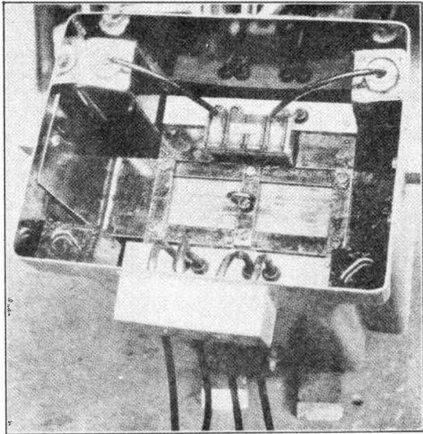
Fig. 8. This photo shows the inside of a small distribution transformer with the oil removed. Many transformers of this type are provided with a terminal block mounted on the core inside of the tank so that the connections can be changed to obtain different voltages.
