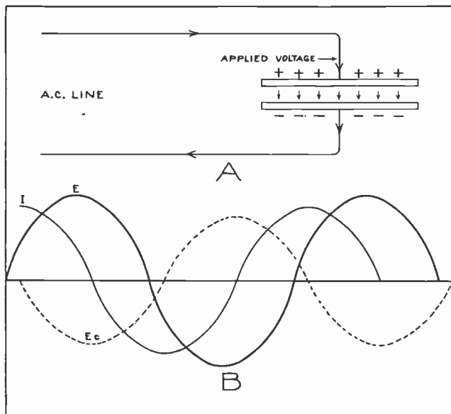
Fig. 6. This diagram shows the current leading the voltage by nearly 90^\circ , due to capacity or condenser effect in the circuit.
