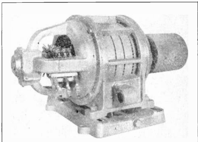
Fig. 12. This photo shows a complete slip-ring motor to which variable resistance can be connected for starting and speed-regulating duty. Note the slip rings and rotor connections on the left-hand end of the machine. (Photo courtesy General Electric Co.)
