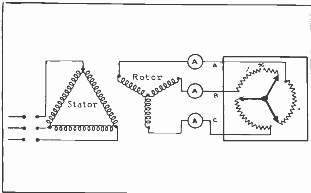
Fig. 14. Diagram showing methods of testing with ammeters to locate an open circuit in a secondary resistance.
