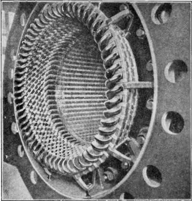
Fig. 8. This photo shows the end of a stator winding for a high speed turbo-alternator. Note the rigid bracing of the coil ends.
