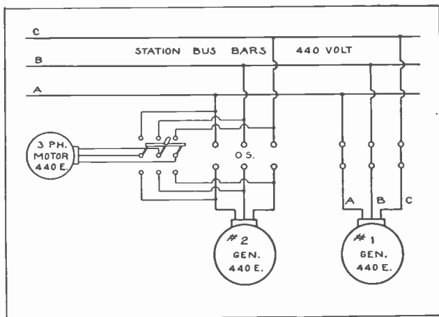
Fig. 2. The above sketch shows the connections and illustrates the method for phasing out an alternator by means of a three-phase motor.
