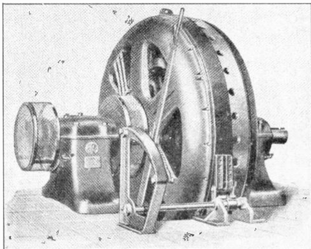
Fig. 9. Super-synchronous motor which is equipped with a revolvable stator and brake to obtain high starting torque. (Photo courtesy G. E. Company.)
