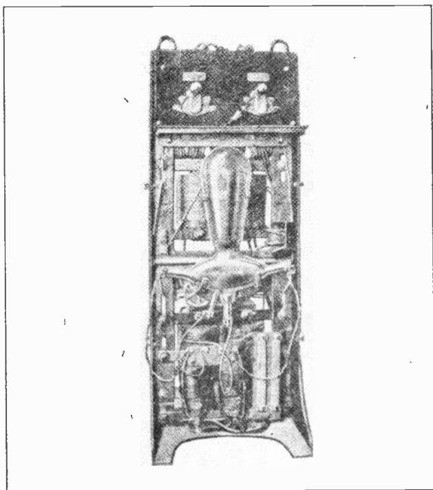
Fig. 3. Rear view of a complete mercury arc rectifier showing the bulb and also the auto transformers, resistors, tap adjusters, etc.
