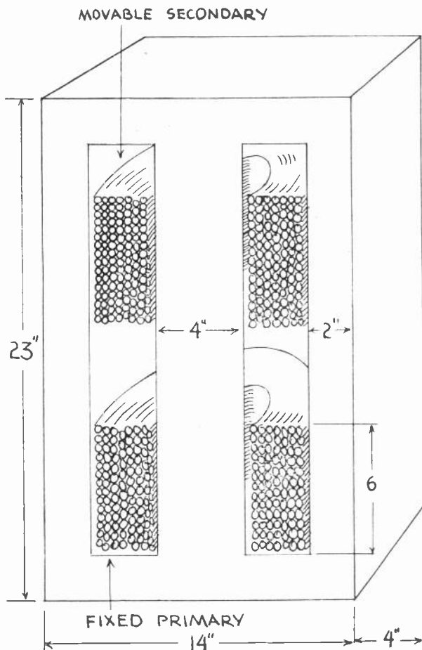
Fig. 14. A 19 Kv-a. welding transformer designed for operation on a 220 volt line.
