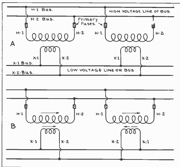
Fig. 3. A shows two single-phase transformers with like polarities connected in parallel. B shows the proper method of connecting two single-phase transformers in parallel when the polarity of one is subtractive and the other is additive. Note the polarity markings in each case.
