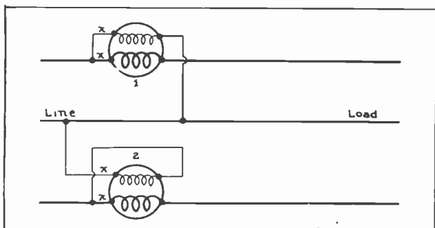
Fig. 7. This diagram shows the connections to the lower wattmeter reversed to obtain proper readings on circuits with low power factor.
