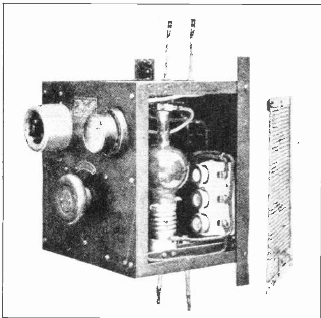
Fig. 8. The above photo shows a side-view of a Tungar rectifier with the bulb in place in the socket and the tap adjusting knob on the front panel. (Courtesy General Electric Company).
