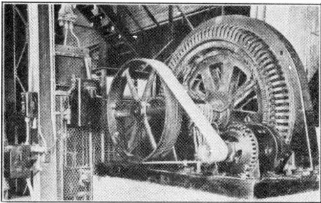
Fig. 5. 150-h. p., 2300-volt, low-speed, synchronous motor and exciter. The speed of the large motor is 144 R.P.M. (Photo courtesy Allis-Chalmers Mfg. Co.)
