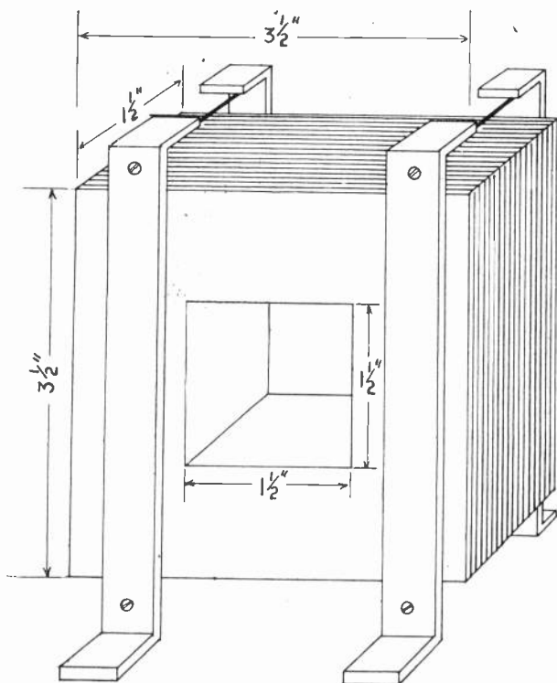
Fig. 13. A 50 w. transformer core constructed from strips 1'' \times 2\frac{1}{2}'' . Note the method of binding the strips together.
