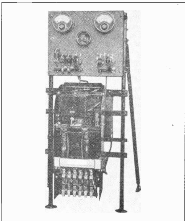
Fig. 2. This photo shows another view of a compensator with both the front cover and the oil tank removed. The contacts which operate under oil can be seen at the bottom of the controller. (Courtesy General Electric Co.)
