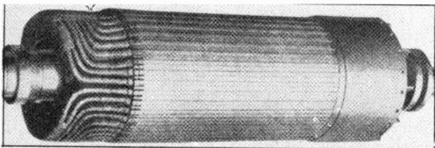
Fig. 12. This photo gives an excellent view of a high speed field rotor such as commonly used in turbine-driven alternators. Note how the field coils are placed in slots in the solid rotor so that when they are excited with D. C. they will create two field poles on opposite sides of the rotor. (Photo Courtesy Allis Chalmers Mfg. Co.)
