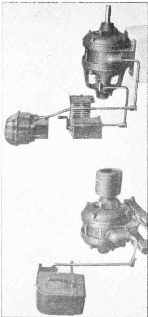
Fig. 20. The above two views show methods of connecting compensators and drum controllers to induction motors by means of rigid and flexible conduit. While in some temporary installations open wires which are properly supported and protected may do very well, in general a neat, permanent installation of the wires in conduits is a much safer and better arrangement.
