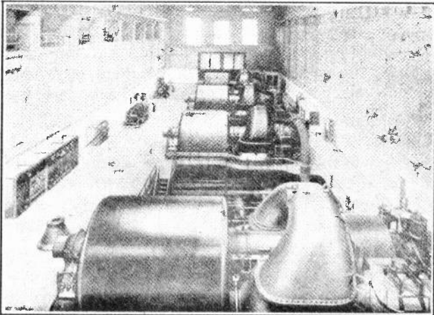
Fig. 7. Interior view of a large power plant showing several of the steam-turbine-driven alternators and also part of the switchboard and the exciter-generators.
