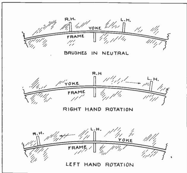
Fig. 4. The above sketches show markings on motor frame and brush yoke, for setting repulsion motor brushes for right or left-hand rotation.
