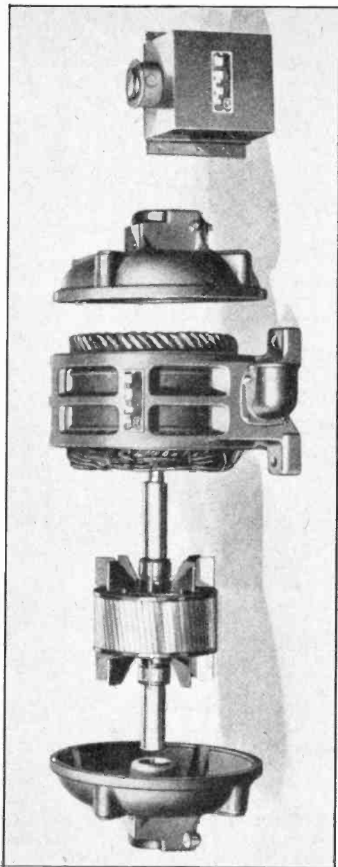
Fig. 15. This photo shows an excellent disassembled view of a squirrel-cage induction motor for single-phase operation and also the condenser by which it obtains the split phase currents for its stator winding.
