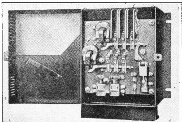
Fig. 11. Automatic controller which uses magnetically-operated contactors to cut the resistance out of the motor circuit in two steps. (Courtesy Cutler Hammer Mfg. Co.)
