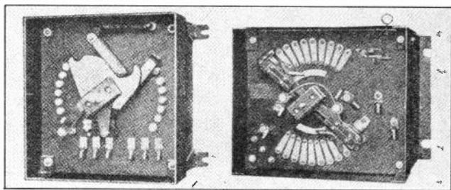
Fig. 6. This view shows two different face plate starters of the resistance type for use with either single-phase or three-phase A. C. motors. (Courtesy Cutler Hammer Mfg. Co.)
