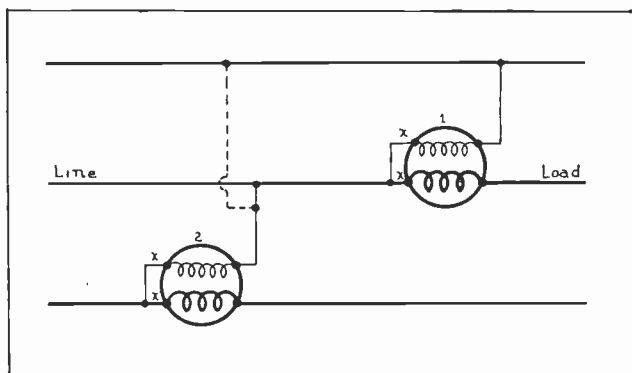
Fig. 8. This sketch shows the correct and incorrect methods of connecting one of the wattmeters when measuring three-phase power by the "two wattmeter method."
