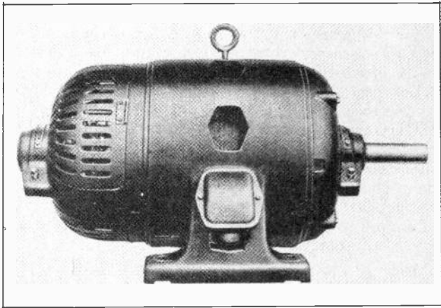
Fig. 21. This photo shows a completely assembled Fynn-Weichsel motor with a guard enclosing the slip-rings and commutator. (Courtesy Wagner Electric Corp.)
