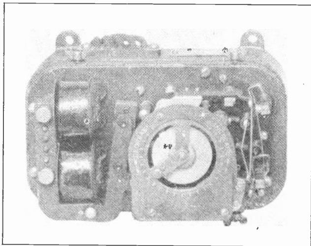
Fig. 6. This photo shows a front view of the motor-operated timing relay for which the connections were shown on Fig. 5. Note the relay magnet and time-setting dial on this unit. (Photo courtesy General Electric Co.)
