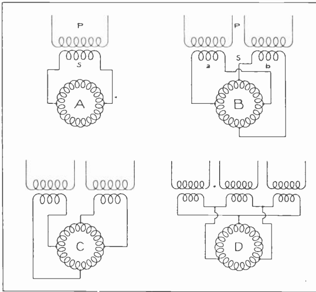
Fig. 8. A. Transformer connections for a single-phase converter. B. Transformer connections for a two-phase, diametric converter. C. Transformer connections for a two-phase, adjacent tap converter. D. Transformer connections for a three-phase converter. The armature connections in all of the above diagrams are for two-pole machines.
