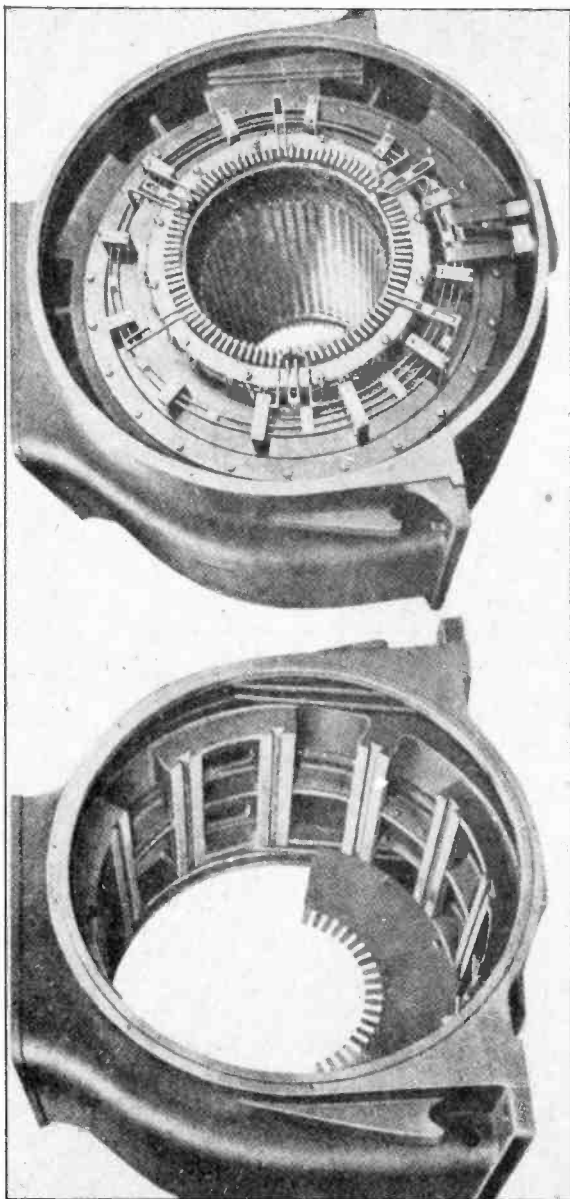
Fig. 7. The above two views show very clearly the method of construction of the stator core and windings of high speed steam-turbine-driven alternators.
