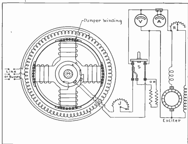
Fig. 14. This diagram shows the connections of the stator and rotor of a three-phase alternator with the exciter-generator, rheostats, meters, and field discharge switch.
