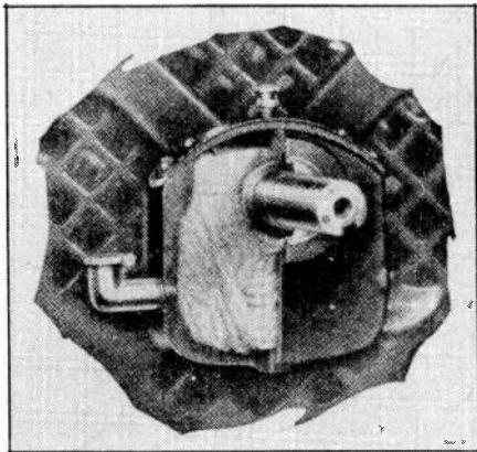
Fig. 9. Bearing with cotton filled oil well, for wick oil feed action to shaft.
