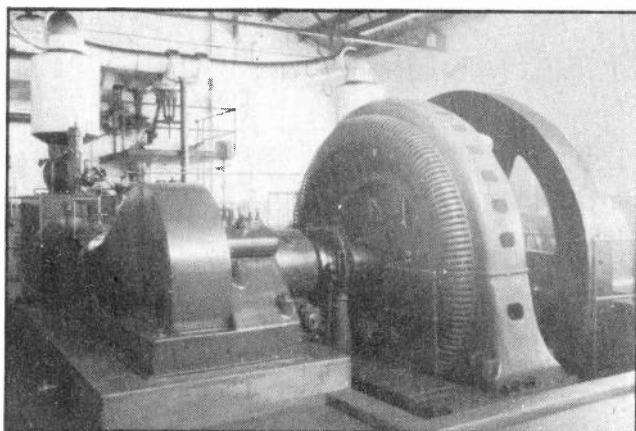
Fig. 4. This photo shows a direct connected steam engine-driven alternator in a small power plant. Note the flywheel used to stabilize the alternator speed and smooth out the pulsations of the engine strokes. Courtesy Allis-Chalmers Mfg. Co.
