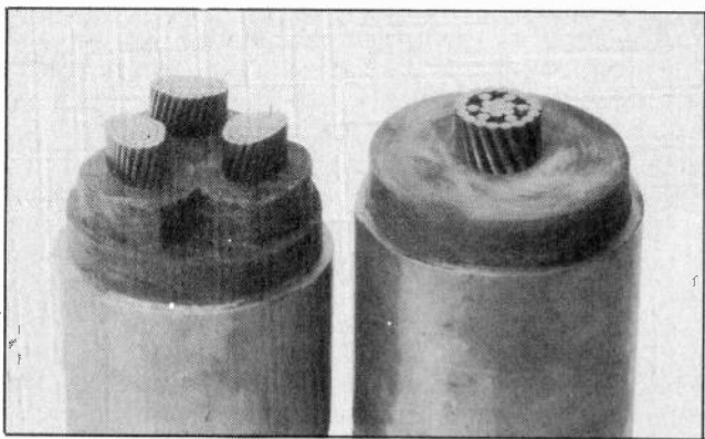
Fig. 6. These views show sections of high-voltage three conductor and single conductor, underground transmission cables. Note the arrangement of conductors and insulation inside of the lead sheath. Courtesy General Electric Co.
