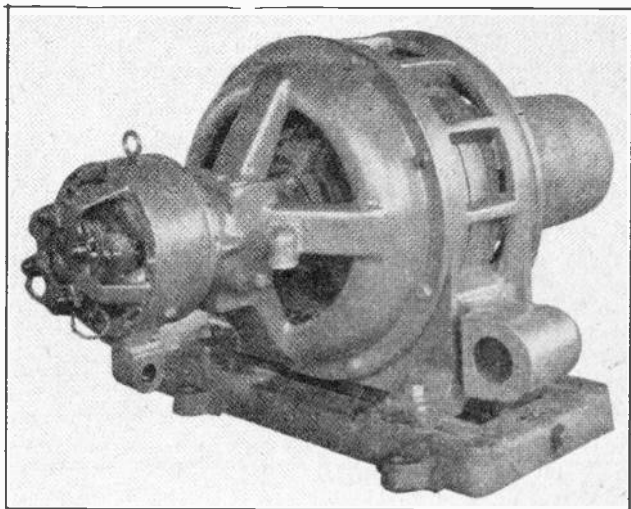
Fig. 1. This photo shows a 75 h. p. synchronous motor of the revolving field type. Note the small exciter-generator which supplies D. C. to the field of the large motor. (Photo courtesy General Electric Co.)
