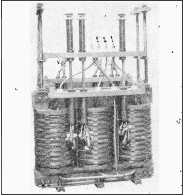
Fig. 7. Complete three-phase transformer core and windings ready to be placed in the tank and covered with oil. (Photo courtesy General Electric Co.)
