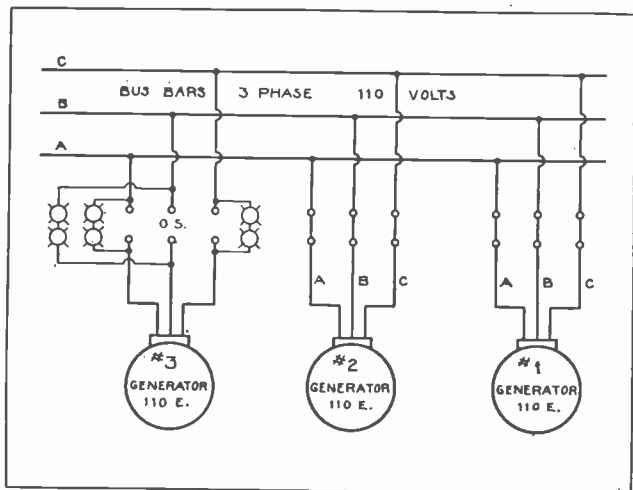
Fig. 1. This diagram shows the method of connecting lamps for phasing out an alternator which is to be operated in parallel with two others.
