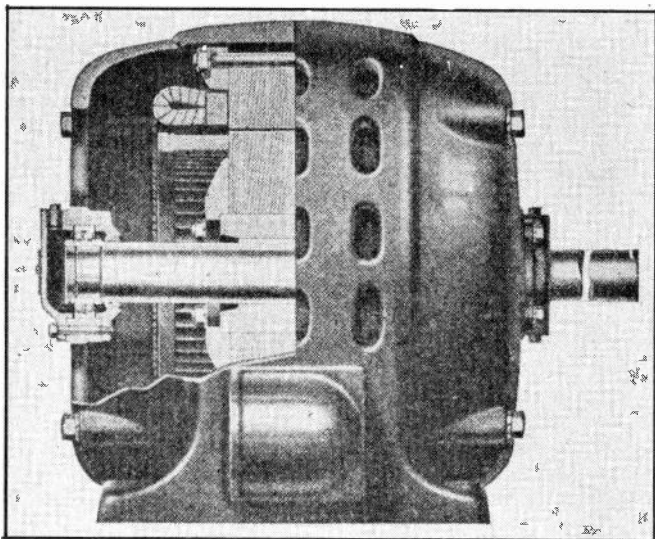
Fig. 8. Sectional view of a squirrel-cage induction motor showing the position of the rotor and bars with respect to the stator core and winding.
