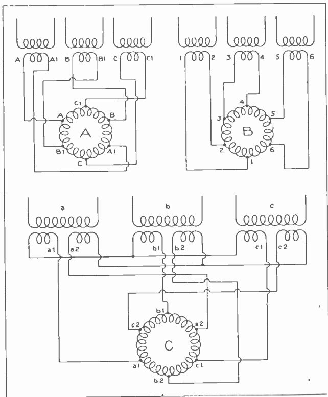
Fig. 10. A. Transformer connections for a six-phase, diametric converter. B. Transformer connections for a six-phase adjacent tap converter. C. Transformer connections for a six-phase, double star-connected converter. Each of these diagrams show the connections for a two-pole machine.
