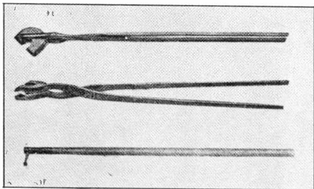
Fig. 20. At the top are shown two wood handled fuse tongs for removing and replacing high-voltage fuses, and below is shown a wood handled switch stick or pole for operating disconnect switches. Courtesy of Schweitzer & Conrad, Inc.
