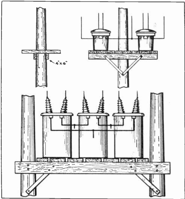
Fig. 4. The above sketches illustrate methods of mounting transformers on platforms on one or two poles.
