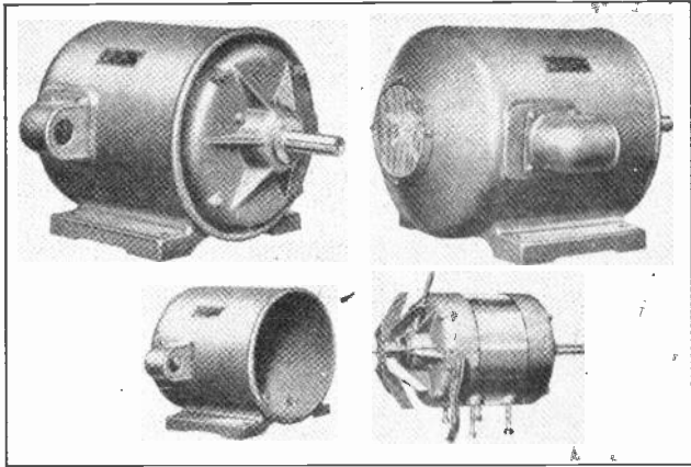
Fig. 22. Completely enclosed A.C. induction motor with special air-jacket to direct the cooling air over the surface of the motor casing. These motors are ideal for use in extremely dirty locations or in places where there are explosive vapors or dust.
