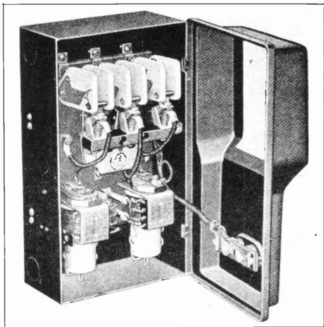
Fig. 4. In this view are shown the overload-relays located beneath the magnetic contactors of an across-the-line starter. (Courtesy Allen Bradley Co.)
