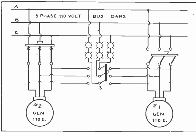
Fig. 3. Connection diagram for synchronizing either of two alternators with the bus bars by means of a lamp bank and double-throw switch.
