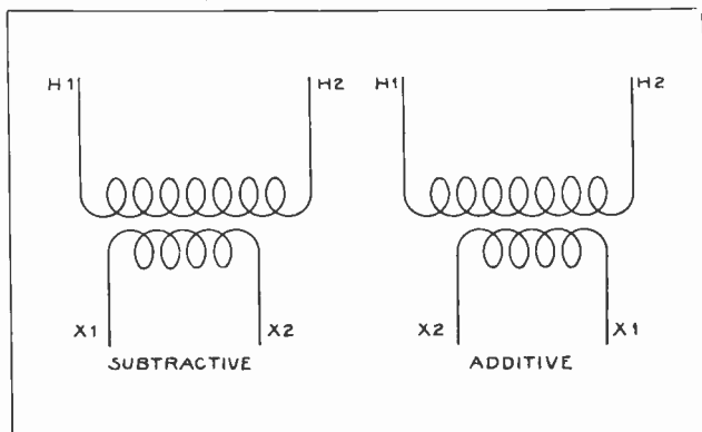
Fig. 19. This sketch shows windings of two transformers with their leads properly marked for subtractive and additive polarities.
