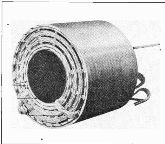
Fig. 6. This view shows a transformer winding which is built up in layers that are spaced apart with wood strips to allow circulation of cooling oil through the windings. (Photo courtesy General Electric Co.)
