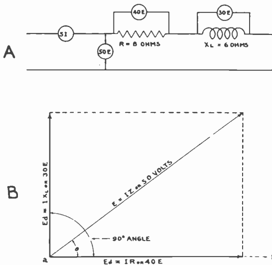
Fig. 8. "A." A resistance coil connected in series with an inductance coil in an A. C. circuit. "B". This sketch shows the method of determining the amount of impedance of the circuit shown at "A".
