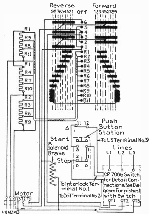
Fig. 18. Wiring diagram of a General Electric drum controller for starting, reversing, and speed regulation of a three-phase, slip-ring motor. Note how the numbers simplify the making of proper connections, even though the wires from the resistance to the drum contacts may be bunched in a cable.
