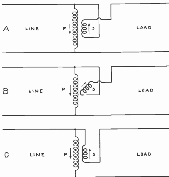
Fig. 6. The above three sketches show the connections and illustrate the principle of an induction voltage regulator. Study carefully each of the three diagrams while reading the explanations given on these pages.
