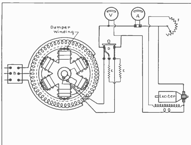
Fig. 6. The above diagram shows the connections for the stator and field of a synchronous motor and also the exciter-generator field discharge switch and instruments.
