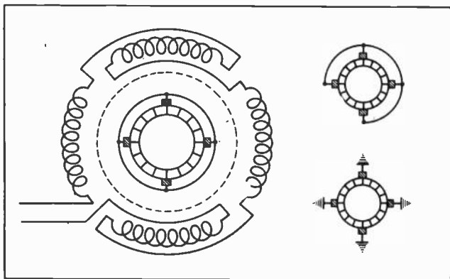
Fig. 17. This diagram shows the connections of the stator winding and brushes of a single-phase A. C. repulsion motor.
