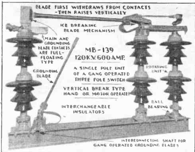
Fig. 14. Single pole unit of 120,000-volt, 600-ampere air-break switch with auxiliary grounding blade. Note the description of the various parts in this figure. Courtesy of Delta-Star Manufacturing Company.
