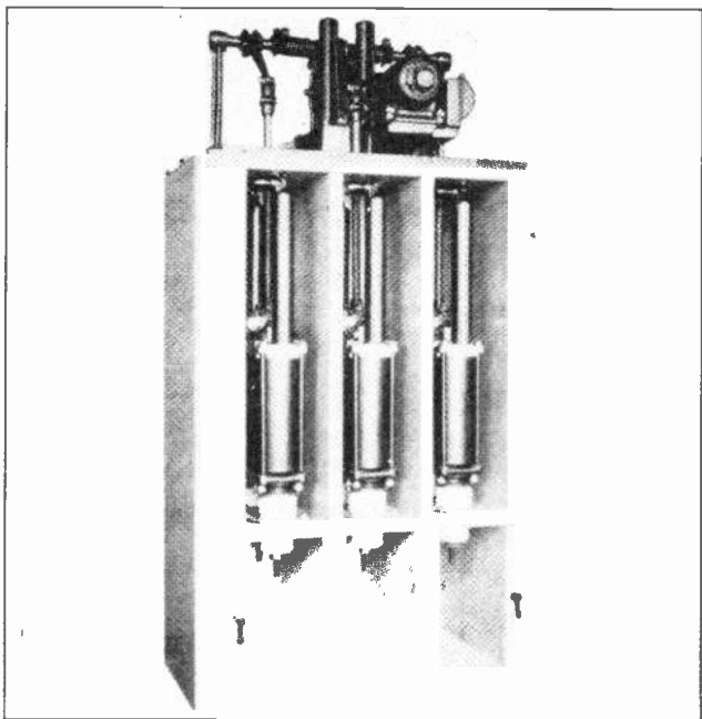
Fig. 6. Modern three-pole oil switch with expulsion type contacts and with pole units located in separate cells or compartments. Courtesy of G. E. Company.
