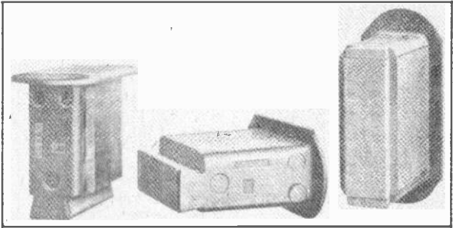
Fig. 9. Several views of laminated field poles such as commonly used in revolving field alternators.
