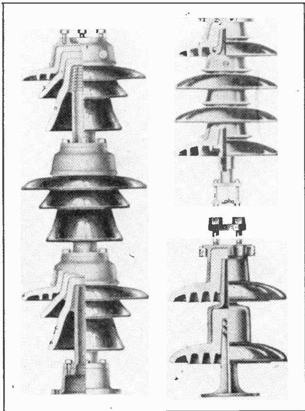
Fig. 20. Three styles of pedestal type insulators which can be built up in rigid pedestal or pillar form to support high-voltage bus bars and switching equipment.
