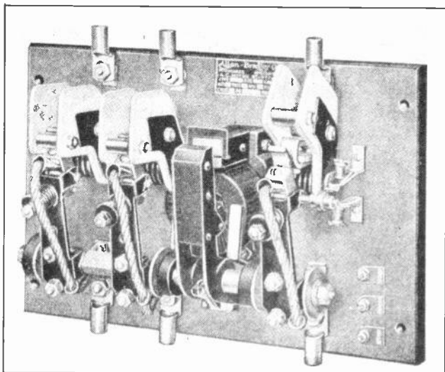
Fig. 16. This photo shows a good view of the magnetically operated contactors used with an automatic, carbon pile resistance starter. Note the arc barriers and blow-out coils on each contactor. (Photo courtesy Allen Bradley Co.)
