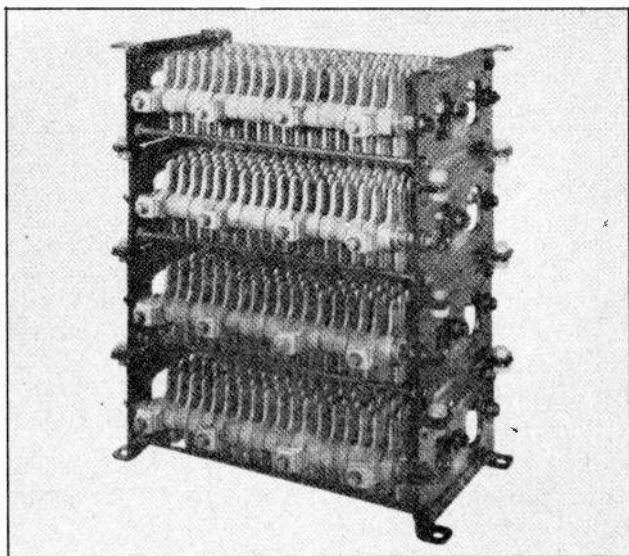
Fig. 13. Photo of complete grid resistor unit for slip-ring motor controllers.
