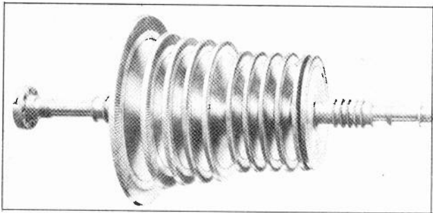
Fig. 13. Complete rotor of a modern steam turbine, showing several sets of moving blades through which the steam passes in succession. Courtesy of Elliott Company.
