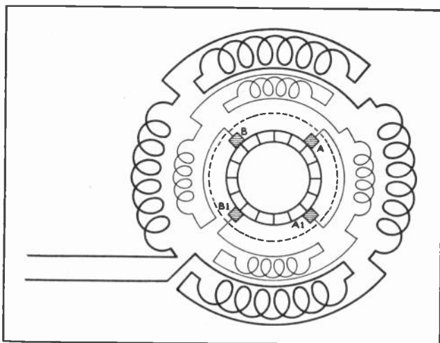
Fig. 18. Diagram of the connections for a repulsion motor with a compensating winding which improves the power factor of this type of machine.
