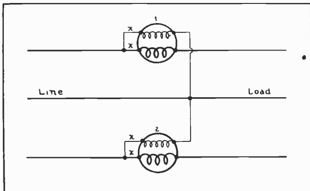
Fig. 6. This sketch shows the connections for using two single-phase wattmeters to measure the power in a three-phase circuit.
