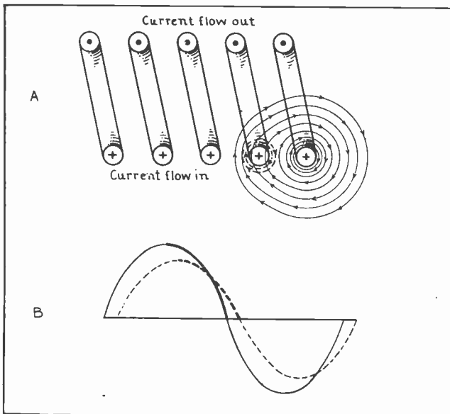
Fig. 4. This sketch shows the same coil as in Figs. 2 and 3 during a period when the current through the coils is decreasing from maximum to zero value. Note how the flux contracts and cuts across the turns of the coil.
