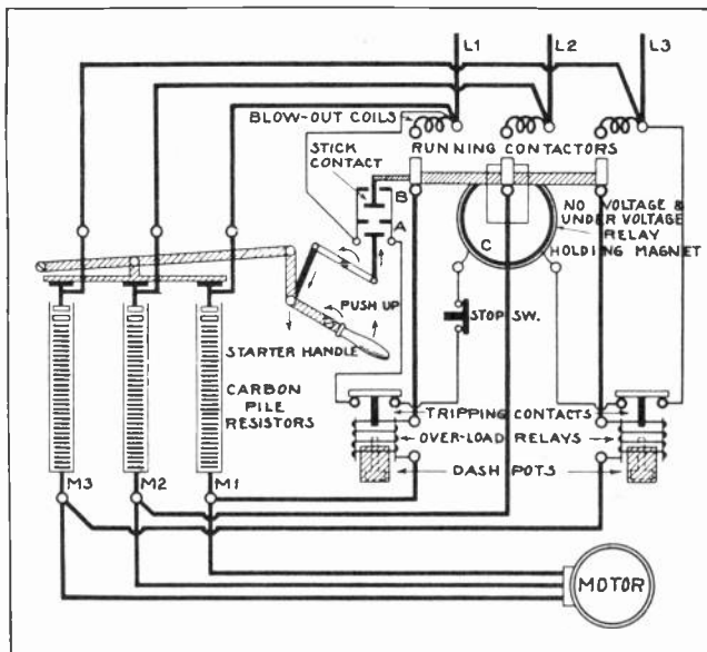
Fig. 13. Diagram showing the wiring and connections of a manually-operated, carbon pile resistance starter for three-phase A. C. motors. Trace this circuit carefully with the accompanying explanation.
