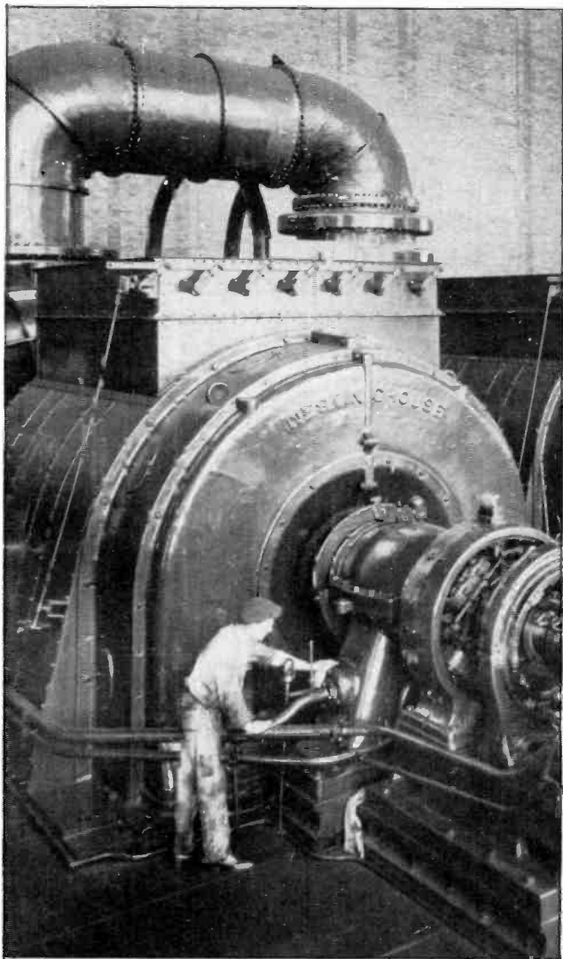
View in the turbine room of the Hell Gate Plant of the United Electric Light and Power Company showing a 50,000 kw tandem compound turbo-generator. Photo by Ewing Galloway, N. Y.
