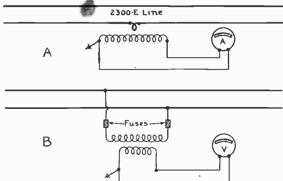
Fig. 1. A shows the connections for a current transformer which is used to operate A. C. ammeters, wattmeters, and current relays. B. Connections for potential transformer used to operate voltmeters, potential elements of wattmeters, potential relays, etc.
