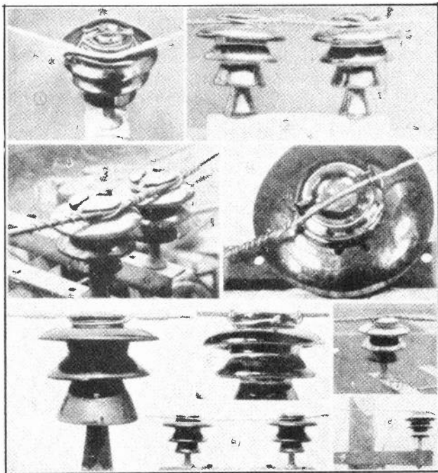
Fig. 17. Above are shown a number of common types of line ties used for attaching conductors of transmission and distribution lines to pin type insulators. Examine each type very carefully as you read the accompanying descriptions and also compare them with the sketches in Fig. 18. Courtesy Lapp Insulator Company, Inc.
