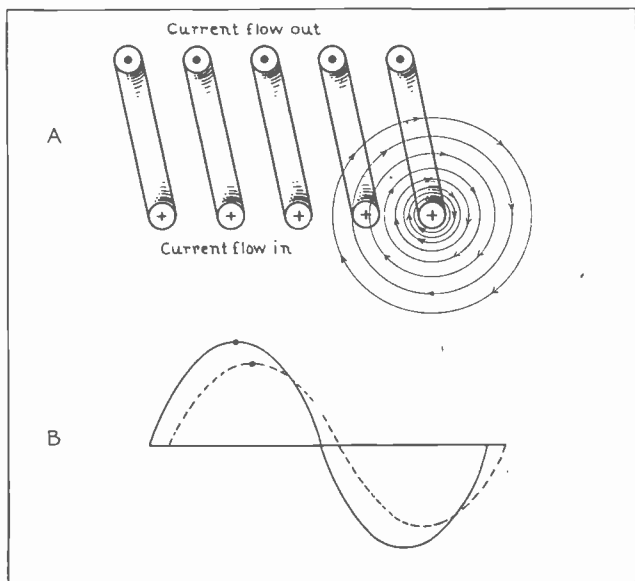
Fig. 3. This view shows the flux around one turn of a coil during the period when the current is at maximum value. The flux is neither contracting nor expanding at this period, and therefore produces no voltage of self-induction.
