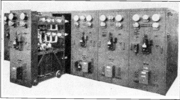
Fig. 4. View of truck-type switchboard showing one section removed to allow repairs or adjustments to be conveniently and safely made. Boards of this type are very popular in modern industrial plants as well as in certain power plants and substations. Courtesy of G. E. Company.
