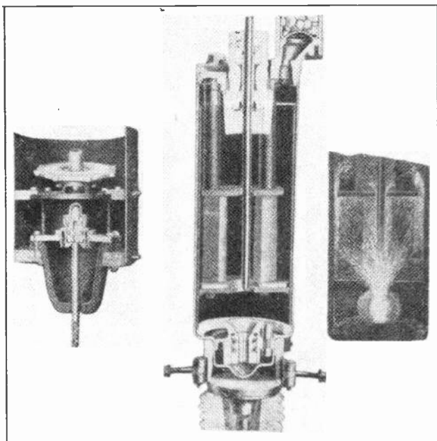
Fig. 8. The above views shows two types of expulsion contacts used in modern oil switches and also one of these contacts in action opening a circuit.
