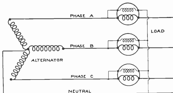
Fig. 12. This diagram shows the connections for three wattmeters to measure the power of a three-phase, four-wire system.
