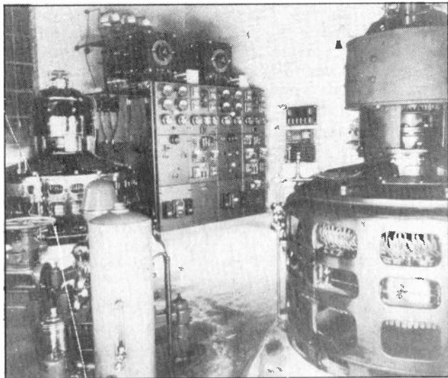
Fig. 20. Interior view of a small automatic hydro-electric generating station. The two generators can be seen in the foreground, and the switchboard in the background of this photo. Courtesy Allis-Chalmers Mfg. Co.
