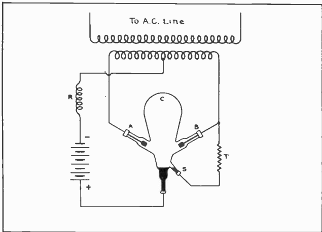
Fig. 2. Circuit diagram of a bulb type mercury arc rectifier used for battery charging purposes. Trace this circuit carefully with the accompanying explanation.
