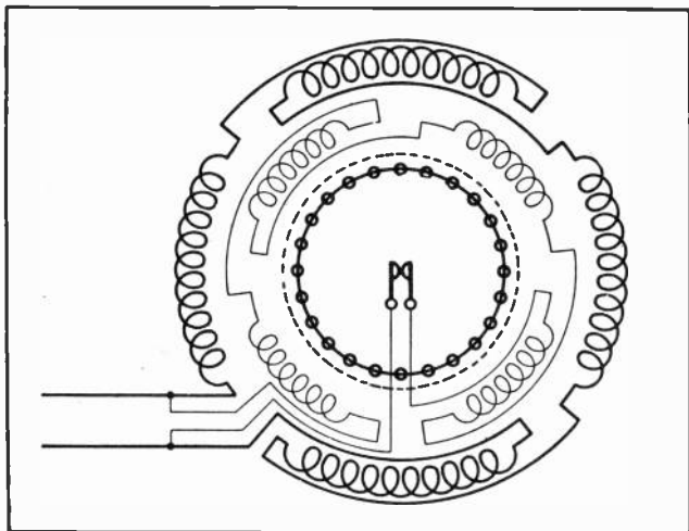
Fig. 11. This sketch shows the connections of the starting and running windings of a single-phase, split-phase A. C. motor.
