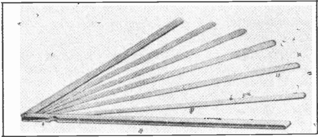
Fig. 11. Common motor air gap gauge, for measuring clearance between the armature or rotor and the field poles or stator. Note the several different "feelers" or blades which are of different thicknesses.
