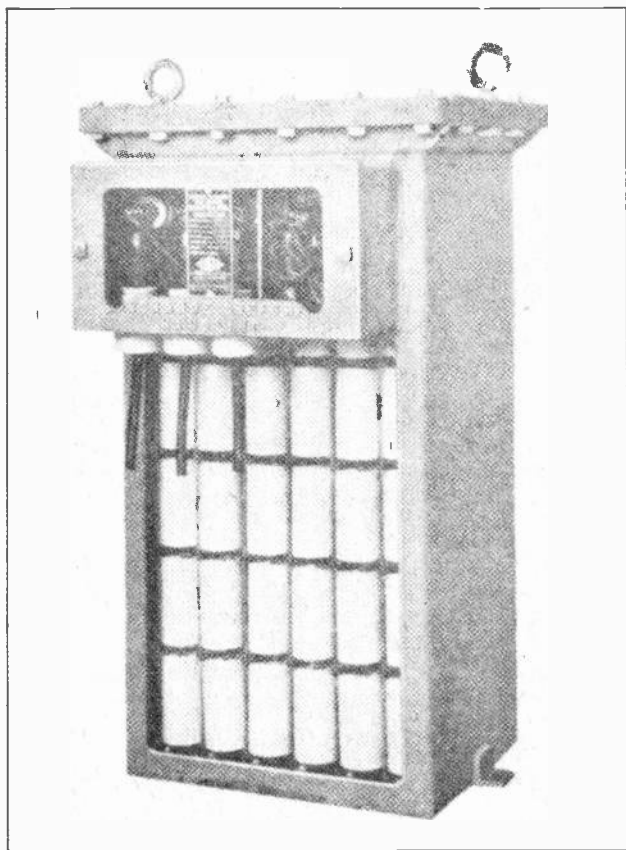
Fig. 5. Complete static condenser with side of tank cut away to show arrangement of roll-type condenser units. (Courtesy Electric Machinery Mfg. Co.)
