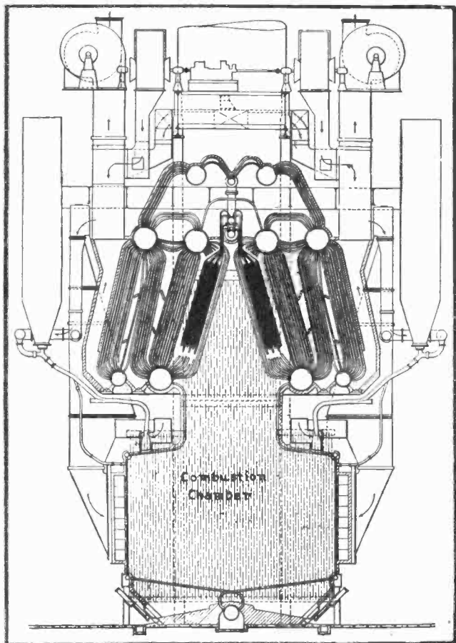
Fig. 8. Another type of large modern power plant boiler showing the combustion chamber, boiler tubes, super-heater, draft fans, etc.
