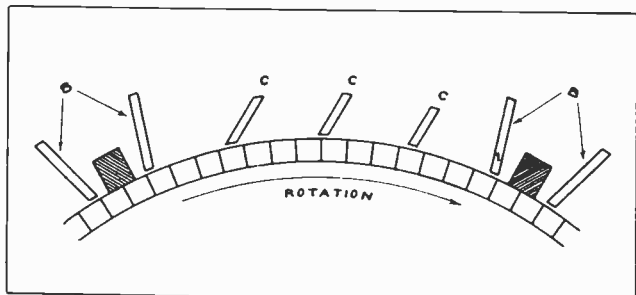
Fig. 14. This diagram shows the position of the flash barriers and arc chutes used to prevent flash-overs between positive and negative sets of brushes on the D. C. end of converters.
