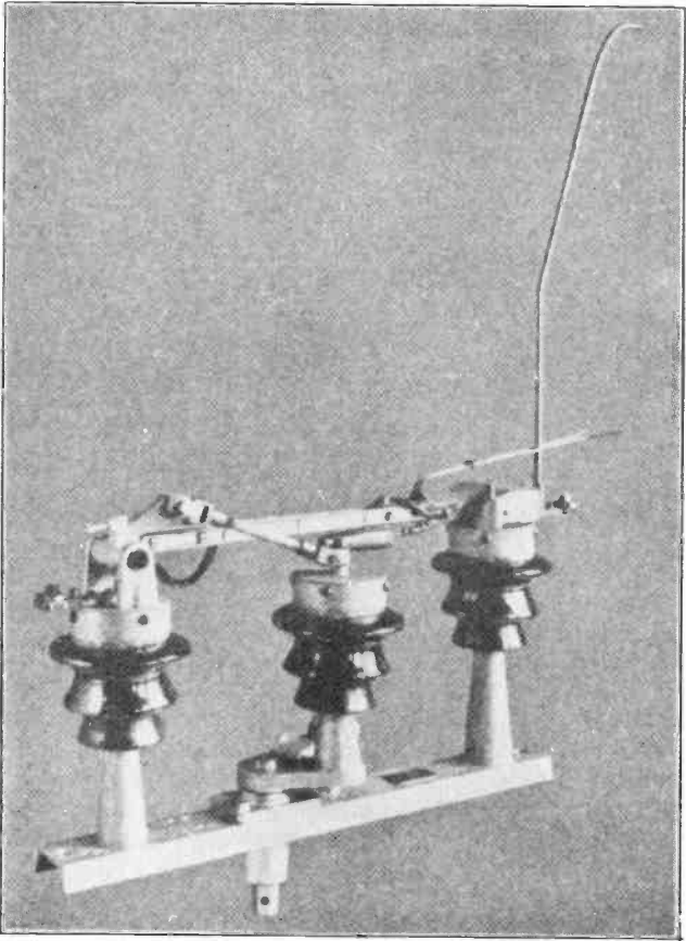
Fig. 11. High-voltage air break switch for pole top mounting or use in substation structures. Note the arcing horns used to prevent pitting and damage to the switch contacts. Courtesy of Hi-Voltage Equipment Company.
