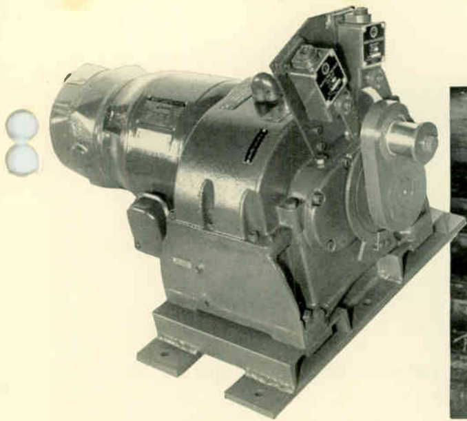
Direct-acting Motocylinders (left) are used to drive roll case unloaders in sawmills (right). Motocyliner is located below unloader
