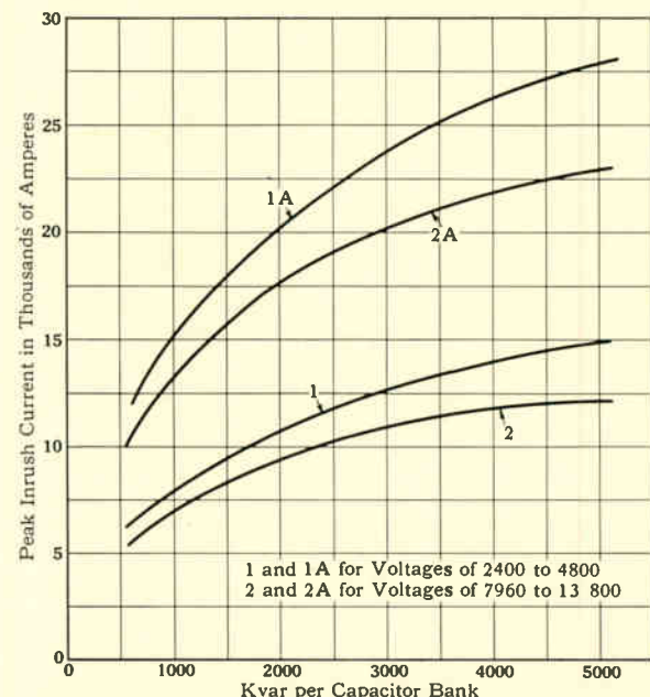
Fig. 6—Energizing inrush currents for capacitor banks located at a point on a circuit where more than one bank is connected. Curves 1 and 2 give current values obtained with one bank already energized; 1A and 2A give values likely with ten or more banks energized.
