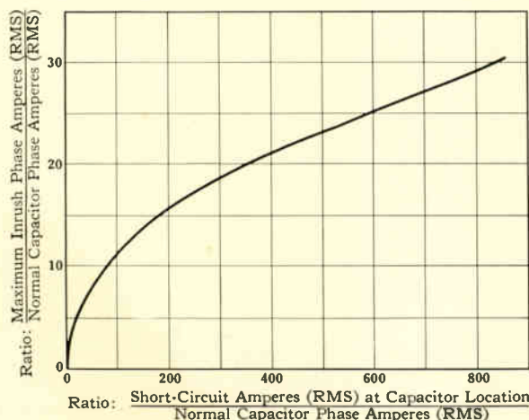
Fig. 5—Energizing inrush currents for fully discharged isolated capacitor banks.
