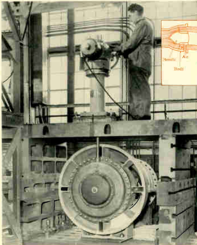
A 30-inch hollow-jet valve being checked at the factory. The sketch at right shows the operation of these valves.
