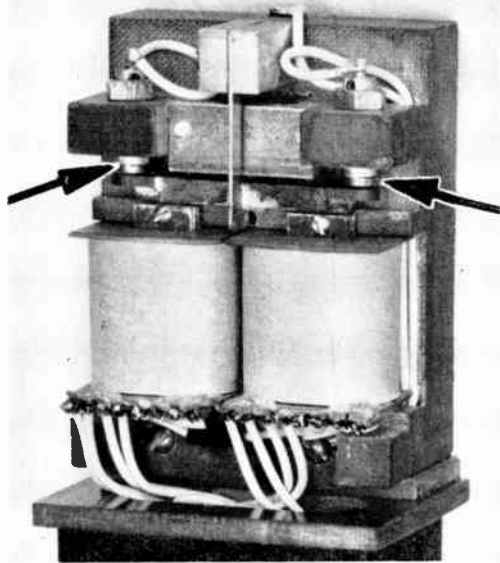
Figure 6—Model of new Western Union "bar" relay. Arrows point to contacts
