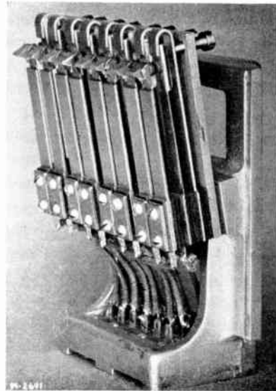
Figure 9—Contact assembly of transmitter impulse unit
