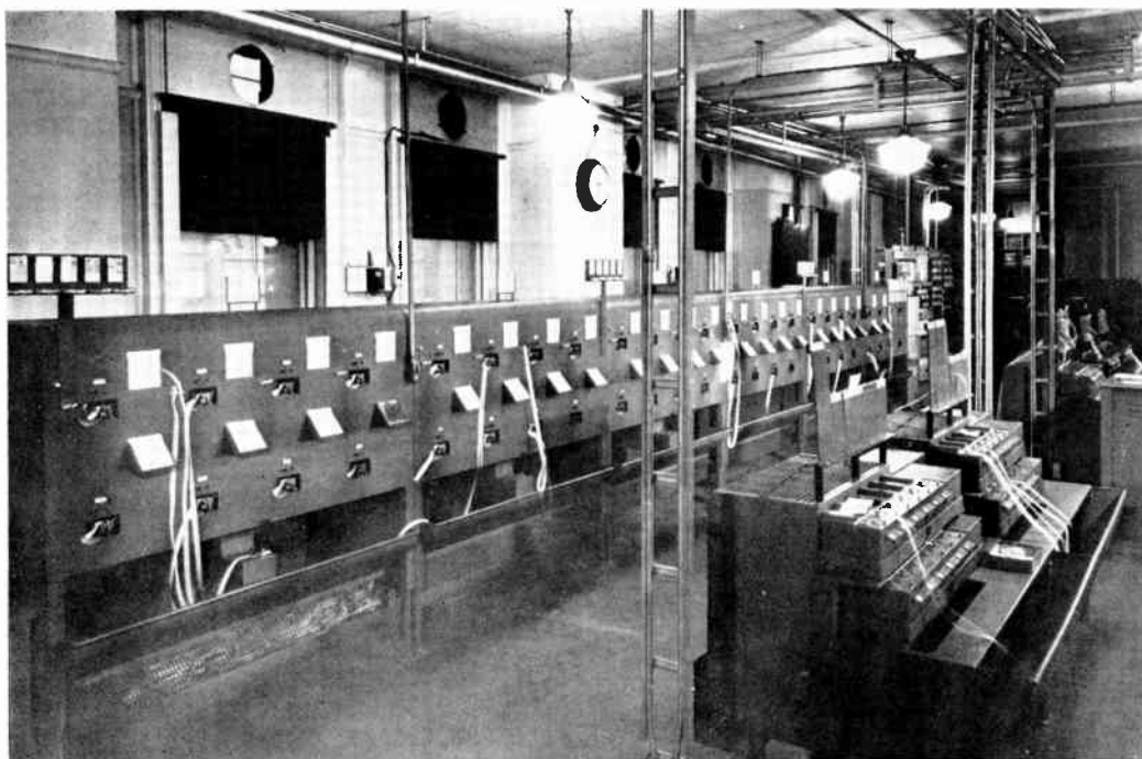
Figure 2—Typical Postal Telegraph semi-automatic switching center installation
