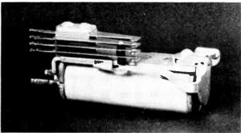
Figure 8—Spring-leaf relay with palladium contacts
