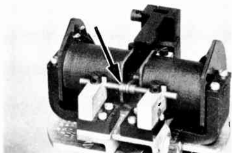
Figure 5—Western Union 17-B relay contact assembly
