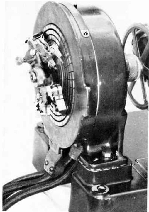
Figure 4—Multiplex sending and receiving head with copper brushes
