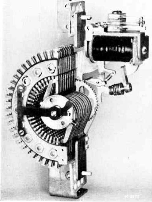
Figure 3—Rotary switch with phosphor-bronze contacts
