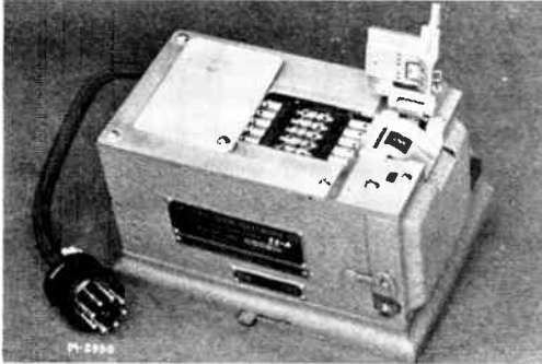
Figure 7—Transmitter actuated by perforated tape
