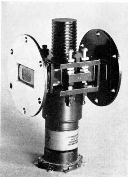
Figure 7. The Sperry SAC-19 synchrondyne tube
