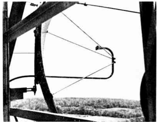
Figure 6. The horn fed truncated parabolic reflector antenna
