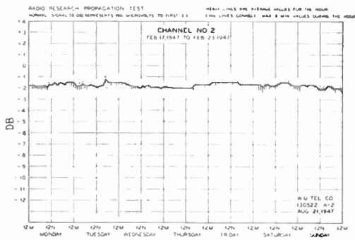
(a) Hourly fading data on 7.2 cm, February 17-23, 1947
