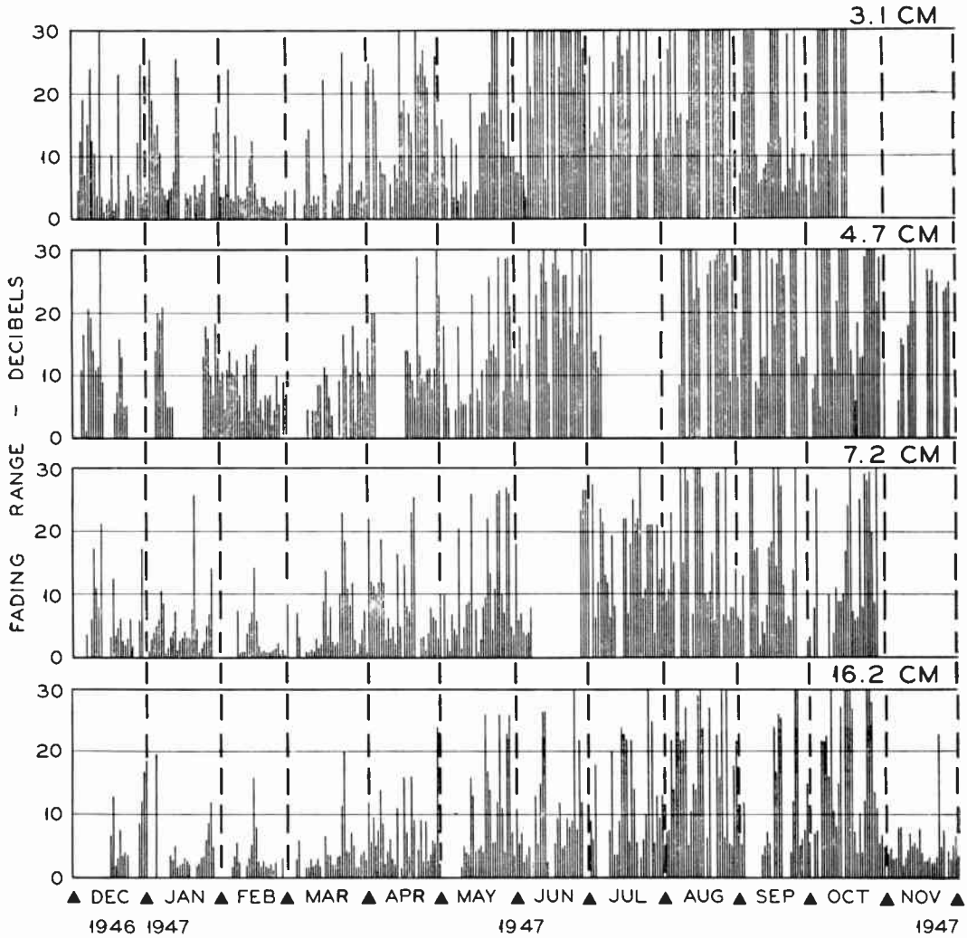
Figure 5. Daily fading ranges from December 1946 through November 1947
