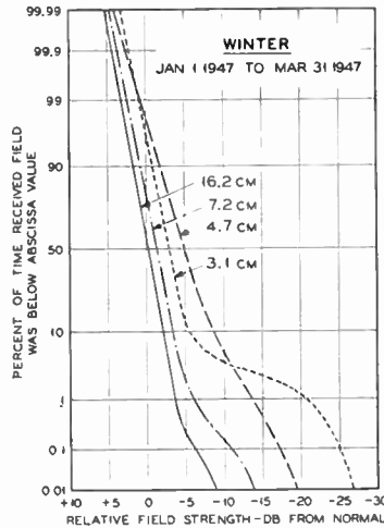
Figure 10. Relative field strength—winter
