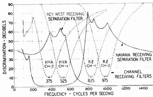
Figure 4. Receiving filter characteristics
