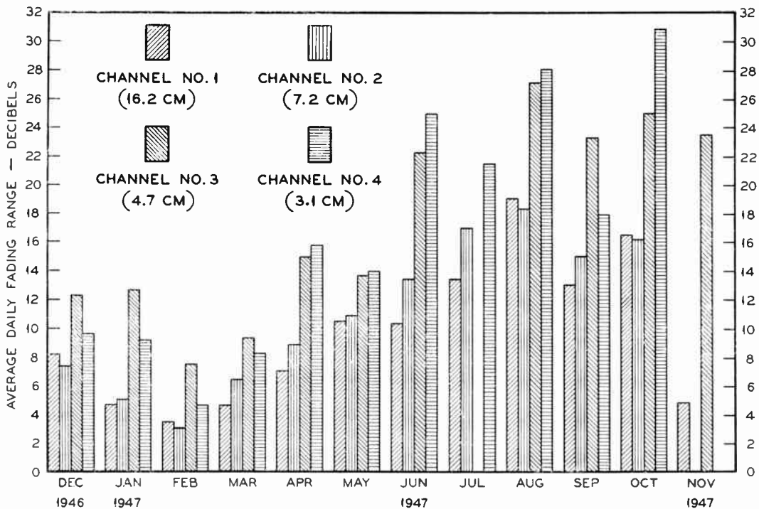
Figure 6. Seasonal variations in fading at different wavelengths
