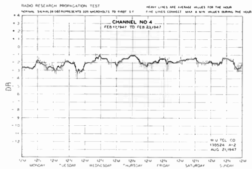
(b) Hourly fading data on 3.1 cm, February 17-23, 1947
