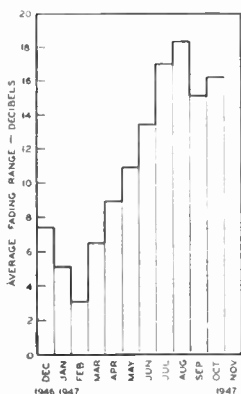
Figure 7. Seasonal variation in fading at 7.2 cm
