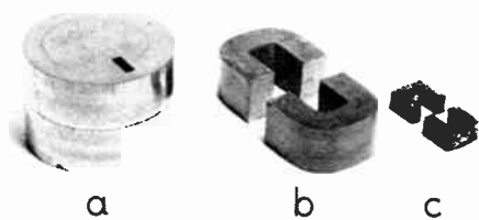
Figure 5. Compressed powder core and wound strip cores
