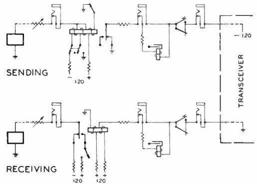
Figure 7. Schematic of telegraph leg circuits
