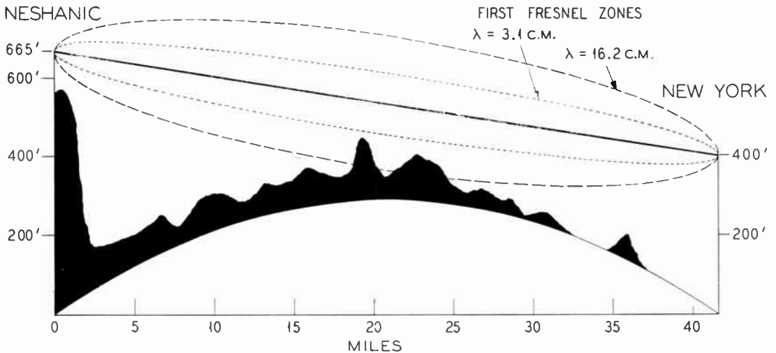
Figure 2. Profile of propagation test path (true earth radius)
