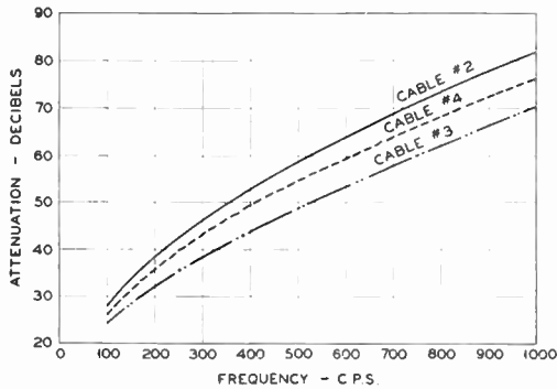
Figure 1. Attenuation of Key West-Havana cables
