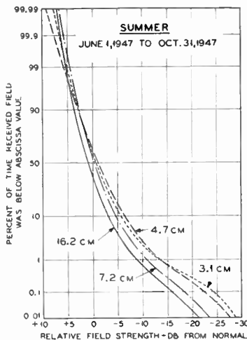
Figure 9. Relative field strength—summer
