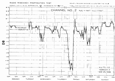
(c) Hourly fading data on 7.2 cm, August 11-17, 1947
