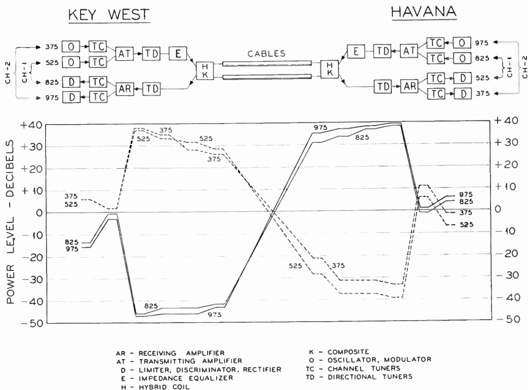
Figure 5. System power levels
