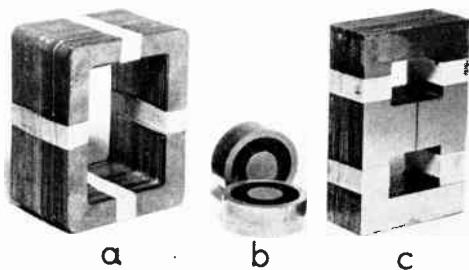
Figure 4. Cores used in filter coils
