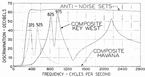
Figure 6. Frequency characteristics of composites and anti-noise sets
