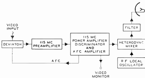
Figure 5. Block diagram of the terminal transmitter
