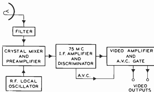
Figure 8. A block diagram of the terminal receiver
