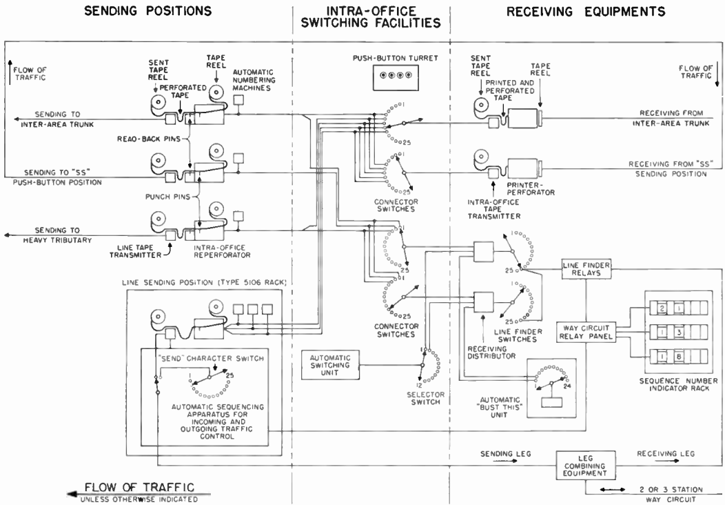
Figure 55. Automatic switching for way circuits
