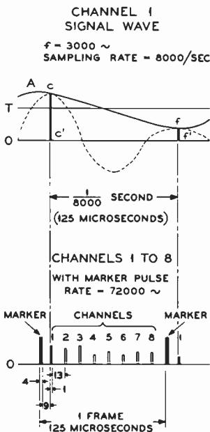
Figure 2. Combining channel samples for multiplex transmission
