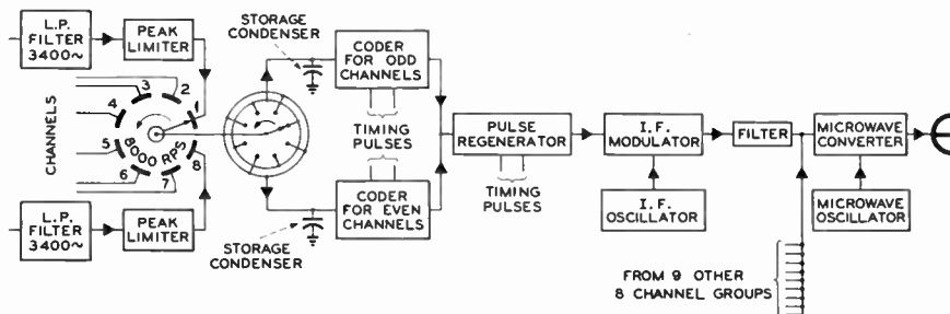
Figure 5. Transmitter for pulse code modulation system
