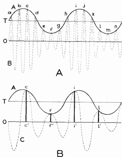
Figure 1. Carrier modulation and sampling processes
