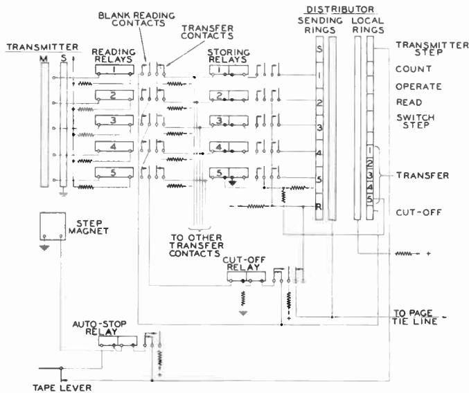
Figure 3. Transfer, auto-stop and cut-off circuits
