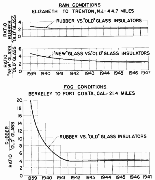
Figure 4. Relative insulation resistance of open wire circuits
