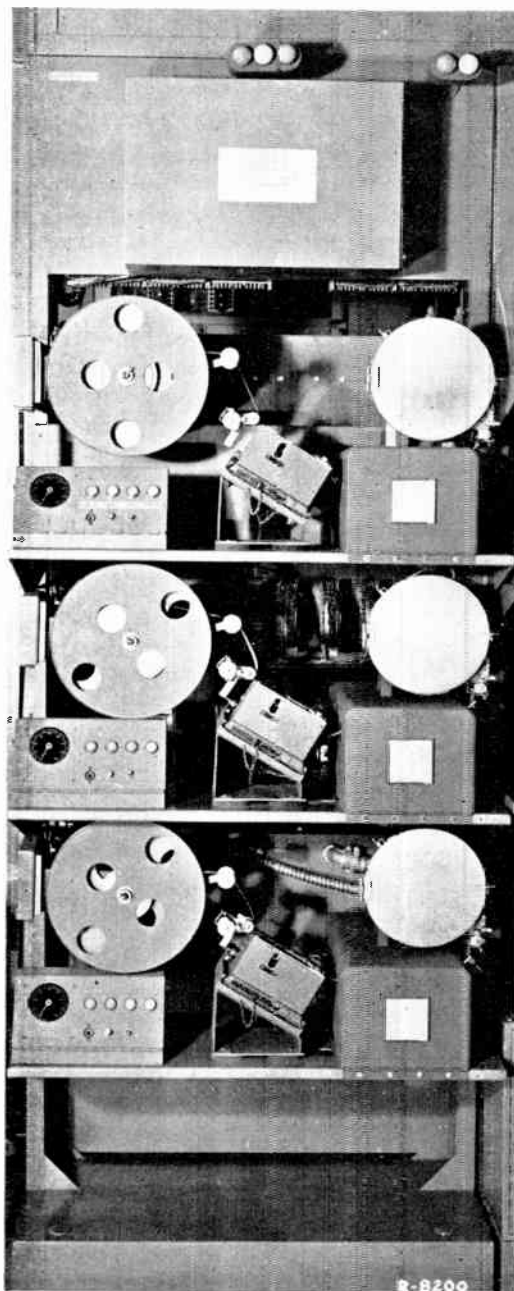
Figure 6. Tape-to-page translator rack for three translators
