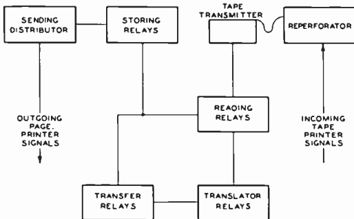
Figure 2. Block diagram of translator
