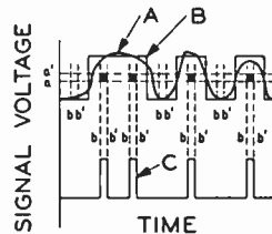
Figure 6. Operation of slicing and gating circuits
