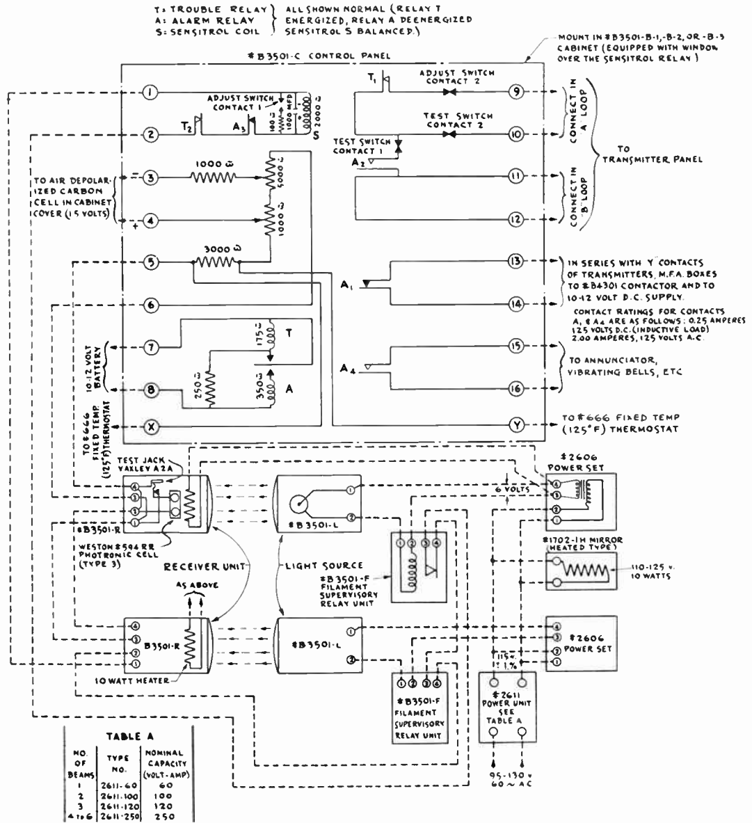
Figure 3. Schematic diagram of ADT Smoke Detection System
