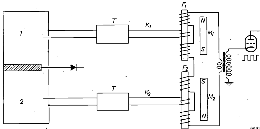
Fig. 5. Diagram of modulation system. The coaxial lines K_1 and K_2 couple the resonators 1 and 2 to the ferrocube rods F_1 and F_2 , which are successively magnetized by an alternating current of rectangular waveform. The permanent magnets M_1 and M_2 pre-magnetize the ferrocube in opposite directions; T = matching transformers.
