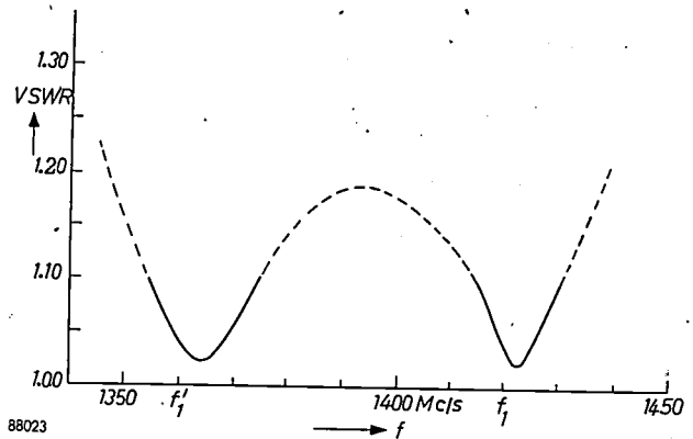
Fig. 3. Matching of antenna to 50 \Omega coaxial feeder at frequencies of f_1 = 1420 and f_1' = 1360 Mc/s (wavelengths 21.12 and 22.08 cm). The degree of matching achieved is expressed by the measured VSWR (voltage standing wave ratio). Perfect matching occurs when VSWR = 1.
