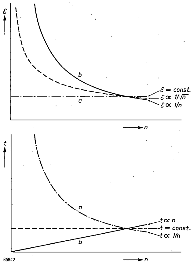
Fig. 11. The relative statistical error \epsilon and required counting time t , as functions of the counting rate n , for three different types of counting strategy.
