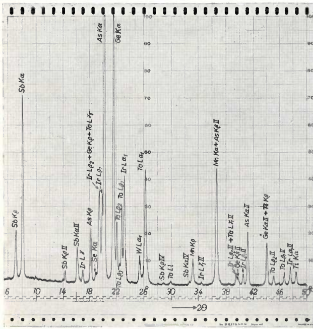
Fig. 6. Qualitative analysis of a mixture of several elements using a quartz analyzing crystal (1011-plane), scintillation counter, scanning speed 1/2^\circ per minute. The K-spectra of 22 Ti, 25 Mn, 32 Ge, 33 As, 34 Se, 51 Sb and the L-spectra of 73 Ta, 74 W and 77 Ir can be seen. (The higher order reflections are indicated by Roman numerals.)
