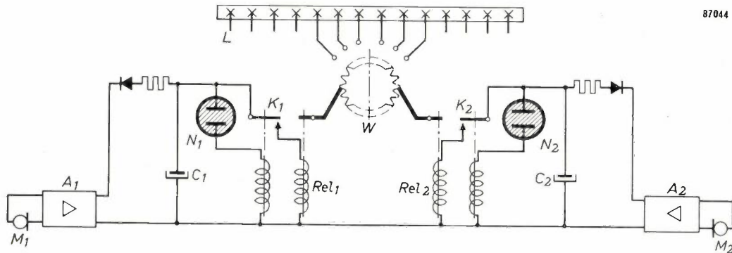
Fig. 8. Circuit of the "Phililoei". M 1 , M 2 are microphones; A 1 , A 2 amplifiers; C 1 , C 2 condensers; N 1 , N 2 neon lamps 85 A 2; K 1 , K 2 relay contacts; Rel 1 , Rel 2 exciting coils of the multi-contact switch W and L indicator lamps.
