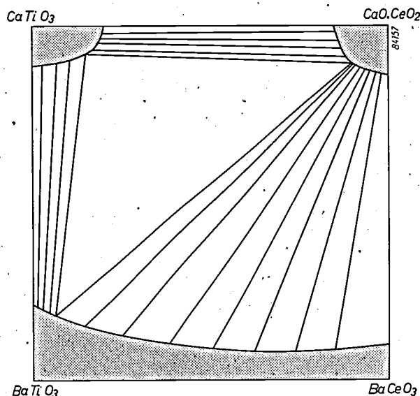
Fig. 10. Phase diagram for the system \text{BaTiO}_3 - \text{CaTiO}_3 - \text{CaO} \cdot \text{CeO}_2 - \text{BaCeO}_3 (schematic). In this diagram, besides the two perovskite phases, a third phase with fluorite structure, occurs in the \text{CaO} \cdot \text{CeO}_2 corner. The Gibbs free energy is so small there that the disposition of the connodes in this diagram differs from that in fig. 7.
