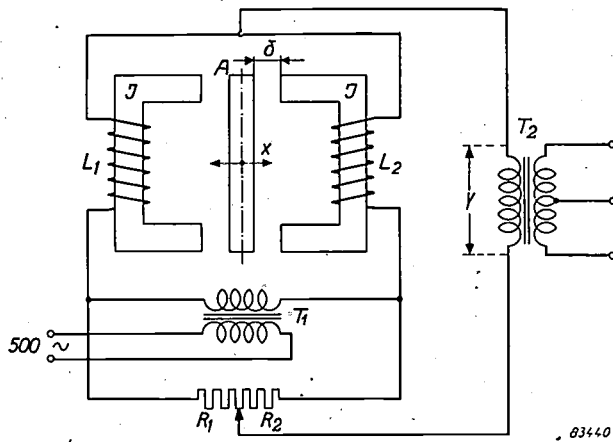
Fig. 7. Schematic diagram of inductive displacement pick-up. The coils L_1 and L_2 , together with the resistors R_1 and R_2 , form a bridge circuit fed by an valve oscillator (500 c/s) via transformer T_1 . The bridge is balanced if armature A is located mid-way between the yokes J . If the armature is located to the left or to the right of the centre, a voltage y is produced across the primary of the output transformer T_2 .
