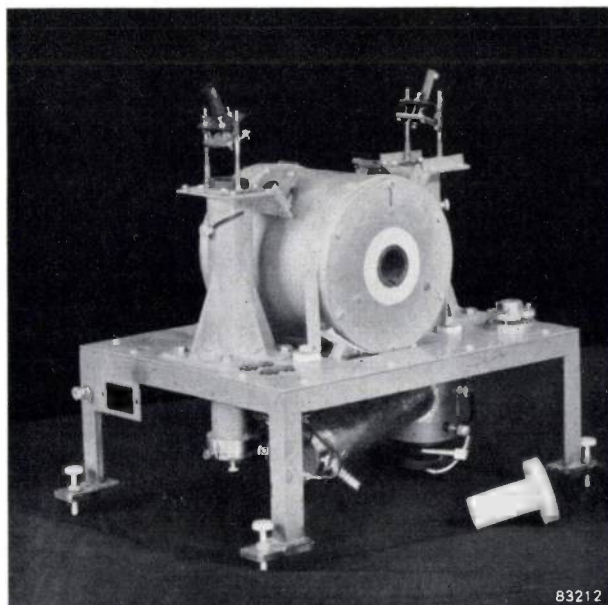
Fig. 3. Photograph of the apparatus sketched in fig. 2 . The components marked in fig. 2 are easily identified. A spirit level can be seen on the right of the base plate of the furnace; the slide carrying the glaze sample must lie horizontally so that the glaze will not move out of the beam of light during the test.
