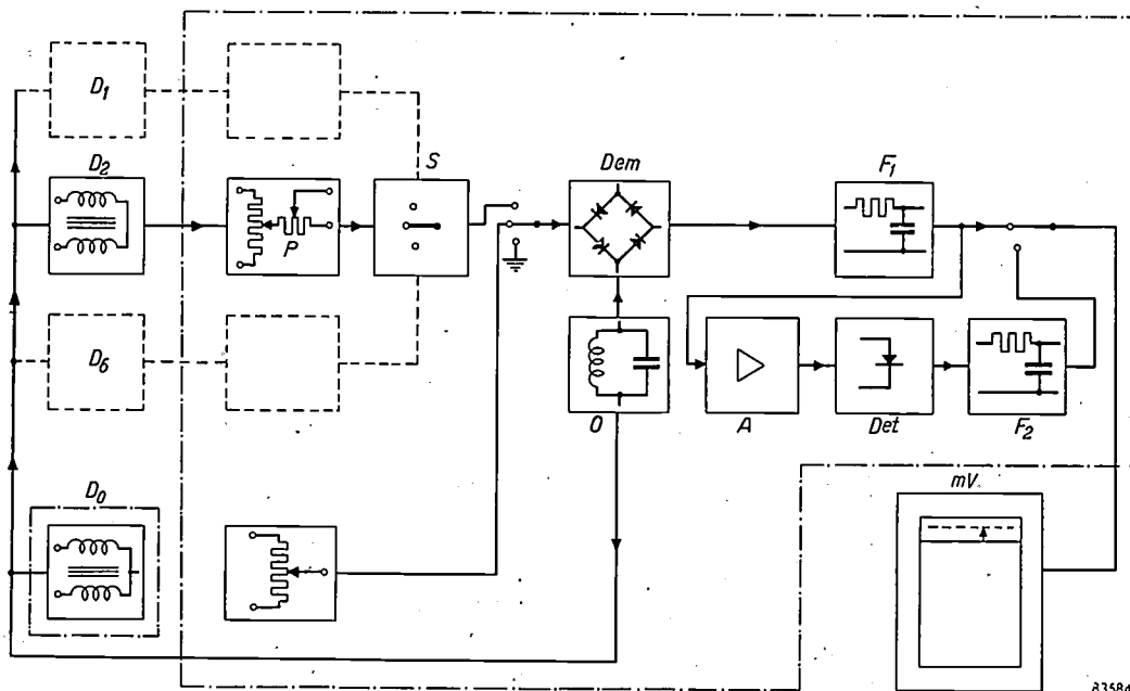
Fig. 13. Simplified block diagram of the circuit for monitoring changes in length and eccentricity. D_1 \dots D_6 six displacement pick-ups. D_0 calibration pick-up. P potentiometers for adjusting the zero point and the sensitivity. S rotary switch. O oscillator 500 c/s. Dem demodulator. F_1 smoothing filter 500 c/s. A amplifier. Det detector. F_2 smoothing filter shaft frequency. ( A , Det and F_2 only function for measuring the eccentricity at rotor speeds above 48 r.p.m.) mV recording millivoltmeter.
