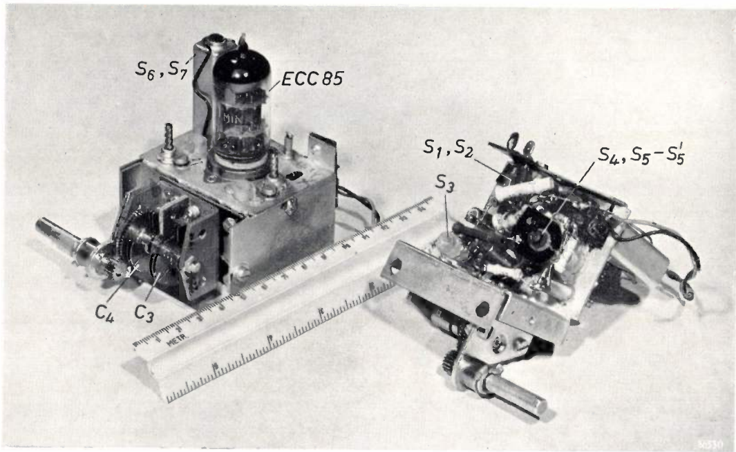
Fig. 3. One form of the circuit of figure 2a, seen from above and below. The letters refer to the corresponding components in fig. 2.
