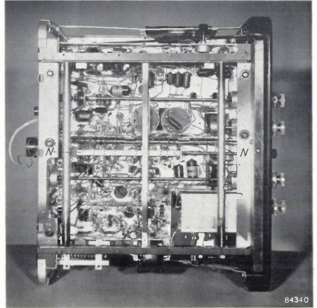
Fig. 2. Chassis of the set illustrated in fig. 1, seen from below. NN is the spindle of the standard selector which runs right through the chassis.
