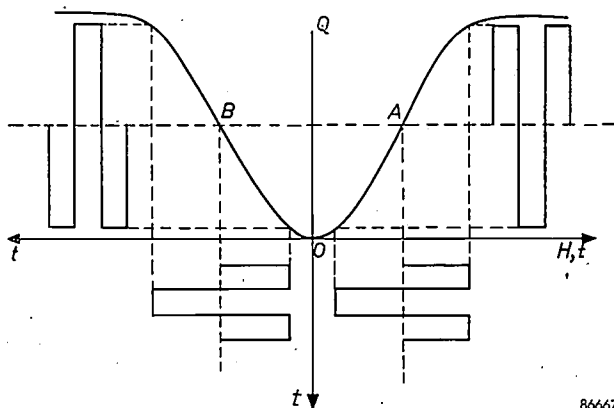
Fig. 6. The quality factor Q of the cavity resonator as a function of the magnetic field H surrounding the ferrocube. The Q factor of the two cavity resonators is oppositely modulated by oppositely pre-magnetizing the ferrocube rods, the direction of H being the same.
