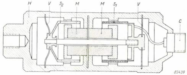
Fig. 2. Cross section of the electro-dynamic vibration pick-up PR 9260. M permanent magnet, mounted in the housing H . S 1 output coil (with connection contact C ). S 2 damping coil (copper sleeve acting as a short-circuited winding). The coils are mechanically connected and suspended between the spring membranes V .
