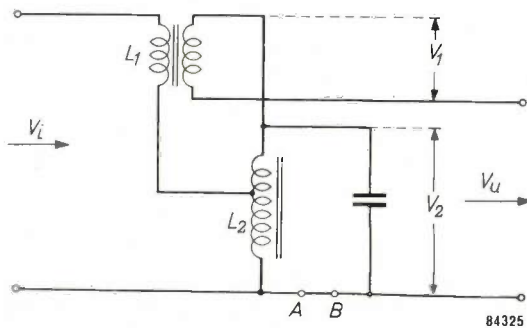
Fig. 4. Stabilizer similar to that of fig. 3, with compensation winding on L_1 . Here L_2 is in the form of an autotransformer, so that V_u is equal to the nominal value of V_i .
