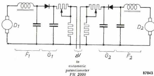
Fig. 5. Circuit diagram of the "Knijp van Jut" (Test your Clench). D_1 , D_2 are hand-dynamos; F_1 , F_2 low-pass filters and G_1 , G_2 rectifiers.
