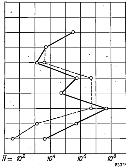
Fig. 1. Average number of quanta or particles ( \bar{N} ), for a round detail 2 mm in diameter, effective for 0.2 sec, in different image-stages in fluoroscopy without the image intensifier (dotted line) and with it (full line). Object: 8 cm "Philite" + stationary scatter grid. Distance to focus 90 cm. 40 kV, 1 mA.
