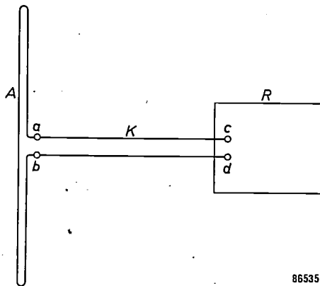
Fig. 8. Folded dipole A connected by a feeder K to the receiver R .
