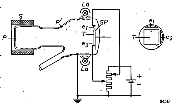
Fig. 6. Schematic cross-section of a "P.E.S. Photicon" (reproduced from fig. 7, page 145, of the article referred to in note 4). P' auxiliary photo-cathode, illuminated by a ring of incandescent lamps La. Segment-shaped control electrodes e 1 and e 2 with variable voltage, direct the low-velocity photo-electrons from P' to parts of the target plate T where the concentration of redistribution electrons is low. This suppresses the spurious signals. Meanings of the other letters as in fig. 2.
