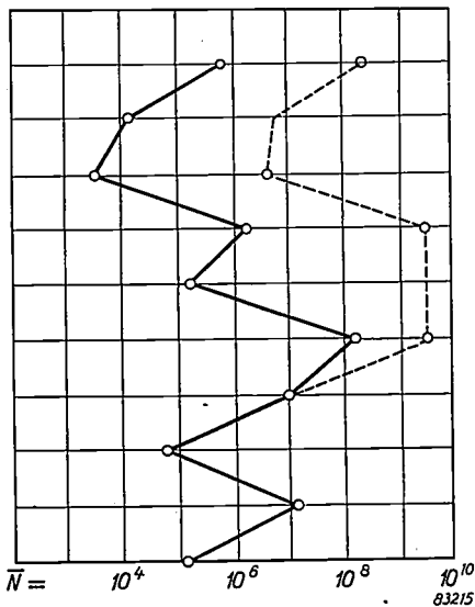
Fig. 2. Average numbers of quanta or particles ( \bar{N} ), per detail 2 mm in diameter, effective in miniature radiography without the image intensifier (dotted line) and with it (full line). Without the image intensifier: Fluorescent screen photographed with a mirror camera, f/d = 1 , on 70 mm film ("Scopix Ortho"). Total reduction 7 \times . Exposure 40 kV, 180 mA sec. With the image intensifier: Viewing screen of the image intensifier photographed through an optical system (two lenses: f/d = 1.5 , f = 55 mm, and f/d = 2.0 , f = 75 mm) on 35-mm film (Agfa "Fluorapid"). Total reduction 6.5 \times (that is, reduction in image intensifier 9 \times , optical magnification 1.4 \times ). Exposure 40 kV, 0.6 mA sec. Object: 8 cm "Philite" + stationary scatter grid. Distance to focus 90 cm.
