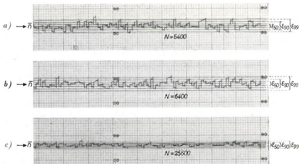
Fig. 22. Measurements of a constant X-ray intensity with the counting-rate computer, in order to check the statistical fluctuations of the counting rate. In each of the three cases, 100 measurements of a fixed number N of counts are performed.
