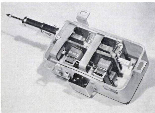
Fig. 11. The displacement pick-up of fig. 10 with the cover removed and closed ready for mounting. For calibration, the amount of the displacement can be read direct from a scale; this reading should correspond to the deflection of the recording meter.
