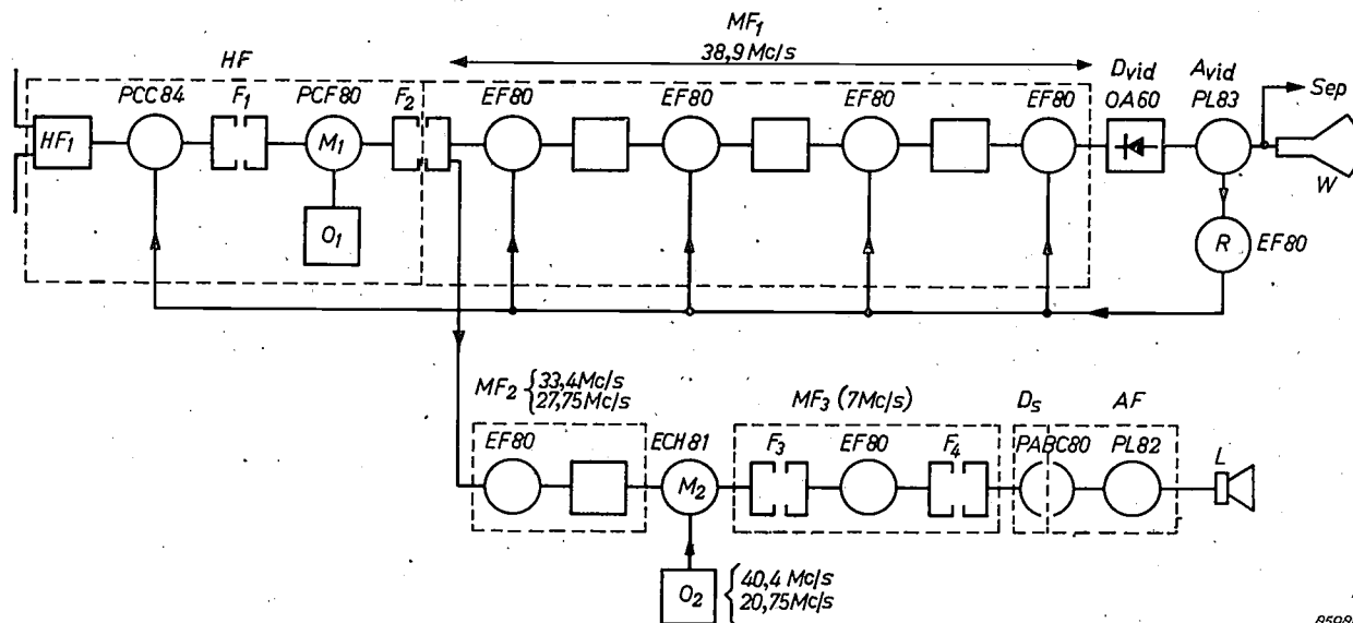
Fig. 7. Block diagram of the television receiver for four standards. HF high frequency section (incorporating the channel selector, see fig. 3), with high frequency band filter F_1 , first oscillator O_1 , first frequency-changer M_1 and part of the I.F. band filter F_2 . Vision channel: MF_1 intermediate frequency amplifier with four tubes EF 80, D_{vid} video detector, A_{vid} video amplifier, R
