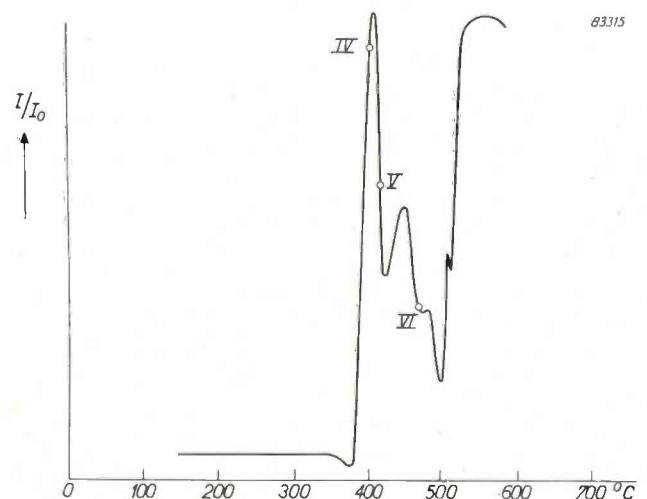
Fig. 7. Recorded gloss curve of an experimental glaze prepared in the laboratory. The heating-rate was 2 °C per minute. As the heating-rate increased, the curve was displaced as a whole towards somewhat higher temperatures without appreciable changes in the various features of the curve.
