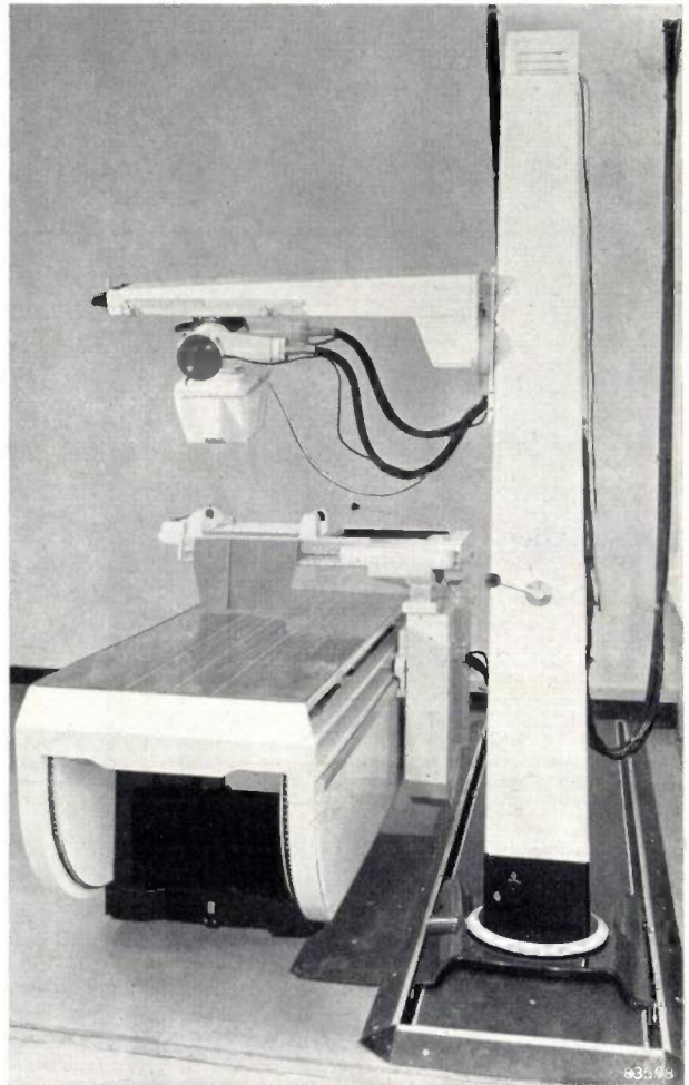
Fig. 11. Column carrying the alternative X-ray tube, for use with the "Symmetrix" stand. The column runs on double floor rails and rotates on its axis. The X-ray tube and its diaphragm are attached to an arm and can be moved to and fro along it. The arm rotates on its axis and can be raised and lowered on the column.
