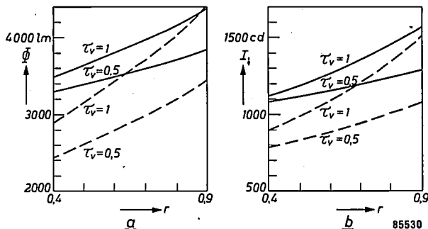
Fig. 10. a) Effect of the reflection factor r of the reflector of a two-lamp trough fitting on its luminous flux. The full lines refer to "TL" F lamps, the dotted lines to normal lamps. Both types of lamp were measured in a clean condition ( \tau_v = 1 ) and with a layer of dirt on the upper surface ( \tau_v = 0.5 ). b) As for (a), but showing the effect on the luminous intensity vertically downwards, I_{\downarrow} .
