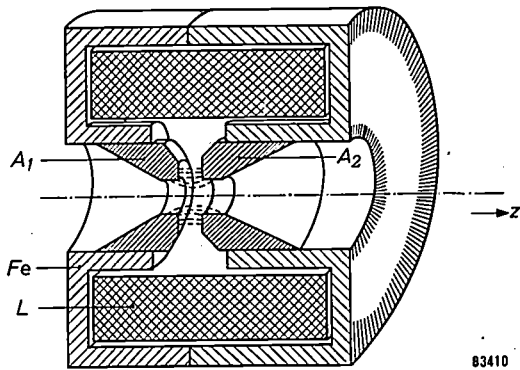
Fig. 2. Magnetic electron lens. L coil, Fe iron jacket, A 1 , A 2 pole pieces. The electrons move close to the z -axis, which is the axis of rotational symmetry of the magnetic field of the lens.
