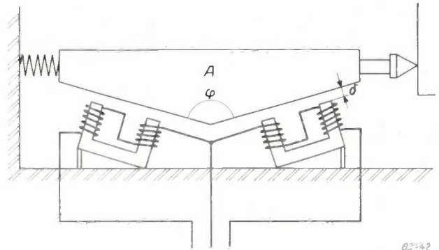
Fig. 10. Displacement pick-up for measuring the absolute change in length of the casing. The principle is the same as that of the pick-up of fig. 7, but owing to the tapered shape of armature A , a change in length of the shaft now corresponds to a 50 times smaller change of the air gap \delta . The angle \varphi , actually about 178^\circ , is shown smaller for the sake of clarity.
