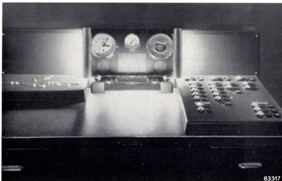
Fig. 11. Control desk. Left: plan of airfield with monitor lamps at points corresponding to the positions of the real runway lights. Right: push buttons and signal lamps of the main switches and the runway and luminous intensity selectors. Centre: panel with clock and meteorological instruments. The spaces on either side are for telecommunications equipment.
