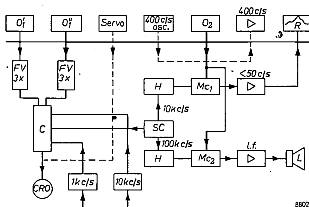
Fig. 6. Simplified block diagram of the frequency calibration circuits (full lines) and control circuits (broken lines). The units above the horizontal line are parts of the receiver proper (see fig. 2). FV frequency multipliers, C calibration panel, KO cathode ray oscilloscope, SC secondary frequency standard, H harmonic generators, Mc 1 and Mc 2 mixer circuits, L loudspeaker.
