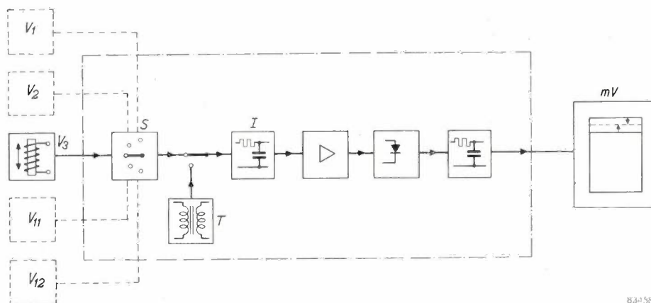
Fig. 5. Block diagram showing the connection of the vibration pick-ups V_1 \dots V_{12} (7 in fig. 1 ) alternately connected via a rotary switch S to the integrating network I . The output voltage of I is applied via an amplifier, a rectifier and a smoothing filter to a recording millivoltmeter mV (see fig. 6 ). T calibration transformer.
