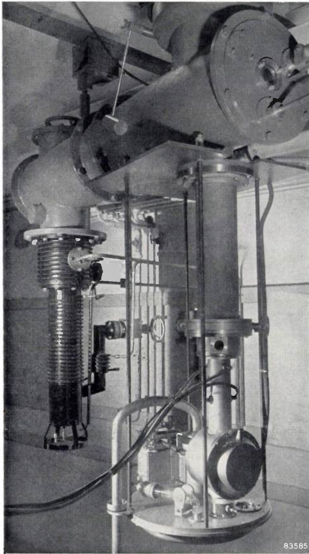
Fig. 2. The earthed lower end of the acceleration tube (a floor lower than in fig. 1). In the background is the pump installation which maintains the high vacuum in the acceleration tube.
