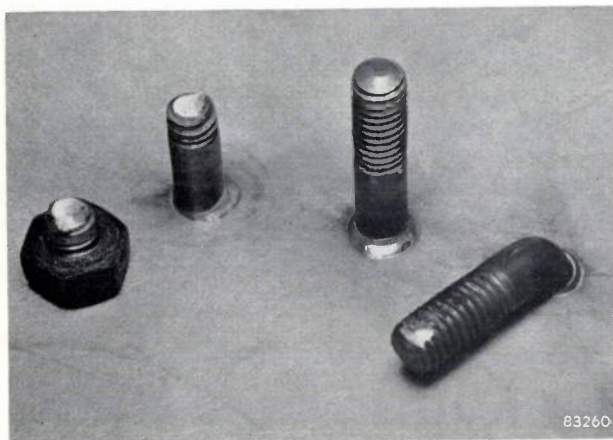
Fig. 13. Simple tests to determine the mechanical strength of the joint between stud and work. Right: a stud bent through 90^\circ by hammering. Left: a stud sheared off by turning a nut against a metal sleeve (not shown in the photograph) fitted round the stud. The part of the stud broken off, with the nut still on it, is seen on the extreme left of the picture.
