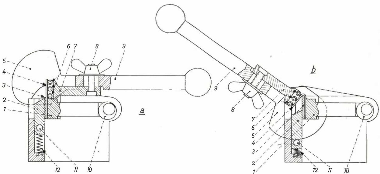
Fig. 2. Structural design: 1 clamping piece; 2 support bar; 3 radius plate; 4 test specimen; 5 cam, which depresses support bar; 6 rollers, mounted in thrust block 7, which is fixed by wing-nut 8 to lever 9; the eccentric 10 serves to hold clamping piece against specimen; 11 pin by which the support bar is depressed against spring 12. a) Machine ready for operation after insertion of test specimen; b) after bending through 145°.
