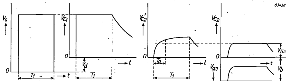
Fig. 7. Various voltages in the circuit of fig. 5, as functions of the time t , for a fortissimo passage (duration T_1 ; the revolution time of the record is T_0 ). V_s = signal voltage. V_{C1} = voltage across capacitor C_1 . The voltage across C_2 would be as that shown for V_{C2} if no limiter were present; with the limiter the voltage is as shown for V_{C2} . The voltage between grid and cathode of the reactance tube is V_{g3} ; this voltage determines the frequency of the oscillator.
