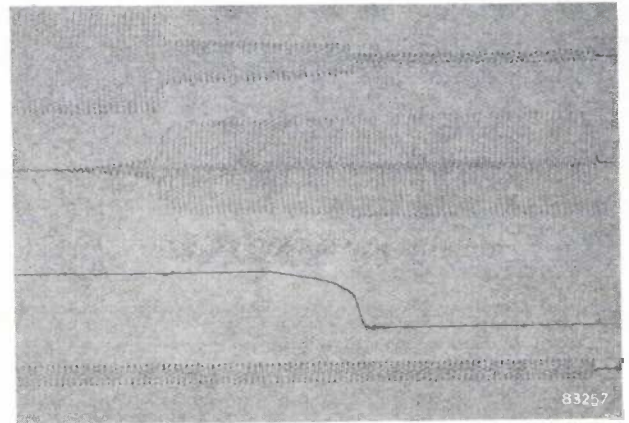
Fig. 9. Diagram recorded during the welding of a \frac{1}{2} -inch stud. Starting at the top we have, plotted against time: the voltage, the current, the displacement of the stud, and a constant 50 c/s A.C. voltage which serves as a time scale.
