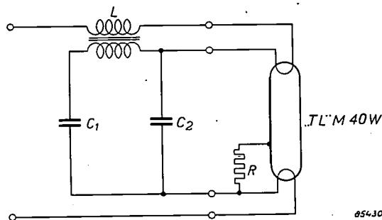
Fig. 4. Circuit diagram of ballast for "TL" 40 W lamp. The two coils L on one core possess a certain leakage. C_1 resonance capacitor. C_2 capacitor for interference suppression. R resistor of 1 M \Omega connecting the conductive strip to one of the electrodes.
