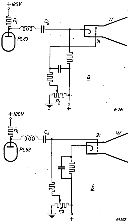
Fig. 10. Control of the picture tube W (with control grid, g_1 ), a) with negative modulation, b) with positive modulation. A double-pole switch (not shown) makes the change from one to the other. R_1 anode resistor of the video tube PL83 . C_5 coupling condenser. P_2 brightness control.
