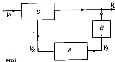
Fig. 7. Block diagram of a stabilizer with feedback. The deviation of V_u from its nominal value is converted into a voltage V_1 by the detecting device B . This error voltage is amplified by A and is used for regulating the output voltage by means of the controller C .
