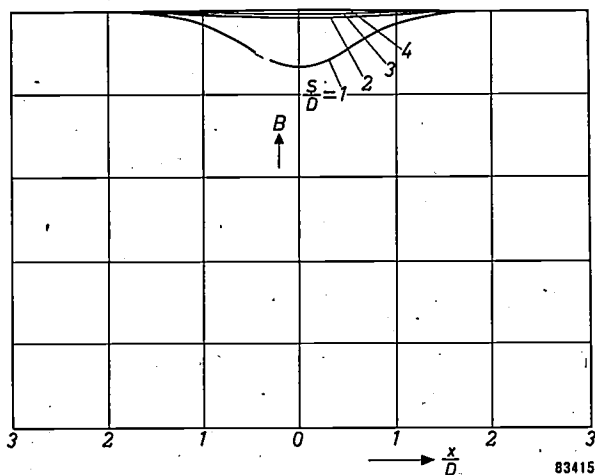
Fig. 7. Variation along the x -axis, see fig. 6, of the magnetic induction B , for lenses with differing values of S/D (the change of field with respect to x/D depends only on this ratio). It has been assumed that each lens is excited so that the maximum induction occurring in the gap reaches a given value (at which no troublesome saturation of the steel of the pole pieces occurs).
