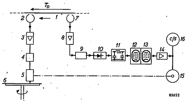
Fig. 4. Block diagram of the equipment for transferring the magnetic recording (1) to a lacquer disc (6) via replay head 2, amplifier 3, corrective network 4 and groove-cutter 5. The equipment for variable groove pitch is on the right: 7 auxiliary replay head, situated about one revolution ( T_0 ) of the disc ahead of head 2; the signal from 7 passes through amplifier 8, filter 9, rectifier 10 and delay network 11 to the reactance tube 12. The latter regulates the frequency of a valve oscillator 13, which supplies a synchronous motor 15 via an amplifier 14; the synchronous motor displaces the groove-cutter radially; 16 frequency meter.
