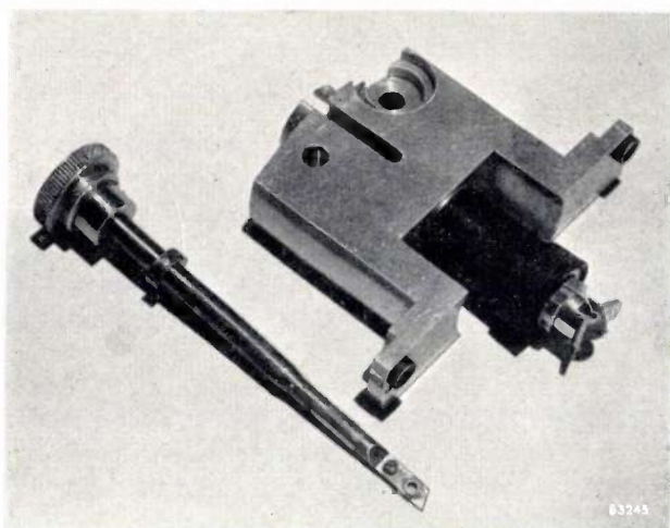
Fig. 15. The specimen stage and specimen holder (left). The cylindrical central section of the specimen stage contains a vacuum lock through which the specimen holder is inserted into the microscope tube.
