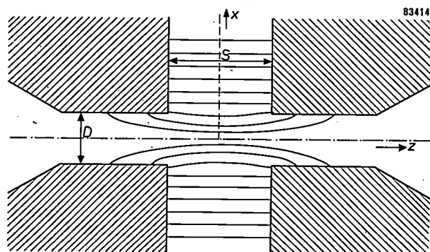
Fig. 6. The configuration of a magnetic lens is characterised by the diameter D of the bore through which the electrons pass ( z -direction), and the width S of the gap between the pole pieces.
