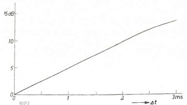
Fig. 10. Differences in intensity (in dB) plotted against the phase differences \Delta t which produce the same angular displacement of the sound image.
