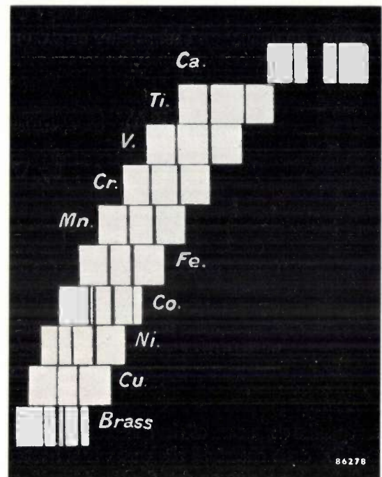
Fig. 2. X-ray spectra of a number of elements photographed by Moseley. (From Phil. Mag. 26, 1024, 1913.)
