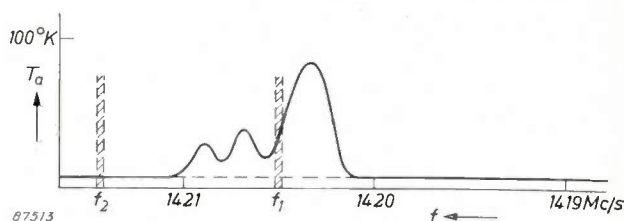
Fig. 7. Schematic representation of a line profile, i.e. of the average intensity (expressed as antenna temperature T_a ) of the Galactic radiation as a function of the frequency near the 21 cm line.
