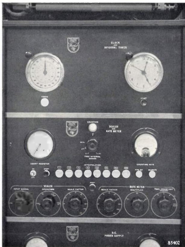
Fig. 13. Front view of the panels which contain the scaling and rate meter circuits (below, cf. also fig. 1), the interval timer and clock (above).
