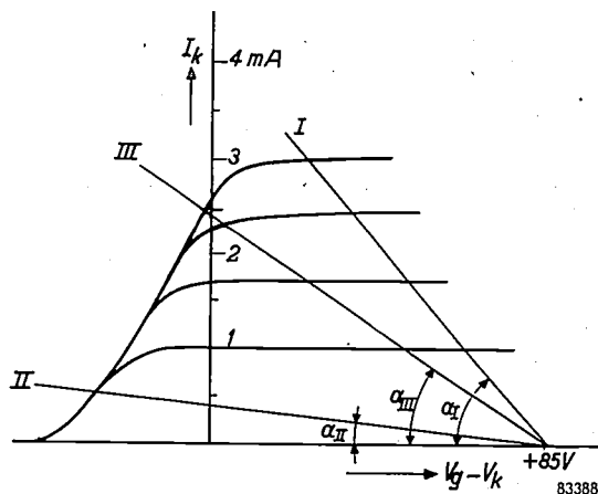
Fig. 4. The current I_k through the cathode circuit of the ionization manometer shown as a function of the voltage V_g - V_k between the control grid and the cathode, for various values of the saturation emission of the cathode, and at constant control-grid and anode potential (respectively +85 V and +255 V relative to earth). The working point of the triode so formed is given in the usual way by the point of intersection of the relevant characteristic with a straight line (the load line), passing through the point +85 V on the abscissa. (This latter point is in reality considerably further to the right than shown in this schematic diagram.) The load line makes an angle \alpha with the abscissa; \cot \alpha is a measure of the resistance between cathode and earth. If this resistance is low ( R_2 connected in parallel to R_1 , and R_3 completely short-circuited, see fig. 3 ), then the saturation current flows through the tube (load line I). If R_2 is switched off, \cot \alpha_{II} = R_1 + R_3 ; the cathode current can now be accurately adjusted at 0.5 mA by means of R_3 , (load line II). If R_2 is switched out, the load line can be placed in position III by means of R_3 , provided the saturation emission is sufficient; the anode current now amounts to 2.5 mA.
