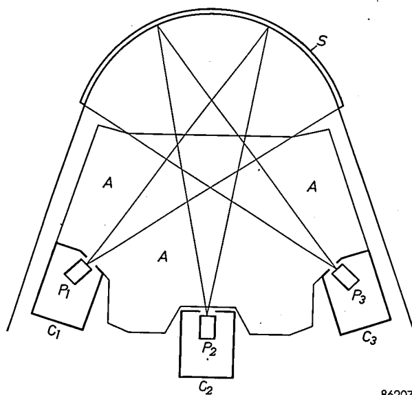
Fig. 1. Schematic diagram of the Cinerama system, showing the arrangement of the screen S , the three projectors P 1 , P 2 and P 3 in their projection rooms C 1 , C 2 and C 3 , and the audience A . 86207
