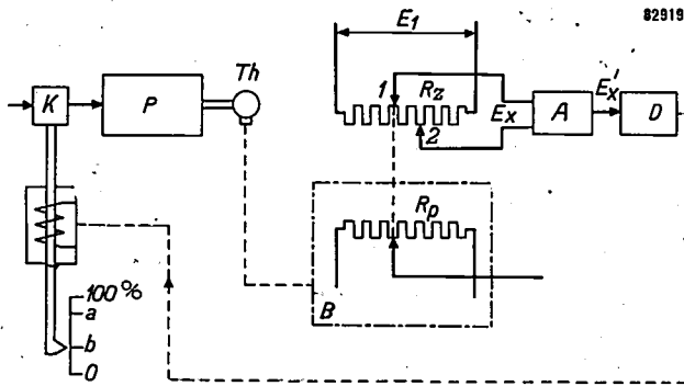
Fig. 3. Circuit for two-step control of the temperature of a furnace. A amplifier; D phase-sensitive detector. The other letters have the same significance as in figs. 1 and 2 .
