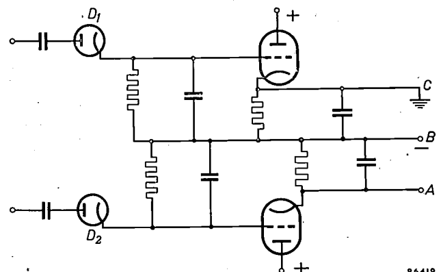
Fig. 8. The output stage of the circuit. The voltage at A is fed to the control electrode of the transmitting valve.
