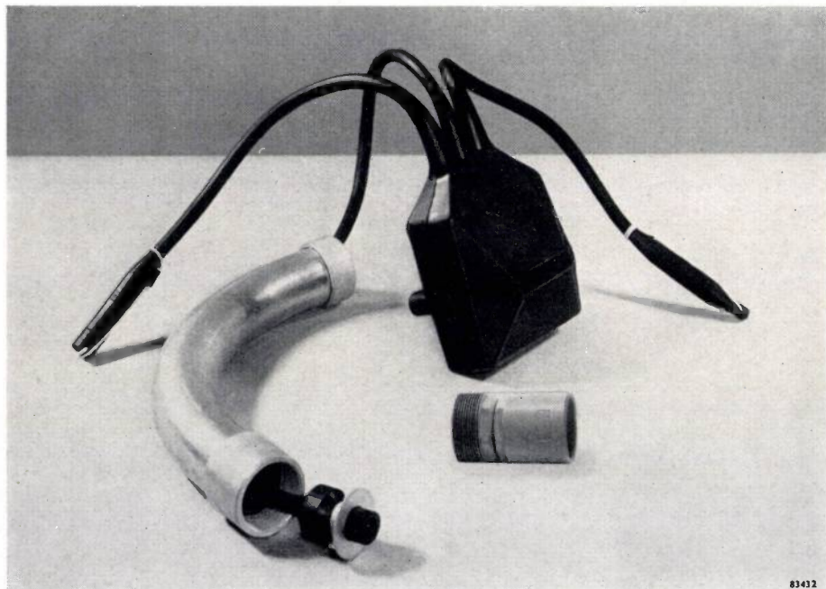
Fig. 15. 200 W, 6.6 A lamp transformer for circuits operating with 5000 V supply. It is completely enclosed in rubber, moulded in one piece with the insulation of the leads. The secondary lead (passing through the curved pipe) is fitted with a lamp socket. If the light is knocked over, the safety joint, that is, the small weakened pipe seen in front of the transformer, breaks (see page 282 of the article referred to in note 1 ) and the plug is pulled out of the secondary socket. The leads on the extreme right and left are the primary leads. Note the end sleeves employed to protect them from corrosion in storage or in transit.
