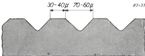
Fig. 2. Cross-section of unmodulated grooves in a long-playing record.
