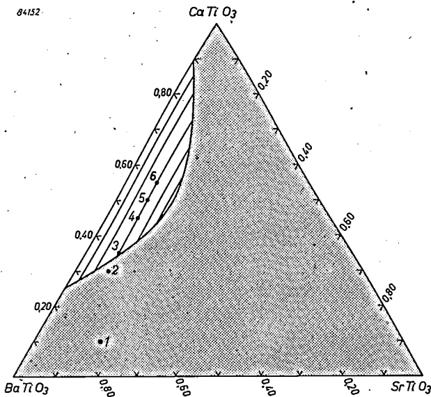
Fig. 5. Phase diagram at 1350 °C of the combination \text{BaTiO}_3 - \text{SrTiO}_3 - \text{CaTiO}_3 . \text{BaTiO}_3 and \text{CaTiO}_3 are only partly miscible: random mixtures of these two materials separate out into two equilibrium phases, viz. mixed crystals of 26% \text{CaTiO}_3 + 74% \text{BaTiO}_3 , and mixed crystals of 89% \text{CaTiO}_3 + 11% \text{BaTiO}_3 . The miscibility is improved by the addition of \text{SrTiO}_3 . In the segregation region, the straight lines (connodes) join the mixed crystals which are in equilibrium with each other.
