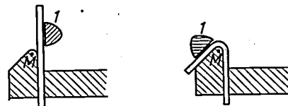
Fig. 7. Bend test employing special tools. The axis of rotation of thrust block I coincides with the centre of curvature M of the curved member over which the specimen is bent.
