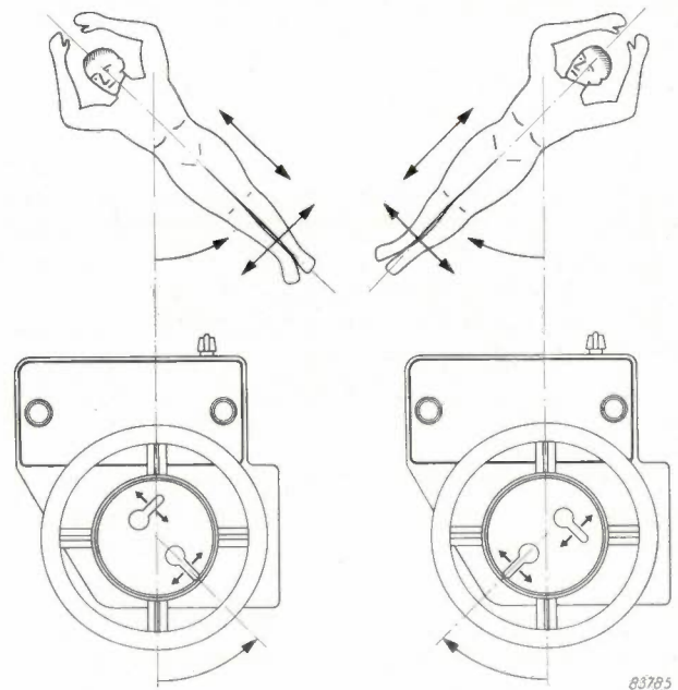
Fig. 8. The hub of the hand wheel driven by a small motor housed in the control box, rotates with the patient so as to maintain the switches in the same positions relative to the patient-movements controlled by them.
