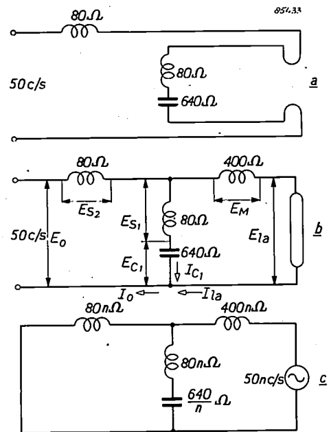
Fig. 5. Impedances occurring in the circuit of fig. 4 : a) before lamp ignites, frequency 50 c/s; b) with lamp ignited, frequency 50 c/s; c) with lamp ignited, frequency 50 n c/s. Owing to the impedance of 80 n \Omega in series with the supply, the mains current is distorted only very slightly.
