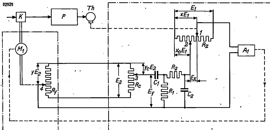
Fig. 13. Layout of circuit for proportional, integral and derivative control.
