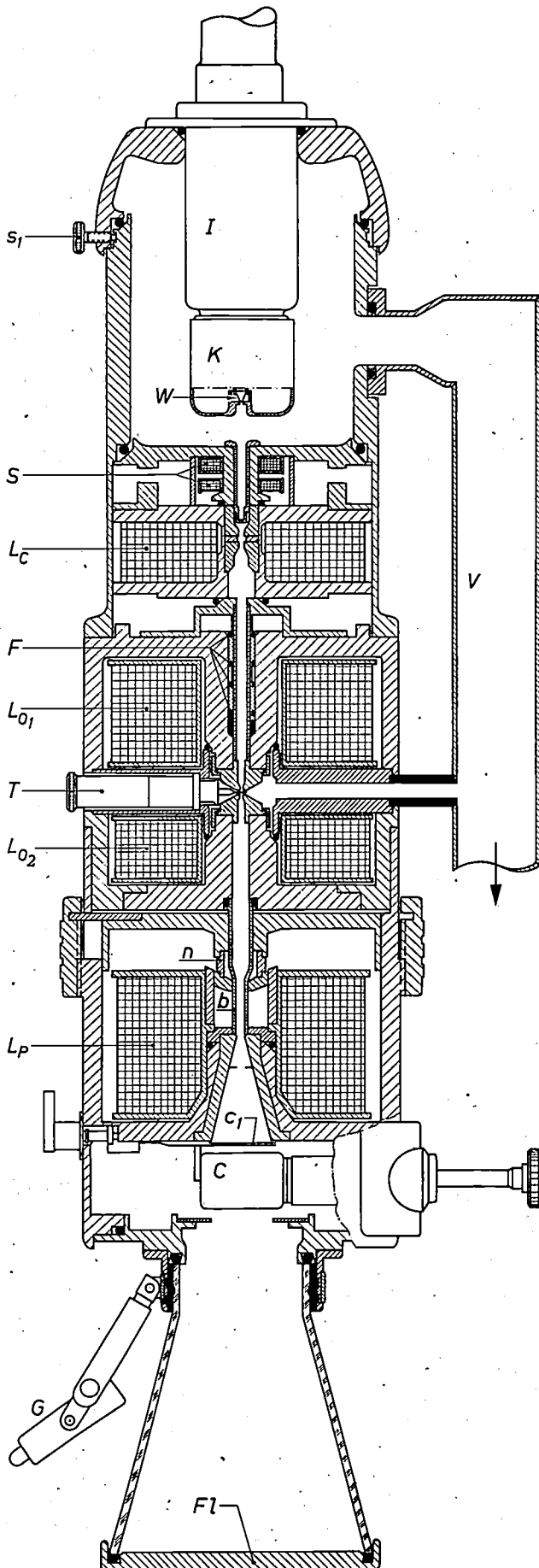
Fig. 12. Cross-section (simplified) of the microscope tube of the EM 75 kV. K cathode with filament W; S deflection coils for centring the electron beam Lc condenser lens; L 01 , L 02 ; objective lens composed of two parts with specimen stage T; F auxiliary coils to assist in the focusing; Lp projector lens, n non-magnetic spacer, b brass tube carrying pole-pieces; C camera with operating rod (turned through 90° for reasons of clarity), c 1 shutter; Fl fluorescent screen; G observing lens; V vacuum connection. The cap of the tube with the bushing insulator I, which carries the cathode, can be moved laterally by means of three screws (s 1 etc.) for centring of a changed filament.
