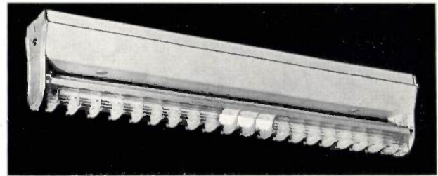
Fig. 12. Method of reducing the high brightness of the gap of a "TL" F lamp by means of refracting side-panels. The light radiated sideways is refracted downwards. In the photograph (a) a portion of a side-panel in the centre has been removed. It can be seen that the brightness is much greater there than elsewhere. The principle is illustrated in the diagram (b).
