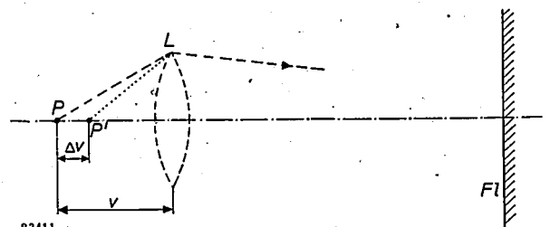
Fig. 3. If the acceleration voltage of the electrons or the excitation current of the objective L vary, the image on the fluorescent screen FI is not that of the object plane P , but is the image of a plane P' displaced by \Delta v from the object ( v is the distance between object and objective lens).
