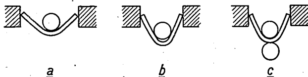
Fig. 5. Specimen from fig. 4 arranged in vice for bending through angles greater than 90^\circ . The jaws of the vice are moved toward each other. a ) As in fig. 4c , unwanted bending occurs; the mandrel also becomes displaced ( b ) causing too sharp a bend. Supporting the mandrel ( c ) avoids displacement but the specimen is then no longer subjected to a pure bending.
