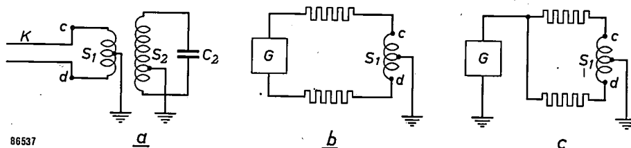
Fig. 10. a) Input of an F.M. receiver showing the feeder K of the built-in dipole. S_1 , S_2 and C_2 as in fig. 1. b) and c). Checking for symmetry. G signal generator. The millivoltmeter connected in the set should show a deflection no greater in case (c) then it was in (b), when the generator voltage is made 10 times smaller than in the latter case.
