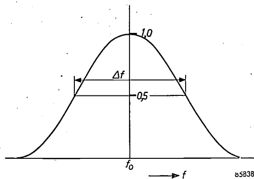
Fig. 5. Sinusoidal band-pass response of the I.F. filter.
