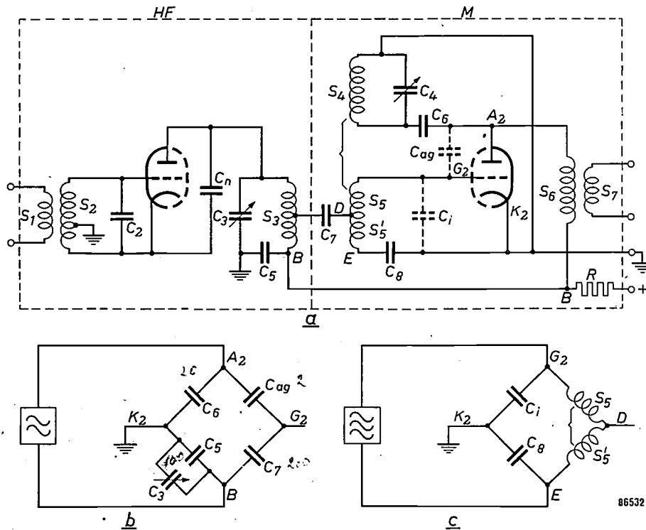
Fig. 2. a) Simplified diagram of high frequency amplifier HF and mixing stage M. For S_1, S_2, S_3, C_2, C_3 and C_n see figure 1. A_2, G_2, K_2 are electrodes of the other half of the double triode ECC 85. S_4-C_4 oscillator circuit. S_5 + S'_5 feed-back coil. S_6-C_6 primary circuit of the first I.F. band-pass filter. S_7 coupling coil. C_1 input capacitance. b) Bridge circuit in circuit (a) which, at the correct value of C_5 , causes a reduction in the damping of the band-pass filter. c) Second bridge circuit, incorporated in (a) which, at the correct value of C_8 , ensures that no voltage at the oscillator frequency appears at point D, so that there is no radiation.
