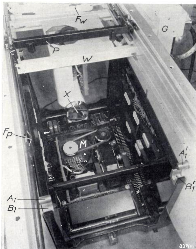
Fig. 9. Base of the "Symmetrix" table seen during assembly. M centrally mounted electric motor to drive the table; A_1 , A_1' spindles and B_1 , B_1' their associated open bushes. In B_1' there is a feeler switch which causes the table to rotate at the lower speed when passing through the horizontal position; the switch operates through a relay system which is visible in the side wall of the base. X X-ray tube; W tube carriage with "concertina" cable ( F_w ); G mounting for viewing system; P frame of Potter-Bucky diaphragm, with concertina cable ( F_p ).
