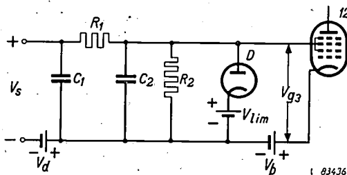
Fig. 5. Circuit of the delay network 11 of fig. 4. V_s input signal (varying direct voltage). V_d threshold voltage. C_1 capacitor from which capacitor C_2 is given a delayed charge via resistor R_1 . R_2 discharge resistor. The diode D with bias V_{lim} forms the limiter. V_b grid bias. 12 reactance tube.
