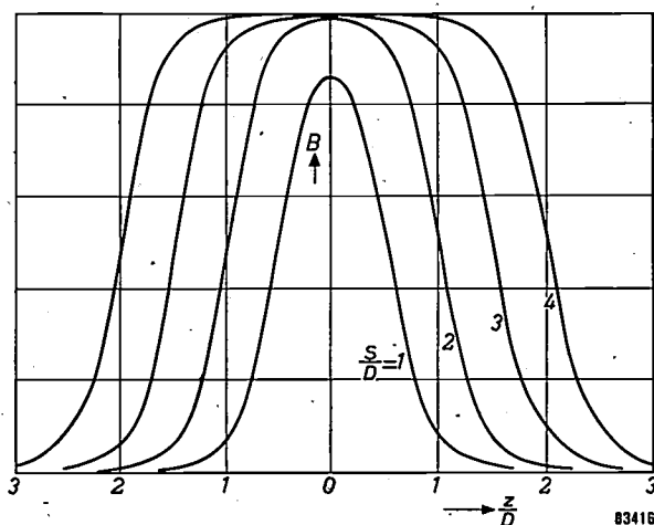
Fig. 8. Variation of the magnetic induction B along the z -axis, for various values of S/D . The induction at z = 0 is equal to that at x = 0 in fig. 7; the field here is at a saddle point.
