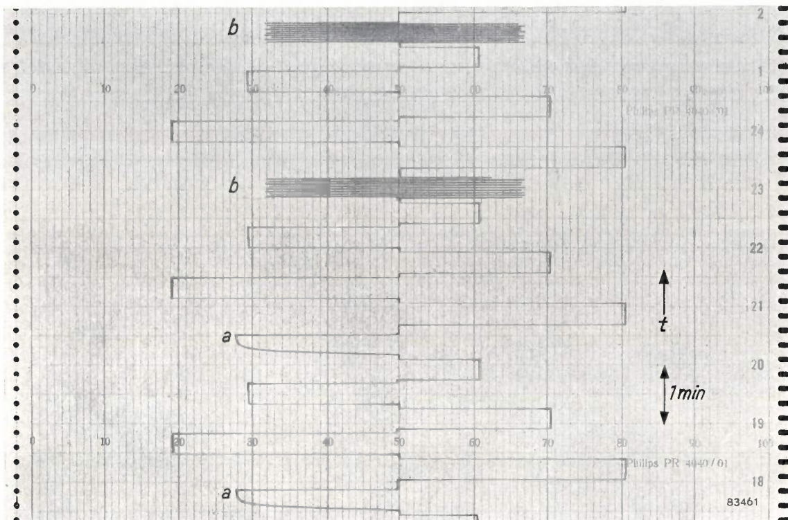
Fig. 14. Section of strip chart, showing the conditions during slowing down of a turbine. At a the eccentricity was recorded with the detector Det (fig. 13) functioning (rotor speed still above 48 r.p.m.); at b without this detector (rotor speed below 48 r.p.m.): the indicator now follows the demodulated alternating voltage. The intermediate rectangular deflections relate to changes in length.
