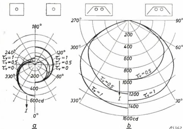
Fig. 6. a) The light distribution curves for "TL" F lamps with dirt layers on the upper half having the same values of \tau_v as in fig. 2a are shown on the left. The slot is directed downwards. For comparison purposes, the curves of fig. 2a for the normal lamp are reproduced on the right. b) The same for a two-lamp trough fitting with dirty "TL" F lamps. The curves on the right of the figure are for normal "TL" lamps as already given in fig. 2b.
