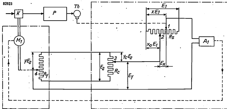
Fig. 7. Schematic lay-out of a proportional control system. The right-hand part (surrounded by chain line) is situated near the measuring element, the left-hand part near the correcting element (valve).
