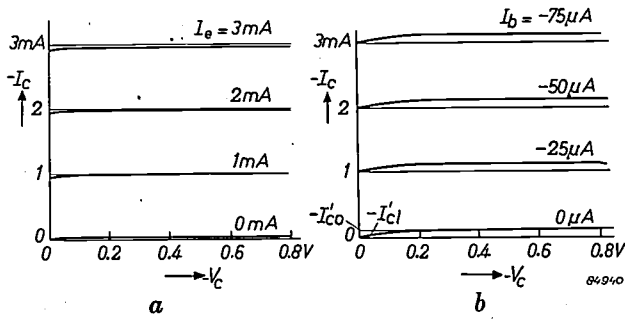
Fig. 9. Theoretical characteristics of a transistor: collector current I_c as function of the collector voltage V_c for various values of the input current. According to the sign convention (fig. 4) V_c and I_c are negative: -V_c and -I_c have therefore been plotted.
