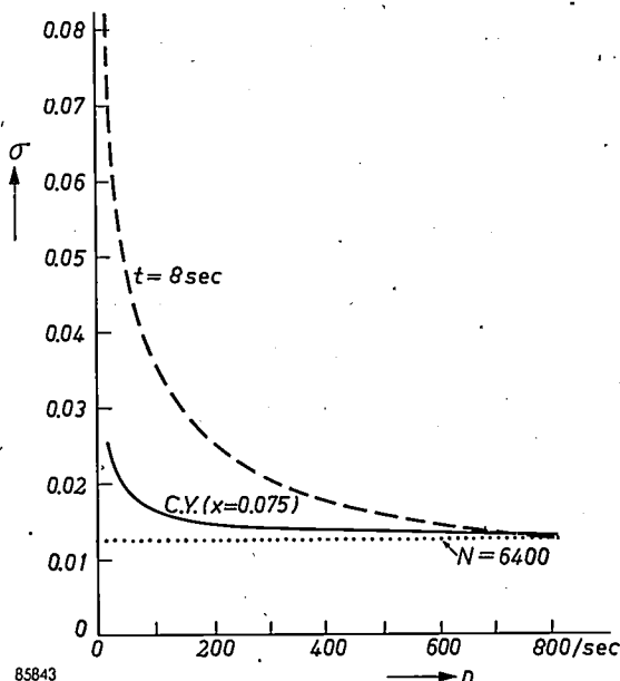
Fig. 16. The standard deviation \sigma as a function of the counting rate n , for the Cooke-Yarborough method (C.Y.), for fixed time measurements with t = 8 sec (---) and for fixed count measurements with N = 6400 (.....).
