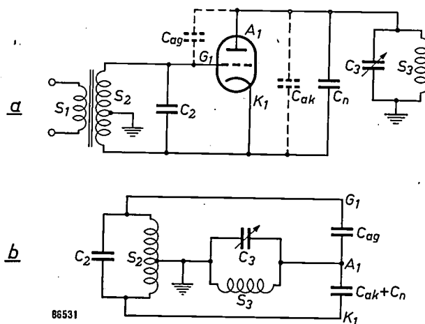
Fig. 1. a) Diagram of the H.F. amplifier in "Zwischenbasis" circuit. b) Equivalent circuit. S_1 primary coil. S_2 - C_2 secondary circuit, tuned to a fixed frequency at the middle of the frequency range (94 Mc/s). A_1 anode, G_1 grid and K_1 cathode of one half of the double triode ECC 85. S_3 - C_3 output circuit. C_{ag} grid-anode capacitance. C_{ak} anode-cathode capacitance. C_n neutralizing capacitance. The power supplies are not shown.
