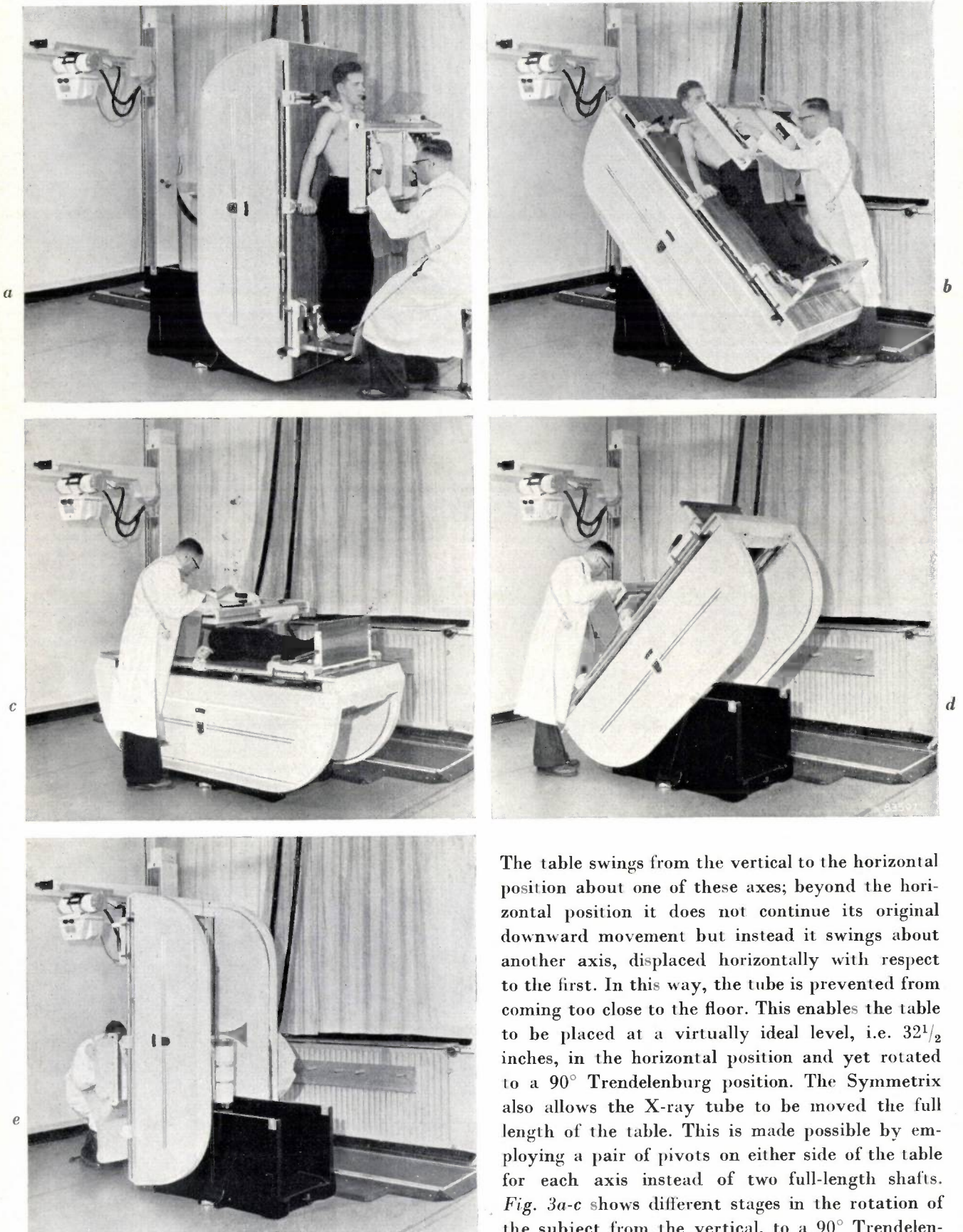
Fig. 3. The "Symmetrix" examination table can be rotated from the one vertical position (a) to the horizontal position (c) and thence to the opposite vertical position (e). In spite of this, the surface of the table in the horizontal position is only 32\frac{1}{2} inches above the floor.
