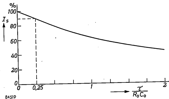
Fig. 9. Signal current ( I_s ; on relative scale), plotted as a function of \tau/R_0C_0 . The values of R_0 and C_0 are chosen so as to give an I_s equal to 90% of the maximum value ( \tau/R_0C_0 = 0.25 )
