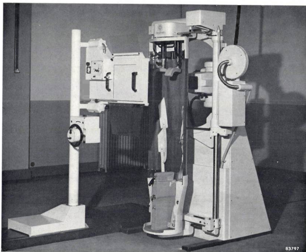
Fig. 1. The "Müller" UGX diagnostic X-ray unit. The column seen on the left of the picture, running on floor rails, carries the viewing system and the control box; a cradle of thin wood, to carry the patient, supported by a frame mounted on the base is seen in the centre of the picture; on the right of the cradle and base is the X-ray tube, on a separate stand, also on floor rails.
