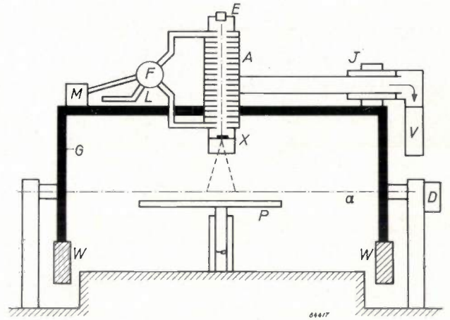
Fig. 2. Schematic representation of the machine shown in fig. 1 . A is the accelerator proper (corrugated waveguide 1 metre long), mounted in gantry G rotatable about the axis a by means of an oil motor D . E electron gun, X X-ray head, M magnetron, F feedback bridge, V diffusion pump, J rotating vacuum joint, W counterweights, P patient's couch, L water load.
