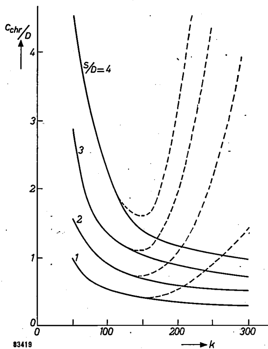
Fig. 11. Chromatic blur for a number of lenses with different S/D , as a function of the excitation factor k . C_{chr} is the proportionality factor between \delta_g and 2\alpha_0 , which must be substituted in equation (4) for \Delta v in more accurate calculations. C_{chr}/D has been plotted to give generally applicable curves. The acceleration voltage is here fixed at 80 kV. These curves may only be used up to that value of k which gives the maximum permissible induction in the gap between the pole pieces.
