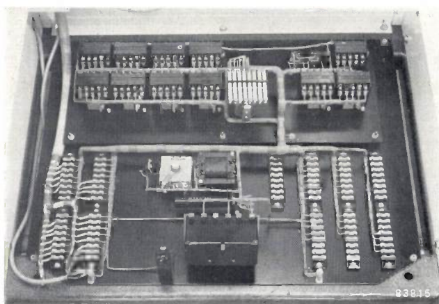
Fig. 9. Relay system, housed in the base of the apparatus, through which the limit contacts, "memory" switches, etc., control the various movements.
