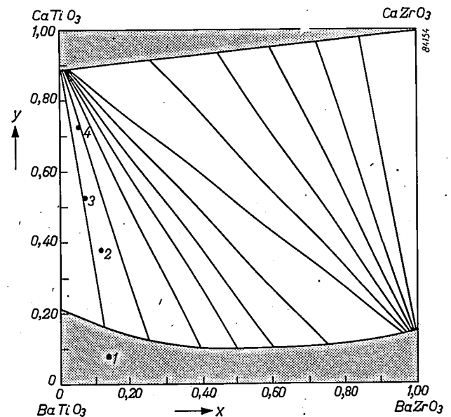
Fig. 7. Phase diagram at 1300 °C of the system \text{BaTiO}_3 - \text{CaTiO}_3 - \text{CaZrO}_3 - \text{BaZrO}_3 with two perovskite phases (shaded areas). The ratio \text{Zr}/\text{Ti} is x/(1-x) , the ratio \text{Ca}/\text{Ba} is y/(1-y) . The straight lines in the segregation region are the connodes. From the direction of the connodes it can be seen that the combination \text{BaZrO}_3 + \text{CaTiO}_3 is more stable than the combination \text{BaTiO}_3 + \text{CaZrO}_3 .
