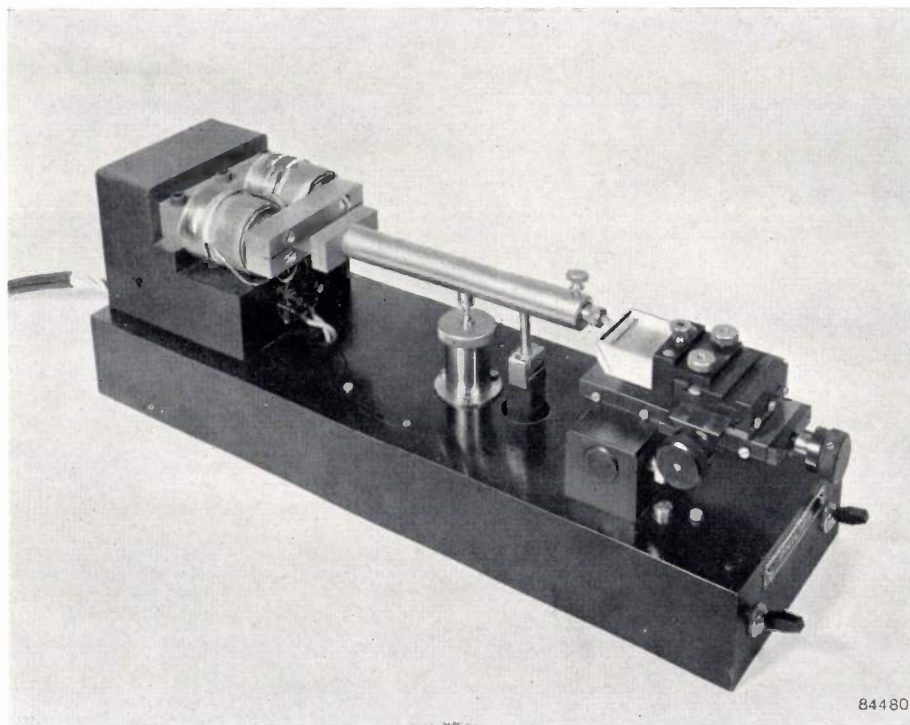
Fig. 1. The new ultramicrotome designed at Eindhoven.
