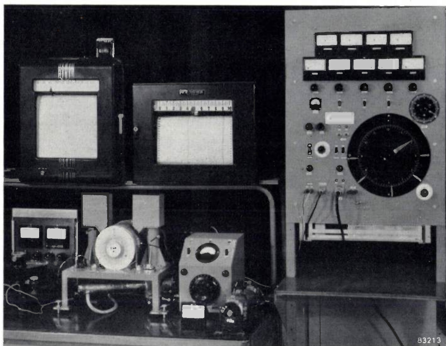
Fig. 4. Complete arrangement for the objective determination of the gloss point. Top left is the X-Y recorder, and beside it an instrument which records the temperature as a function of time (for checking the heating-rate of the furnace; see fig. 7). Below the recorders is the furnace, with meters on either side giving direct indications of the separate photo-electric currents and the temperature and for adjusting the furnace power. At the right is the programming apparatus for controlling the furnace temperature.
