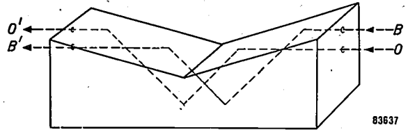
Fig. 6. Prism as described by J. Taylor (Brit. J. Phot. 14, 348, 1867); it produces three reflections, thus exchanging the top and bottom of the image. If the prism be rotated with an angular velocity \omega about direction OB' , the image in the field of view will rotate with double this angular velocity, i.e. 2\omega .
