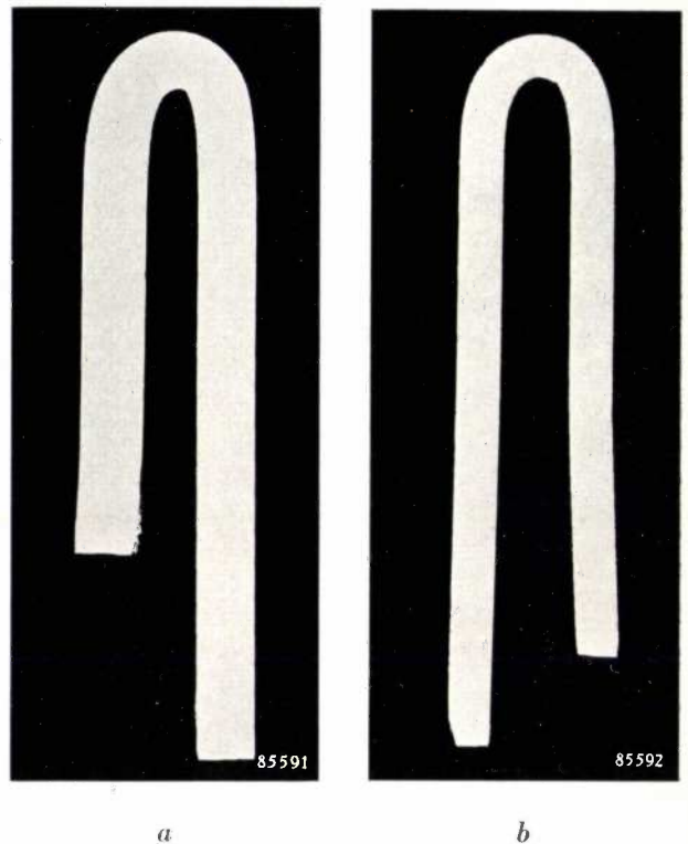
Fig. 3. a) Section of a test specimen of chrome steel, bent through 180° by the machine shown in fig. 1 (tensile strength of specimen approx. 65 kg/mm 2 ; specimen thickness d = 1.9 mm; diameter of radius plate D = 0.95 mm; thus D/d = 0.5 ). b) Section of a test specimen of mild steel (tensile strength approx. 40 kg/mm 2 ; d = 1.0 mm; D = 1.2 mm, and D/d = 1.2 ).
