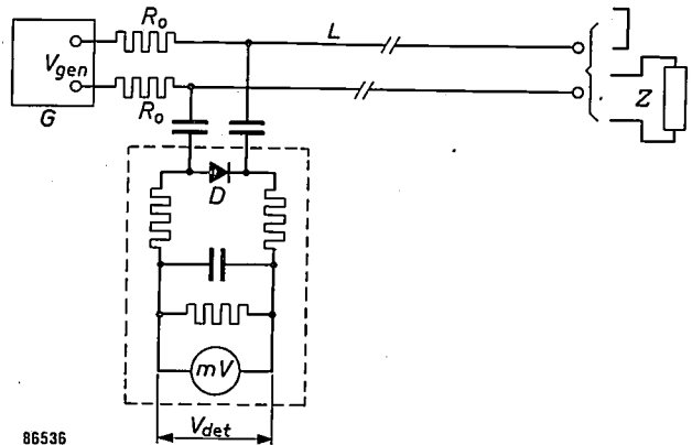
Fig. 9. Circuit for measuring impedances. G is a signal generator with adjustable frequency and voltage, amplitude-modulated. L is a long transmission line. Z is the impedance to be measured, D the detector and mV the electronic millivoltmeter.
