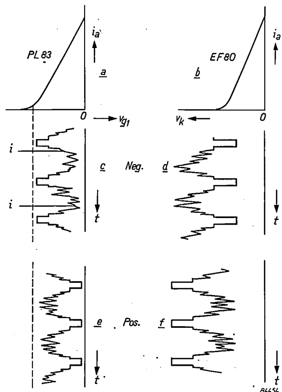
Fig. 11. a) Anode current i_a as a function of the control grid voltage v_{g1} , for the video tube PL83 . b) i_a as function of the cathode voltage v_k (with earthed grid), for the control tube EF80 . c) Control grid voltage of the PL83 , and d) cathode voltage of the EF80 as a function of the time t , with negative picture-modulation; e) and f) the same for positive picture-modulation.
