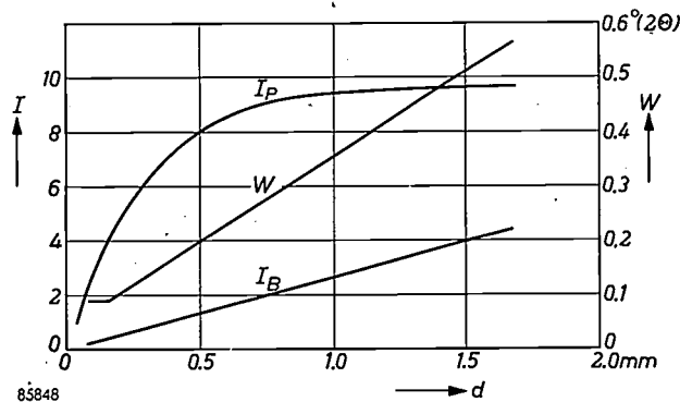
Fig. 18. When a diffraction line is scanned with receiving slits of increasing widths d , the recorded peak intensity I_P (with background subtracted) also will increase. When the receiving slit becomes wider than the line, the intensity no longer increases and the peak value indicates the integrated line intensity. The background I_B and the width W (degrees 2\theta at half peak height) of the recorded line profile continue to increase with receiving slit width. These curves were obtained using the 111 line of silicon with Cu K\beta radiation using an angular aperture 2\alpha = 1^\circ . Wider lines and K\alpha -doublet separation will change the given values.
