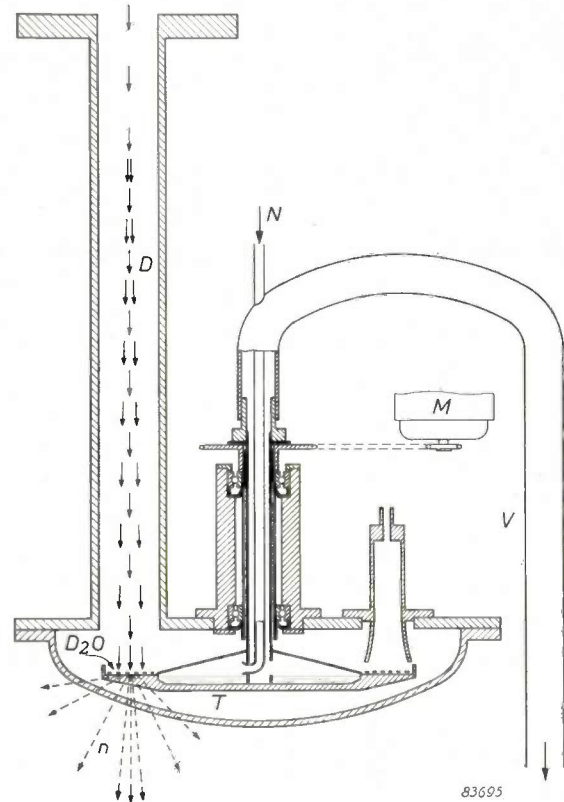
Fig. 3. Cross-section of the lower end of the acceleration tube, with hollow target T and its hollow axis of rotation. D deuteron ion beam, D_2O layer of heavy ice, n neutrons produced, M electric motor, N supply of liquid nitrogen, V chimney for extracting the evaporated nitrogen.
