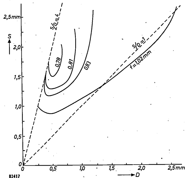
Fig. 9. Focal length f , calculated for lenses of various bore D and gap S when the lens is excited so as to give a maximum induction in the gap of 1.8 \text{ Wb/m}^2 . The acceleration voltage of the electrons is fixed at 75 kV. Points with equal f have been joined in the diagram. (The curves turn upwards slightly at the left-hand side and appear to bend backwards a little at the right; it is not clear whether these effects are real or arise from the approximations in the calculation, but they are of little importance in the S - D range under consideration.
