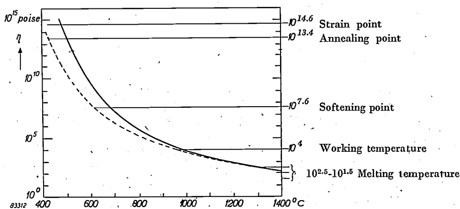
Fig. 1. The viscosity \eta (in poise) of two types of glass as a function of the temperature. The full curve applies to soda glass, the dashed curve to lead glass. For processing, certain values of \eta are required, which thus determine the processing temperatures.
