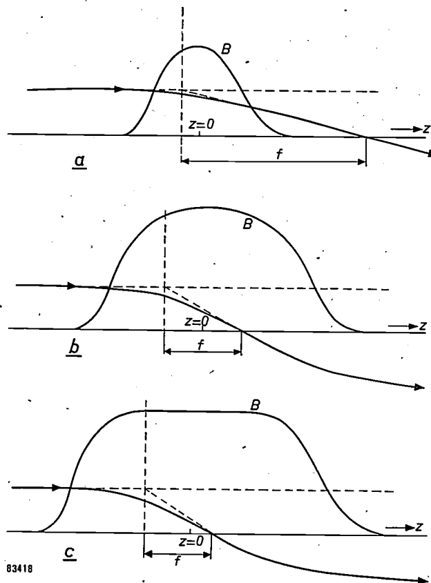
Fig. 10. Path of an electron coming from the left and entering the magnetic field of an electron lens parallel to the axis. The change of induction B is also shown. a) Relatively "thin" lens ( S/D small). b) Longer lens. c) Very long lens.
