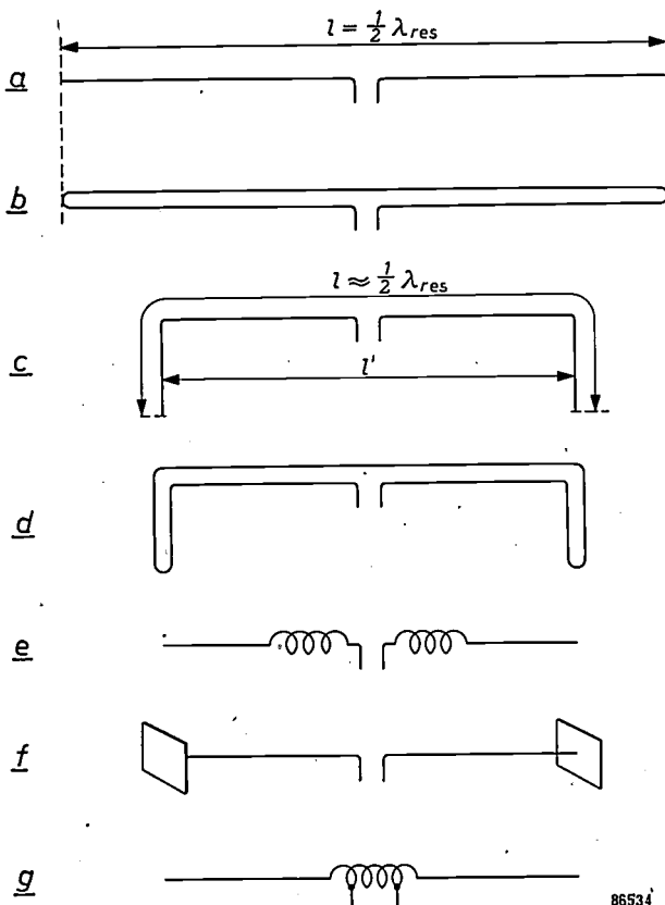
Fig. 7. Forms of dipole aerials. a) Normal dipole; length l equal to half the resonance wave length \lambda_{res} . b) Folded dipole. In order to fit the dipole into a cabinet of length l' < l , it can either be bent ( c, d ), or provided with two coils ( e ), two end plates ( f ) or one coil ( g ).
