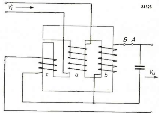
Fig. 5. Magnetic stabilizer with one core. The right limb becomes saturated earlier than the left limb with the air gap.
