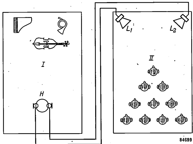
Fig. 3. Stereophony. Each microphone on the artificial head (H) in hall I is connected to its own loudspeaker (L 1 , L 2 ) in hall II. Here too, the audience in II receives a spatial impression of the sound.
