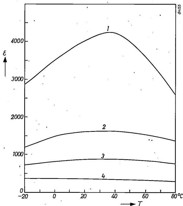
Fig. 8. \epsilon - T curves for sintered specimens prepared from BaCO 3 , CaCO 3 , TiO 2 and ZrO 2 , corresponding to the compositions 1 to 4 in fig. 7. Here too, the strong flattening action of the increasing proportions of the phase rich in CaTiO 3 is demonstrated.
