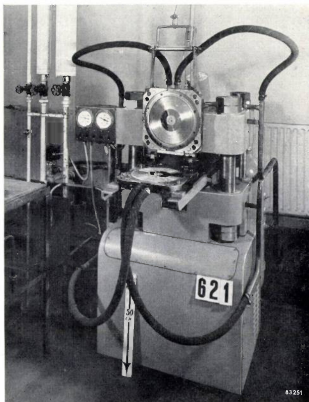
Fig. 11. Gramophone record press shown open.
