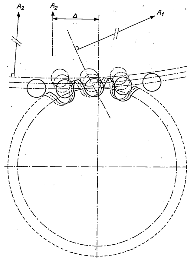
Fig. 8. The teeth of one of the rotating sprocket wheels and the rollers of the sprocket engaging with it (rotation about axis A 1 ), in three consecutive positions. Instead of being vertically below axis A 2 , the sprocket wheel axis is displaced a certain distance ( \Delta ) inwards.
