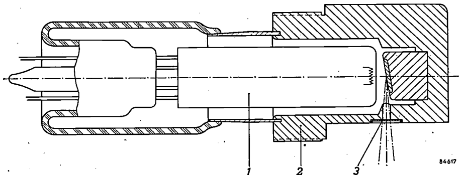
Fig. 1. Cross-section of the 5 kV X-ray tube used in the CMR 5 apparatus. 1 cathode with tungsten filament; 2 anode with tungsten target; 3 beryllium window, 50 \mu thick. Length of tube approximately 8 cm.
