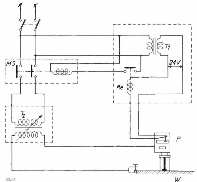
Fig. 8. Circuit of the electrical equipment employed in the new stud welding process with welding cartridges. This process enables alternating current to be used, which means that ordinary welding transformers (open-circuit voltage roughly 75 V) can be employed. A micro-switch built into the grip of the welding gun P operates the coil of a relay Re . Since the energising voltage of this relay is only 24 V (transformer T 1 ), the micro-switch can be touched without risk, even when defective. The relay operates a magnetic switch MS controlling the welding transformer T 2 . W is the workpiece to which the stud is to be welded.
