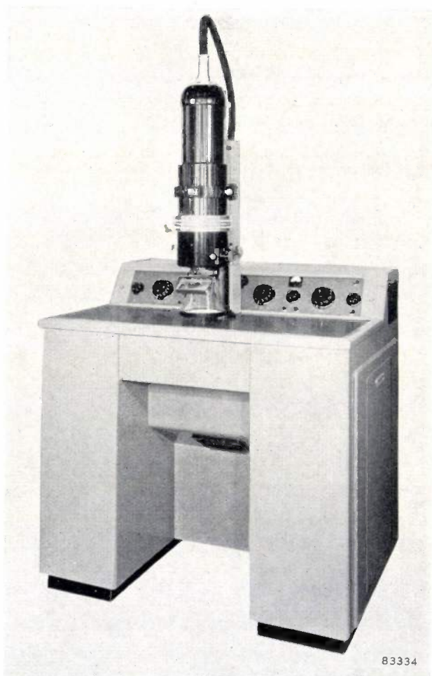
Fig. 1. The small electron microscope EM 75 kV (for 75 kilovolts, type 11981). The electron beam traverses the vertically mounted microscope tube from top to bottom. The desk houses the pump installation and the entire electrical equipment.
