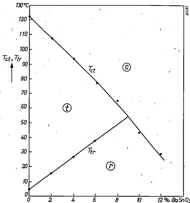
Fig. 4. The effect of BaSnO_3 on the transition points of BaTiO_3 (an almost similar figure applies for additions of BaZrO_3 ) c = region of cubic structure, t = tetragonal, r = rhombic.
