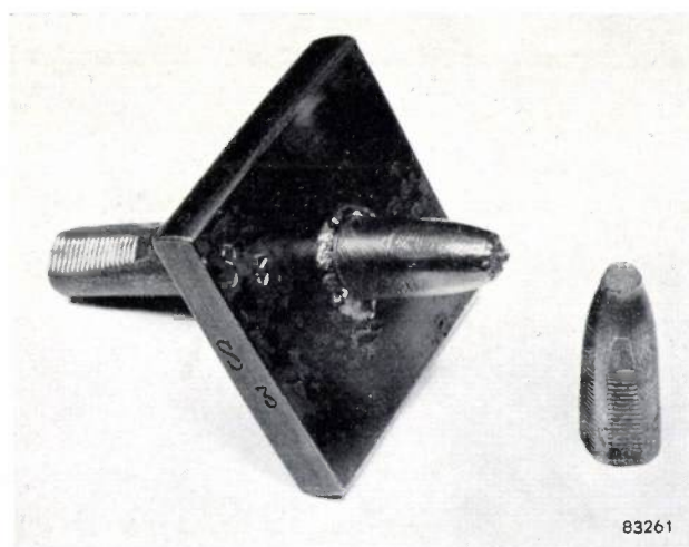
Fig. 14. a) Result of a tensile test on two studs welded end to end to opposite sides of a plate. b) Result of a fatigue test.
