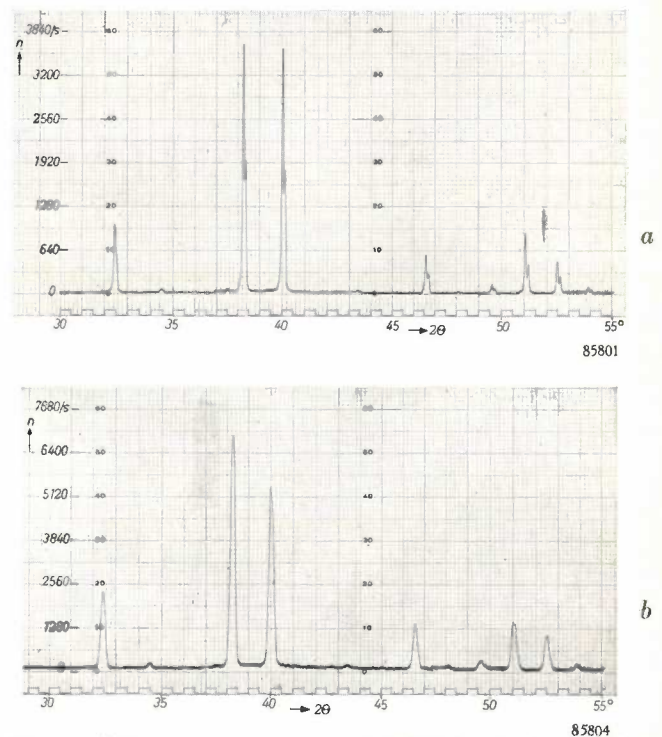
Fig. 9. Diffractometer pattern of \text{Sr}(\text{NO}_3)_2 obtained with \text{CuK}\alpha radiation, 30 kV peak, 20 mA. a) Recorded with 0.15 mm receiving slit at scanning speed v = \frac{1}{4}^\circ/\text{min} and with time constant T = 4 sec. b) Recorded with 0.60 mm receiving slit, v = 1^\circ/\text{min} and T = 2 sec. The total number of counts is approximately the same in both cases (92 290 and 88 260 respectively, after subtraction of background), but the angular resolution of record (b), which took only \frac{1}{4} of the time necessary for (a), is much poorer. Peak-to-background ratio for (a) 96.5, for (b) 42.7 (cf. fig. 18).
