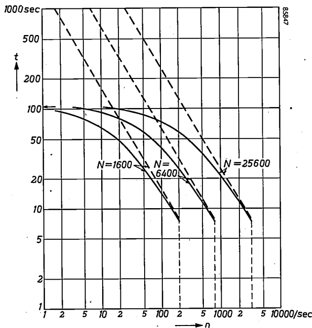
Fig. 15. Time t required to accumulate a number of counts N , in normal operation (dotted lines) and in the Cooke-Yarborough method (solid lines). The added pulse frequency f is 0.075 times the full scale counting rate.
