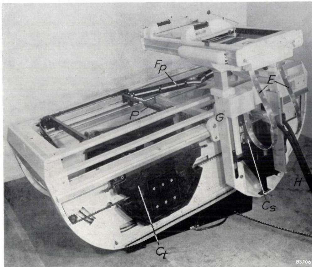
Fig. 10. The "Symmetrix" table during assembly. The table top, the side plates of the table and the cover plates of the viewing unit mounting G are not in position. C_s is the counterweight to balance the perpendicular movement of the viewing unit. One of the two heavier counterweights C_t employed to balance the movement of viewing unit and X-ray tube carriage along the table can be seen in the side wall of the table. H high-tension cables, passing through a lateral guide to the X-ray tube under the table; E flat multi-core cables connecting the controls on the viewing unit to the mounting; F_p concertina cable to connect the scatter grid P to the table (only the frame of P is shown).
