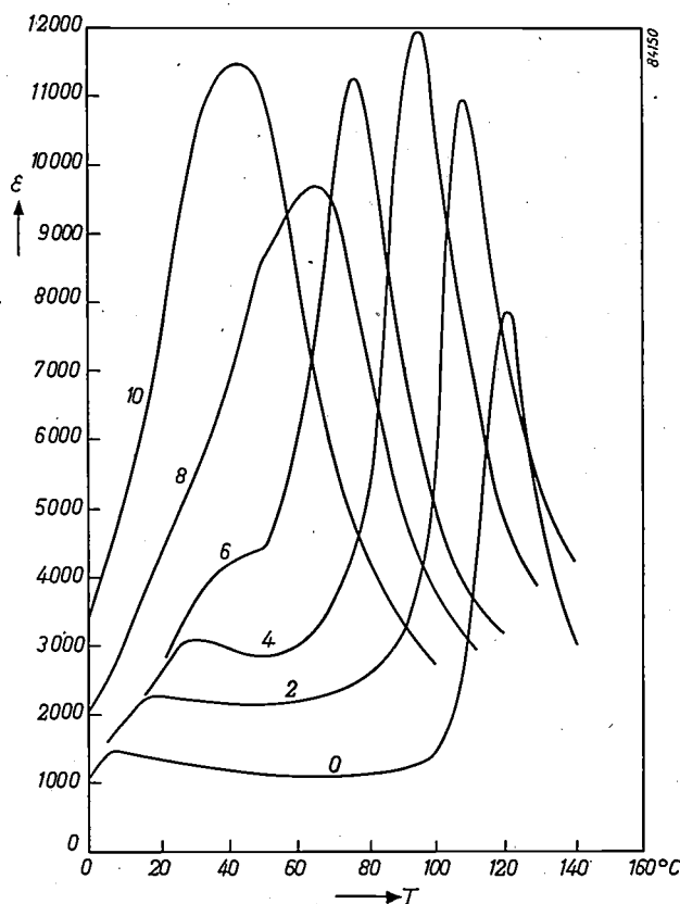
Fig. 3. \epsilon - T curves for mixed crystals of BaTiO 3 and BaSnO 3 . The figures beside the lines give the percentage of BaSnO 3 present. The mixed crystals have a higher \epsilon maximum than pure BaTiO 3 . For specimens where the first and second maxima lie close together (see fig. 4) a disturbance occurs which makes this effect less obvious.
