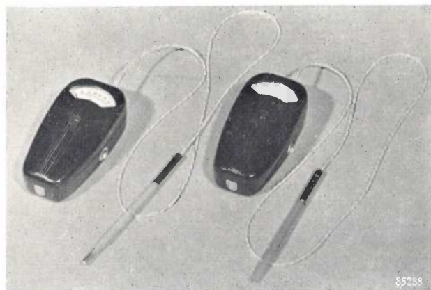
Fig. 1. Left, the electrical clinical thermometer, consisting of a probe and an indicating instrument, connected by a flex. The button visible on the right of the instrument is pressed in order to take a reading. The reading may be taken about 13 seconds after insertion of the probe. Right, the model for skin thermometry.
