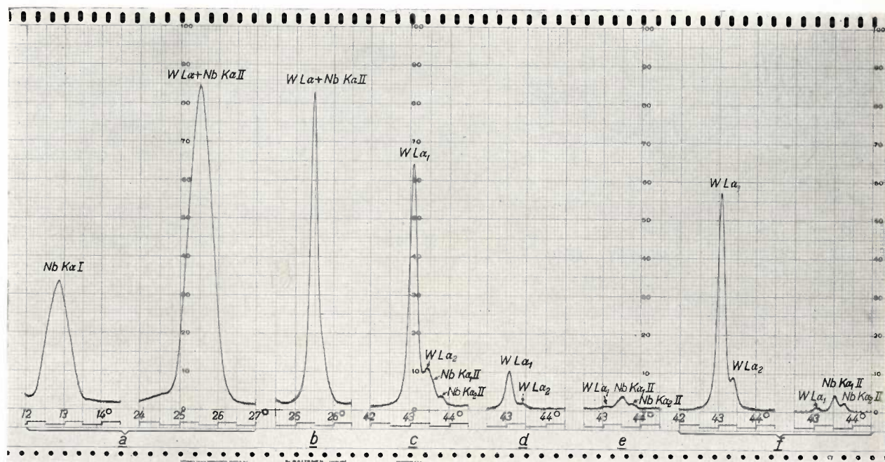
Fig. 19. Methods of separating overlapping spectral lines. The specimen contains WC 72%, TiC 10%, NbC 10%, Co 8%; i.e. approx. W 67.6% and Nb 8.9%. Tungsten target X-ray tube, 50 kV peak, 45 mA (except for method d , see below). Full scale intensity = 6400 counts/sec for (a) and 3200 counts/sec for (b-f). Scanning speed \frac{1}{2}^\circ per min, time constant 4 sec, scintillation counter.
