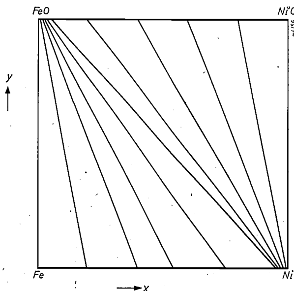
Fig. 9. Phase diagram for the system Fe-Ni-FeO-NiO (schematic). This diagram serves to elucidate fig. 7. The connodes have been drawn in order to demonstrate that the combination Ni + FeO is more stable than the combination Fe + NiO.
