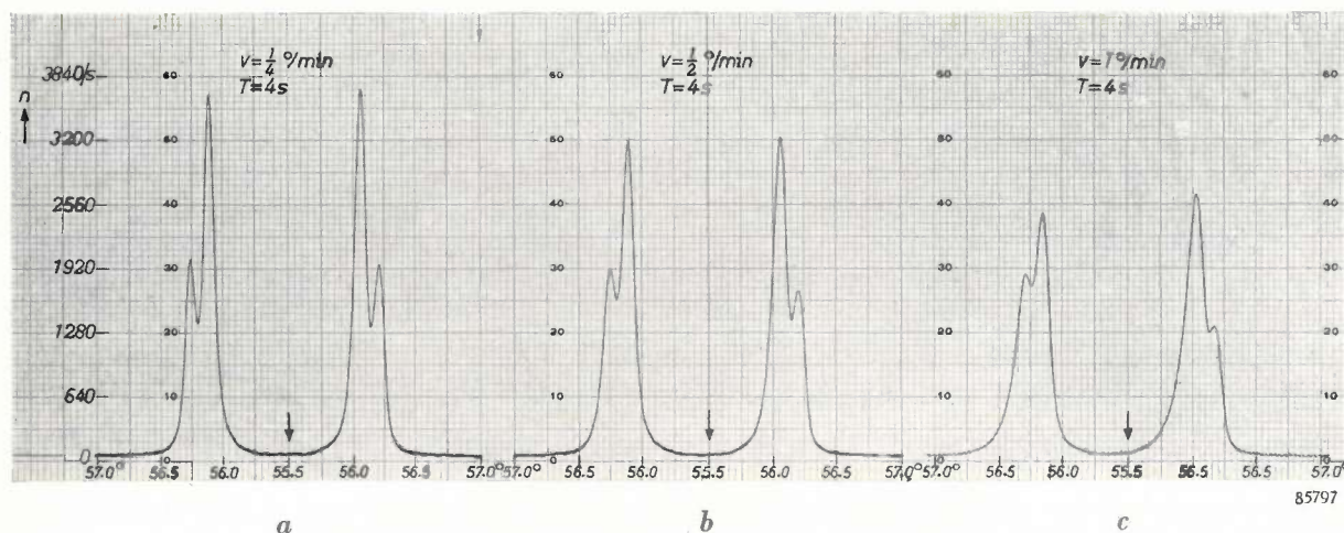
Fig. 5. a-c ) Diffraction line (silicon, reflecting plane 311) recorded with the counting-rate meter at three different scanning speeds v ; time constant T = 4 seconds. Unfiltered \text{CuK} radiation, angular aperture 1^\circ , receiving slit width 0.15 mm. Each recording shows the line scanned in both directions (reversal of direction at the arrow). The line profile is seen to deteriorate as the scanning speed is increased. The speed of the recorder chart, which can be varied independently of the goniometer speed v , was selected to make the width of the recordings a ) - c ) equal. The number of counts accumulated in any given angular interval naturally decreases with increasing v .
