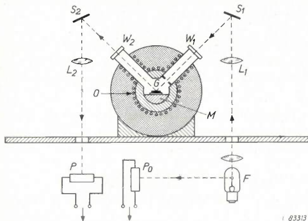
Fig. 2. Basic layout for the objective determination of the gloss point. In the furnace O the sample G is placed on a chrome-iron block M . By means of a small incandescent lamp F , lens L 1 and mirror S 1 , a narrow beam of light is directed through window W 1 on to the glaze. Specially reflected light leaves the furnace via window W 2 and is directed upon photo-electric cell P by mirror S 2 and lens L 2 . Direct light from the light source falls upon the photo-electric cell P 0 . The ratio of the photo-electric currents from P and P 0 is recorded as a function of the furnace temperature.
