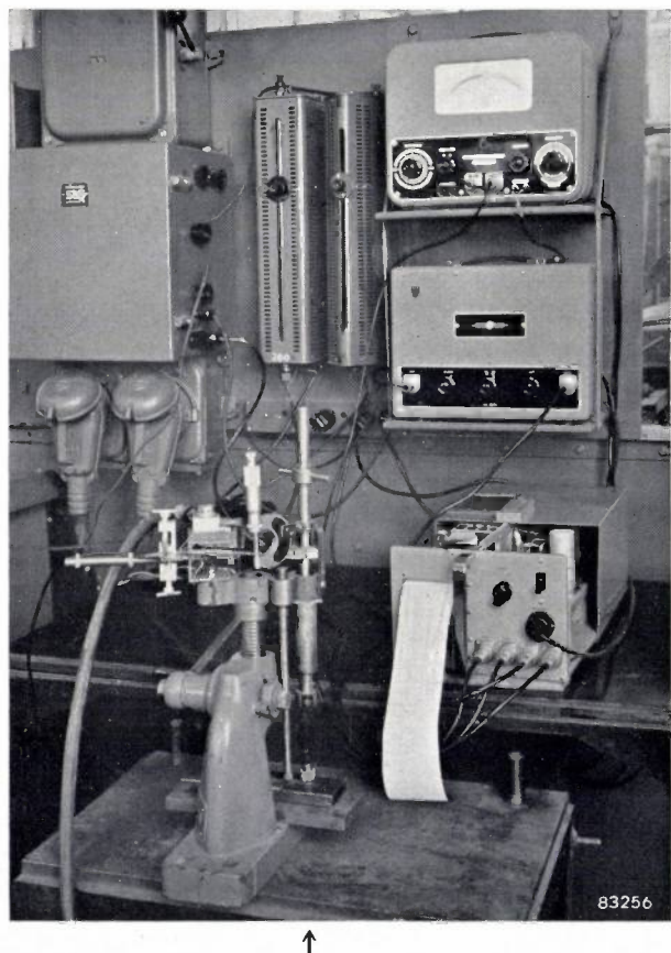
Fig. 11. The equipment employed to record variations in the voltage and the current, and in the distance between the stud and the work, as a function of time during the welding process. The ordinary welding gun was not employed during these measurements. The arrows indicate the position of the welding cartridge.
