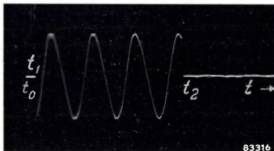
Fig. 8. Oscillogram referring to fig. 7. At t = t_0 , the push button of S_2 is pressed, with S_1 already closed. After a certain delay, depending upon the design of S_1 , the contacts of S_1 open, that is at t = t_1 . A 50 c/s voltage then appears on the oscilloscope; this voltage is suppressed when S_2 closes (at t = t_2 ). The interval between t_1 and t_2 is 3\frac{1}{2} cycles.
