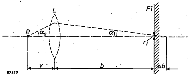
83412 Fig. 4. Illustrating the geometrical blur, \delta_g . P specimen, L electron lens, FI fluorescent screen. (The projector lens can here be neglected.)
