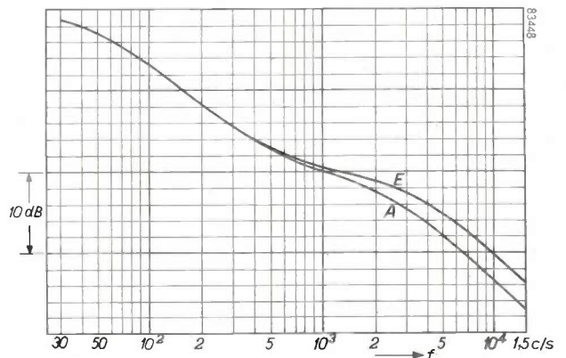
Fig. 3. Proposals for a standard reproduction channel for long-playing records, submitted to the I.E.C. for consideration. The speed v of the needle point for a constant sound intensity is plotted along the vertical axis. Along the horizontal axis the frequency f is plotted. Both are on a logarithmic scale. Curve A corresponds to the American proposal, curve E to the European proposal.
