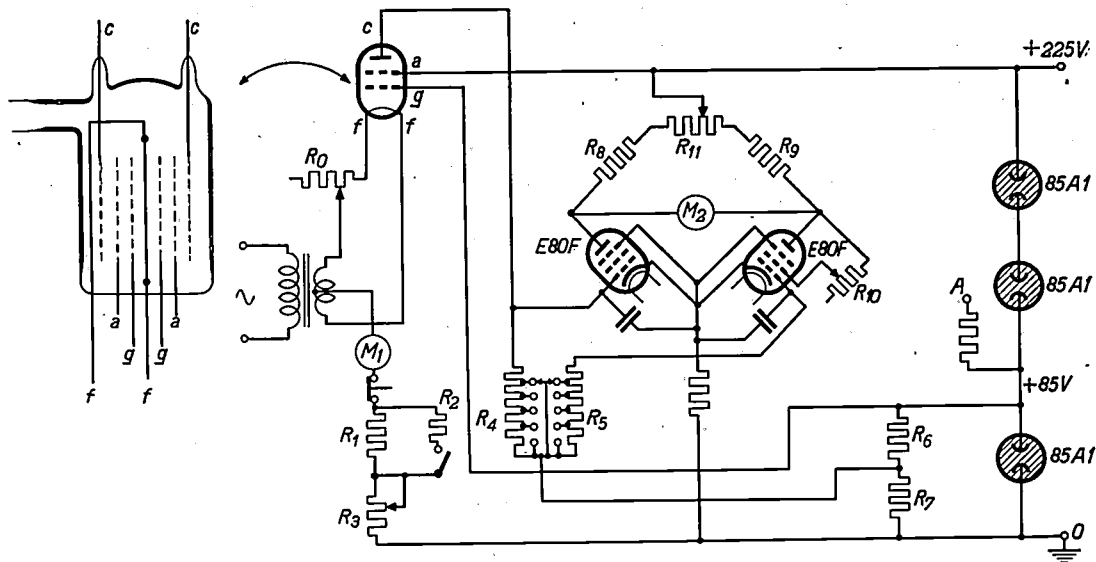
Fig. 3. Circuit diagram of the ionization manometer. The manometer tube is shown as a normal tetrode. The drawing on the left shows the tube more in its actual form. The glass wall is covered with an earthed conducting layer, except where drawn with thin lines. The meter M_1 is used for adjusting the ionizing electron current; the pressure is read from M_2 .
