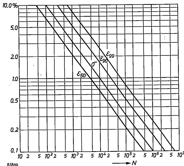
Fig. 3. Probable fractional error \epsilon_{50} of counting rate, and 90\% and 99\% confidence limits \epsilon_{90} and \epsilon_{99} , as functions of the accumulated number of counts N , for a Gaussian distribution.
