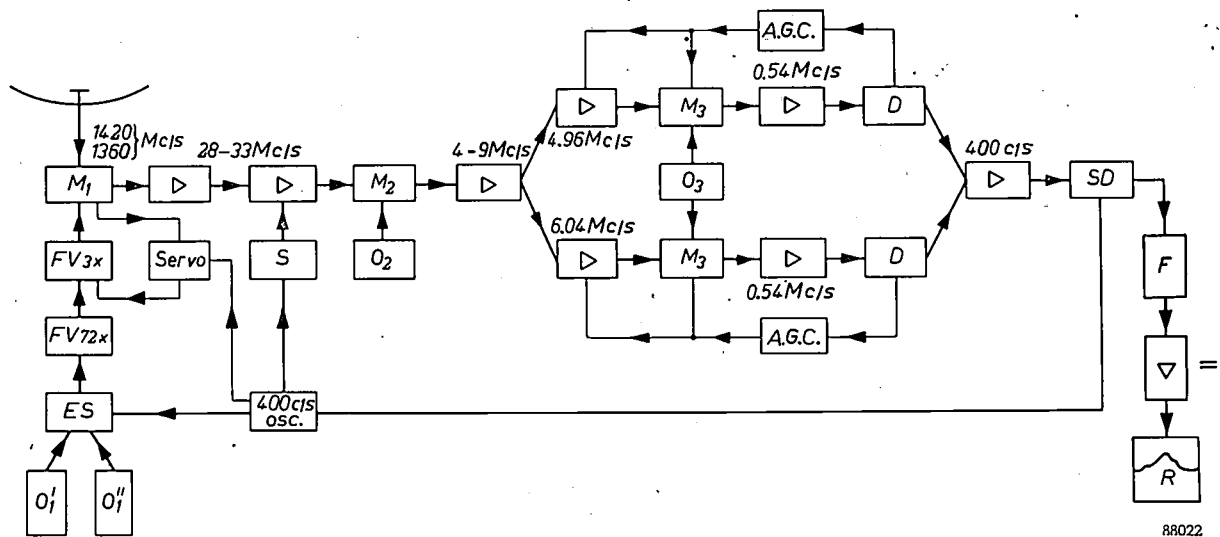
Fig. 2. Block diagram of the receiver. The units joined by thick lines constitute the receiver proper; those joined by thin lines represent control circuits. O'_1 and O''_1 are the crystal oscillators of the first mixer stage M_1 ; O_2 and O_3 are the oscillators of the second and third mixers, M_2 and M_3 respectively. FV frequency multipliers, ES electronic switch, D detectors, AGC automatic gain control, SD synchronous detector, F low pass filter, R strip-chart recorder.
