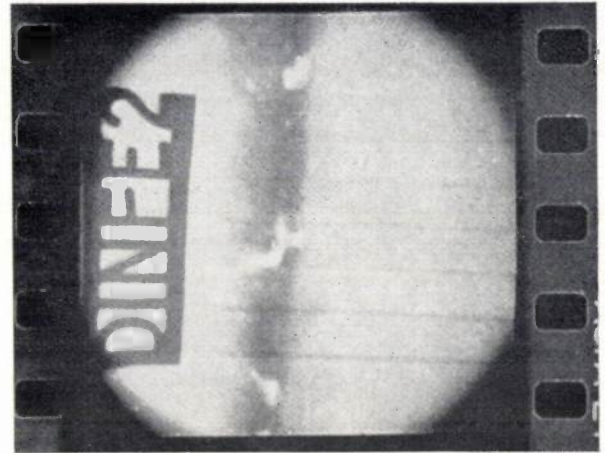
Fig. 5. Welded seam in steel sheet 15 mm thick, photographed with the image intensifier. Note the faults in the seam, and the shadow of the DIN test-object placed in front of the plate. X-ray tube data: 140 kV, 3 mA; focus 0.4 \times 0.4 mm. Exposure 15 seconds.
