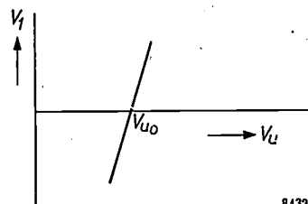
Fig. 8. Relationship between V_u and V_1 (fig. 7). V_1 is a measure of the deviation of V_u from its nominal value V_{u0} .
