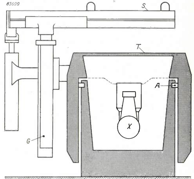
Fig. 5. Cross-section of the "Symmetrix" table. The base forms a U, over which the table, with its two sidewalls, fits as an inverted U. G is the mounting of the viewing system S. For the other letters see fig. 1 and fig. 3.
