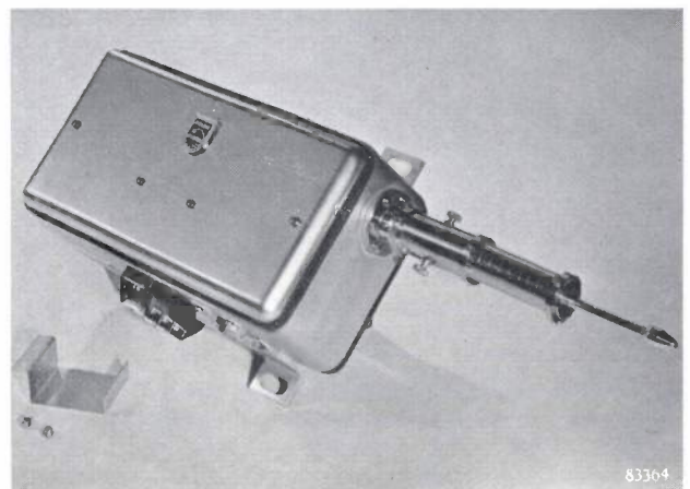
Fig. 11. The displacement pick-up of fig. 10 with the cover removed and closed ready for mounting. For calibration, the amount of the displacement can be read direct from a scale; this reading should correspond to the deflection of the recording meter.
