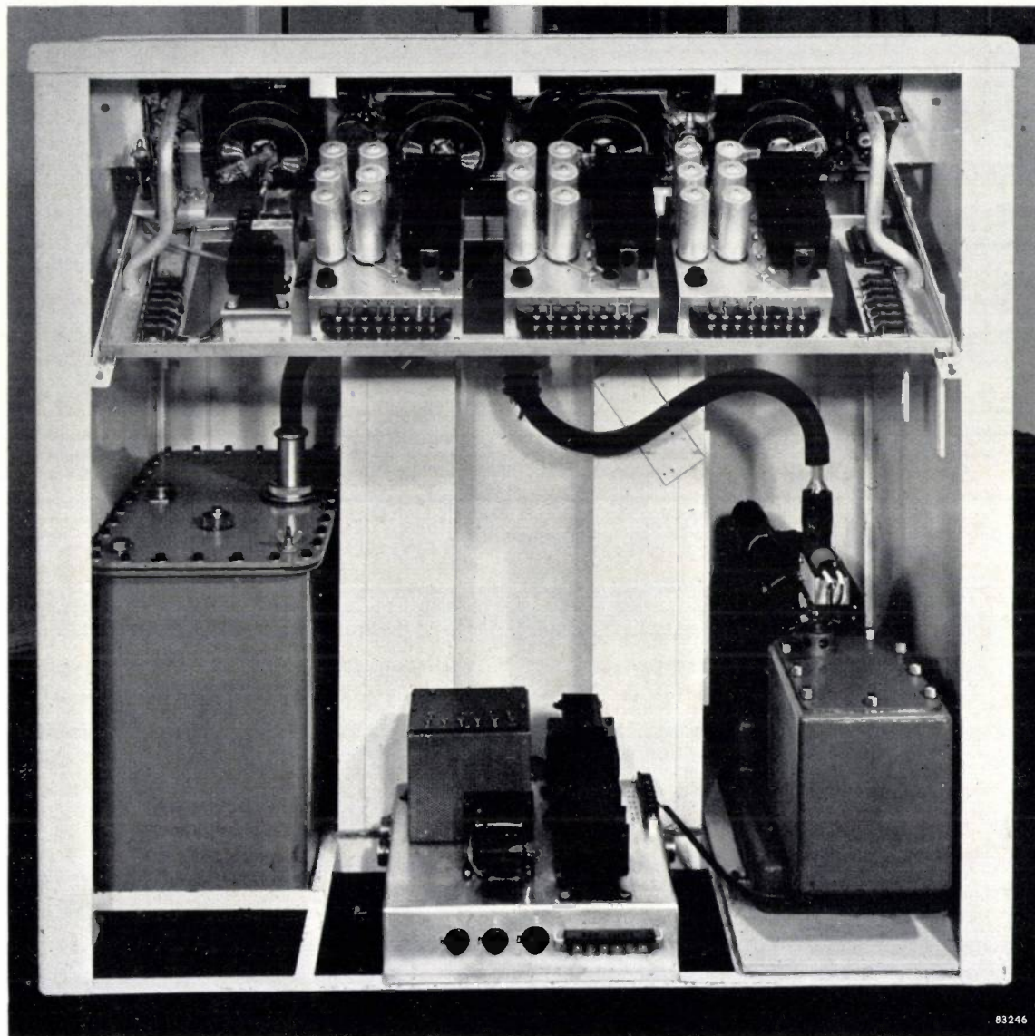
Fig. 16. The desk of the EM 75 kV seen from the back (back panel removed). Bottom left, tank containing the oil-immersed high tension generator, rectifier valves and filament current transformer. Bottom right, backing vacuum pump. Centre magnetic mains voltage stabilizer. Above, rectifiers and smoothing condensers, which supply the energizing current for the three electron lenses. Behind them is the back of the operating panel with knobs and switches.
