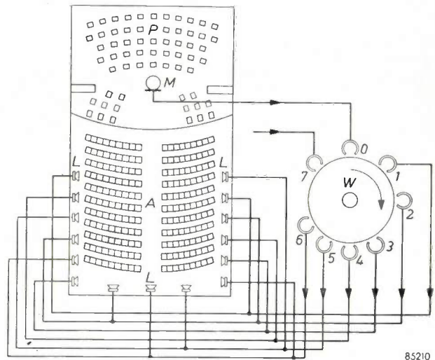
Fig. 1. Installation for simulating indirect sound with various time lags. A auditorium. P platform. M microphone. W delay wheel, coated on the edge with magnetic material suitable for magnetic sound recording. O recording head, 1...6 play-back heads. 7 erasing head. L loudspeakers.
