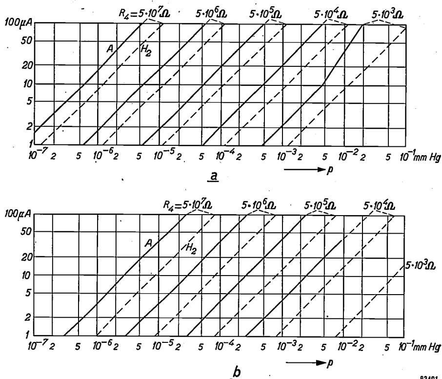
Fig. 5. Calibration curves for the large type of manometer tube (a) and for the smaller type (b). The full lines apply to argon (A), the broken lines to hydrogen ( H_2 ). The ionizing electron current was 0.5 mA. The value of the saturation emission has some influence on the calibration at pressures higher than 5 \times 10^{-3} mm Hg. In the present case the saturation emission was 1 mA. Both the pressure p and the current read from M_2 (see fig. 3) (not the ion current itself!) have been plotted logarithmically. Only a straight line with a slope of 45^\circ then represents a linear relationship between pressure and current, so that with this instrument the current increases slightly more than proportional to the pressure. The values of the resistor R_4 , corresponding to the various parts of the graphs, are included in the diagram. If the ionizing electron current is adjusted to 2.5 mA, pressures down to about 10^{-8} mm Hg can be measured. The ion current itself may be evaluated from the bridge sensitivity ( 760 \mu A/V ) and the value of R_4 .
