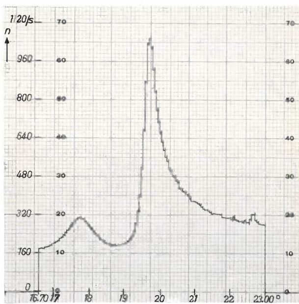
Fig. 14. Part of recording of a diffraction pattern ( 16.7^\circ < 2\theta < 23.0^\circ ) made with the counting rate computer. Montmorillonite (dry specimen), \text{CuK}\alpha radiation with nickel filter, steps 0.05^\circ with N = 6400 ; recording time 2\frac{3}{4} hours.
