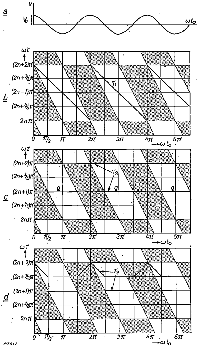
Fig. 2. a) The high-frequency voltage v = V_0 \cos \omega t_0 . b), c) and d) Electron transit-time diagrams; t_0 is the moment at which the electrons first pass through the resonator gap; \tau is the transit time, i.e. the time between two outward excursions by the electrons. The various transit-time functions \tau_1 (b), \tau_2 (c) and \tau_3 (d) are described in the text.
