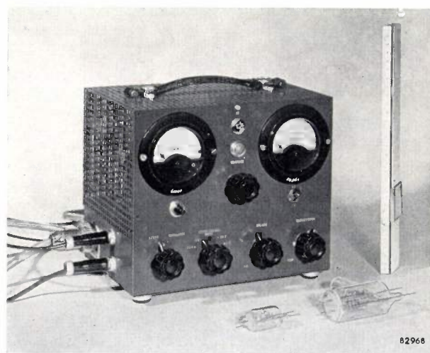
Fig. 2. The ionization manometer, showing two manometer tubes, one of a large and one of a small type.
