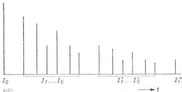
Fig. 4. If a report (pulse I_0 ) is produced in a hall with stereo reverberation, the six loudspeakers deliver during one revolution of the delay wheel the six reports I_1 \dots I_6 . If electrical feedback is applied from the sixth play-back head to the recording head, the loudspeakers give a second series of six reports ( I'_1 \dots I'_6 ), a third, and so on. (Acoustic feedback is here neglected.)
