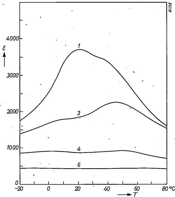
Fig. 11. \epsilon - T curves for a series of specimens in the \text{BaTiO}_3 - \text{SrTiO}_3 - \text{CaTiO}_3 system to which about 10% \text{Mg}_2\text{TiO}_4 has been added. The compositions (calculated without the \text{Mg}_2\text{TiO}_4 ) of 1, 3, 4 and 6 correspond approximately with the similarly numbered points in fig. 5. The effect of the additive is to make the curves flatter than those in fig. 6.
