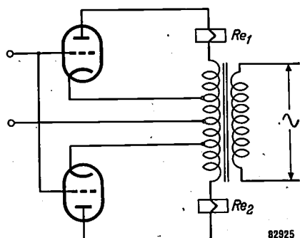
Fig. 9. Combination of two phase detectors, for use with a floating control with constant motor speed.
