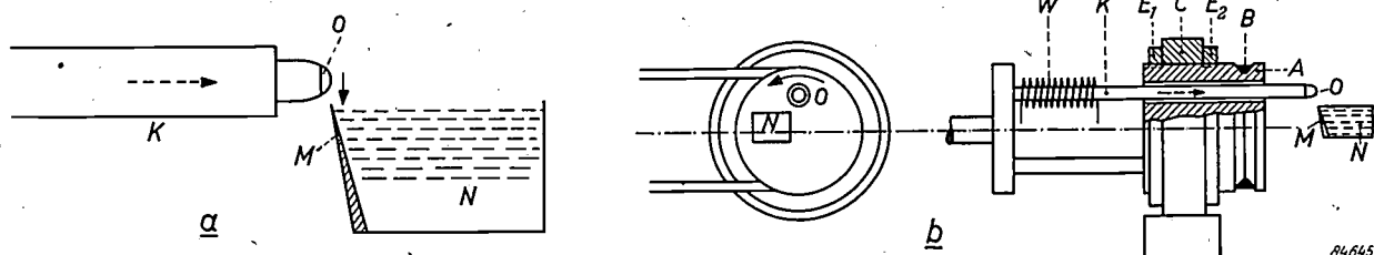
Fig. 2. a) Simplified diagram of an ultramicrotome with displacement by means of thermal expansion. The knife is a safety-razor blade, (M) sharpened and polished in a special way, or in some cases, a knife specially made for this purpose of glass or diamond. The knife is fixed. The specimen (O) is mounted on a metal rod (K) which holds it above the knife. The thermal expansion of the rod (--->) produces the forward motion of the specimen, so that when the rod moves downwards a thin section is cut. A small dish (N) is fixed to the knife and is filled with liquid (usually 20% alcohol) up to the cutting edge of the knife. The sections, when cut, slide off the knife on to the surface of the liquid and usually form a chain. They can easily be transferred from the liquid surface to a formvar film on a specimen carrier. b) In an instrument developed by Sjöstrand the rod K rotates with the specimen O. This is effected by the pulley D driven by the belt B. The pulley runs in bearings in the fixed ring C and is fixed in the axial direction by the rotating rings E 1 and E 2 . Electric heating (winding W) causes the rod to expand. The knife M and the dish N are so placed that the specimen only touched the knife on its downward path. On the upward path, the specimen passes behind the knife.
