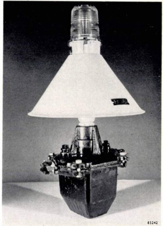
Fig. 14. Taxiway light, mounted on a transformer with cast iron case filled with compound. Note bushings for connection to armoured cables.
