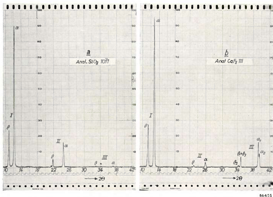
Fig. 17. Molybdenum K-spectrum excited by a tungsten target X-ray tube and reflected by different analyzing crystals. (Nickel filter placed on window of X-ray tube to eliminate scattered L-spectrum of tungsten.) a ) Reflection from quartz cut parallel to 1011. b ) Reflection from fluorite, cleavage plane 111. The first, second and third orders are indicated by Roman numerals.
