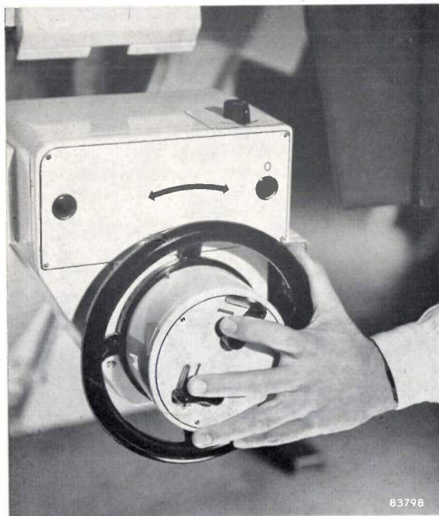
Fig. 7. The control box. The hand wheel controls the rotation of the patient about the horizontal X-ray beam. The two switches on the hub of this wheel control the longitudinal and lateral movements of the patient, and the switch on top of the box controls the rotation of the patient about his longitudinal axis. When the button 0 on the right is pressed, all the moving parts of the apparatus return to their normal positions. The button on the left enables the whole apparatus to be stopped immediately in an emergency.
