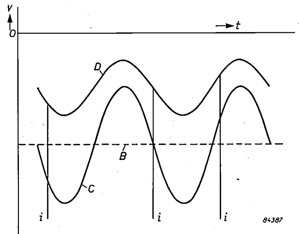
Fig. 13. The straight line B and curves C and D give the voltage variations at the points B, C and D respectively in fig. 12b with respect to earth (O). Interference pulses are clipped at the level B.
