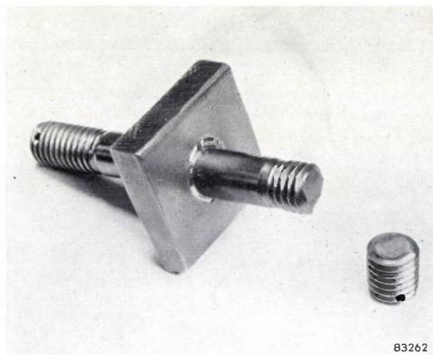
Fig. 14. a) Result of a tensile test on two studs welded end to end to opposite sides of a plate. b) Result of a fatigue test.
