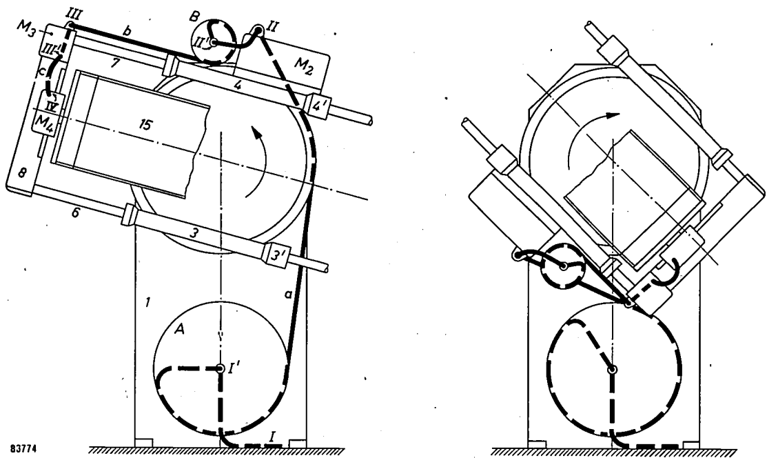
Fig. 6. Connecting cables on the equipment. During all movements, cable sections a and b are held taut between terminal points I , II and III by spring-loaded cable-drums A and B . Section c is prevented from sagging by a wire spiral fitted round it. Other components numbered as in fig. 5. The diagram on the right shows the change in the configuration of the cable sections when the patient is adjusted to another position.
