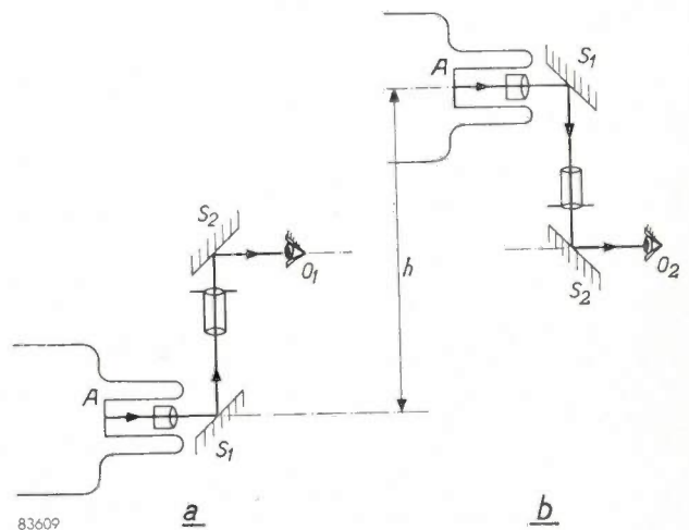
Fig. 6. Periscope optical system. (a) Two mirrors parallel to each other ( S_1 and S_2 ) bend the path of rays, but do not change the position of the observed image. (b) By rotating the whole system about axis AS_1 , the image intensifier can be raised or lowered a distance h without varying the level of the eye ( O_1 or O_2 ). The direction of observation can be varied by tilting mirror S_2 about an axis perpendicular to the plane of the drawing.
