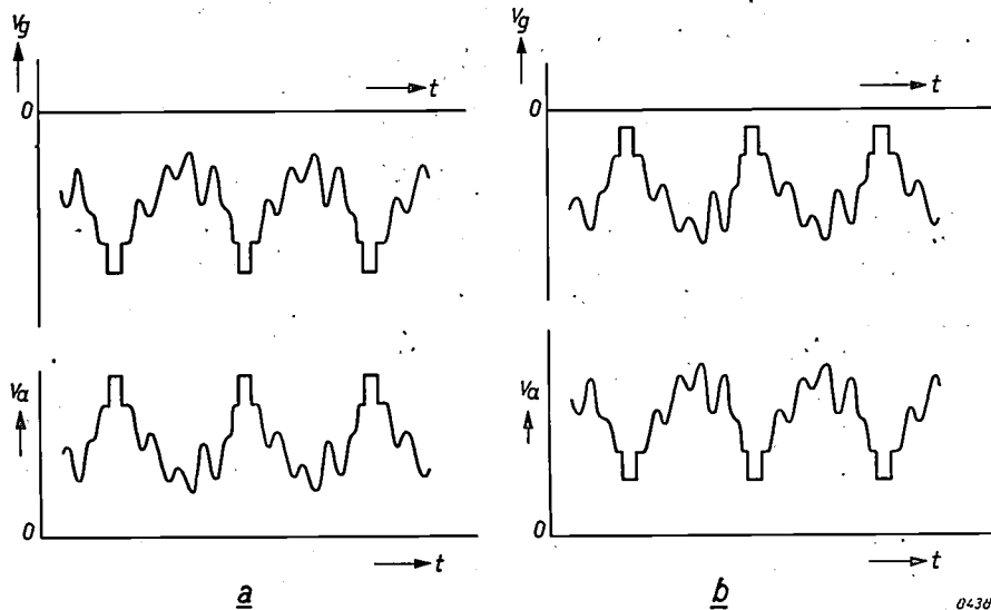
Fig. 9. Control grid voltage v_g and anode voltage v_a of the video tube PL 83 ( fig. 8 ) as a function of time t , a ) with negative modulation, b ) with positive modulation.
