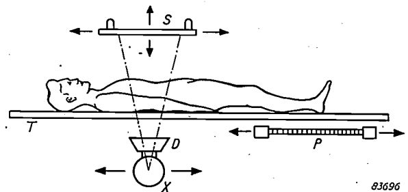
Fig. 1. Essential parts of a table for X-ray diagnosis. T table to carry the patient; X X-ray tube (with adjustable lead diaphragm, D , to limit the X-ray beam); S viewing system comprising a fluorescent screen and film-cassette; P Potter-Bucky diaphragm, and film-cassette employed in conjunction with an alternative separately mounted X-ray tube. The tube ( X ) can be moved parallel to the table, that is, in the directions indicated by arrows, and also at right angles to the plane of the drawing; the viewing system ( S ) moves with the tube, and can also be moved perpendicular to the surface of the table. The table top is made of a material of low X-ray absorption.
