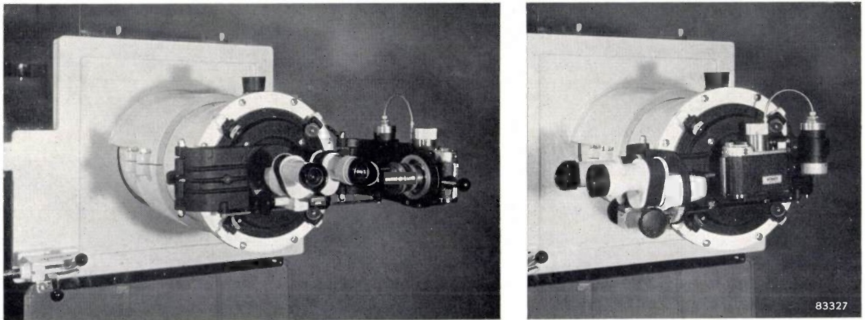
Fig. 5. Binocular microscope and camera, mounted so that they can be swung alternately into position in front of the image intensifier. The left-hand picture shows the microscope in use; in the right-hand picture the camera is in use.
