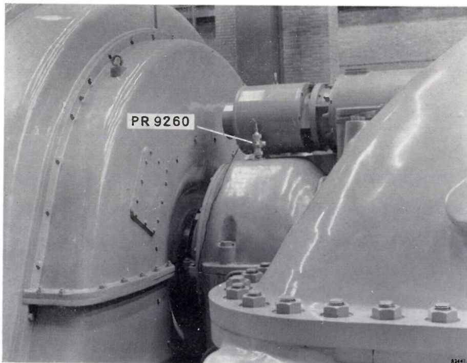
Fig. 3. The vibration pick-up PR 9260 fixed to the bearing cap.
