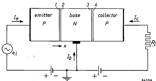
Fig. 4. Schematic representation of a P-N-P-transistor. Between the P-regions to the left and right, respectively designated "emitter" and "collector", is the "base" of N-germanium. I_e , I_c and I_b are respectively the emitter, collector and base currents. Currents in the direction of the arrows are considered positive. 1, 2, 3 and 4 mark the boundary planes of the P-N and N-P junctions. e_i A.C. input source; R_l resistance in the collector circuit, across which the amplified voltage appears.
