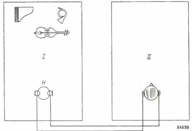
Fig. 2. Binaural hearing. The music played in room I is heard by the listener in II via headphones, each ear-piece of which is connected to a microphone. He thus receives an impression of auditory perspective. The microphones should preferably be fitted on an artificial head (H).
