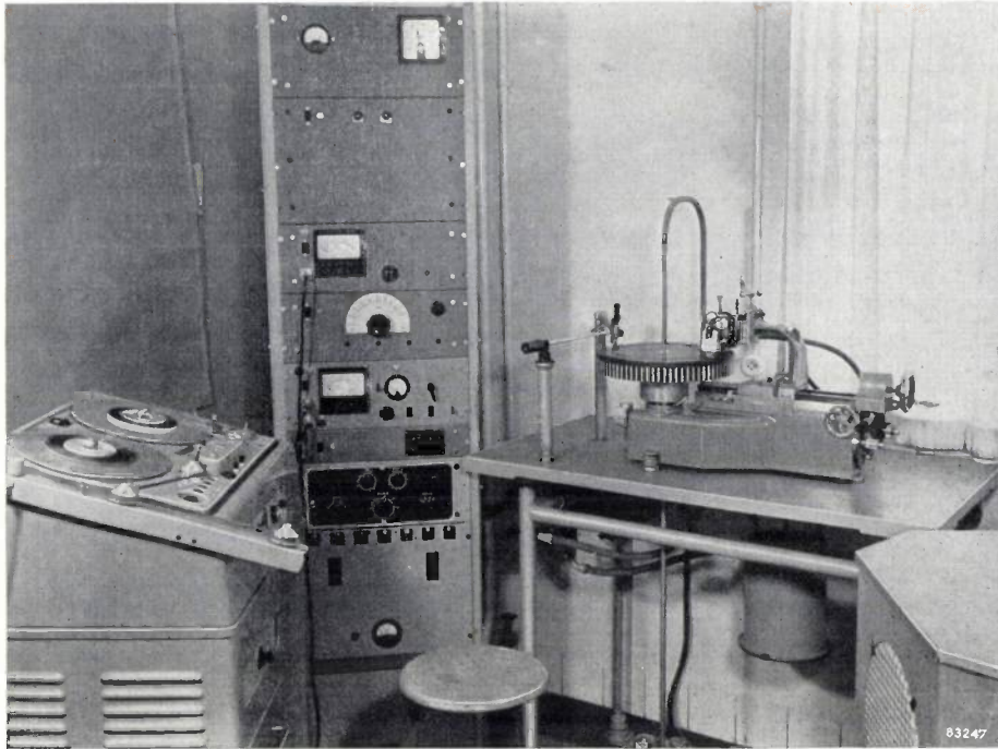
Fig. 1. Equipment for the transfer of magnetic recordings onto lacquer discs. From left to right: the machine in which the magnetic recording is played back, the amplifier rack (also containing other electronic apparatus), the machine on which the lacquer disc is engraved, and a monitoring loudspeaker.
