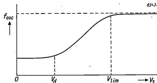
Fig. 6. The frequency f_{osc} of the oscillator (13 in fig. 4) as a function of the signal voltage V_s . The threshold voltage is V_d , the limiting voltage V_{lim} .
