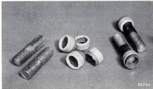
Fig. 5. Threaded studs ( \frac{1}{2} -inch) and the corresponding welding cartridges. Two studs with cartridges fitted are shown on the right of the picture.
