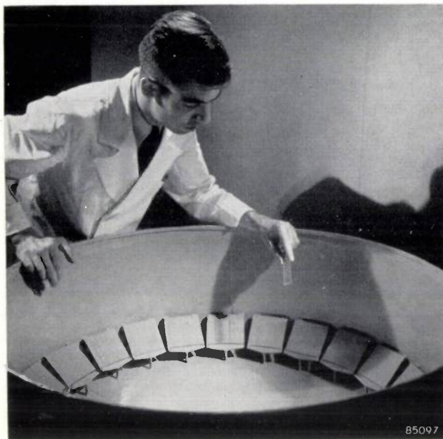
Fig. 4. An apparatus for determining the extent to which fungicidal preparations remain fixed to glass during rainfall.
