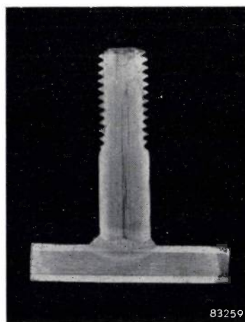
Fig. 12. Cross-section of a \frac{1}{2} -inch stud welded to a plate by the cartridge method of stud welding. The slag enclosures revealed by etching show that the stud and the plate are both made of rimmed steel 4 ).
