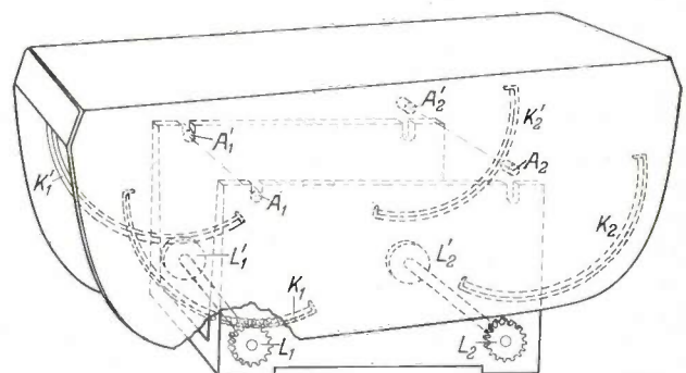
Fig. 6. Schematic drawing of the driving mechanism of the table. The table carries two heavy sprockets acting as toothed segments, K 1 -K 1 ' and K 2 -K 2 ', centring upon the two axes of rotation, A 1 -A 1 ' and A 2 -A 2 ', respectively. These sprockets engage with two pairs of sprocket wheels, L 1 -L 1 ' and L 2 -L 2 ', which are driven (at the same speed and in the same direction) by a centrally mounted motor (see fig. 9).
