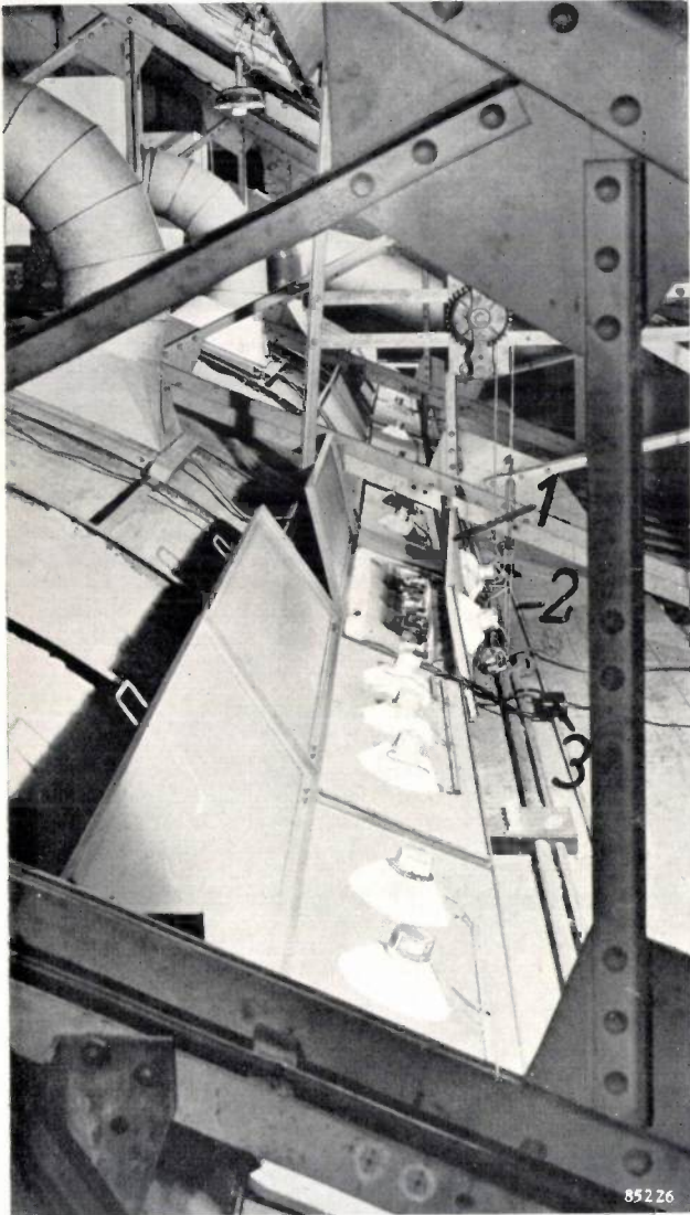
Fig. 9. The loudspeakers of the stereo reverberation installation in the Philips Theatre are mounted in groups of two or three in the panels which cover the lighting cornice ( L in fig. 6). At 1 one of the panels has been lifted up. 2 is the (six-core) cable, 3 a junction box.
