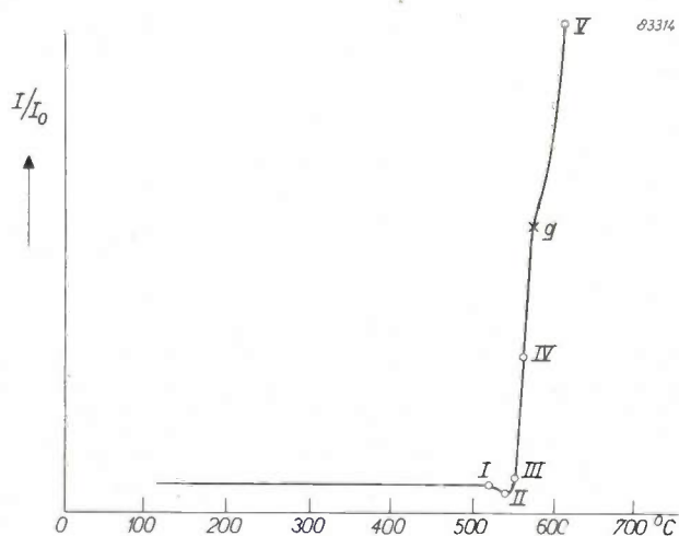
Fig. 5. Recorded gloss curve of a jointing glaze. The ratio I/I_0 of specularly-reflected light to incident light is recorded as a function of the temperature. The test, carried out on a number of samples, was broken off at various points of the curve (I-V), by quickly removing the sample from the furnace. The sudden increase in viscosity, due to rapid cooling, "freezes" the surface appearance of the sample, so that it can be inspected at room temperature. Point g can be regarded as the gloss point.
