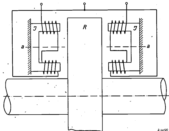
Fig. 9. The displacement pick-up of fig. 7 in a construction suitable for measuring the change in length of the shaft relative to the casing. The yokes J are rigidly connected to the casing. A disc R (of "Permenorm"), fitted on the shaft, functions as armature. (For the sake of clarity the yokes are shown rotated through 90^\circ about line a-a .)
