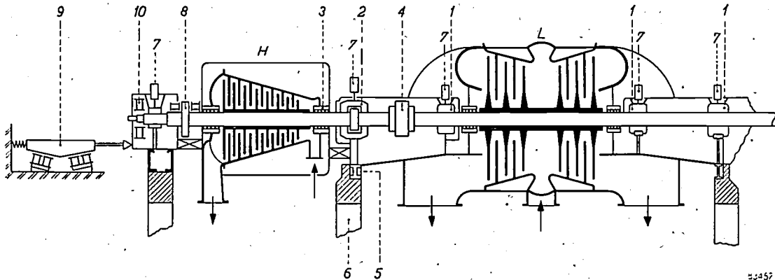
Fig. 1. Cross-section of a steam turbine. H high-pressure stage, L low-pressure stage (the arrows indicate the direction of the steam). 1 slide bearings. 2 thrust bearing. 3 labyrinth gland. 4 flange coupling. 5 point at which the casing is rigidly connected to the foundation. 6. 7 vibration pick-ups for checking the vibrations of the shaft bearings 1 and 2. 8 disc for measuring relative changes in length of the shaft. 9 pick-up for measuring the absolute change in length of the casing. 10 disc for measuring the eccentricity.
