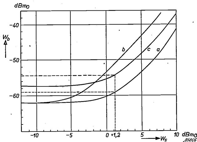
Fig. 13. a ) Experimental curve, showing the noise power W_b in one of the 8 free channels as a function of the power W_s supplied to the remaining 40 channels. b ) Curve computed from a which would apply if, using the same type of transmitters and receivers as in a , transmission were over a standard circuit of length 2500 km, the frequency swing being adjusted to the optimum value for each individual link. c ) Curve which applies if the frequency swing in each of the links were adjusted to the value most favourable to the whole. The power values are plotted in dBm 0 , i.e. in dB relative to a power of 1 mW at points at relative zero level.
