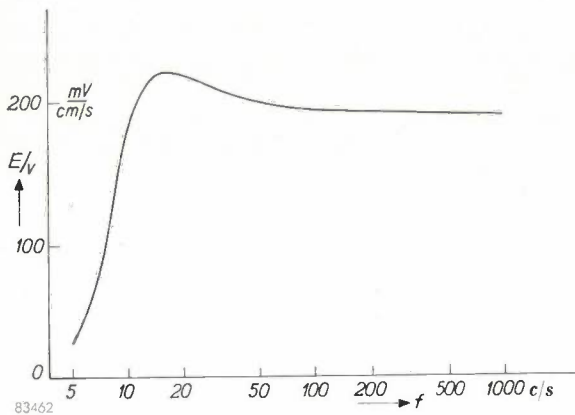
Fig. 4. Response curve of the vibration pick-up PR 9260; the ratio of the output voltage E to the velocity V is plotted as a function of the frequency f .
