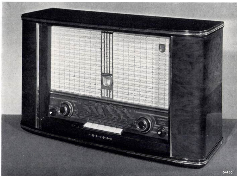
Fig. 6. Receiver (type BX 653 A) with a common tuning knob (the large knob on the right which appears to be double but is, in fact, single). This controls the A.M. tuning when an A.M. button is pressed in and the F.M. tuning when the F.M. button is pressed in. The knob on the left is double; the front knob is the volume control and the rear one adjusts the orientation of the "Ferroceptor" aerials. The knobs on the extreme left and right are independent tone controls for low and high notes.
