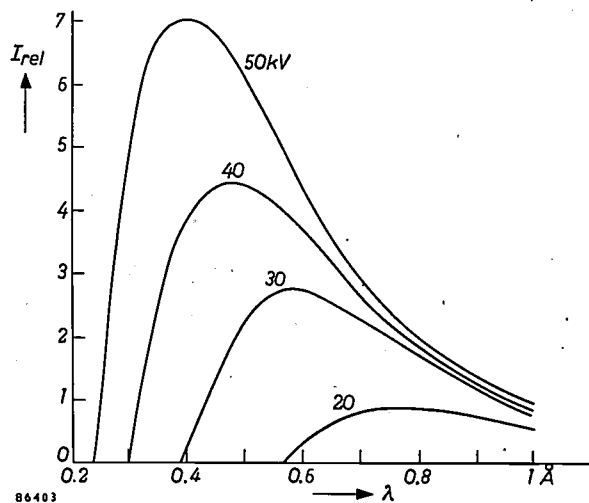
Fig. 8. The continuous spectrum of a tungsten target X-ray tube (relative intensity I_{rel} vs. wavelength \lambda ) obtained with various voltages (peak values) and the same tube current. The curves were redrawn from separate rate meter recordings. Experimental conditions: full-wave rectification, silicon crystal analyzer (111-plane), scintillation counter.
