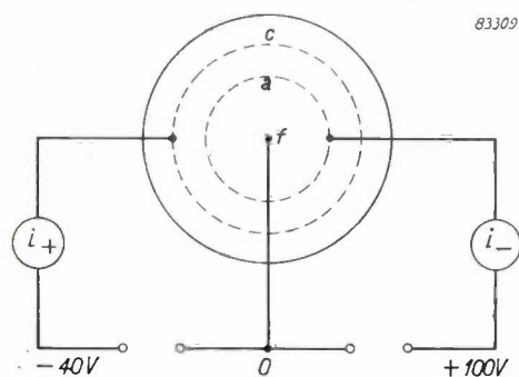
Fig. 1. Principle of the ionization manometer. The electrons emitted by the cathode f are accelerated by the anode a (which has the form of a grid), at which they finally arrive; they produce the current i_- . The ions formed arrive at the ion collector c and produce the current i_+ .
