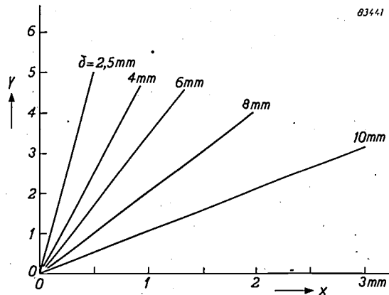
Fig. 8. The voltage y (fig. 7) plotted on an arbitrary scale as a function of the deflection x of the armature from the central position for various values of the air gap \delta .
