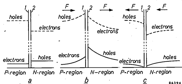
Fig. 1. Concentrations of minority charge carriers (full lines) and of majority charge carriers (broken lines), as functions of position on either side of a P-N junction in a germanium crystal. The concentration of majority charge carriers in practice is between 10^4 and 10^6 times that of the minority charge carriers. 1 and 2 denote the boundary planes of the junction. a) No voltage is applied to the crystal; everywhere outside the junction the concentrations assume uniform equilibrium values. By the addition of suitable impurity elements in the proper proportions, both in the P -region and the N -region, the equilibrium concentrations can be varied within wide limits (on condition that the product of minorities and majorities in any one region remains constant). b) A voltage is applied to the crystal which raises the potential on the P -region with respect to the N -region. The electric field F , whose direction is shown by arrows, drives majority charge carriers (holes in the P -region and electrons in the N -region) towards the P-N junction. c) The polarity of the voltage is opposite to that in (b). The field now drives majority charge carriers away from the junction.
