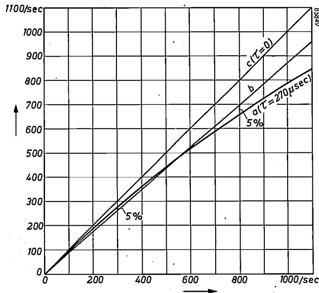
Fig. 19. Response (a) of the Geiger counter tube to random quanta as a function of the true average count rate. The deviation from linearity is due to the finite resolving time for successive quanta. The measured effective "dead time" of the "Norelco" No. 62019 Geiger counter is \tau = 270 \mu\text{sec} for Cu K \alpha radiation from an X-ray tube operated with full wave rectification at 35 kV peak. With the X-ray tube operated at constant potential a smaller effective dead time is found; cf. note 15) . For \tau = 0 , the straight line c would be obtained.
