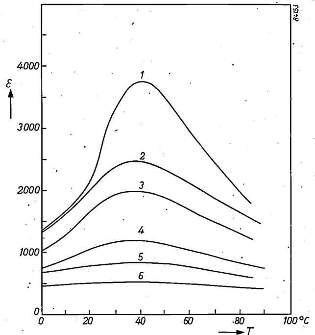
Fig. 6. \epsilon - T curves for sintered specimens, composed of \text{BaTiO}_3 , \text{SrTiO}_3 and \text{CaTiO}_3 , corresponding to the compositions 1 to 6 in fig. 5. Compositions 3 to 6 lie in the two-phase region and in this order contain increasing amounts of the phase rich in \text{CaTiO}_3 , which makes the \epsilon - T curves increasingly flat.
