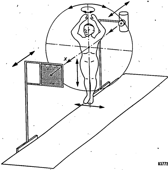
Fig. 4. Degrees of freedom of the patient, the X-ray tube and the viewing system in the "Müller" UGX diagnostic unit. The centre-line of the X-ray beam remains in a fixed horizontal position throughout these movements.
