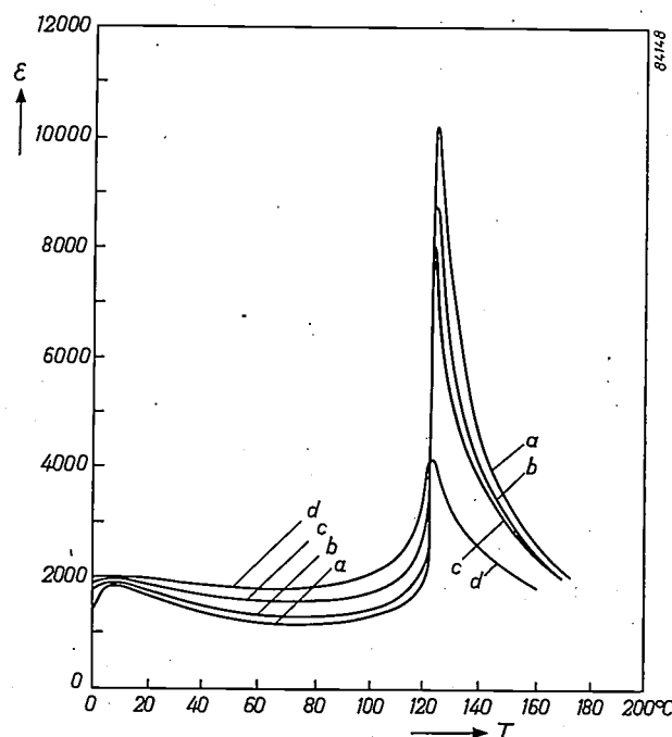
Fig. 1. The dielectric constant \epsilon of \text{BaTiO}_3 as a function of temperature T . The curves a, b, c, d have been measured for specimens sintered at 1400, 1350, 1300 and 1280^\circ\text{C} respectively. In the same order the size of the crystals decreases from about 100 \mu to 5 \mu . The maximum at 123^\circ\text{C} corresponds to the transition from cubic to tetragonal structure, the maximum at about 10^\circ\text{C} to the transition from the tetragonal to the rhombic structure.
