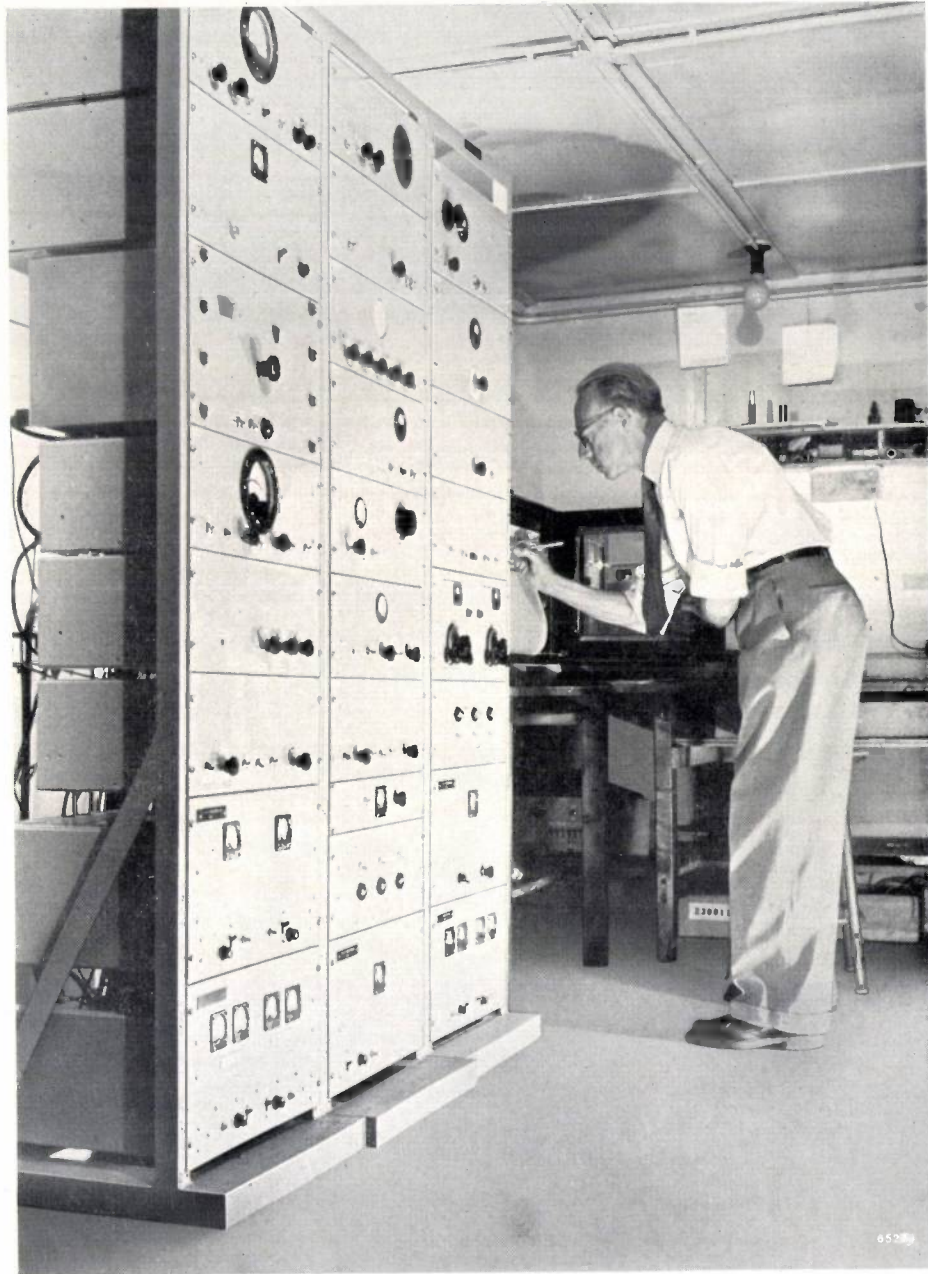
Fig. 8. The radio receiver as installed at Kootwijk.
