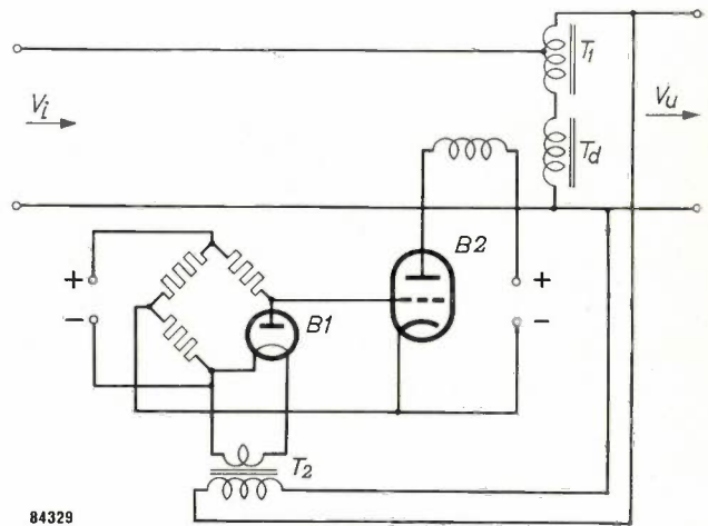
Fig. 10. Simplified circuit diagram of the equipments of fig. 9 . The bridge incorporating the diode B_1 becomes unbalanced if the filament voltage of B_1 deviates from its nominal value; the bridge thus acts as detecting device.
