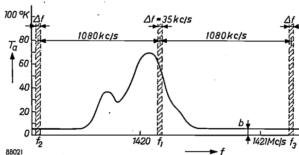
Fig. 1. Schematic diagram of a typical profile of the 21 cm line radiated by interstellar hydrogen. The noise intensity received is expressed in "antenna temperature", T_a . Continuous background radiation is present ( b ), the temperature of which is normally less than 10 °K. The receiver is switched to and fro between the frequencies f_1 (on the spectral line) and f_2 and f_3 (adjacent to it, on opposite sides) The bandwidth in each case is about 35 kc/s. All three frequencies are simultaneously displaced through the spectrum, a constant frequency interval of 1080 kc/s being maintained between them.
