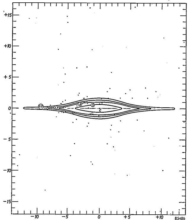
Fig. 1. Schematic section of the Galactic System, perpendicular to the equatorial plane. The Sun is indicated by the open circle (between 0.5 and 1), the centre is the point C. The interstellar matter is shown as a narrow hatched band; the full lines are contours of equal density (relative values indicated by the circled numbers; the contour containing the Sun is arbitrarily chosen as of unit density). The galaxy rotates about an axis through C, perpendicular to the equatorial plane. Scale: 1 unit = 1000 parsec.
