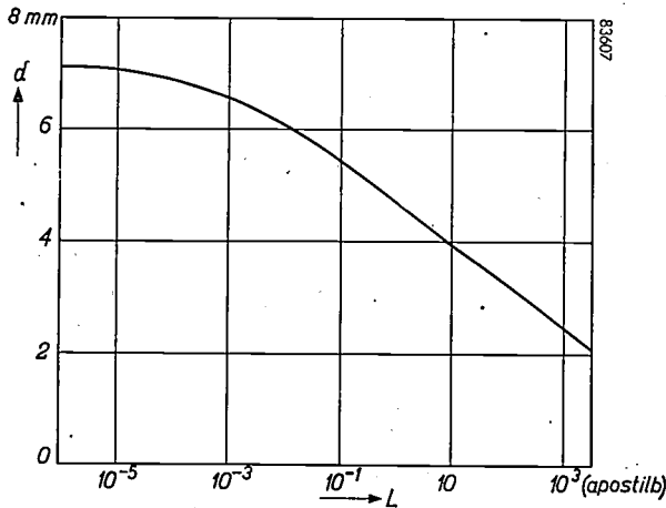
Fig. 3. Diameter ( d ) of the pupil of the human eye, plotted against the luminance L .
