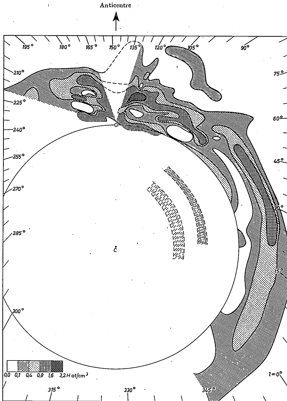
Fig. 4. Distribution of interstellar hydrogen in the equatorial plane of the Galactic System (schematic). The numbers around the edges give the galactic longitude l ; the centre is indicated by C and the Sun by a small circle vertically above it. The hydrogen density is given by the shading (see code bottom left). The spiral character of the arms can be detected. Observations of spiral arms which lie closer to the centre than the Sun, are drawn with broken lines. (Taken from articles 3 ) and 4 ). Between l = 130^\circ and l = 165^\circ the effect of the differential rotation is so small that the measurements are not sufficiently accurate.
