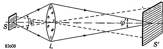
Fig. 4. Derivation of the sine condition. Lens L transforms area S into S' and angle \phi into \phi' .
