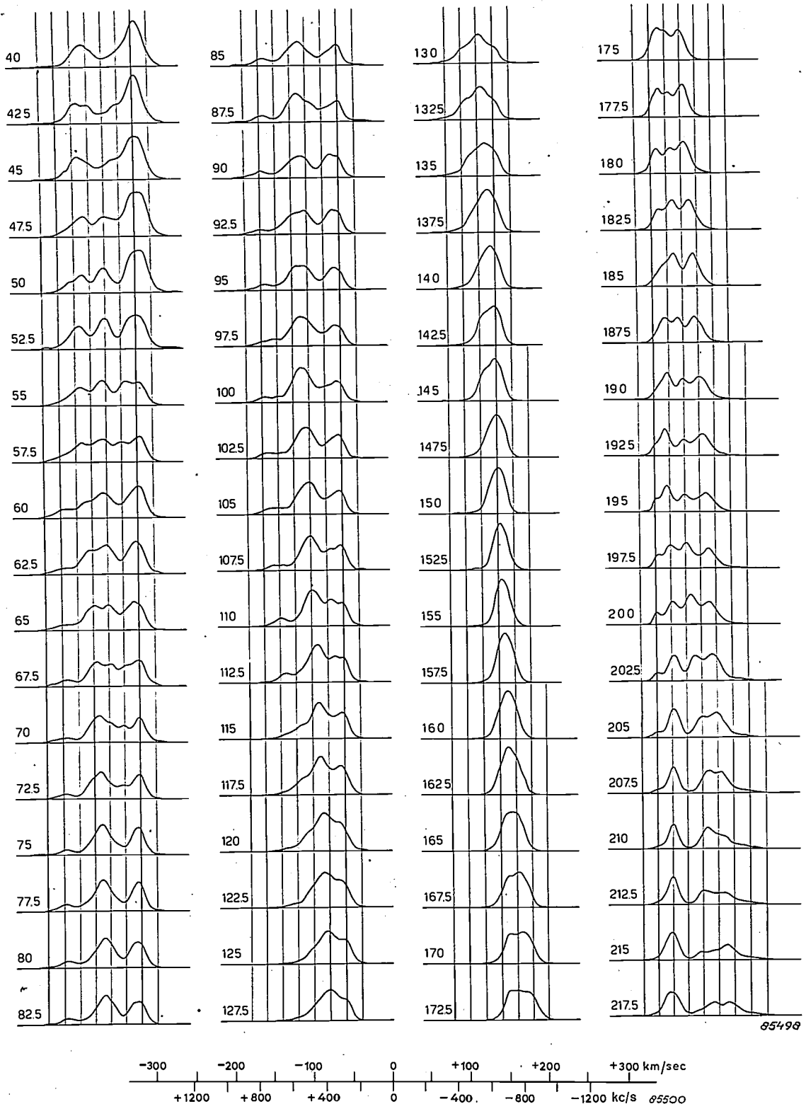
Fig. 3b. As for fig. 3a, for other directions in the equatorial plane of the Milky Way. The ideal profile occurs in the direction of the anticentre ( l = 147.5^\circ ).
