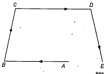
Fig. 3. Schematic diagram of the motion of the specimen in the new ultramicrotome (not to scale). AB ≈ 1-2 μ: retraction by magnetostriction. BC ≈ 3 mm: upward movement of specimen carrier. CD = AB: magnetostriction released. DE = BC: cutting stroke (specimen carrier drops). The distance AE ≈ 50-200 Å corresponds to the thermal expansion during the whole cycle ABCDE.
