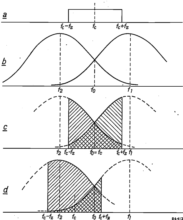
Fig. 1. a) The transmitted frequency band, showing the central frequency f_c and frequency swing f_z . The signal strength is plotted vertically. b) The band-pass curves of cavity resonators 1 and 2, with resonant frequencies f_1 and f_2 . c) The signals (hatched areas) produced by the frequency band in (a) in cavity resonators 1 and 2, when f_c = f_0 . d) The same when f_c \neq f_0 .
