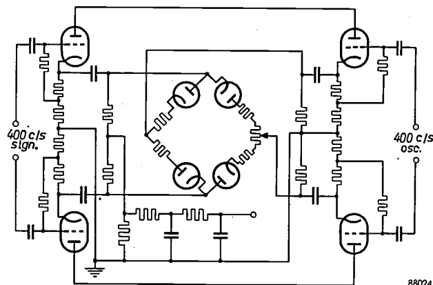
Fig. 4. Simplified circuit of the synchronous detector.
