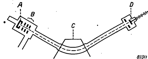
Fig. 6. Principle of a mass spectrometer. The gas to be analyzed, under low pressure, fills the entire spectrometer and is, therefore, also present in the ionization chamber A , where an electron current perpendicular to the plane of the drawing ionizes the gas molecules. The ions thus formed are accelerated by the accelerating and focussing electrodes B . The magnet C produces a field perpendicular to the plane of the drawing, and is so adjusted that ions of the desired component of the gas impinge upon the collector D .
