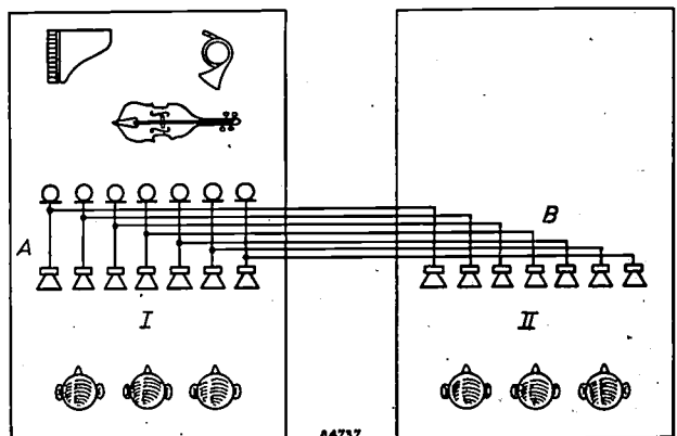
Fig. 4. Explanation of stereophony according to an American view. A is an imaginary "curtain", one side being fully taken up by microphones, the other by loudspeakers. Each microphone is linked via its own channel to the corresponding loudspeaker at the other side of the curtain, and also to a similar loudspeaker on "curtain" B in hall II. Thus, the same sound field is produced in hall II as in hall I. Practical stereophony, necessarily using only a small number of channels, would only be a rough approximation to the ideal case outlined.
