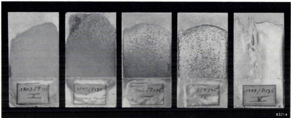
Fig. 6. Photographs of glaze samples, heated to points I-V indicated in fig. 5. I : The grains of glaze powder have only just started to adhere to the underlayer: very first signs of sintering. II : Grains rounded off, beginning of fusion. III : First signs of specular reflection in the hollows between the grains. IV : Whole surface not yet completely bright. V : Completely bright surface; the gloss point ( g ) has been well exceeded.
