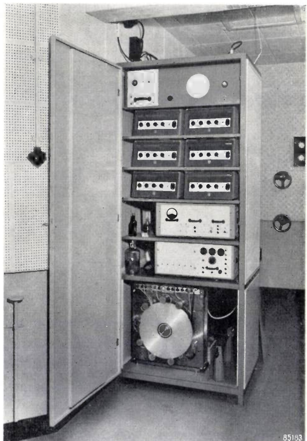
Fig. 2. Stereo reverberation installation in the Philips Theatre at Eindhoven. At the bottom of the cabinet is the delay wheel (cf. fig. 1 ); above it the amplifiers.
