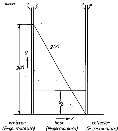
Fig. 5. To explain the essential principle of transistor action, the concentration of only the minority charge carriers g(x) in the base of a junction transistor is given as function of position x . G_b represents the equilibrium concentration of the minority charge carriers in the base.
