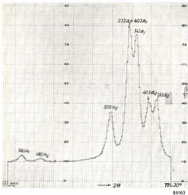
Fig. 2. Chart of diffraction pattern recorded by the "Norelco" counting-rate computer. The Bragg angle steps in this instance are 0.02^\circ (2\theta) ; the statistical error \epsilon_{50} of each point is 0.8\% . This recording took about 3 hours of completely automatic operation.
