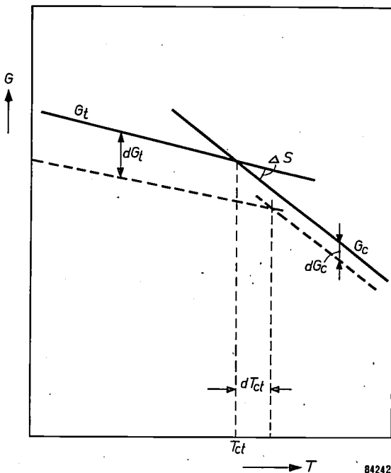
Fig. 2. Variation of the Gibbs free energy G with the temperature T (schematic) for cubic \text{BaTiO}_3 ( G_c ) and for tetragonal \text{BaTiO}_3 ( G_t ). The point of intersection of these lines gives the transition temperature T_{ct} . This point is displaced if, for any reason, the lines G_c and G_t are moved over different distances dG_c and dG_t .
