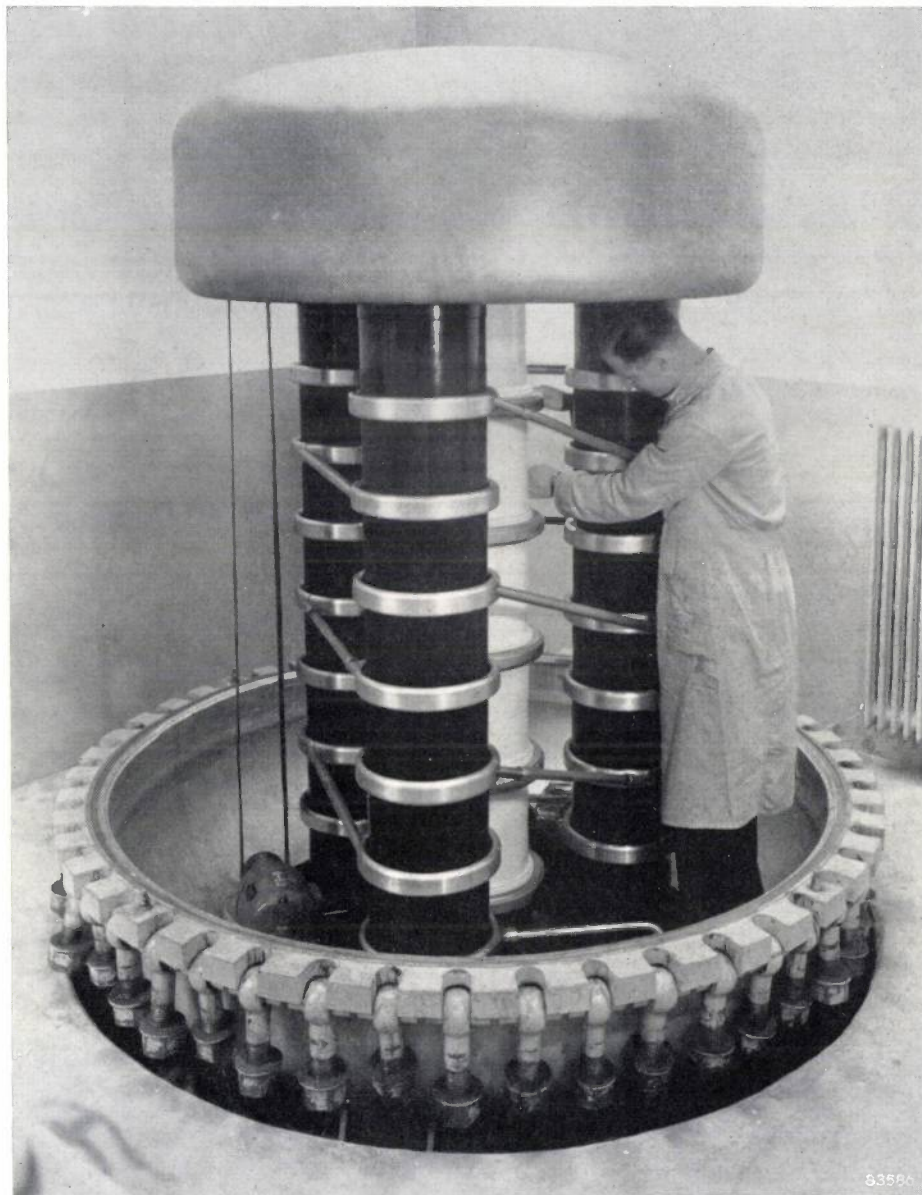
Fig. 1. 1 MeV cascade generator, arranged in three columns around the porcelain acceleration tube. Left, insulating belt which drives the dynamo for supplying the ion source and other auxiliary apparatus.
