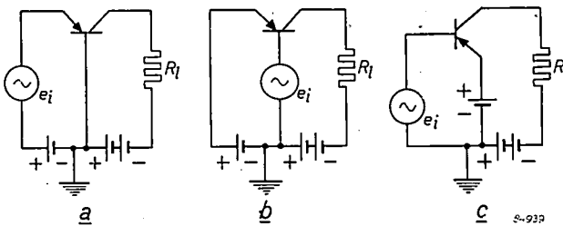
Fig. 7. a) Transistor circuit with common base. If the internal resistances of the D.C. sources are neglected, then A.C. input source e_i and load resistance R_l are both connected directly to the base lead of the transistor.
