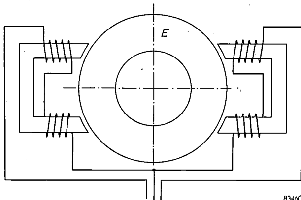
Fig. 12. Inductive displacement pick-up (cf. fig. 7) in a form suitable for measuring the eccentricity of the shaft. Here the armature consists of a disc E (of "Permenorm"), fitted on the shaft.
