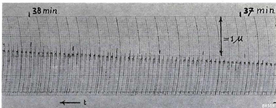
Fig. 5. Section of strip chart recording the displacement of the object during the 40 minutes in which the nickel core was heated. The displacement was measured with an inductive displacement pick-up and meter.
