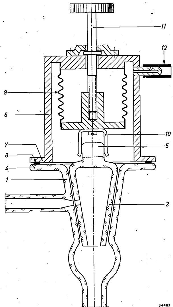
Fig. 2. New high-vacuum tap with short outgassing time. 1 tap housing with glass flange 4, 2 plug with square, solid head 5, 6 metal cap, with flange 7, carrying sealing ring 8, 9 metal bellows, 10 sprung fork, 11 adjusting screw, 12 valve. After the tap is outgassed, the cap is removed.
