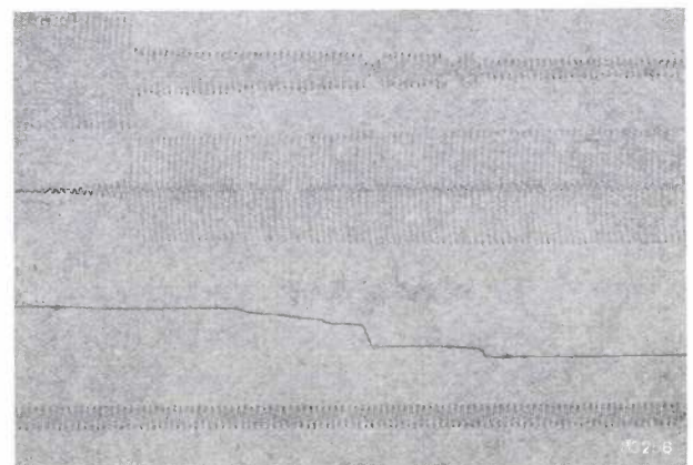
Fig. 10. As fig. 9 , but recorded during the welding of a \frac{1}{2} -inch stud with a coarse thread on the end to be welded. The stud then drops intermittently, thus producing an inferior weld. Premature melting of the screw thread is a possible cause.
