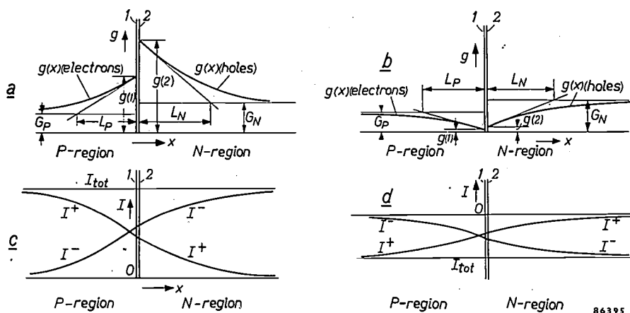
Fig. 3. Variation of the concentration g of the minority charge carriers (electrons in the P-region and holes in the N-region) at the P-N junction. The concentration gradients occurring at the boundary planes 1 and 2 of the junction can be read off the figure, after which the minority currents themselves can be written down directly. L_P and L_N are the diffusion lengths in the P and N regions respectively.
