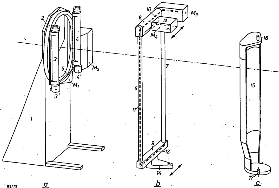
Fig. 5. The various parts of the cradle and drive. a) Base 1 of the diagnostic unit, with electric motor M_1 to drive the rotating ring of the large ball bearing 2; cylindrical slides 3 and 4, and electric motor M_2 to drive the pinions in the end-pieces 3' and 4'; 5 coupling spindle. b) Frame, with long tubes 6 and 7 fitted with racks and supported by slides 3 and 4; 8 and 9 lateral tubes; M_3 electric motor to drive the head and foot members 13 and 14 through spindles 10, 11 and 12 and thus move the cradle and patient laterally. c) Cradle 15, with short spindles 16 and 17 fitting into bearings in the head and foot members 13 and 14; spindle 16 is driven by another electric motor ( M_4 , in b) to rotate the patient about his longitudinal axis.
