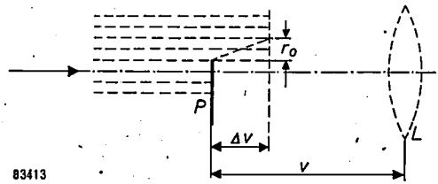
83413 Fig. 5. Illustration of the diffraction blur, \delta_b . A parallel electron beam falls on an opaque object P from the left. The "shadow" which the object throws on the real object plane at a distance \Delta v , is sharply reproduced on the fluorescent screen by the lens L . The shadow itself is not sharp as a result of diffraction of the electron rays at the edge of the object.
