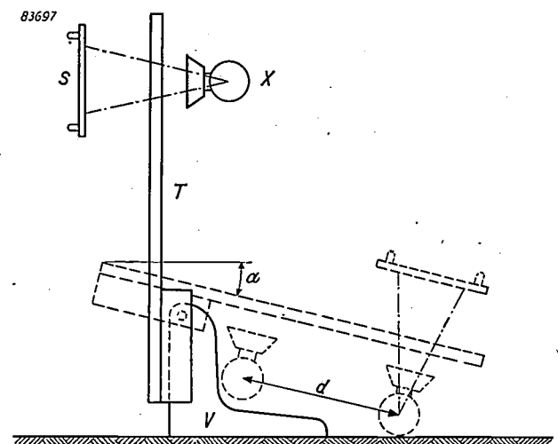
Fig. 2. Diagram of the Philips "Diagnost". The table ( T ) pivots on a spindle at the top of the central base ( V ). When the table is swung from the vertical to the horizontal position and beyond it (Trendelenburg position), there is a risk of the X-ray tube coming in contact with the floor; hence it is necessary, even for relatively small Trendelenburg angles ( a ), to fix the axis of rotation relatively high above the floor. Moreover, owing to the presence of the central base containing the spindle, the X-ray tube can be moved only a short distance ( d ) along the table.
