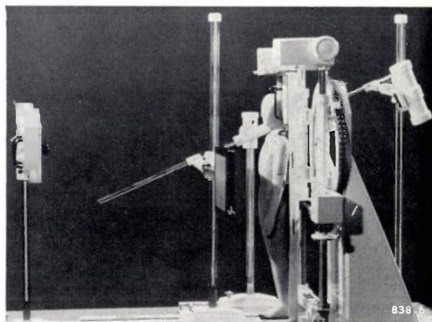
Fig. 10. Model of the UGX diagnostic unit as set-up for planigraphy. The fluorescent screen is not required; it is moved away to make room for a film cassette mounted on a separate stand and connected to the X-ray tube by a coupling rod.
