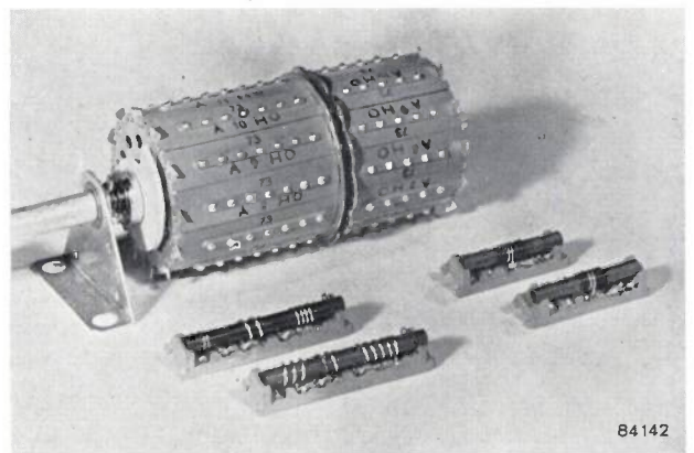
Fig. 3. a) High frequency stage incorporating channel selector (opened) as used in Philips television receivers. PCC 84 H.F. tube, PCF 80 first oscillator and frequency changer (both in screening cans). T rotating drum — shown separately in (b) — and the alternative coils. Each set of coils is mounted on an insulated block with contacts. In the foregrounds some of the coils are shown separately; in (a) from the contact side, in (b) from the coil side.
