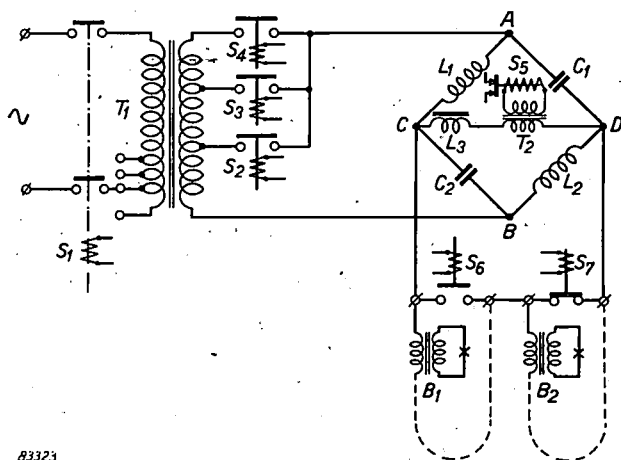
Fig. 6. Simplified circuit diagram of a low power supply unit. S_1 main switch; T_1 isolating transformer; S_2, S_3, S_4 luminous intensity selectors (varying in number from 0 to 5); ACBDA Boucherot bridge; L_3 choke to limit the output voltage when the runway circuit is interrupted; T_2 current transformer; S_5 relay, which, when energised, opens mains switch S_1 ; B_1, B_2 runway light circuits; S_6, S_7 runway selectors.
