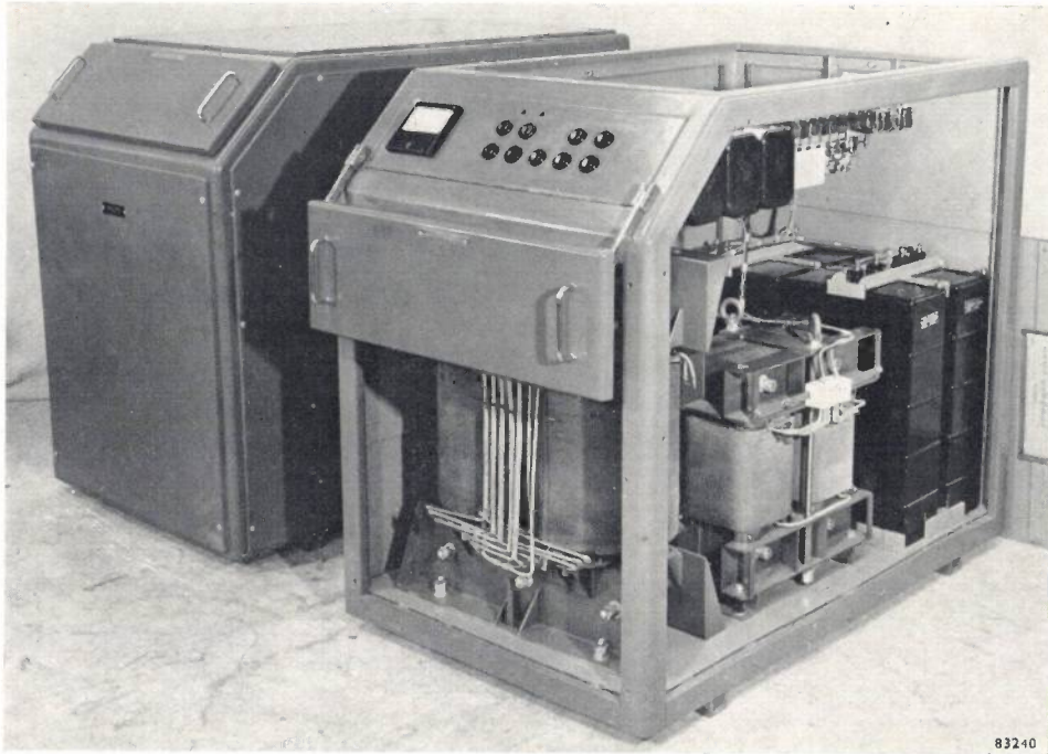
Fig. 10. Two 25 kVA, 20 A supply units, the one on the right with the cover open and the front and sides removed. Note the ammeter and the push buttons on the sloping panel. The isolating transformer, one of the bridge-arm coils and the capacitors can be seen at the bottom, and the magnetic switches at the top of the unit.
