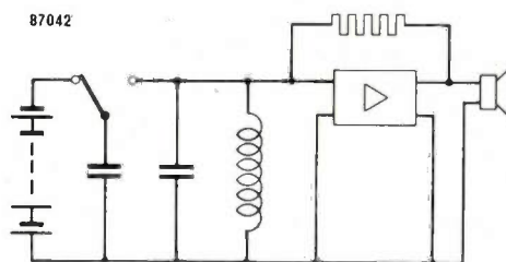
Fig. 2. Circuit diagram of the electronic bass drum.
