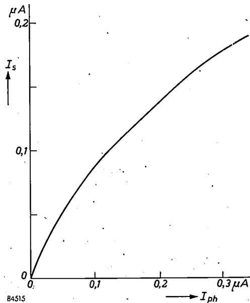
Fig. 4. Signal current I_s plotted against photo-current I_{ph} for image iconoscope 5854.
