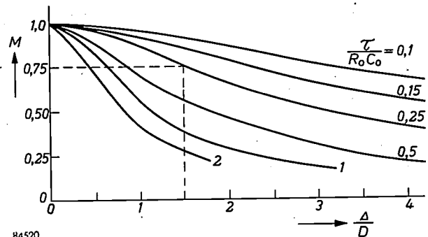
Fig. 10. Relative modulation depth M of the potential pattern on the target, plotted against \Delta/D ( \Delta = thickness of target, D = width of bands in a picture comprising black and white bands), for various values of \tau/R_0C_0 . With \tau/R_0C_0 = 0.25 , \Delta/D must not exceed roughly 1.5 if the modulation depth is to be maintained at a reasonable value.
