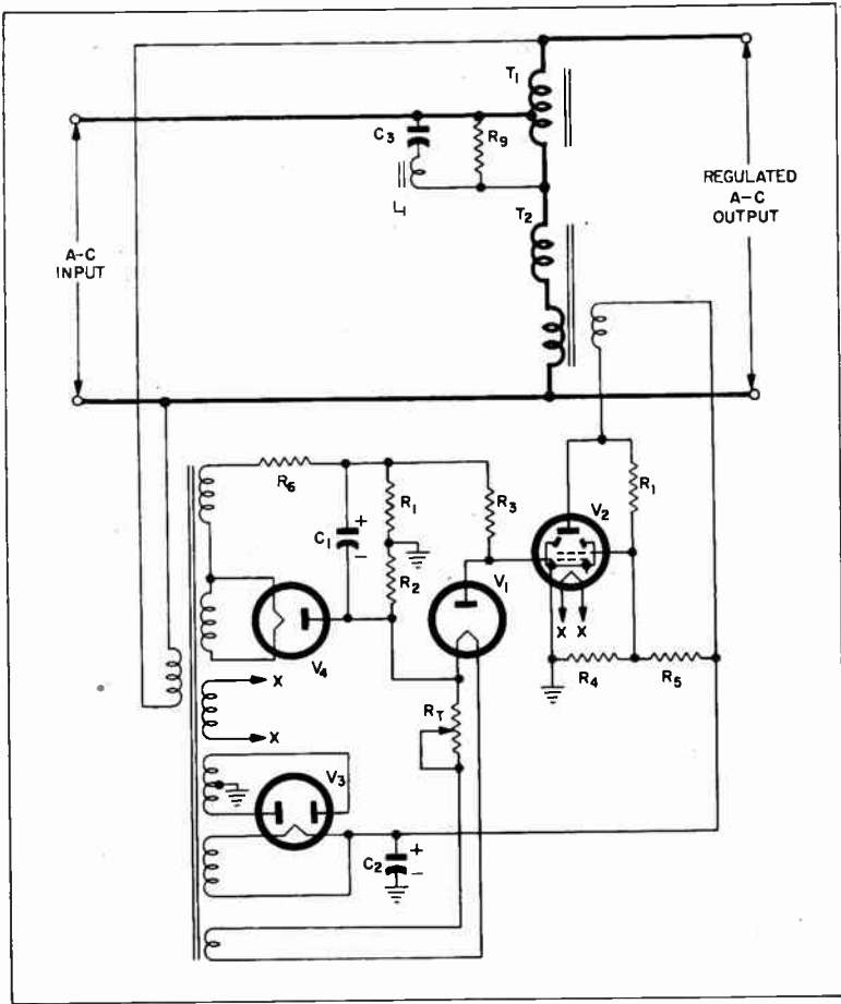
Figure 1. A-C Voltage Regulator Utilizing Saturable-Core Reactor as Regulating Element
