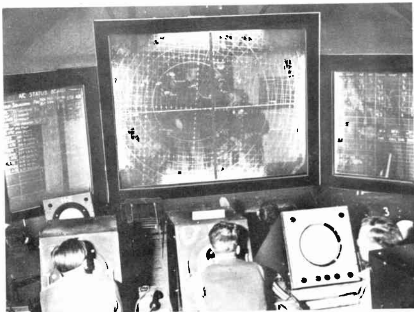
Figure 8. Vertical Plotting Board of MEW, and Remoted Height-Finder Scopes (H-1 and H-2)
