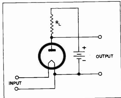
Figure 3. Basic Diode-Amplifier Circuit
