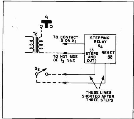
Figure 4. Method of Connecting a Three-Cycle Cutout to Arc Breaker
