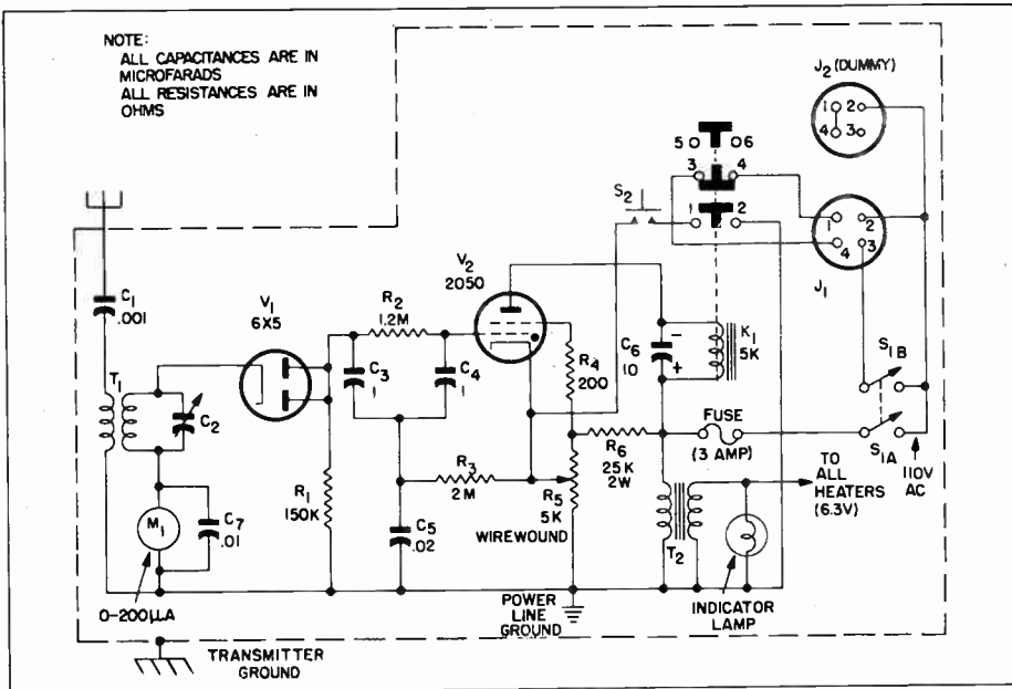
Figure 1. Schematic Diagram of Arc Breaker
