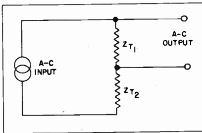
Figure 2. Simplified Equivalent Circuit of Figure 1, Showing Effective Impedances Involved in Regulator Action
