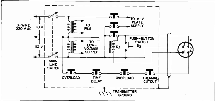
Figure 2. Schematic Diagram of Transmitter Control Circuits
