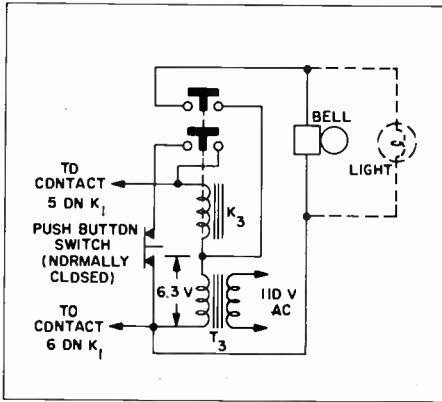
Figure 3. Schematic Diagram of Personnel Alarm
