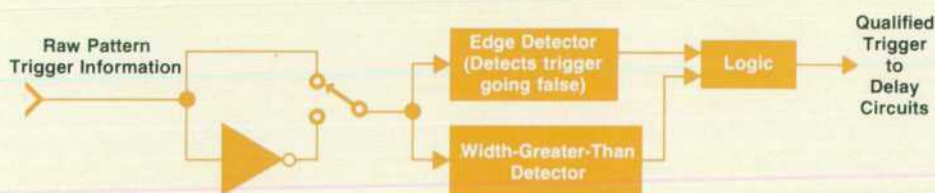
Fig. 8. Organization of time-duration triggering circuitry.
