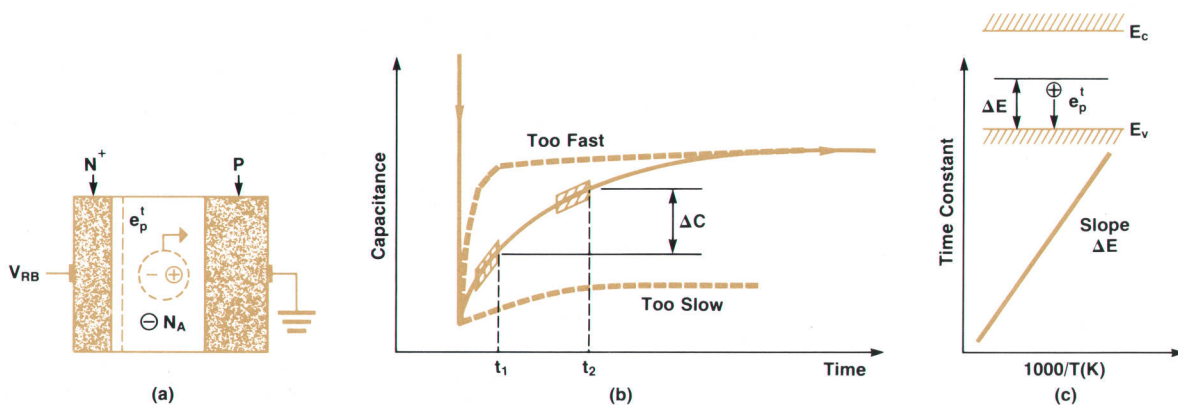
Fig. 2. Principles of capacitance DLTS. (a) Emission of carriers in N + P junction is stimulated by applying bias or infrared radiation. (b) Capacitance transient results when junction is reverse biased. LCR meter measures junction capacitance at two gated time periods. Maximum capacitance change \Delta C occurs at a temperature (i.e., time constant) that is characteristic of the type of defect. (c) Temperature dependence of capacitance time constant.
