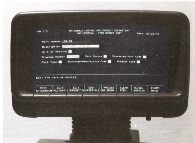
Fig. 1. Eight keys under the HP 250 CRT display can be defined differently in different applications programs to allow the operator to select various functions. The functions appear on the CRT above the keys. Also shown here is an example of a form in which data entry and display are programmed using standard INPUT, ENTER, and DISP statements.
