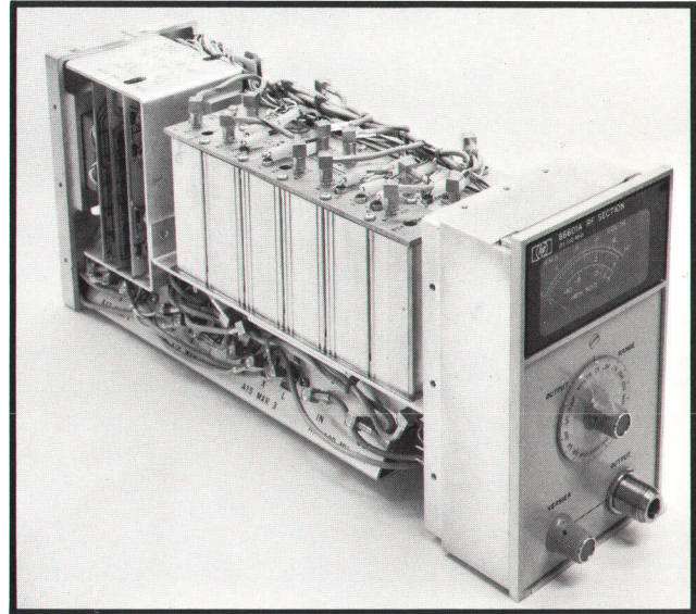
Fig. 8. Each electrical and mechanical assembly of 86601A RF Unit is individually removable.
