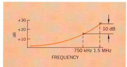
Fig. 6. Typical reproduce system response illustrates how distortion harmonics are accentuated relative to their fundamental.
