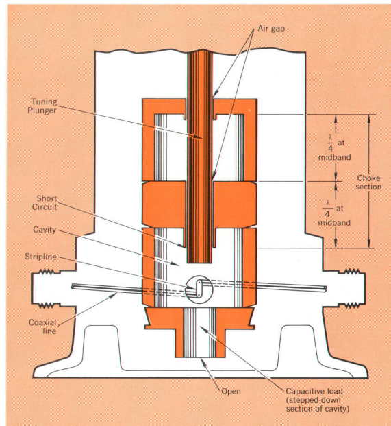
Fig. 4. Simplified cross-sectional view of Model 536A Frequency Meter. Cavity is tuned by moving plunger up and down. Choke section produces excellent short circuit between plunger and cavity walls at point indicated. Model 537A cavity is similar, but uses contacting fingers instead of choke section to produce sliding short.
