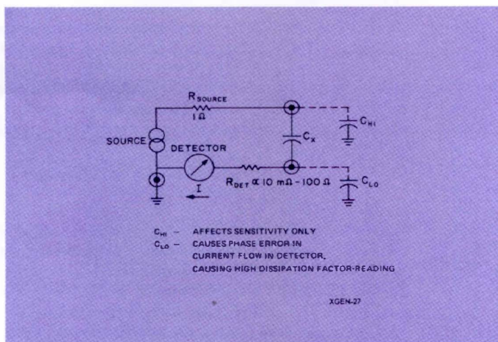
Figure 6. Three-terminal measurement of capacitance.
