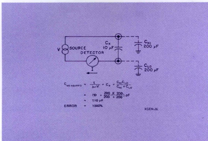
Figure 5. Two-terminal measurement of capacitance.
