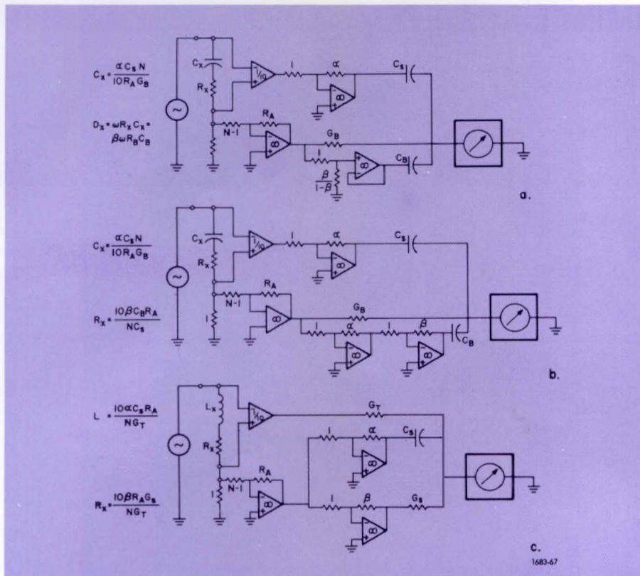
Figure 3. Simplified bridge circuits.
