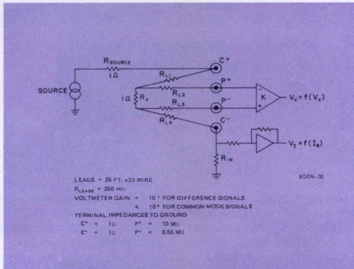
Figure 9. Five-terminal measurement of resistor 25 feet from GR 1683.
