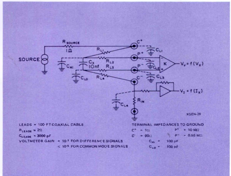
Figure 8. Five-terminal measurement of capacitor 100 feet from GR 1683.
