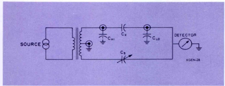
Figure 7. Three-terminal ratio-transformer bridge circuit.
