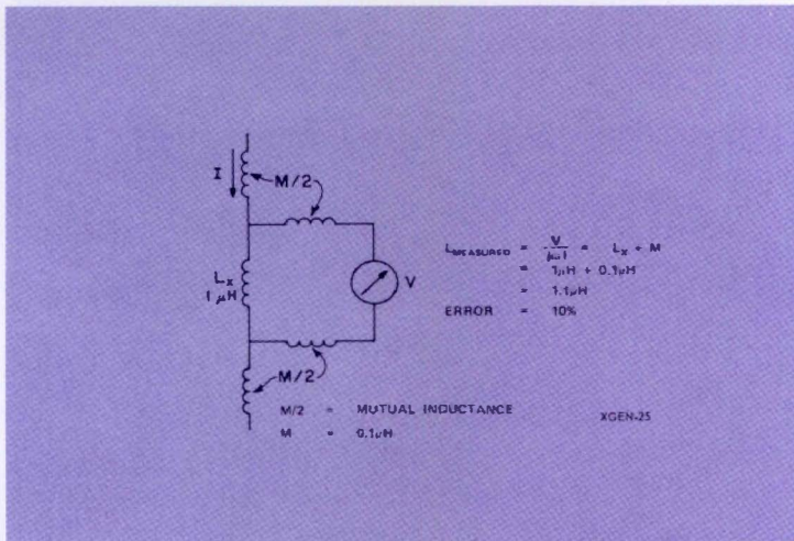
Figure 4. Degradation of inductance measurement by mutual inductance.
