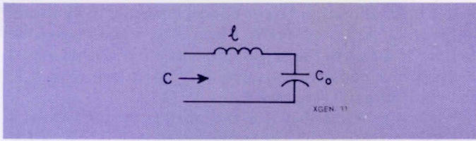
Figure 1. Simple equivalent circuit for two-terminal air capacitor.
