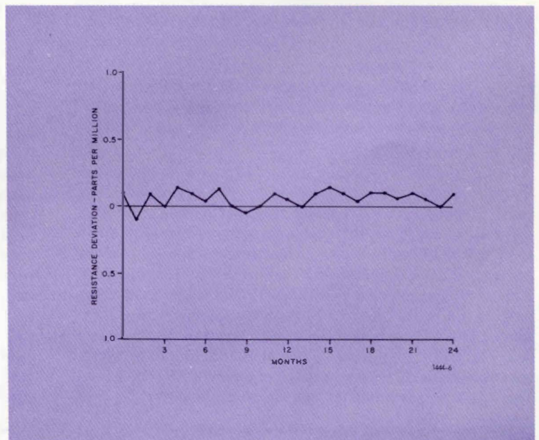
Figure 1. Typical long-term stability of GR 1444 resistors.
