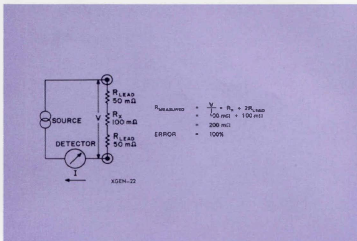
Figure 1. Effect of lead impedance on accuracy of resistance measurement.
