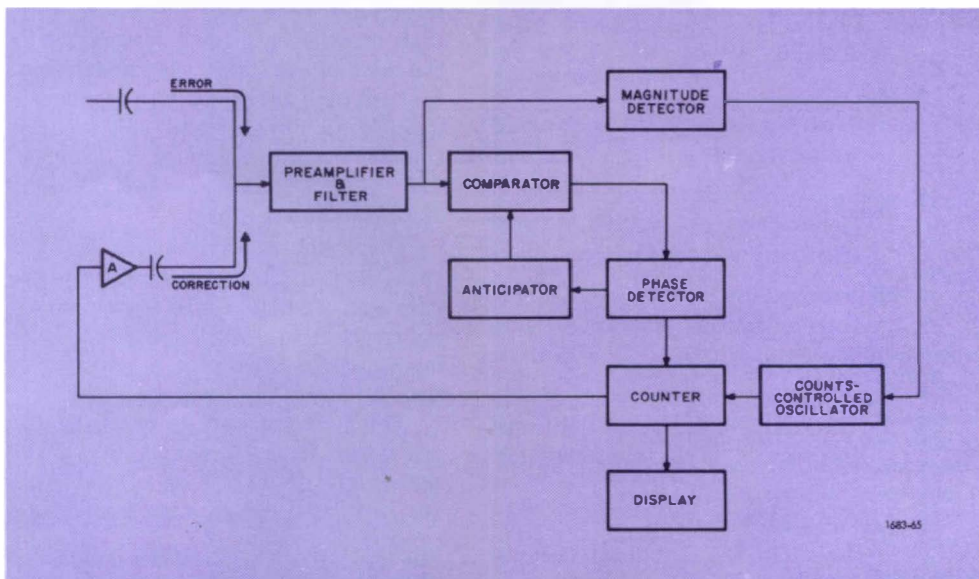
Figure 1. GR 1683 balancing technique.
