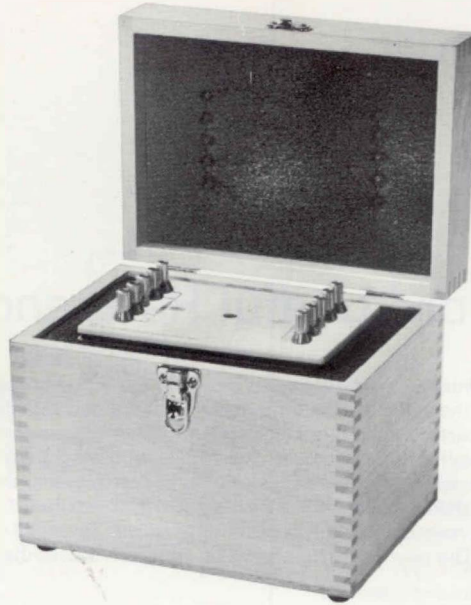
1444-A 10-k \Omega standard with temperature sensor, shown with carrying case.
