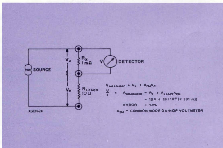
Figure 3. Effect of non-infinite common-mode rejection.
