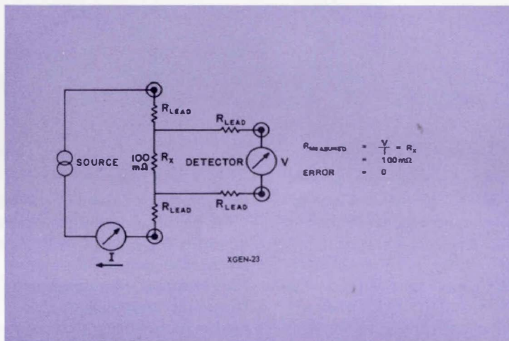
Figure 2. Four-terminal resistance measurement.
