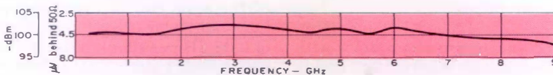
Figure 3. Typical sensitivity curve for receiver system comprising 1236, local oscillator, and Type 874-MRAL Mixer.
