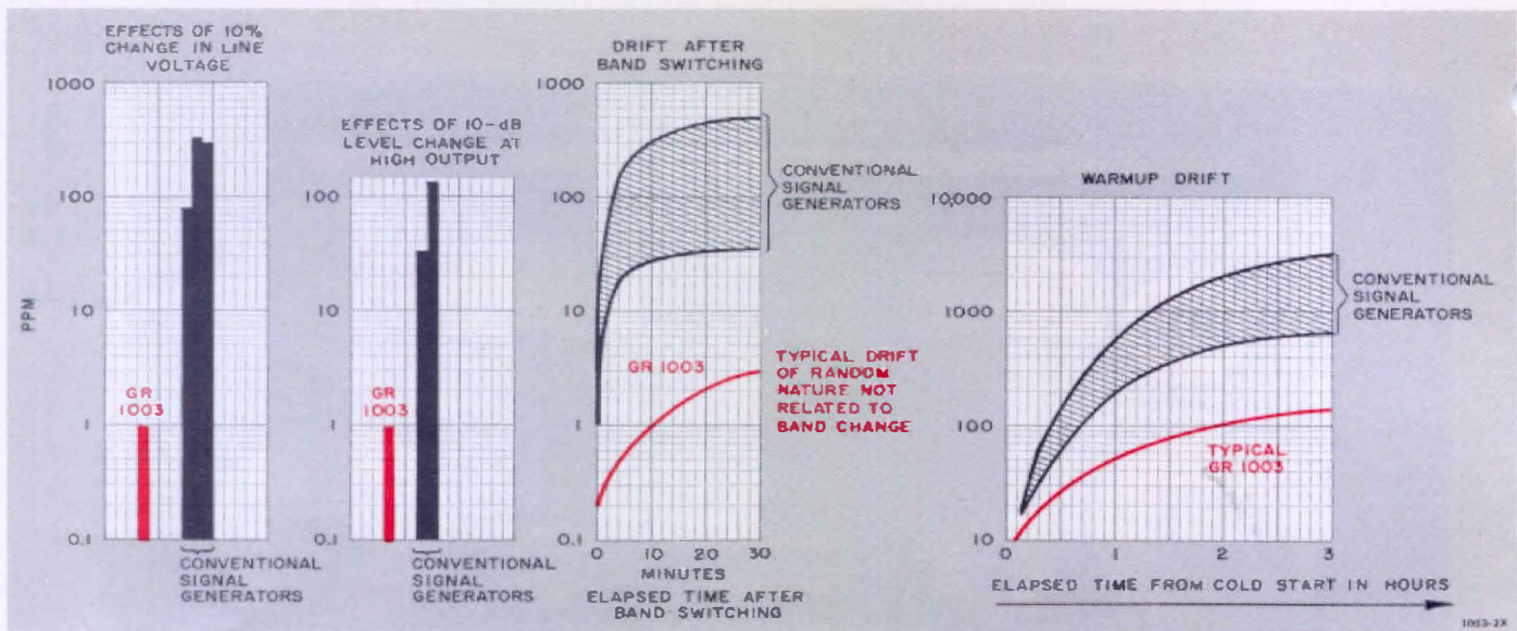
Figure 2. The stability of the 1003 compared with that of typical other signal generators.
