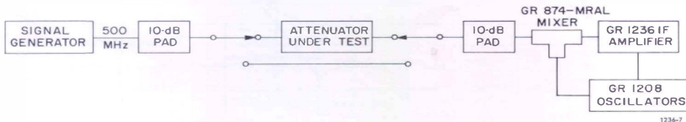
Figure 7. Setup for attenuation measurement described in text.
