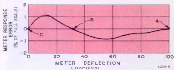
Figure 6. Measured deviation of compensated detector circuit from linear response.
