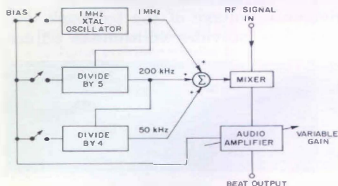
Figure 7. Elementary diagram of the crystal calibrator.
