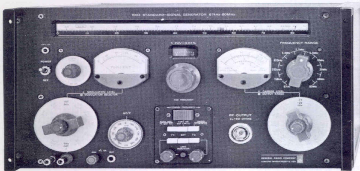
Figure 1. Type 1003 Standard-Signal Generator.
