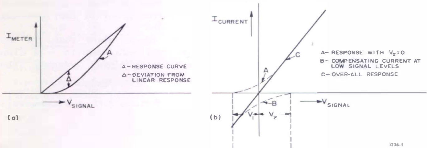
Figure 5. Uncompensated (left) and compensated (right) response of detector circuit.
