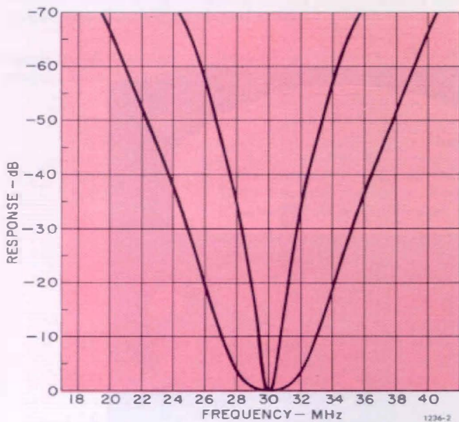
Figure 2. Narrow- and wide-band response characteristics of the 1236.
