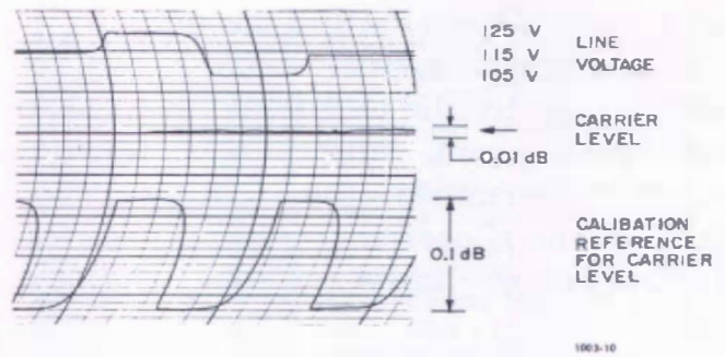
Figure 4. Effects of \pm 10\% line-voltage swing on carrier level.
