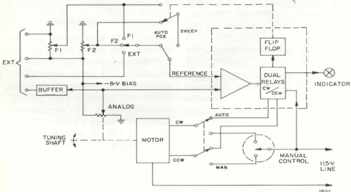
Figure 8. Elementary diagram of the auto-control unit.
