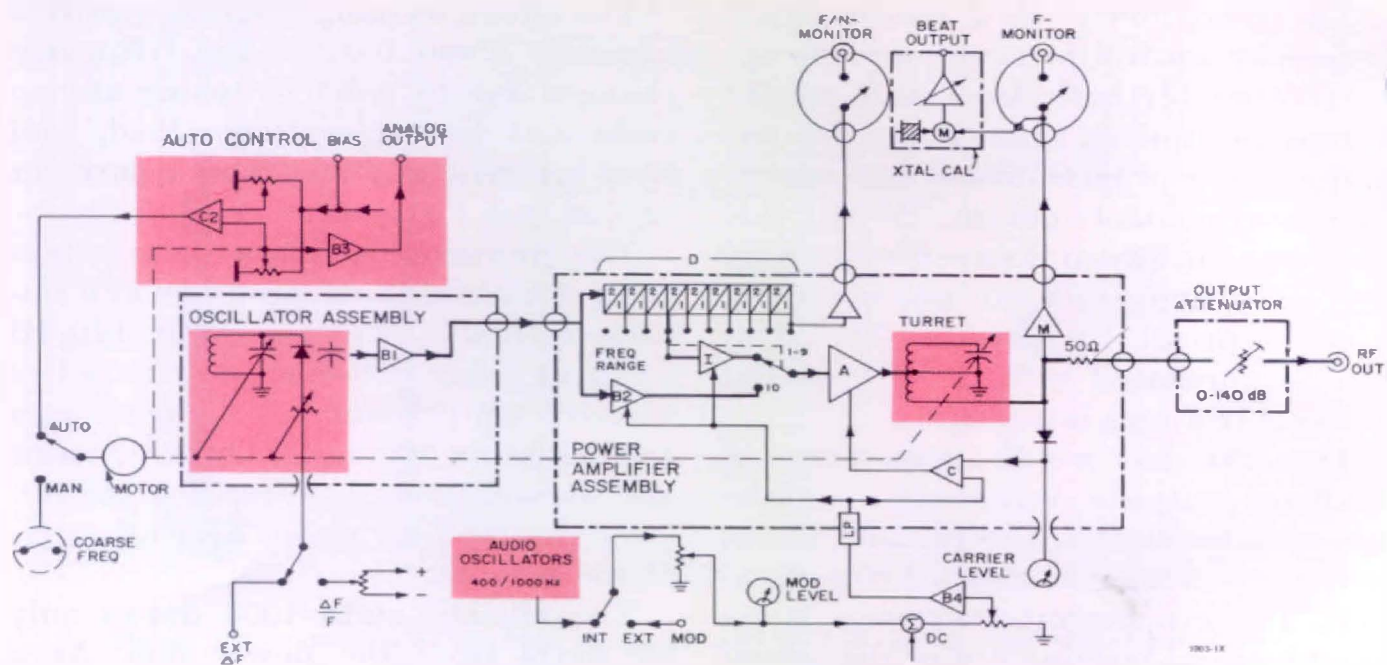
Figure 3. Elementary block diagram.
