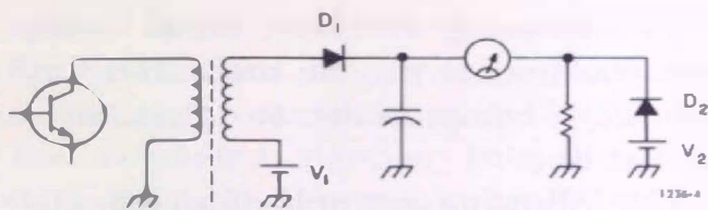
Figure 4. Elementary diagram of the detector linearizing network.
