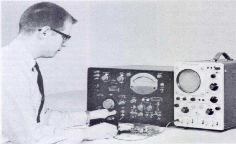
Figure 7. The Type 1309-A Oscillator and associated equipment used for testing of an audio amplifier.
