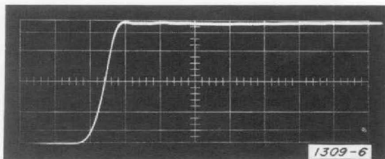
Figure 5. (Left) Leading edge of 10-kHz square wave into 50-ohm load. Horizontal scale: 50 ns/div. (Right) Direct-coupled 10-Hz square wave has flat top. Horizontal scale: 10 ms/div.
