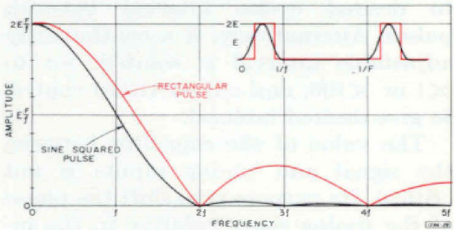
Figure 1. Spectrum envelopes of a rectangular pulse and a sine-squared pulse.
