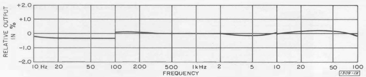
Figure 4. Typical oscillator output voltage versus frequency.
