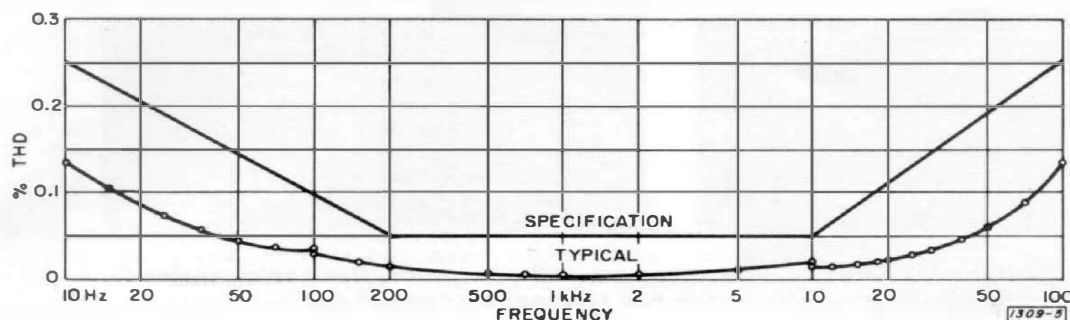
Figure 3. Oscillator distortion for 600-ohm load or open circuit.
